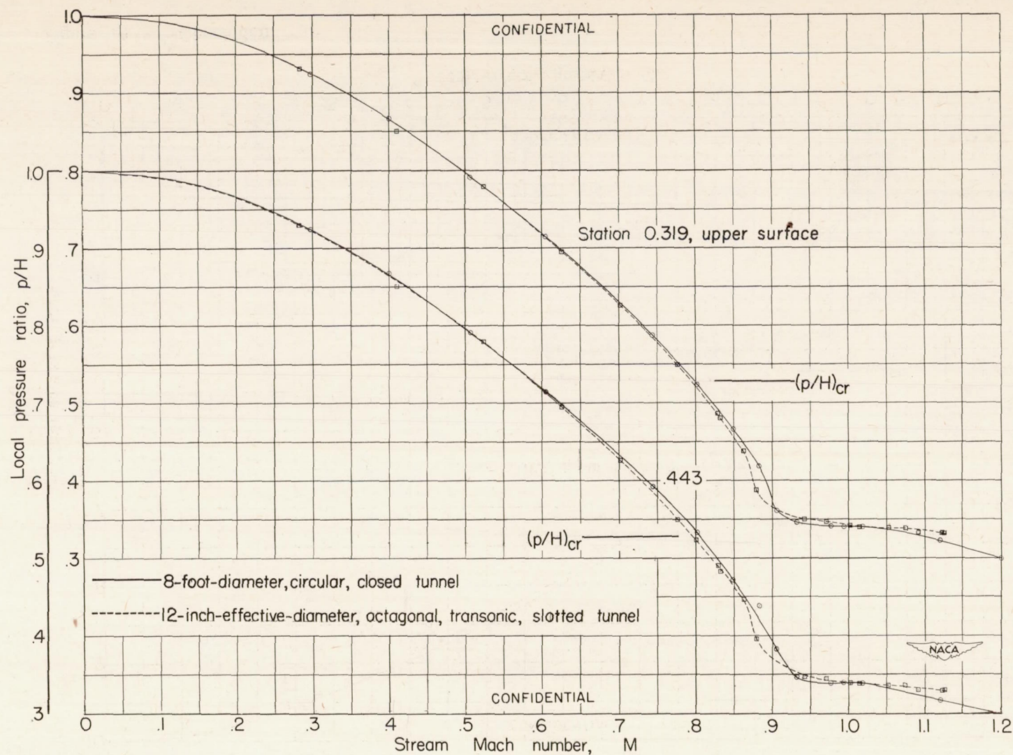
Figure 15.—Comparison of local pressures as a function of Mach number for several spanwise stations along the 50 percent chord of NACA 65-010 wing affixed symmetrically on 1\frac{1}{3} -inch-diameter prolate spheroid in the transonic slotted tunnel and in a large closed tunnel.
