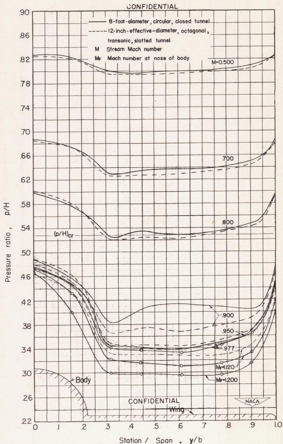
Figure 19.— Comparison of spanwise pressure distributions at 50 percent chord of NACA 65-010 wing affixed symmetrically on \frac{1}{3} -inch-diameter prolate spheroid for several Mach numbers in the transonic slotted tunnel and in a large closed tunnel.
