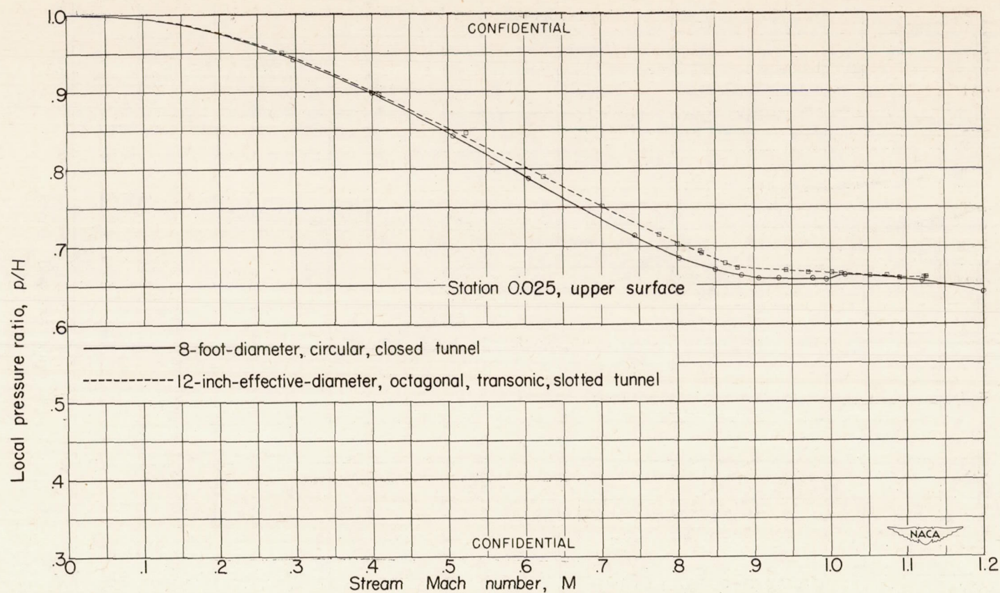
Figure 14.—Comparison of local pressures as a function of Mach number for several chordwise stations along the 50 percent semispan of NACA 65-010 wing affixed symmetrically on 1\frac{1}{3} -inch-diameter prolate spheroid in the transonic slotted tunnel and in a large closed tunnel.
