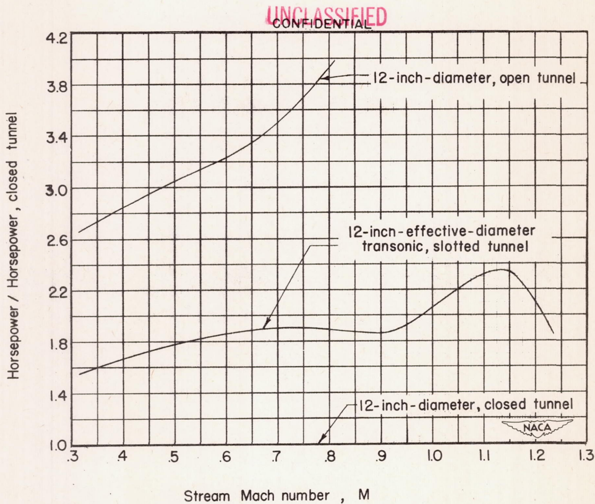
Figure 21.—Typical horsepower ratios as a function of Mach number for slotted and open tunnel configurations.
