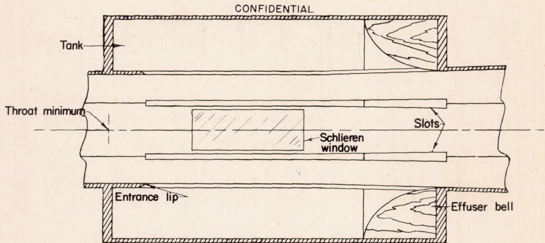
(a) Schematic diagram of transonic slotted tunnel.
