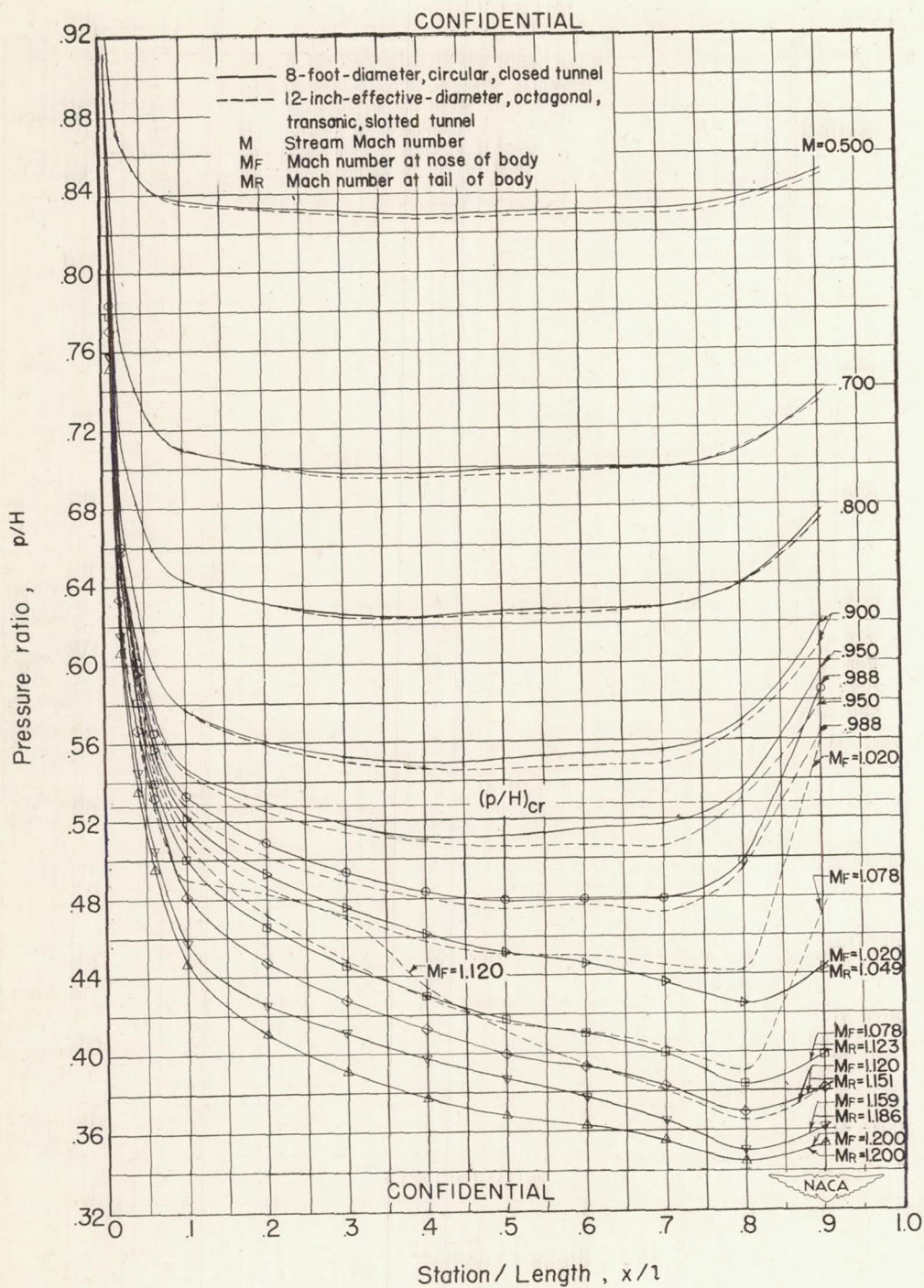
Figure 16.— Comparison of pressure distributions along top meridian of \frac{1}{3} -inch-diameter prolate spheroid for several Mach numbers in the transonic slotted tunnel and in a large closed tunnel.
