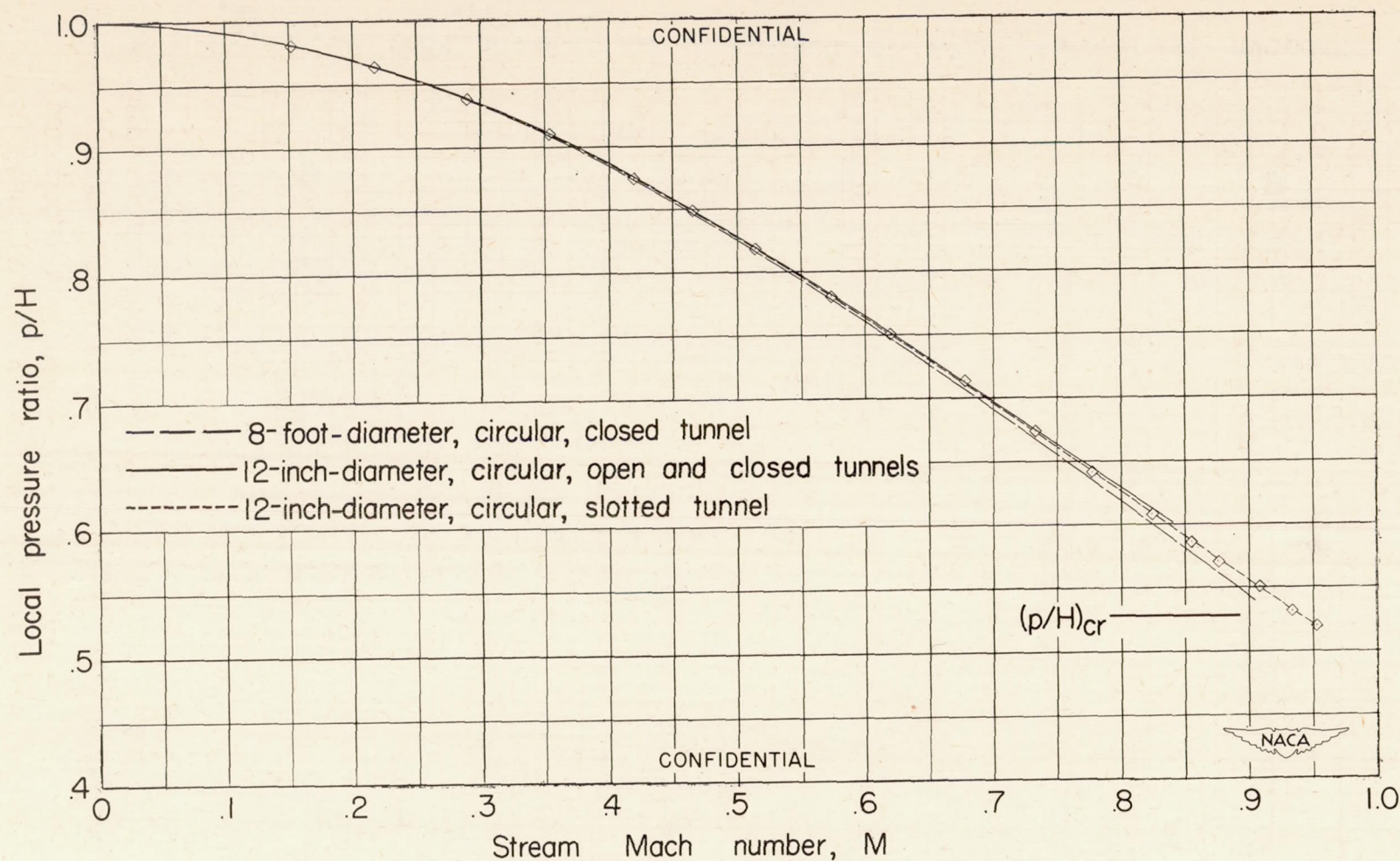
Figure 8. — Corrected local pressure as a function of Mach number at midpoint of 3\frac{1}{2} -inch-diameter prolate spheroid in circular open and closed tunnels compared with uncorrected local pressure on body in circular slotted tunnel.
