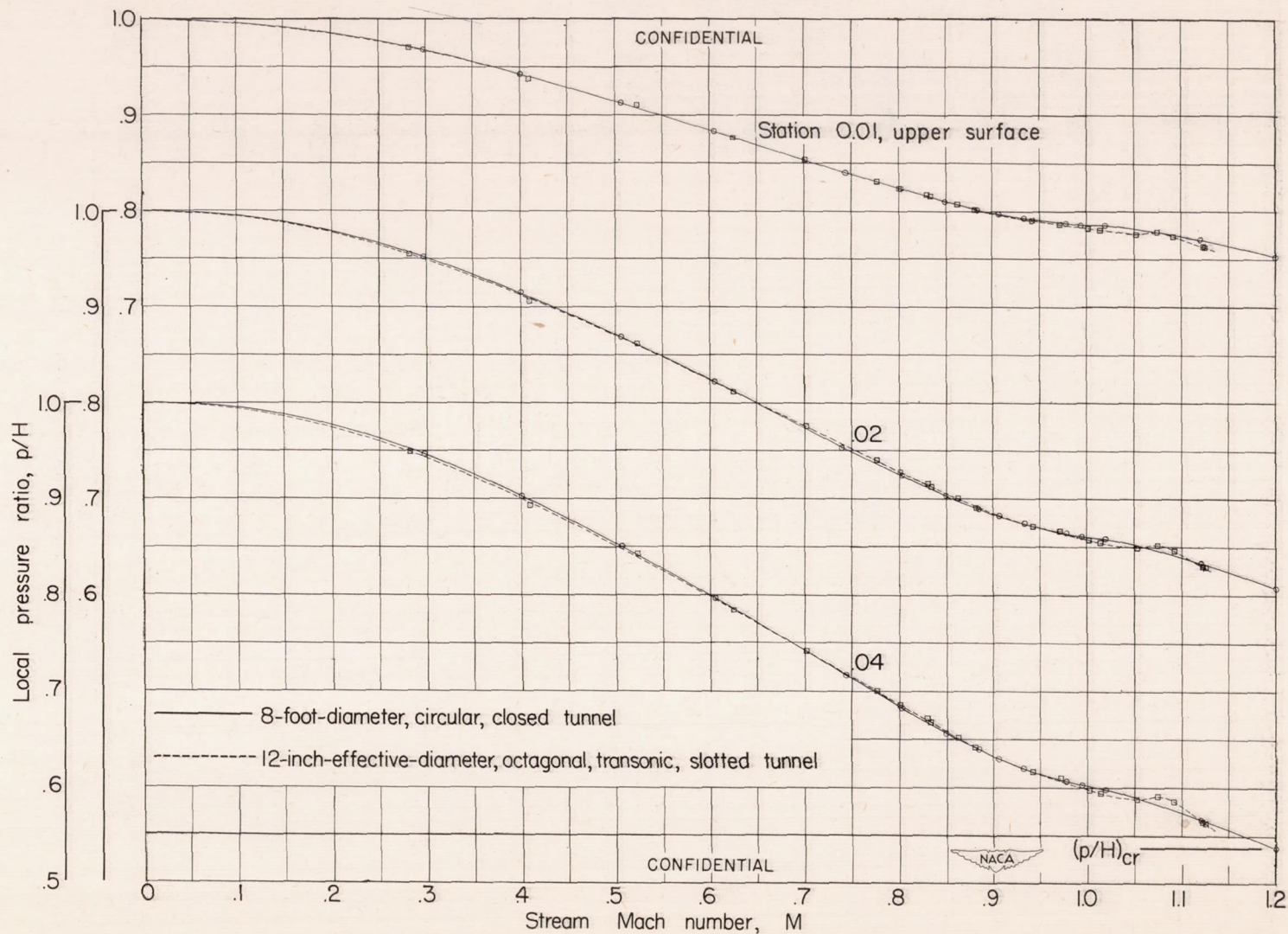
Figure 13 — Comparison of local pressures as a function of Mach number for several longitudinal stations along 1\frac{1}{3} -inch-diameter prolate spheroid, with wing affixed symmetrically, in the transonic slotted tunnel and in a large closed tunnel.
