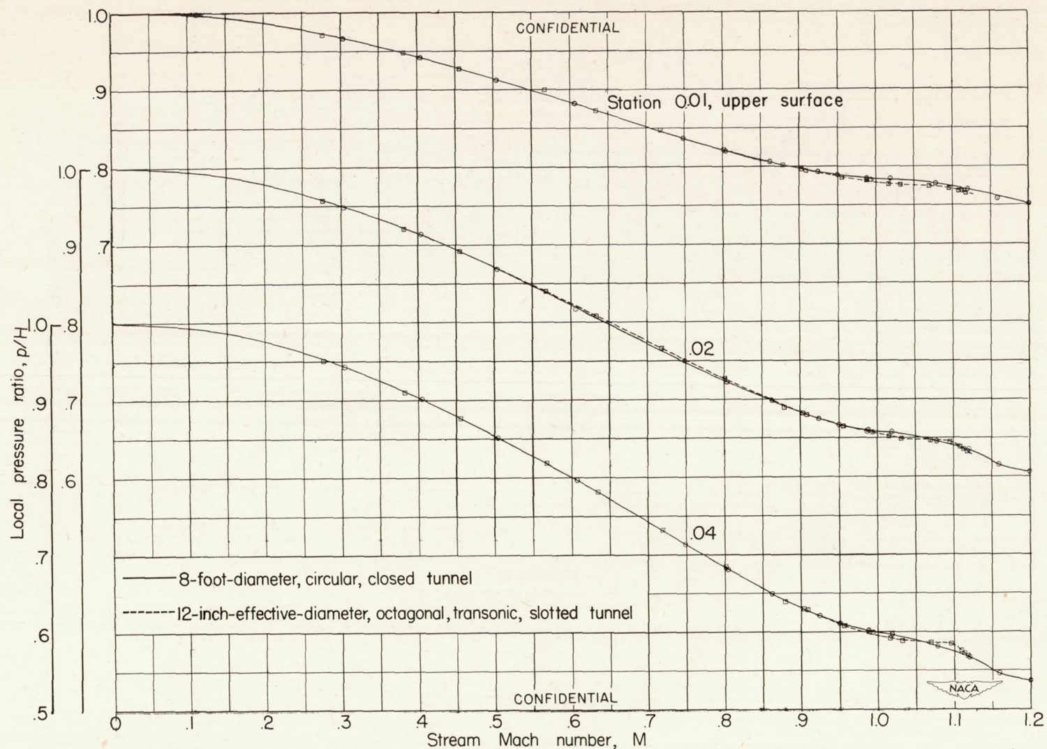
Figure 12.—Comparison of local pressures as a function of Mach number for several longitudinal stations along 1\frac{1}{3} -inch-diameter prolate spheroid in the transonic slotted tunnel and in a large closed tunnel.
