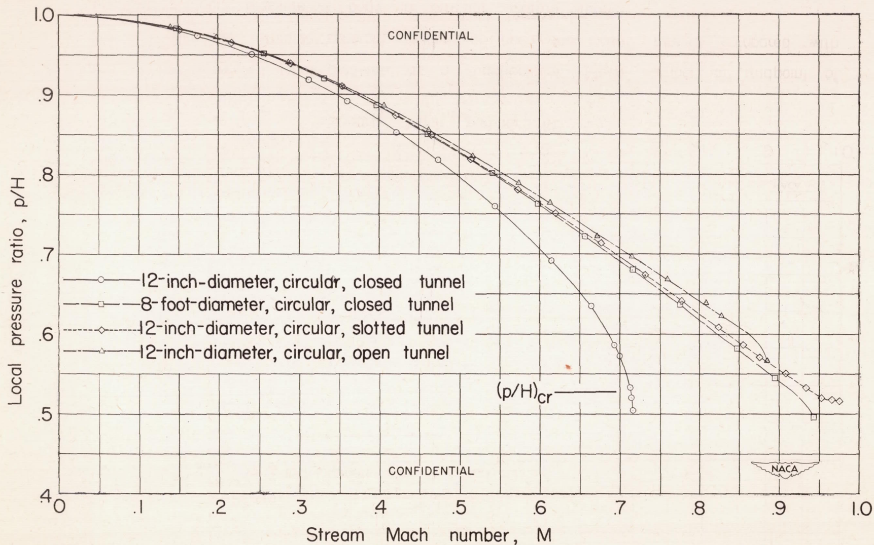
Figure 7.—Comparison of local pressure as a function of Mach number at midpoint of 3\frac{1}{2} -inch-diameter prolate spheroid in circular open, closed, and slotted tunnels.
