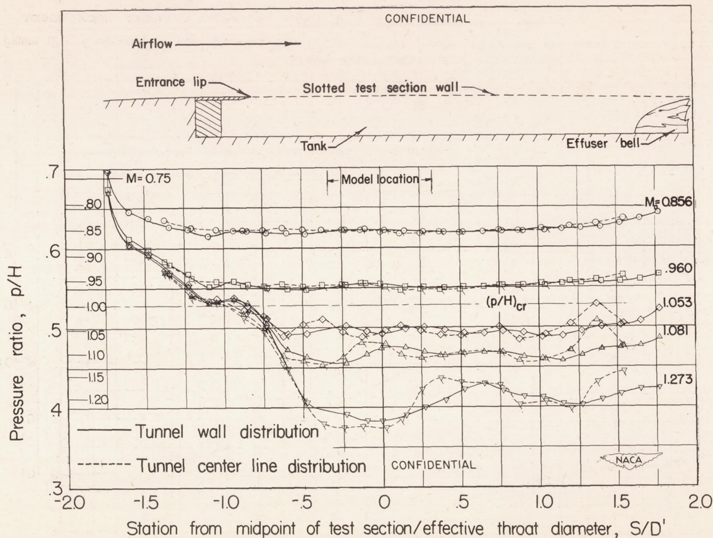
Figure 11.—Axial pressure distribution along wall and center line of 12-inch-effective-diameter, octagonal, transonic, slotted tunnel for several Mach numbers.
