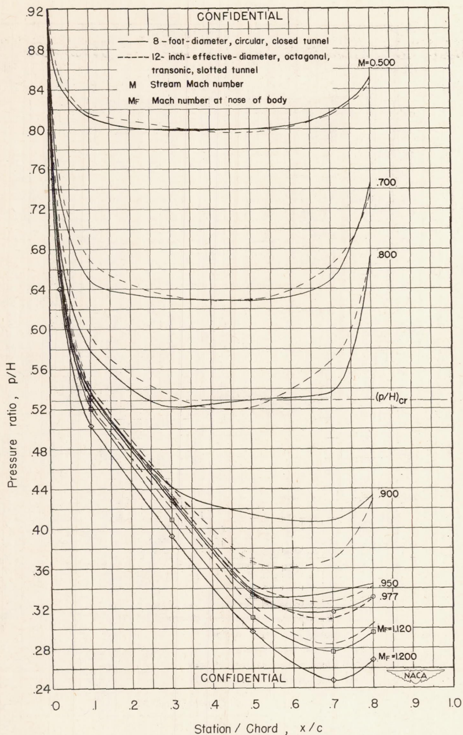
Figure 18— Comparison of chordwise pressure distributions at 61% percent semispan of NACA 65-010 wing affixed symmetrically on 1\frac{1}{3} -inch-diameter prolate spheroid, for several Mach numbers in the transonic slotted tunnel and in a large closed tunnel.
