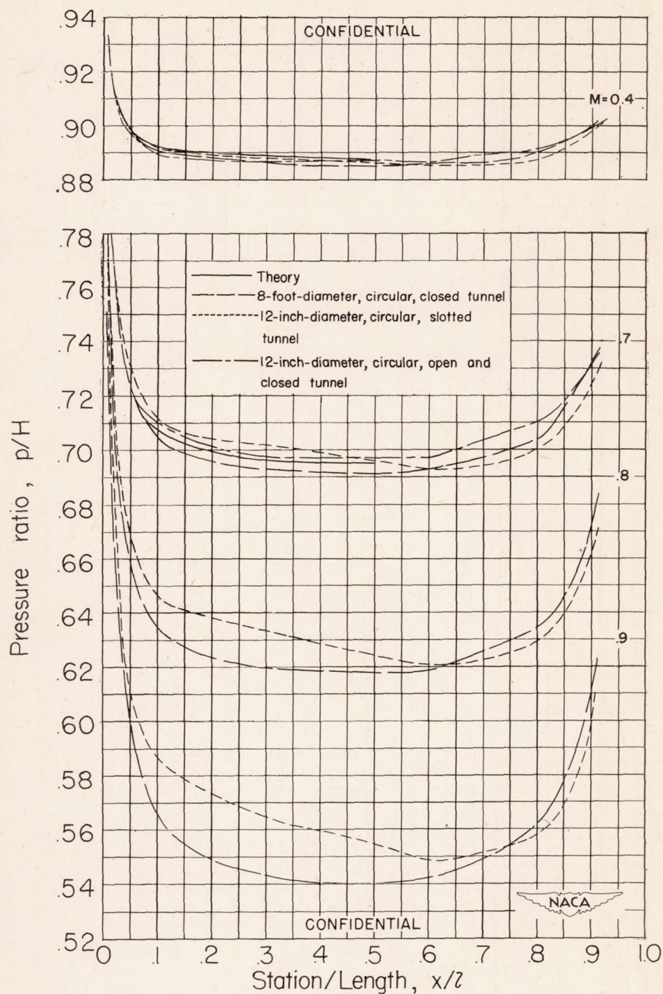
Figure 9.—Corrected pressure distributions along top meridian of 3\frac{1}{2} -inch-diameter prolate spheroid for several Mach numbers in circular open and closed tunnels compared with uncorrected pressure distributions along body in circular slotted tunnel. (Note: Vertical scale double that previously used.)
