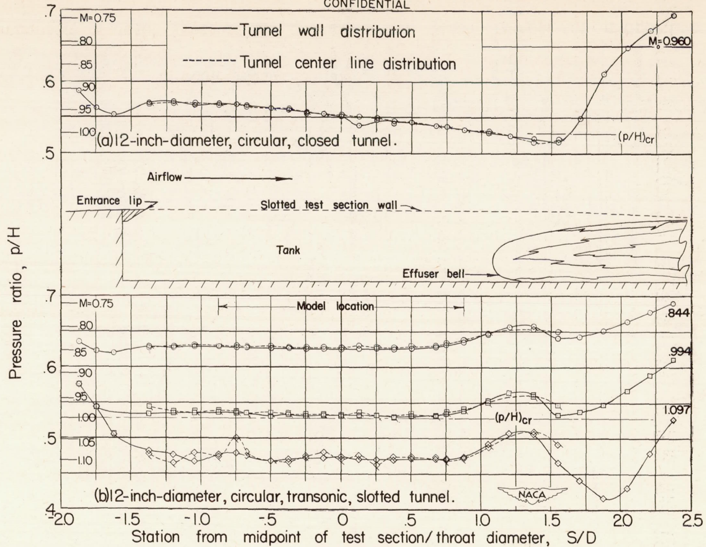
Figure 6.—Axial pressure distribution along the wall and center line of circular closed and slotted tunnels for several Mach numbers.
