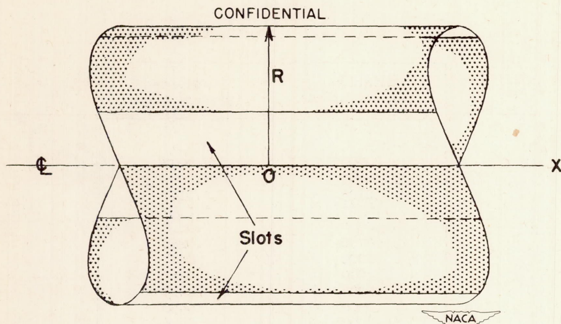
Figure 1.—Circular slotted wind tunnel configuration.
