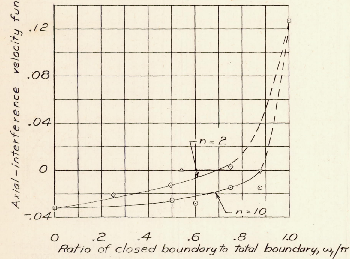
Figure 4.- Axial-interference velocity function in slotted tunnels. \rho = \xi = 0 .
