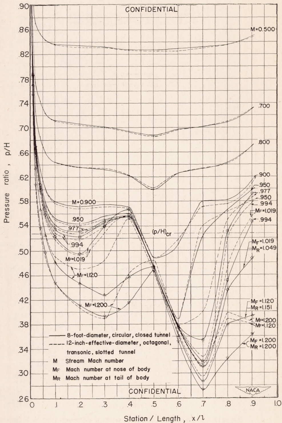
Figure 17.—Comparison of pressure distributions along top meridian of 1\frac{1}{3} -inch-diameter prolate spheroid with wing affixed symmetrically for several Mach numbers in the transonic slotted tunnel and in a large closed tunnel.
