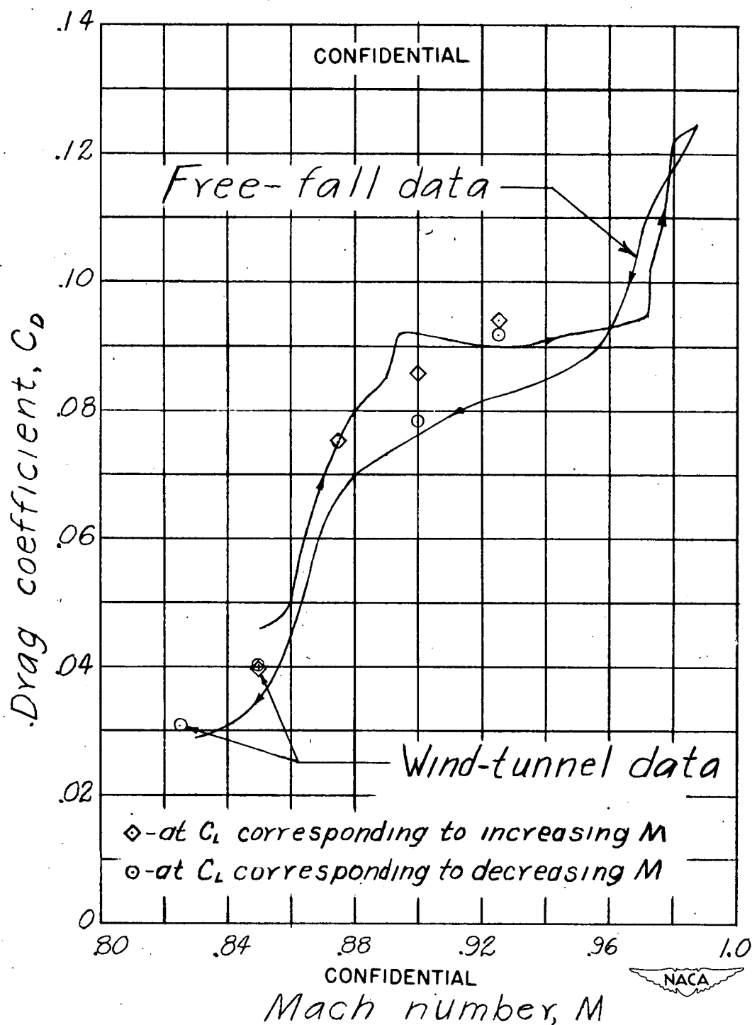
Figure 7.- Comparison of results of free-fall tests of a \frac{1}{4} -scale model of the Bell XS-1 airplane and wind-tunnel tests of a similar configuration; variation of drag coefficient with Mach number.
