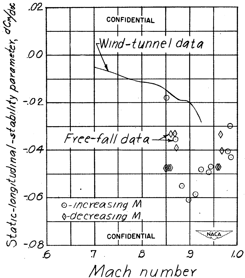
Figure 8.- Static-longitudinal-stability parameter dC_m/d\alpha for a \frac{1}{4} -scale model of the Bell XS-1 airplane.
