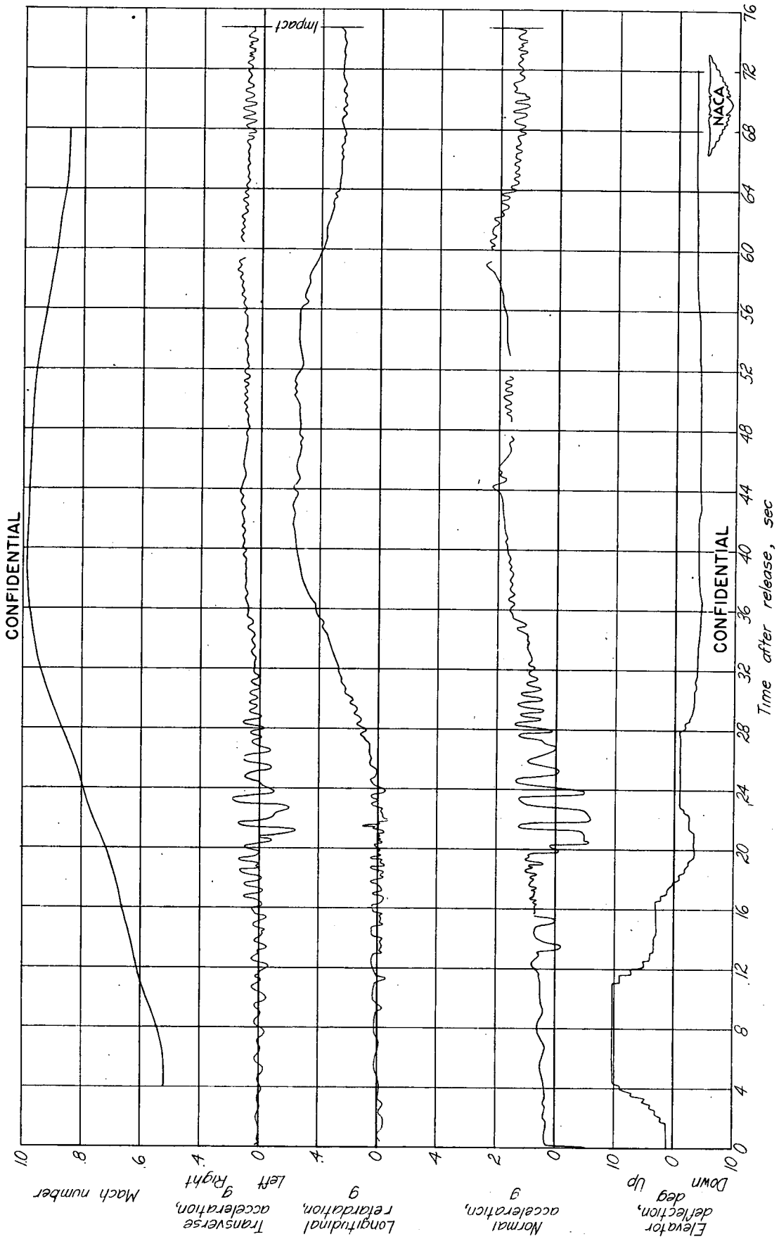
Figure 5.- Time history of free fall of \frac{1}{4} -scale model of the Bell XS-1 airplane.
