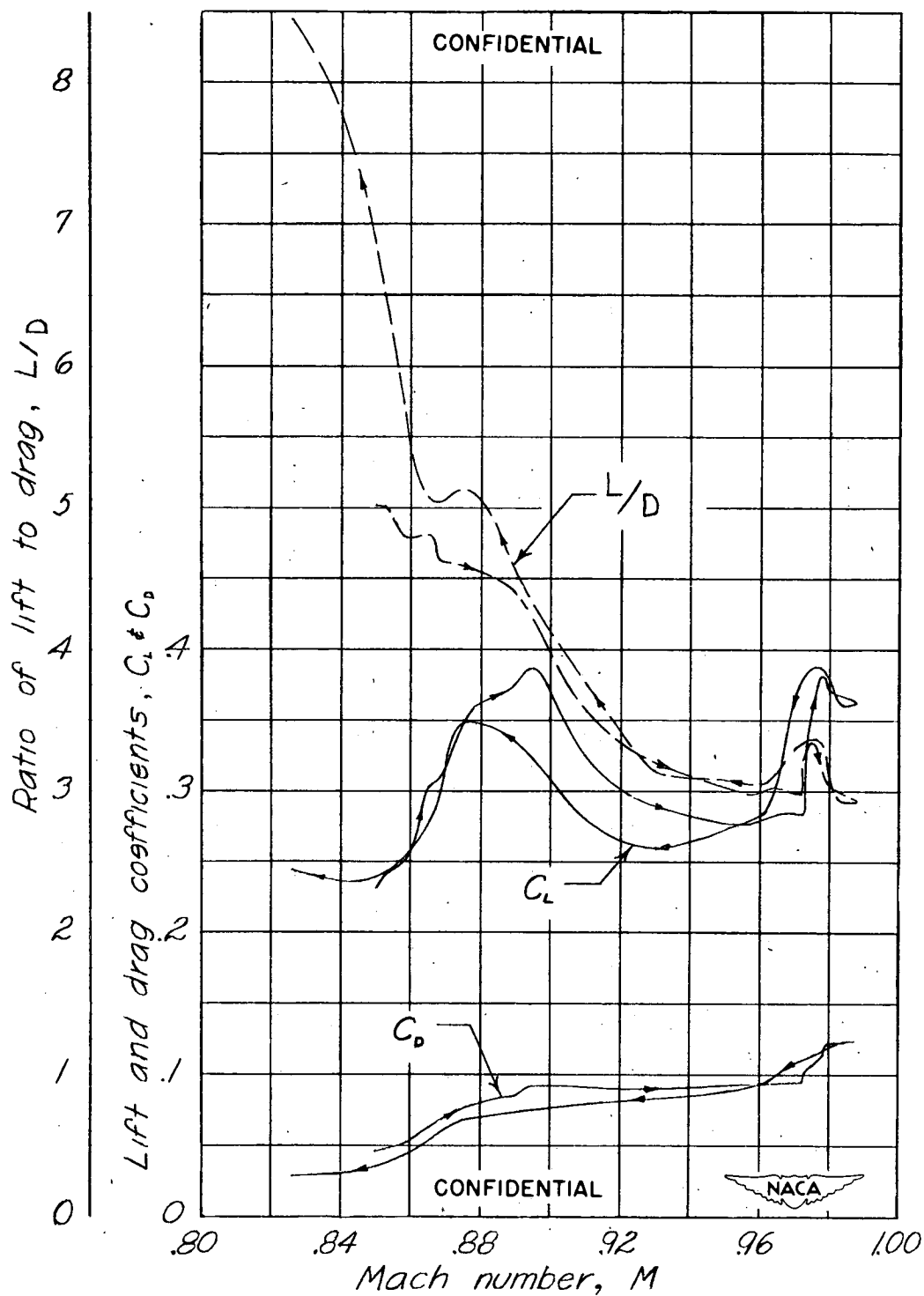
Figure 6.- Variation with Mach number of lift coefficient, drag coefficient, and lift-to-drag ratio of a \frac{1}{4} -scale model of the Bell XS-1 airplane.
