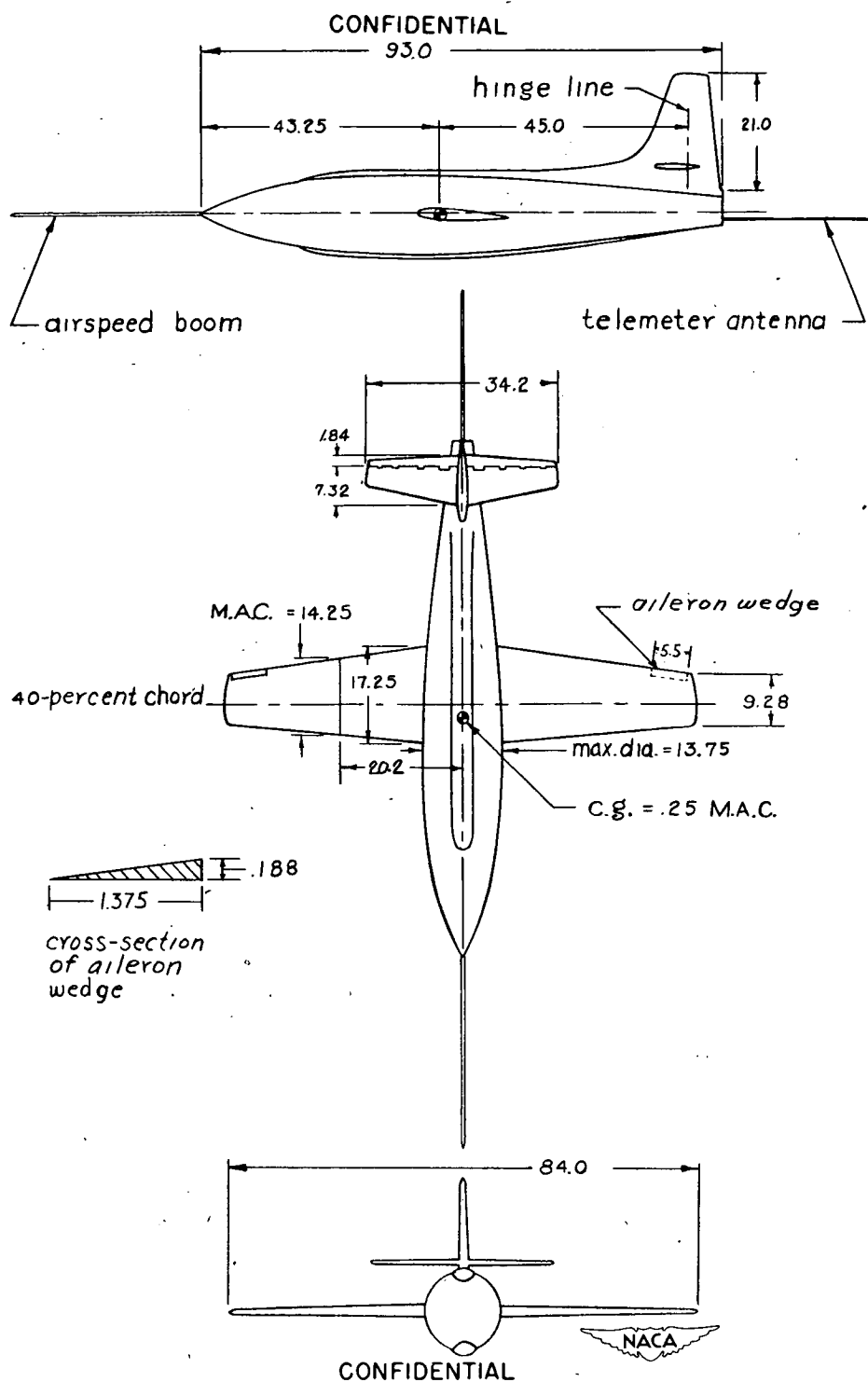
Figure 2.- Three-view drawing of \frac{1}{4} -scale model of the Bell XS-1 airplane used in free-fall test. All dimensions in inches.
