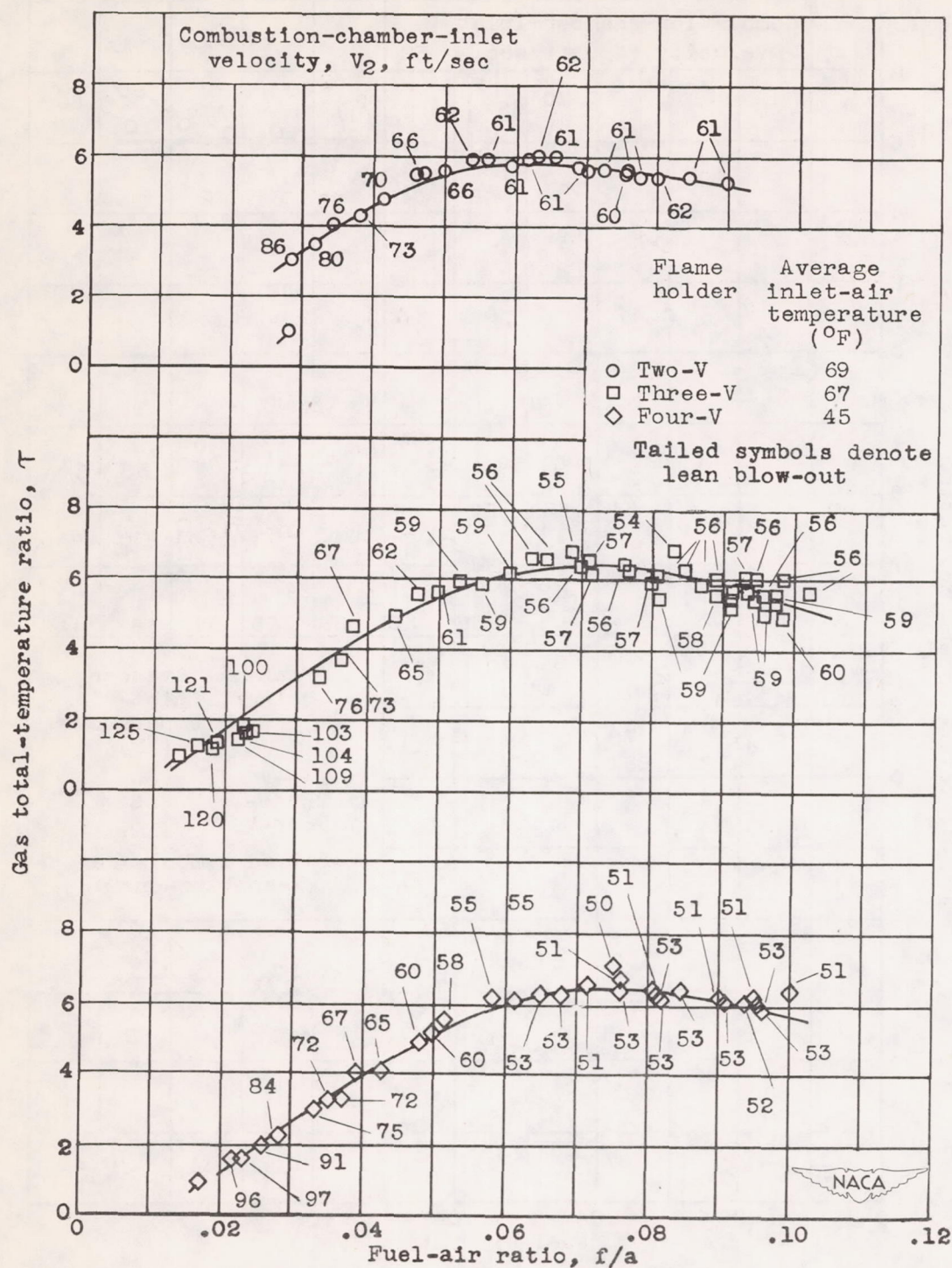
(a) Pressure altitude, 1500 feet; indicated airspeed, 200 miles per hour.
