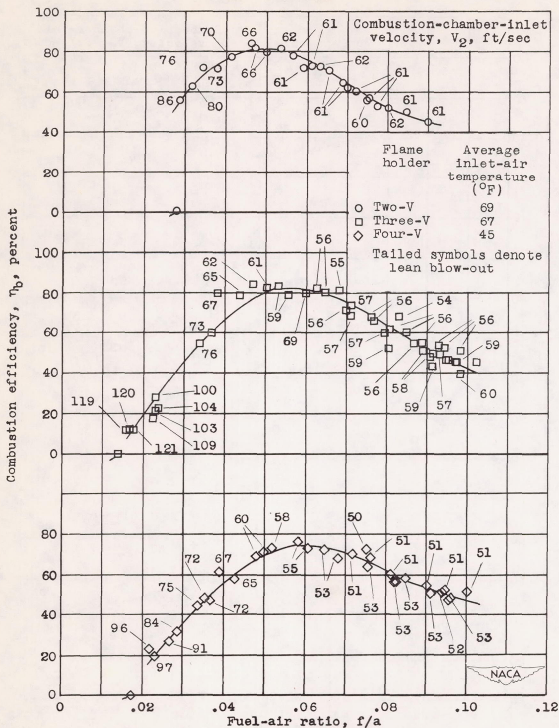
(a) Pressure altitude, 1500 feet; indicated airspeed, 200 miles per hour.
