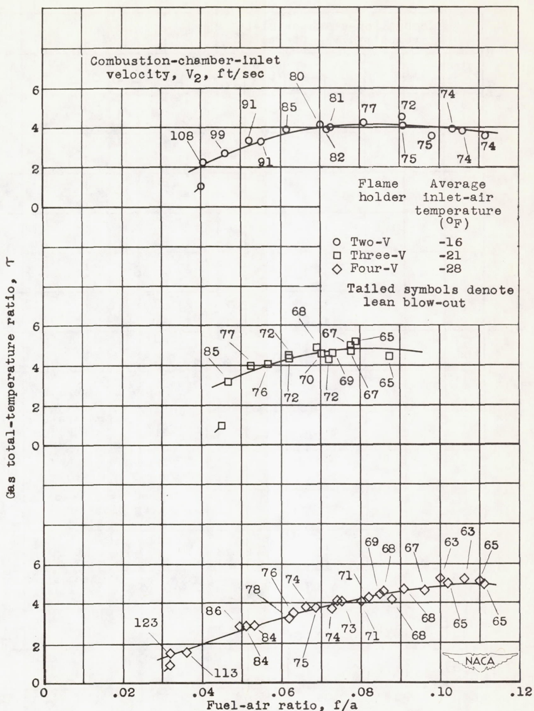
Figure 5. - Concluded. Effect of fuel-air ratio on gas total-temperature ratio for rectangular ram jet incorporating three flame-holder configurations.
