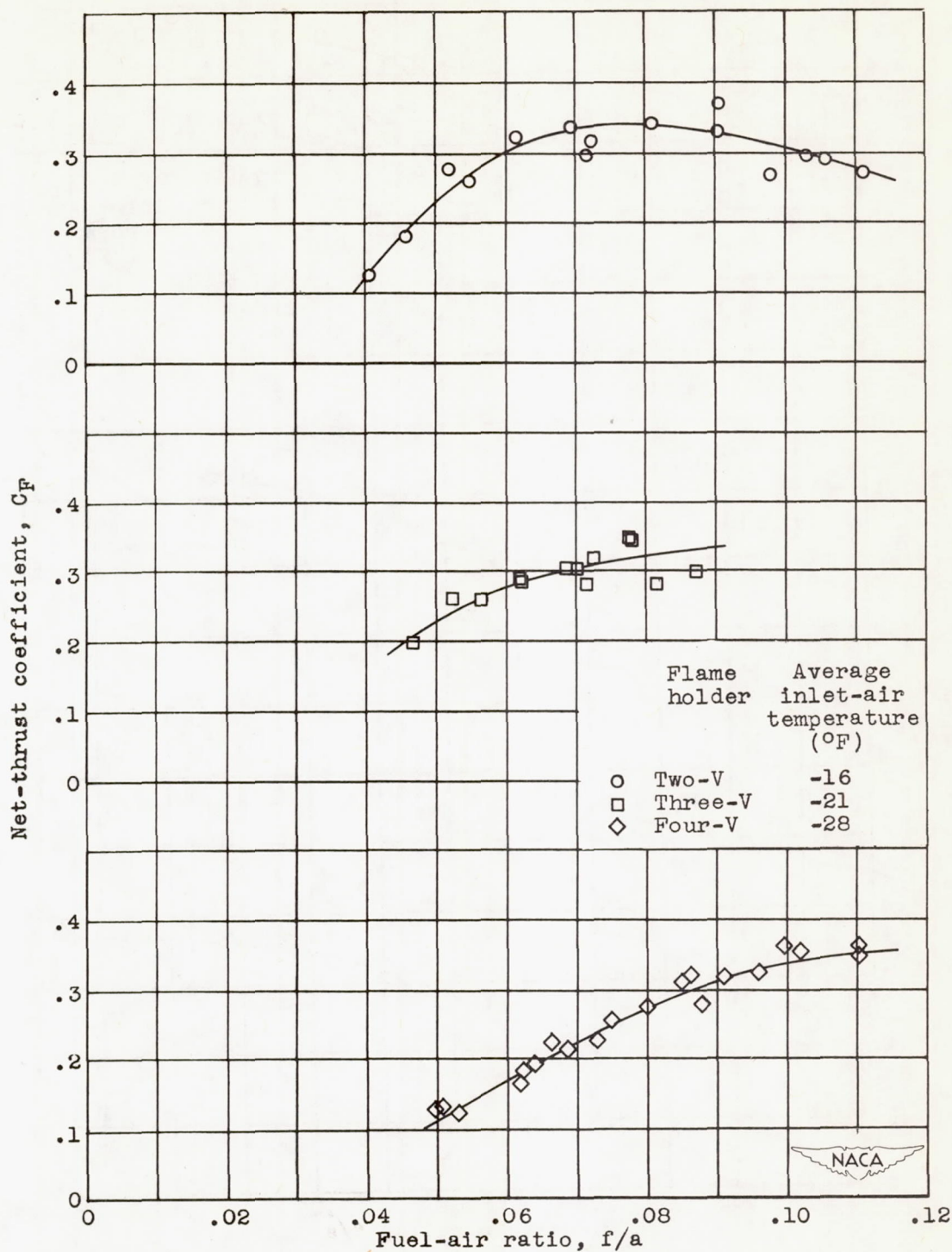
Figure 6. - Concluded. Effect of fuel-air ratio on net-thrust coefficient for rectangular ram jet incorporating three flame-holder configurations.
