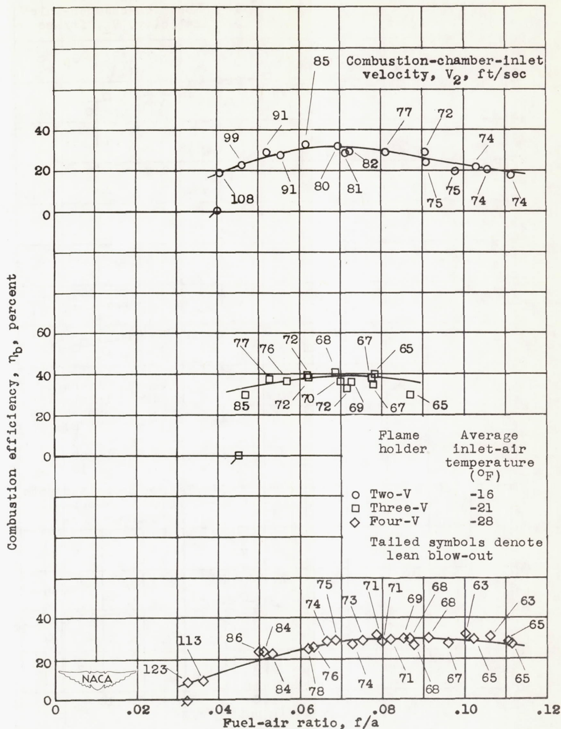
Figure 4. - Concluded. Effect of fuel-air ratio on combustion efficiency for rectangular ram jet incorporating three flame-holder configurations.
