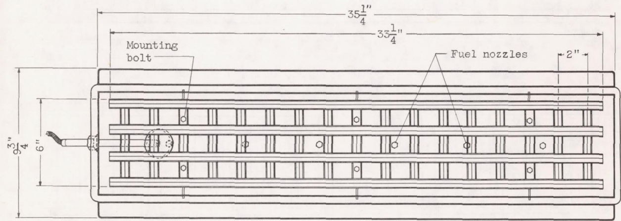
Section A-A Figure 1. - Schematic diagram of rectangular ram jet incorporating four-V gutter-type flame holder.
