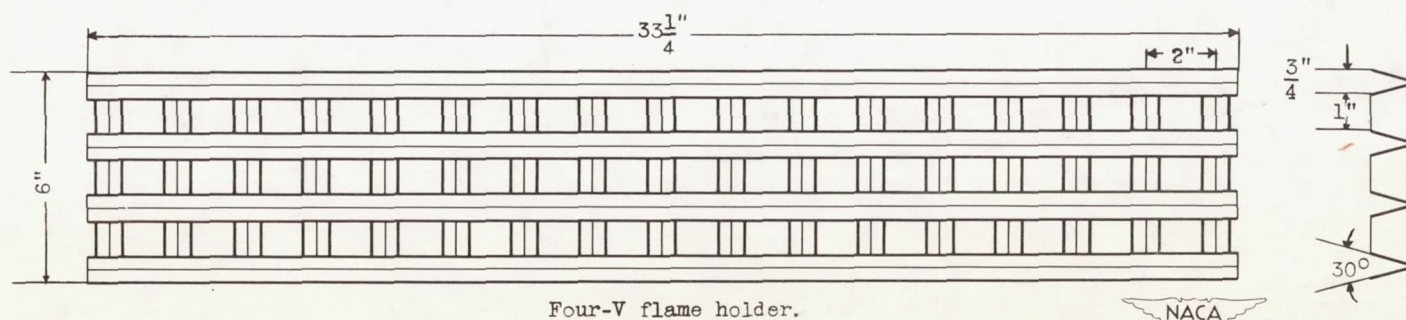
Figure 3. - Various flame-holder configurations investigated with rectangular ram jet.
