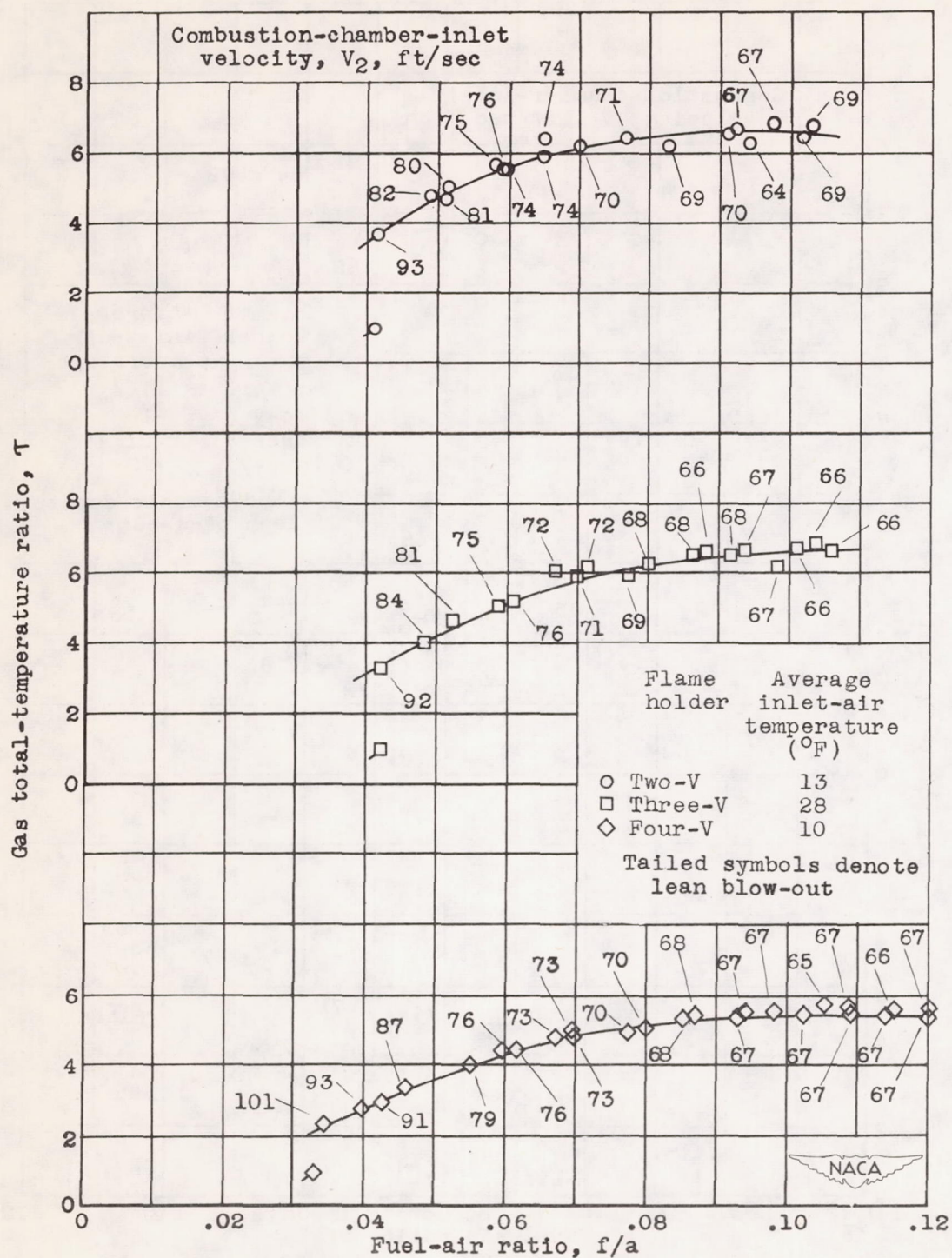
(c) Pressure altitude, 16,000 feet; indicated airspeed, 200 miles per hour.
