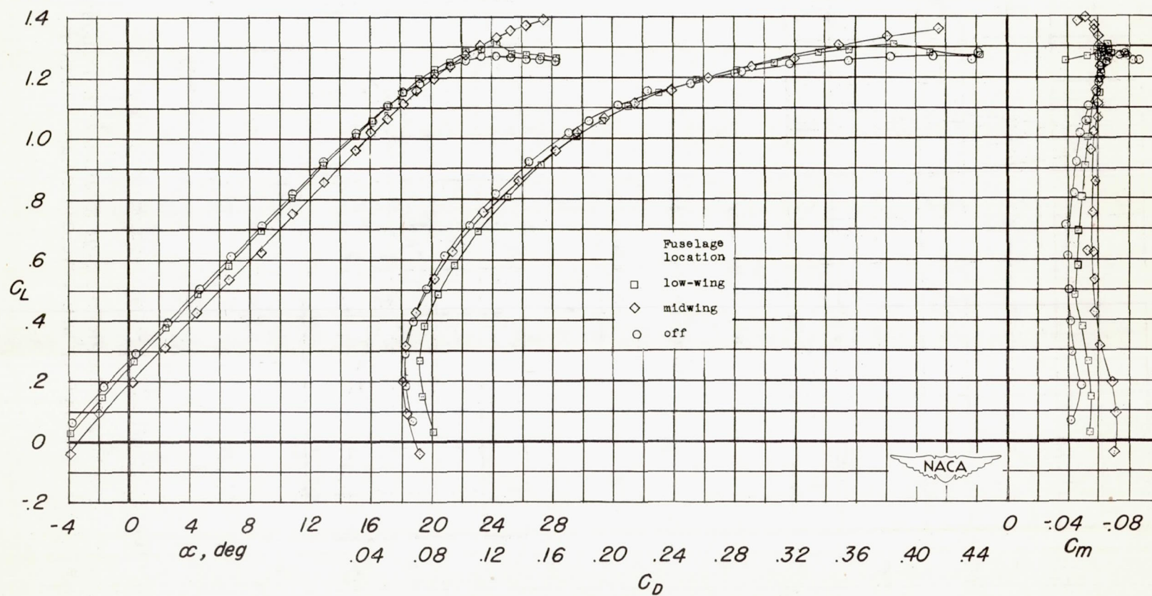
Figure 13.- Aerodynamic characteristics of a 52° sweptback wing with 0.575 \frac{b}{2} -span leading-edge flap, split flaps, upper-surface fences at 0.45 \frac{b}{2} , and fuselage.
