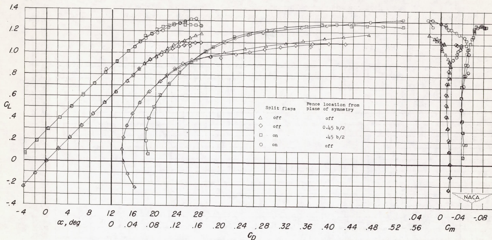
Figure 7.- The effect of split flaps and upper-surface fences on the aerodynamic characteristics of a 52° sweptback wing with 0.575 \frac{b}{2} -span leading-edge flaps.
