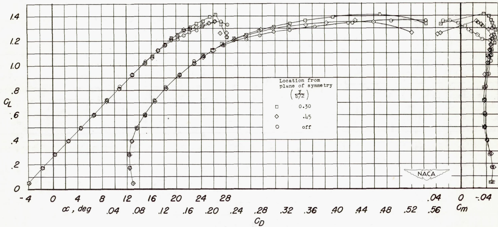
Figure 8.- Aerodynamic characteristics of a 52^\circ sweptback wing with upper-surface fences at two spanwise locations. 0.725\frac{b}{2} -span leading-edge flaps and split flaps on.
