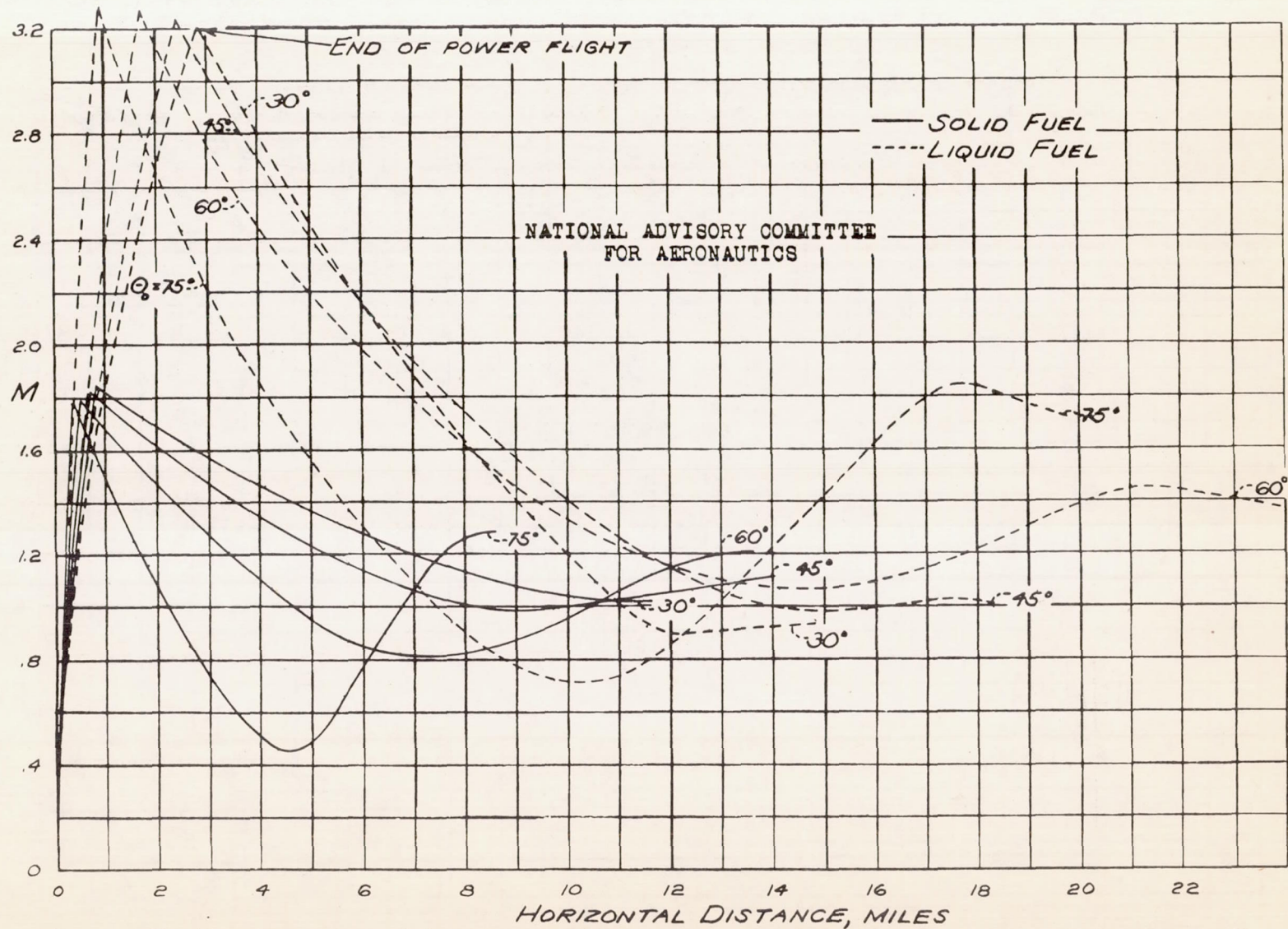
FIGURE 8. VARIATION OF MACH NUMBER WITH HORIZONTAL DISTANCE FOR MISSILE POWERED WITH SOLID-OR LIQUID-FUEL ROCKETS; \beta = 11.12
