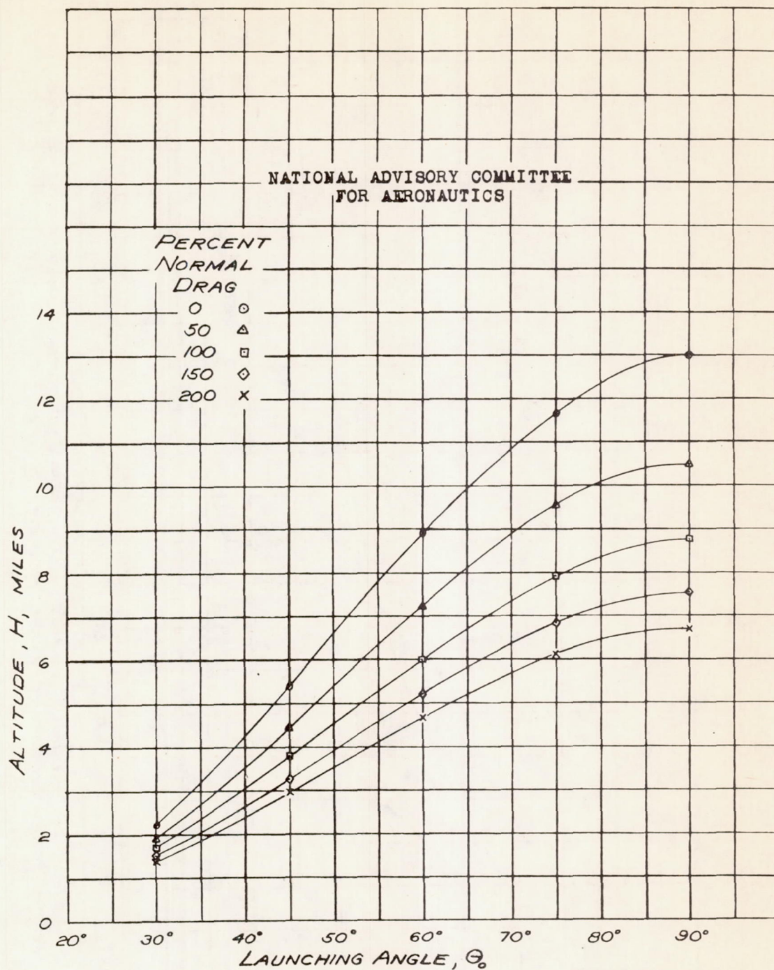
FIGURE 13.-VARIATION OF MAXIMUM ALTITUDE OF THE TRAJECTORY WITH LAUNCHING ANGLE FOR THE MISSILE WITH SOLID-FUEL ROCKET POWER AND SEVERAL ASSUMED VARIATIONS OF THE DRAG COEFFICIENT WITH MACH NUMBER. \beta=11.12
