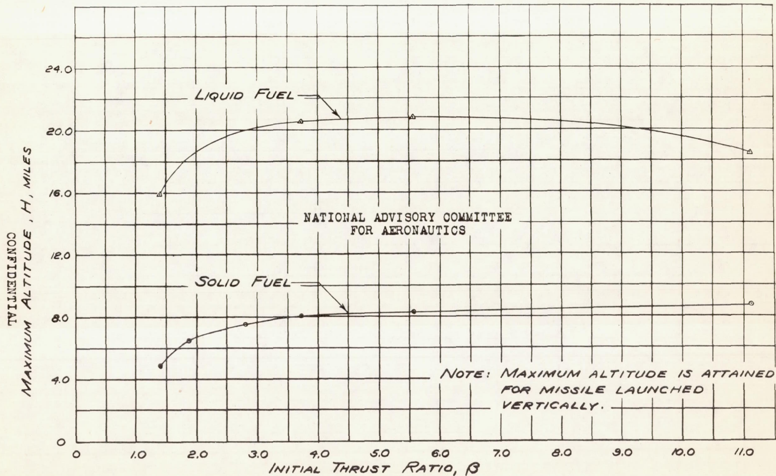
FIGURE 17.- VARIATION WITH INITIAL THRUST RATIO OF THE MAXIMUM ALTITUDE WHICH MISSILE WOULD ATTAIN IF POWERED WITH SOLID- OR LIQUID-FUEL ROCKETS.
