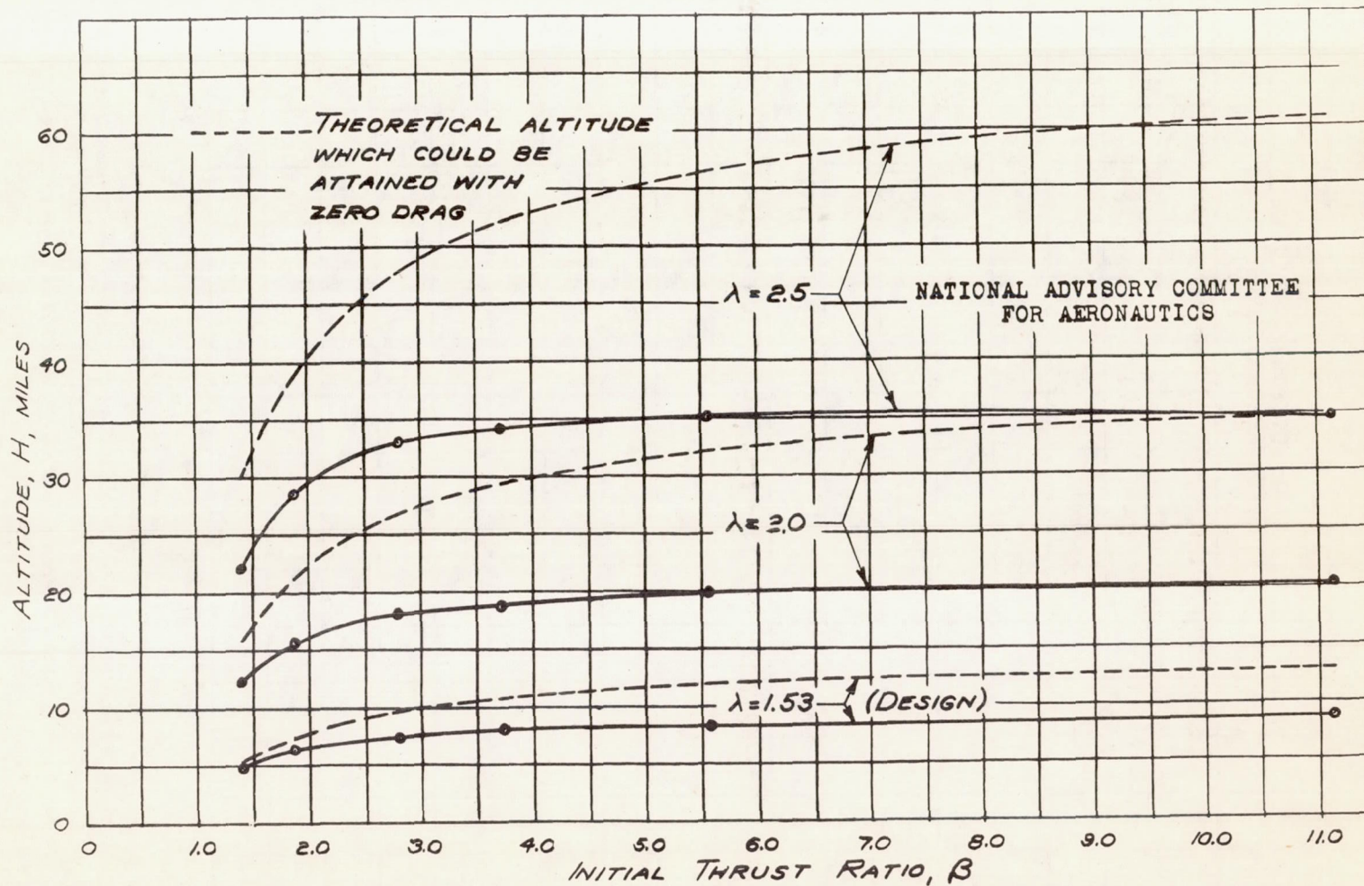
FIGURE 21.-- VARIATION OF ALTITUDE ATTAINED IN THE ATMOSPHERE WITH THE RATIO OF THRUST TO INITIAL WEIGHT FOR THE ASSUMED SUPERSONIC MISSILE POWERED WITH SOLID FUEL AND LAUNCHED VERTICALLY.
