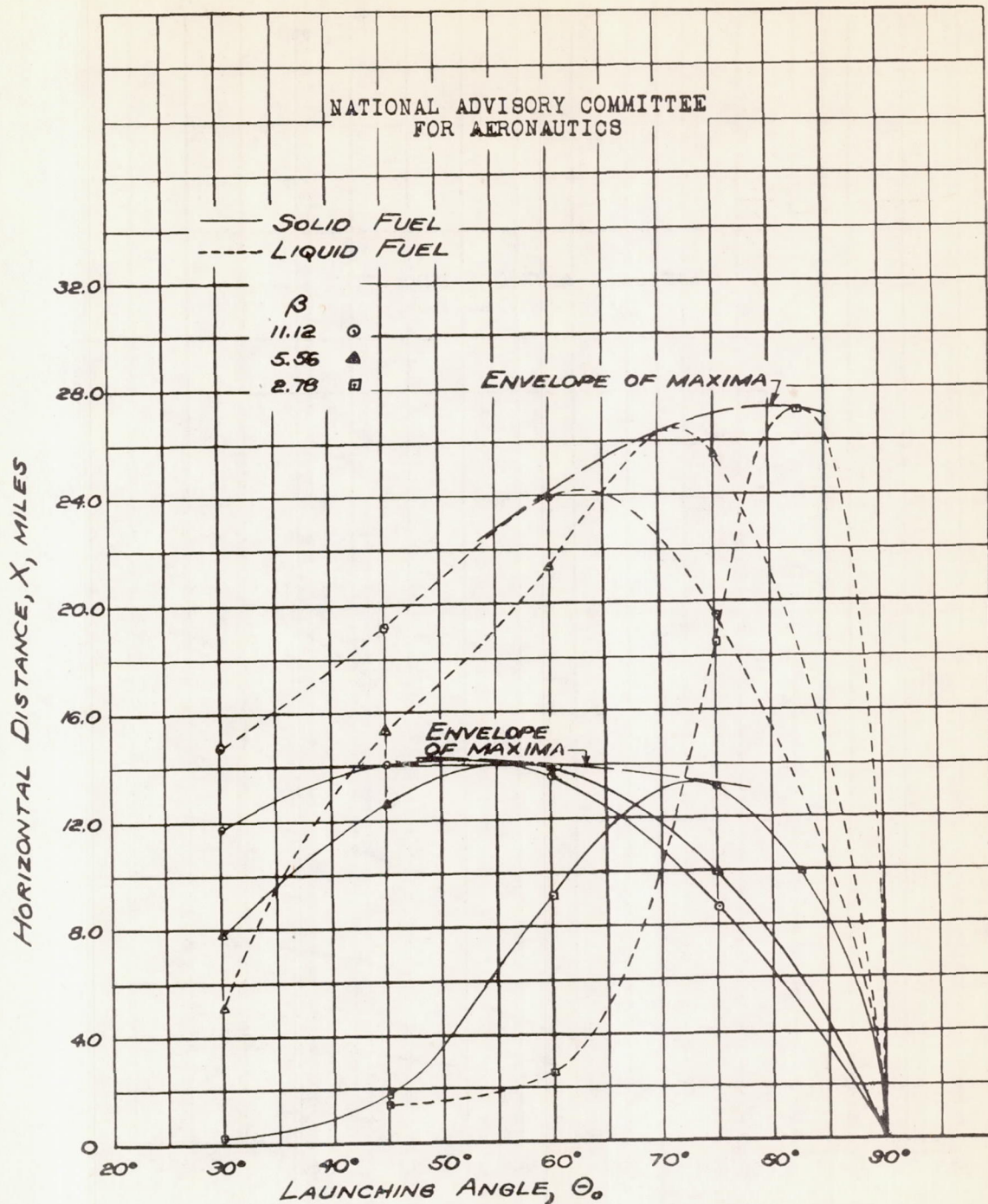
FIGURE 15.— VARIATION OF RANGE WITH LAUNCHING ANGLE FOR MISSILE WITH SOLID- OR LIQUID-FUEL ROCKET POWER FOR THREE VALUES OF INITIAL THRUST RATIO.
