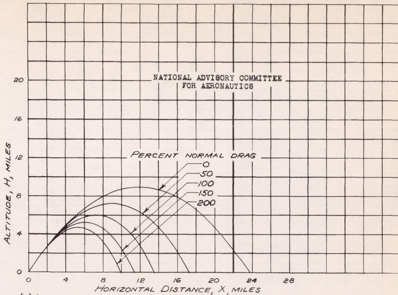
FIGURE 9.- CALCULATED TRAJECTORIES FOR THE MISSILE WITH SEVERAL ASSUMED VARIATIONS OF THE DRAG COEFFICIENT WITH MACH NUMBER. \beta = 11.12 , \theta_0 = 60^\circ
