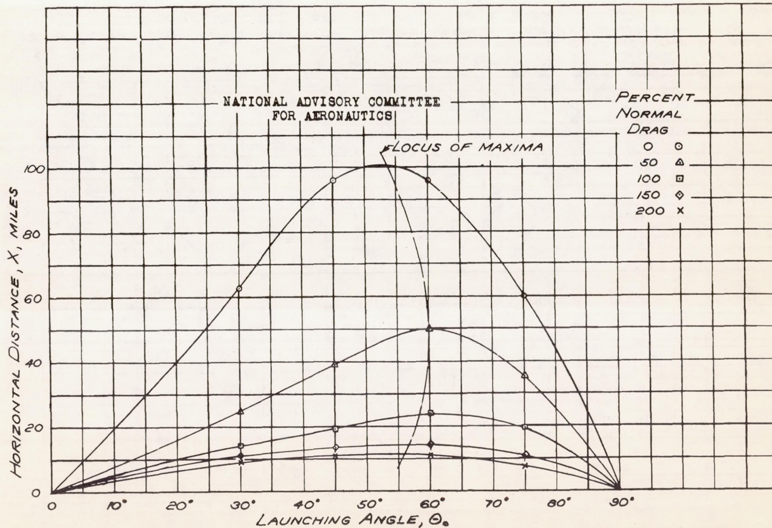
FIGURE 11.—VARIATION OF RANGE WITH LAUNCHING ANGLE FOR THE MISSILE WITH A LIQUID-FUEL ROCKET POWER PLANT AND SEVERAL ASSUMED VARIATIONS OF THE DRAG COEFFICIENT WITH MACH NUMBER, \beta = 11.12 .
