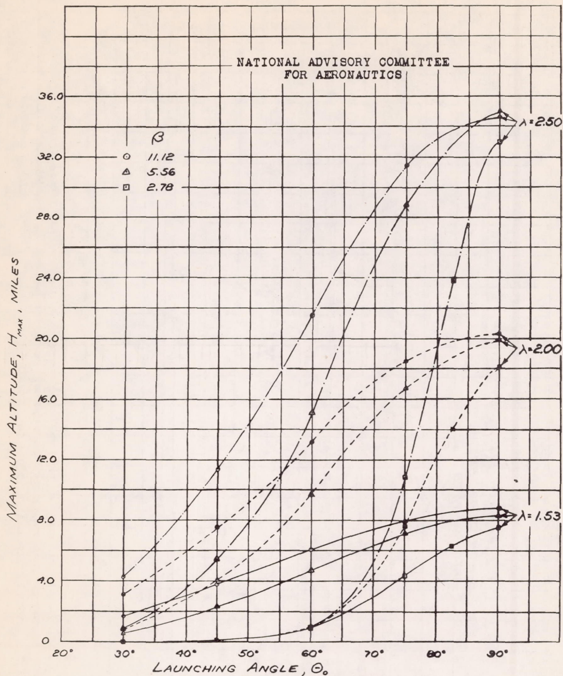
FIGURE 20.—VARIATION OF MAXIMUM ALTITUDE ATTAINED BY SOLID-FUEL-POWERED MISSILE WITH LAUNCHING ANGLE FOR THREE WEIGHT RATIOS AND THREE INITIAL THRUST RATIOS.
