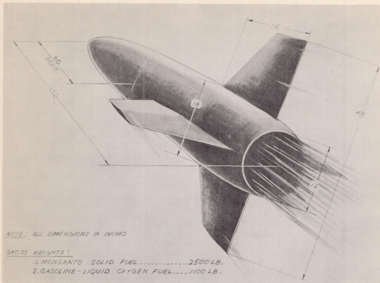
FIGURE 3. EXTERNAL CONFIGURATION OF ASSUMED GROUND-TO-AIR SUPERSONIC MISSILE USED TO COMPARE LIQUID AND SOLID FUEL ROCKET POWER PLANTS.
