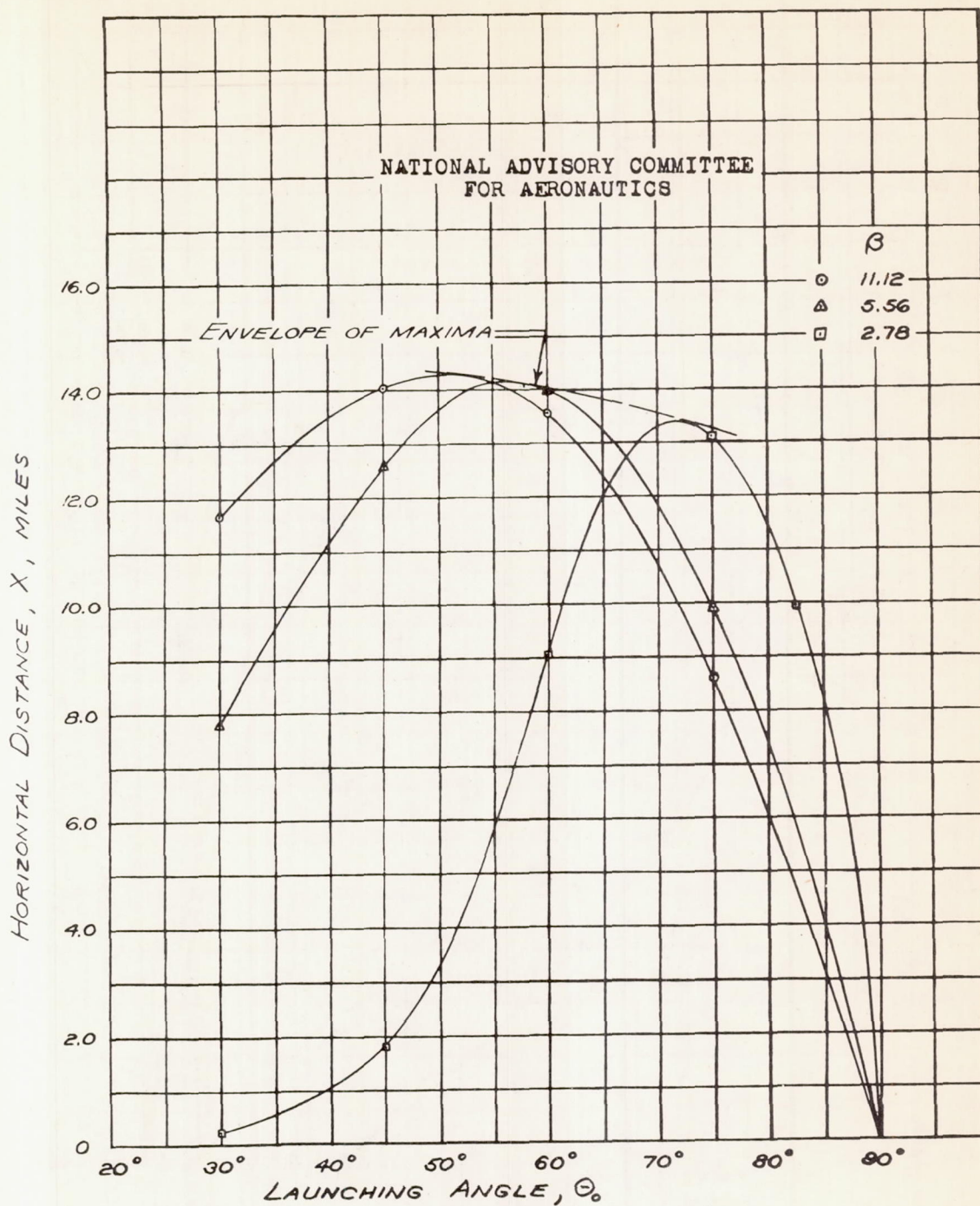
FIGURE 19.- VARIATION OF RANGE WITH LAUNCHING ANGLE FOR SOLID-FUEL-POWERED MISSILE WITH THREE VALUES OF INITIAL THRUST RATIO.
