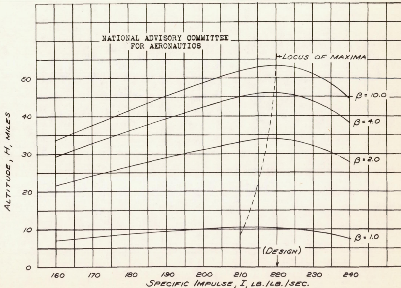
FIGURE 6. VARIATION OF ALTITUDE WITH SPECIFIC IMPULSE FOR THE ASSUMED SUPERSONIC MISSILE WITH ZERO DRAG USING GASOLINE AND LIQUID-OXYGEN FUEL AND HAVING SEVERAL VALUES OF THE RATIO OF THRUST TO INITIAL WEIGHT, \beta .
