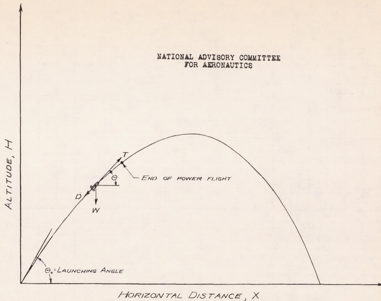
FIGURE 1.- COORDINATE SYSTEM AND FORCE DIAGRAM USED IN ANALYSIS OF SUPERSONIC MISSILES.
