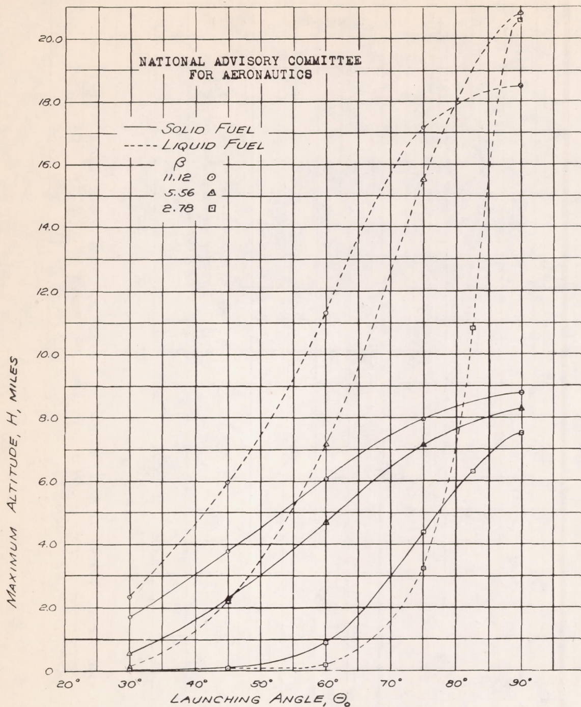
FIGURE 16.- VARIATION OF THE MAXIMUM ALTITUDE ATTAINED WITH LAUNCHING ANGLE FOR SOLID- OR LIQUID-FUEL ROCKET-POWERED MISSILES WITH THREE VALUES OF INITIAL THRUST RATIO.
