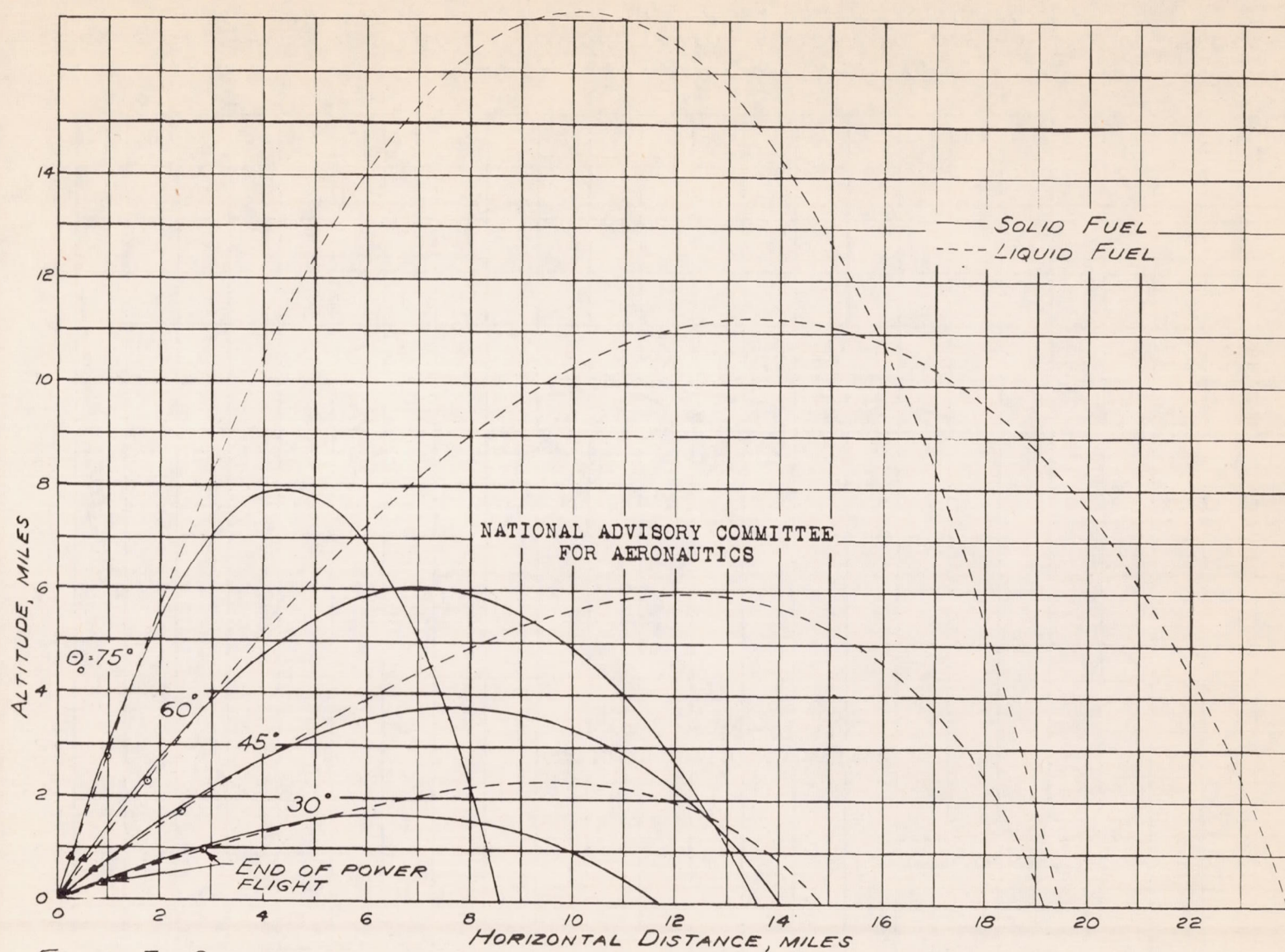
FIGURE 7. CALCULATED TRAJECTORIES FOR MISSILE POWERED WITH SOLID-OR LIQUID-FUEL ROCKETS \beta = 11.12 .
