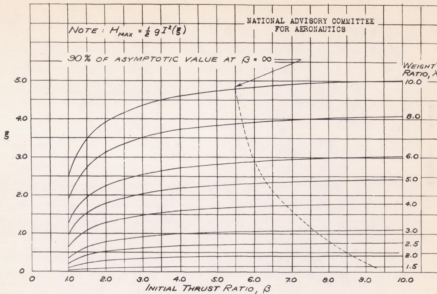
FIGURE 22. - VARIATION OF THE FACTOR \xi WITH INITIAL THRUST RATIO FOR SEVERAL VALUES OF THE WEIGHT RATIO.
