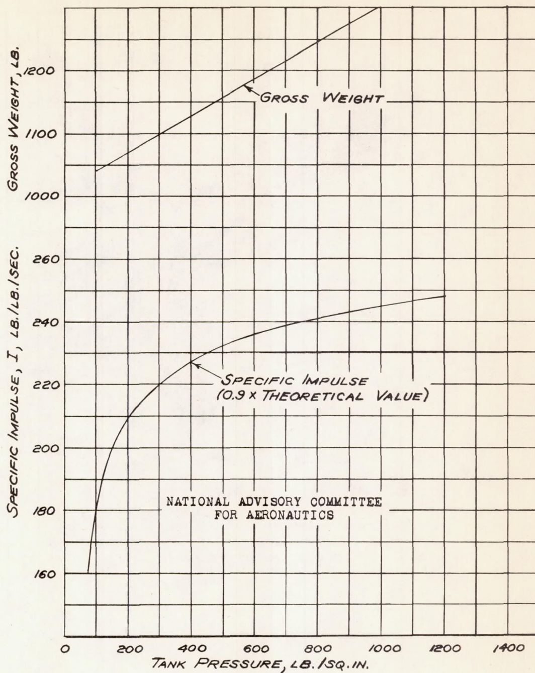
FIGURE 4.- VARIATION OF SPECIFIC IMPULSE AND INITIAL GROSS WEIGHT WITH FUEL-TANK PRESSURE FOR THE ASSUMED SUPERSONIC MISSILE WITH GASOLINE AND LIQUID-OXYGEN FUEL.
