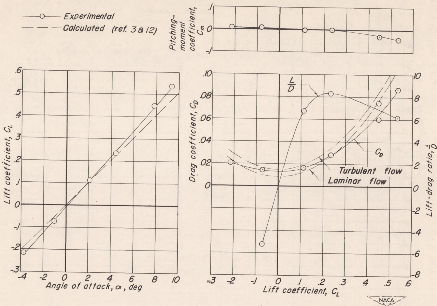
(h) M=1.12 , R=0.85 \times 10^6 Figure 4.- Continued.
