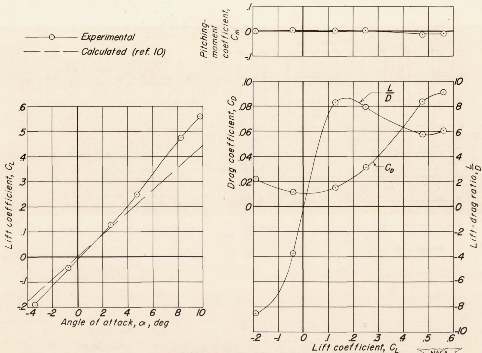
(e) M=0.950 , R=0.84 \times 10^6 . Figure 4.-Continued
