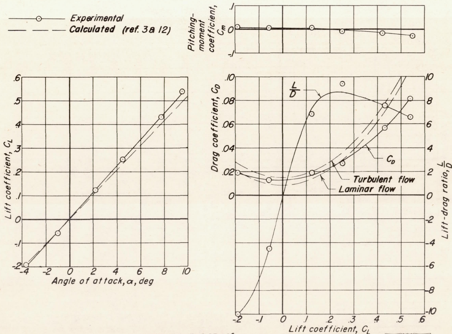
(g) M=1.09 , R=0.85 \times 10^6 . Figure 4.- Continued.
