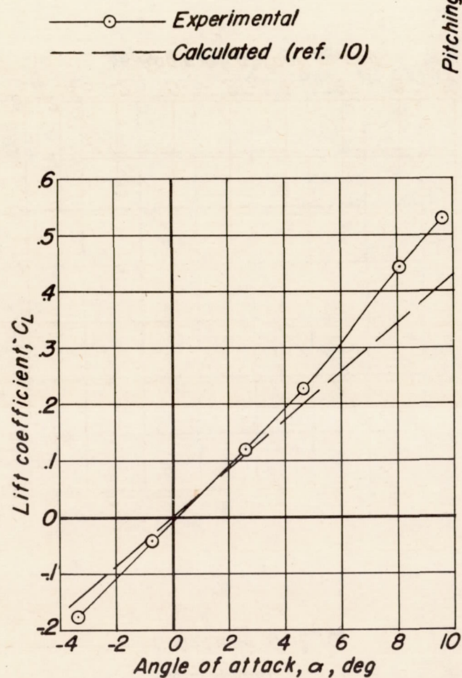
(c) M=0.90 , R=0.85 \times 10^6 . Figure 4.-Continued.
