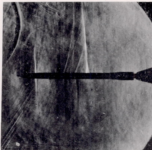
(b) M = 0.95 , side view.
