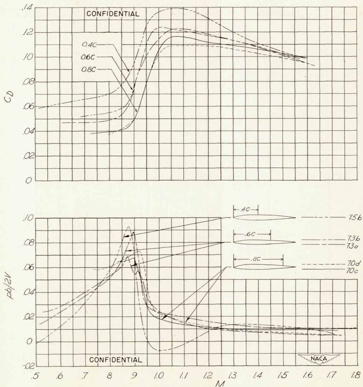
Figure 5.- Effect of chordwise location on spoiler effectiveness.
