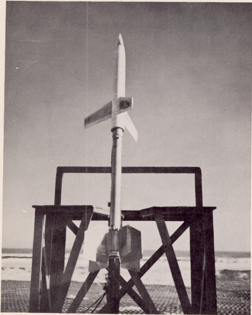
Figure 3.- Typical RM-5 test vehicle prior to launching. CONFIDENTIAL
