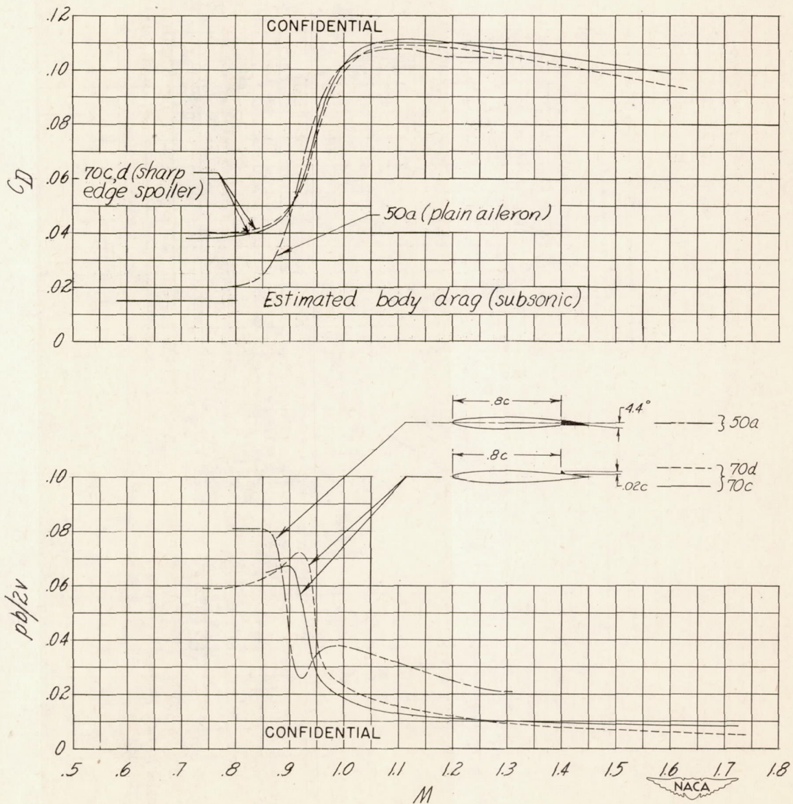
Figure 7.- Comparison of rolling effectiveness and drag coefficient for plain and spoiler ailerons. Airfoil section, NACA 65-009; \Lambda = 0^\circ ; A = 3.0 (reference 4).
