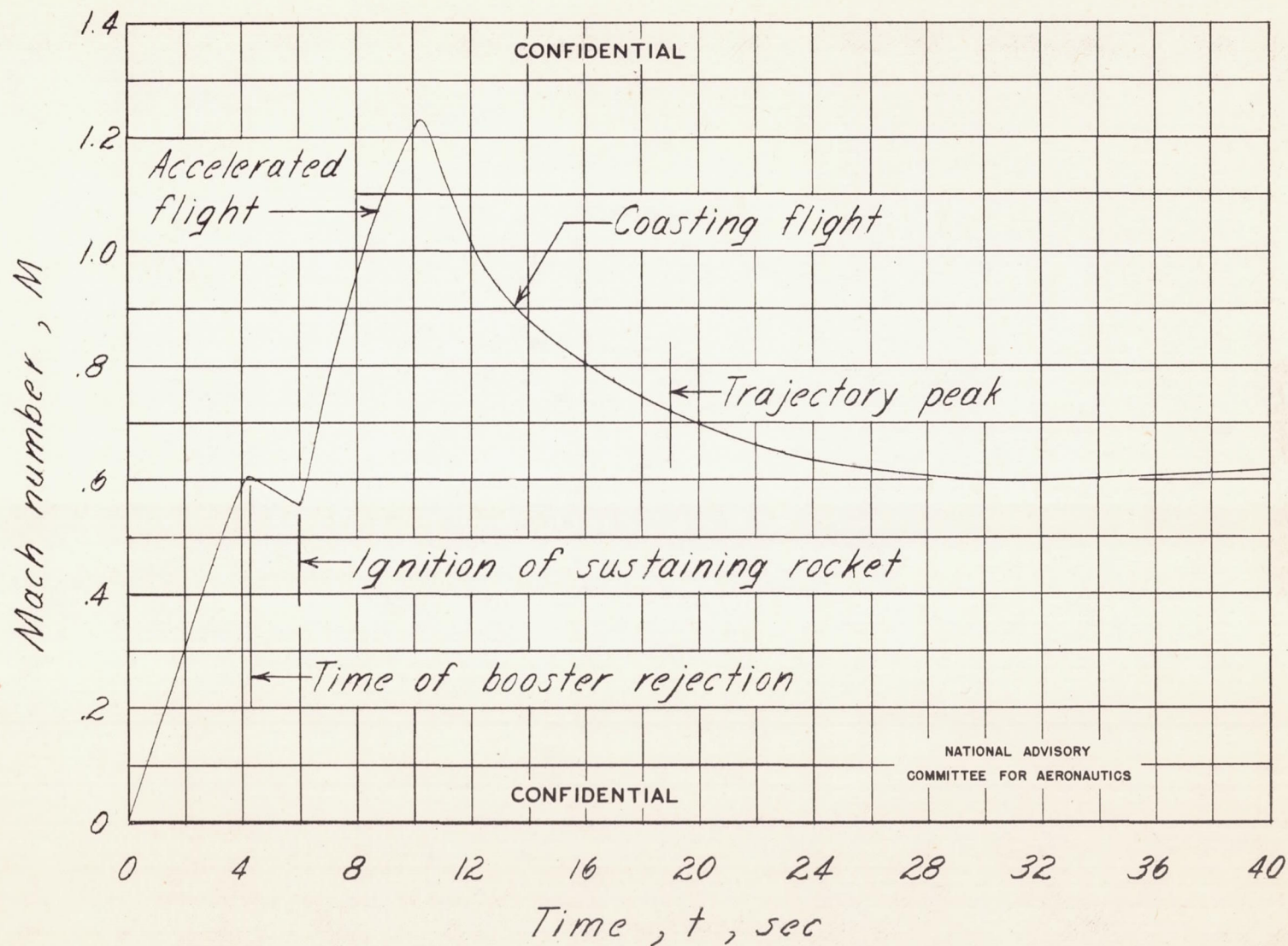
Figure 6.- Time history of Mach number.
