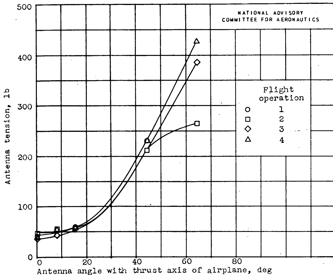
Figure 9. - Variation of antenna tension with antenna angle for antennas of 40, 41, 42, and 43 feet in length. Distance flown in icing region, 115 miles.
