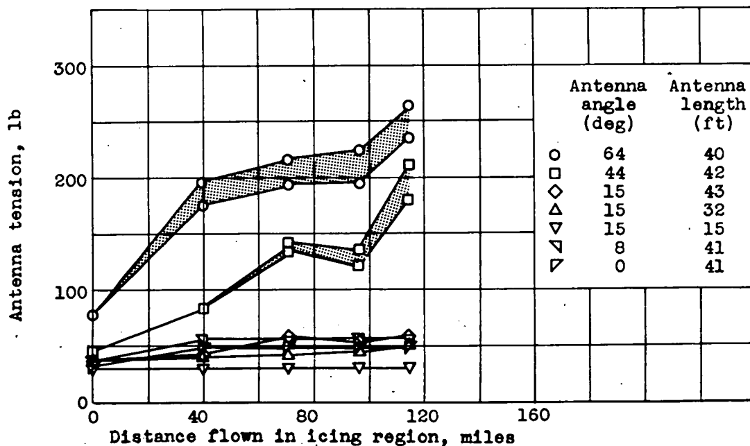
(b) Flight operation 2; pressure altitude, 3700 feet; true airspeed, 177 miles per hour; ambient-air temperature, 25° F; liquid-water content, 0.30 grams per cubic meter; average droplet diameter, 13 microns.
