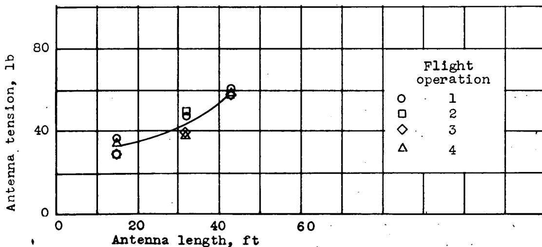
Figure 10. - Variation of antenna tension with antenna length at antenna angle of 15^\circ . Distance flown in icing region, 115 miles.
