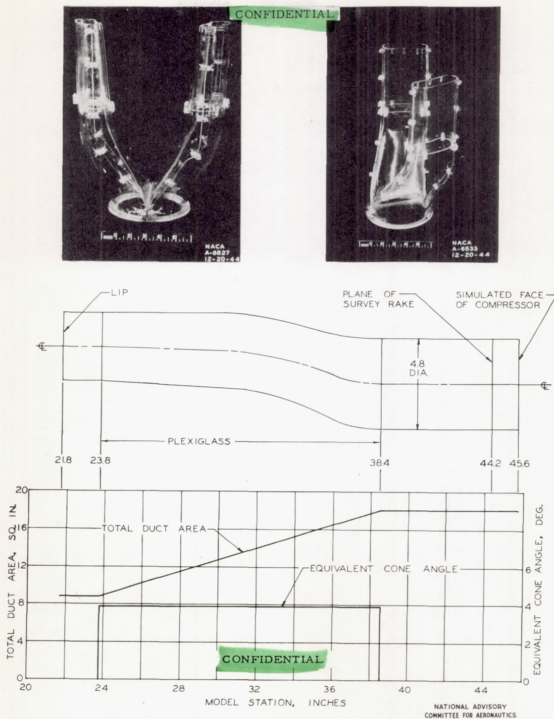
Figure 4.— Dimensional Characteristics of the internal-ducting system, to the stimulated face of the jet-engine compressor for the 1/5-scale model of the fighter airplane equipped with submerged ducts.
