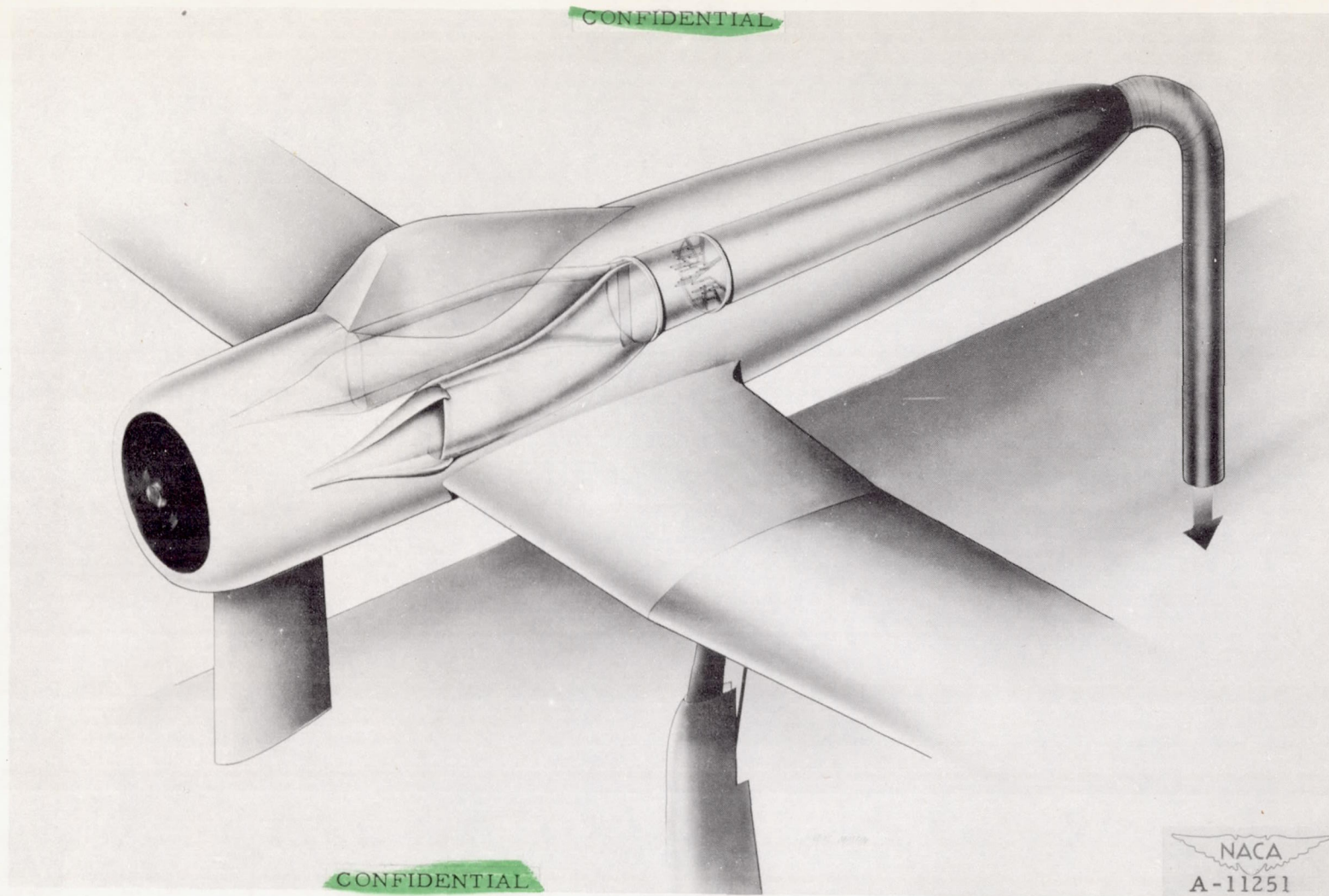
Figure 3.- Schematic view of the wind-tunnel test setup for the 1/5-scale model of the fighter airplane equipped with NACA submerged air inlets.
