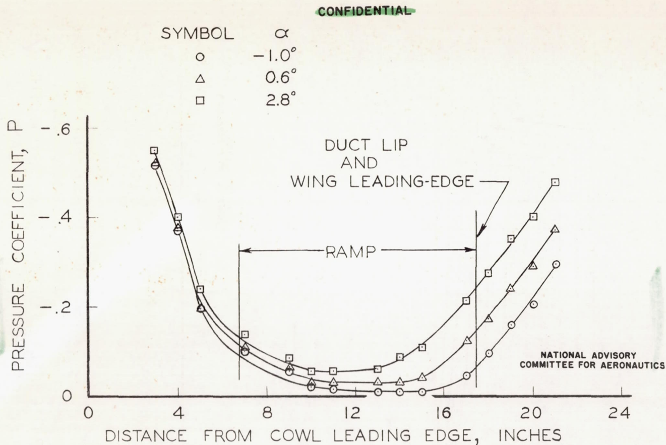
FIGURE 15.—PRESSURE DISTRIBUTION OF THE BASIC FUSELAGE CONTOUR ALONG THE \bar{C}_L OF THE NACA SUBMERGED DUCT ENTRY. 1/5-SCALE MODEL OF THE FIGHTER AIRPLANE. Re = 1.41 \times 10^6
