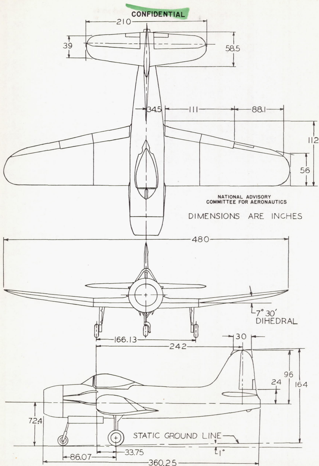
FIGURE 1.-GENERAL ARRANGEMENT OF THE FIGHTER AIRPLANE EQUIPPED WITH NACA SUBMERGED AIR INLETS. CONFIDENTIAL
