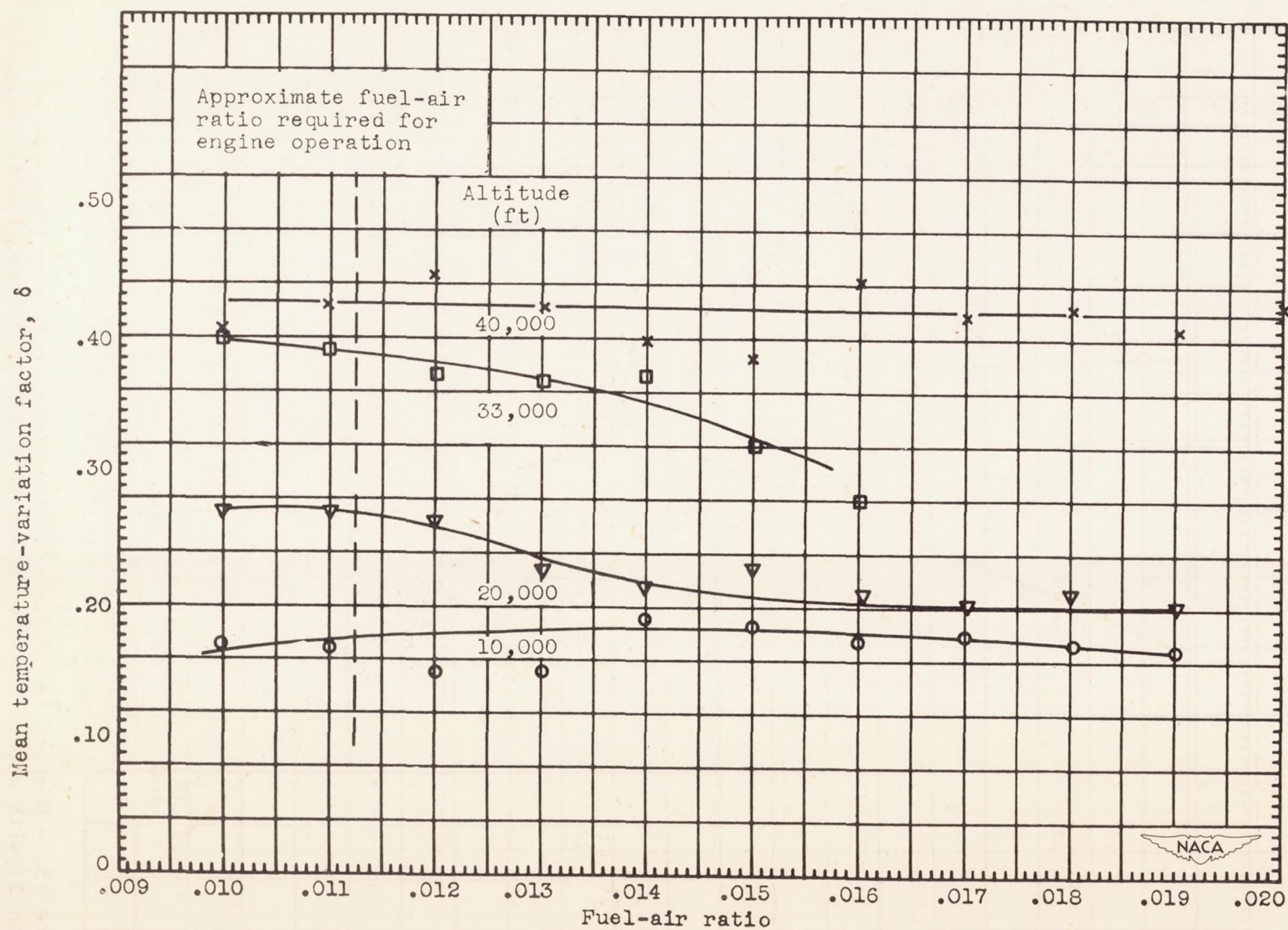
Figure 12. - Effect of fuel-air ratio on mean outlet temperature-variation factor \delta . Engine speed, 16,000 rpm.
