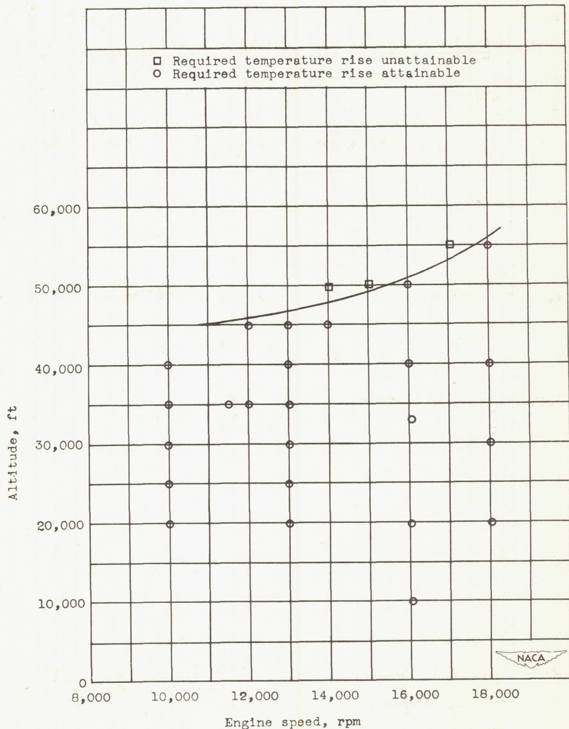
Figure 6. - Altitude operational limits of one-eighth segment of proposed turbojet combustor. Flight speed, 375 miles per hour.
