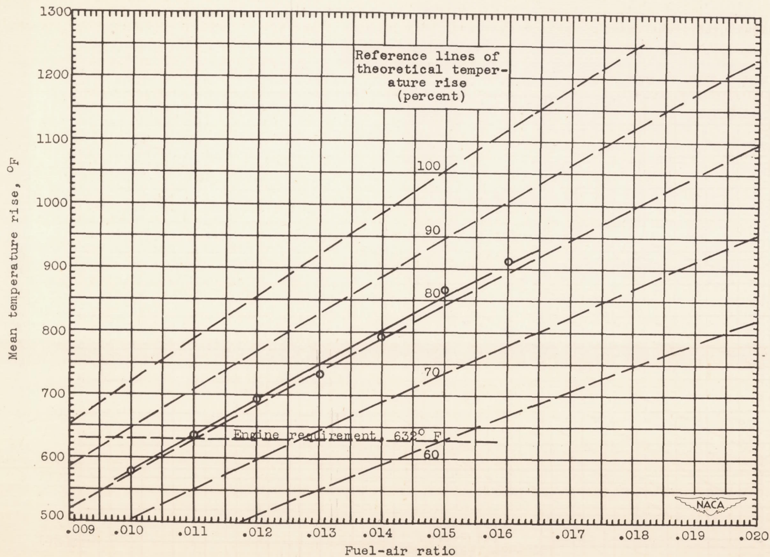
(c) Altitude, 33,000 feet. Figure 7. - Continued. Effect of fuel-air ratio on mean temperature rise through one-eighth segment of proposed turbojet combustor. Engine speed, 16,000 rpm.
