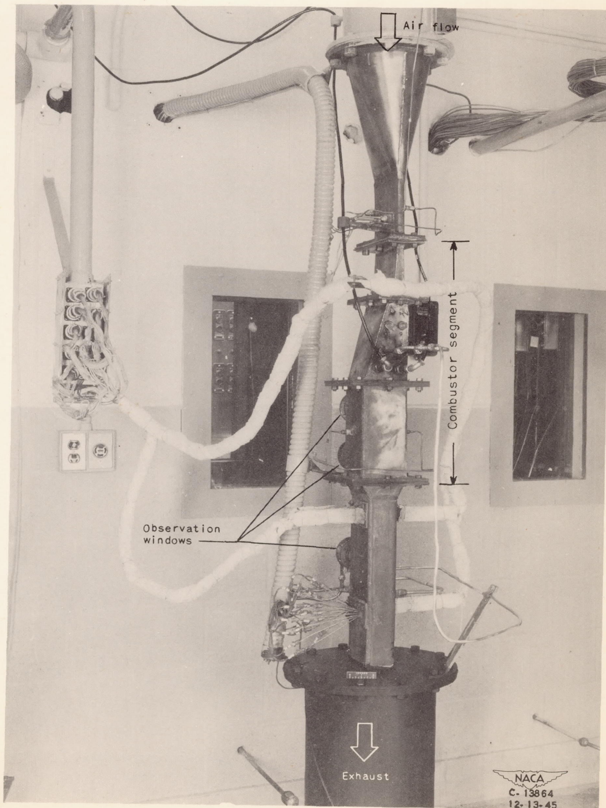
Figure 3. - Installation of one-eighth segment of proposed turbojet combustor.
