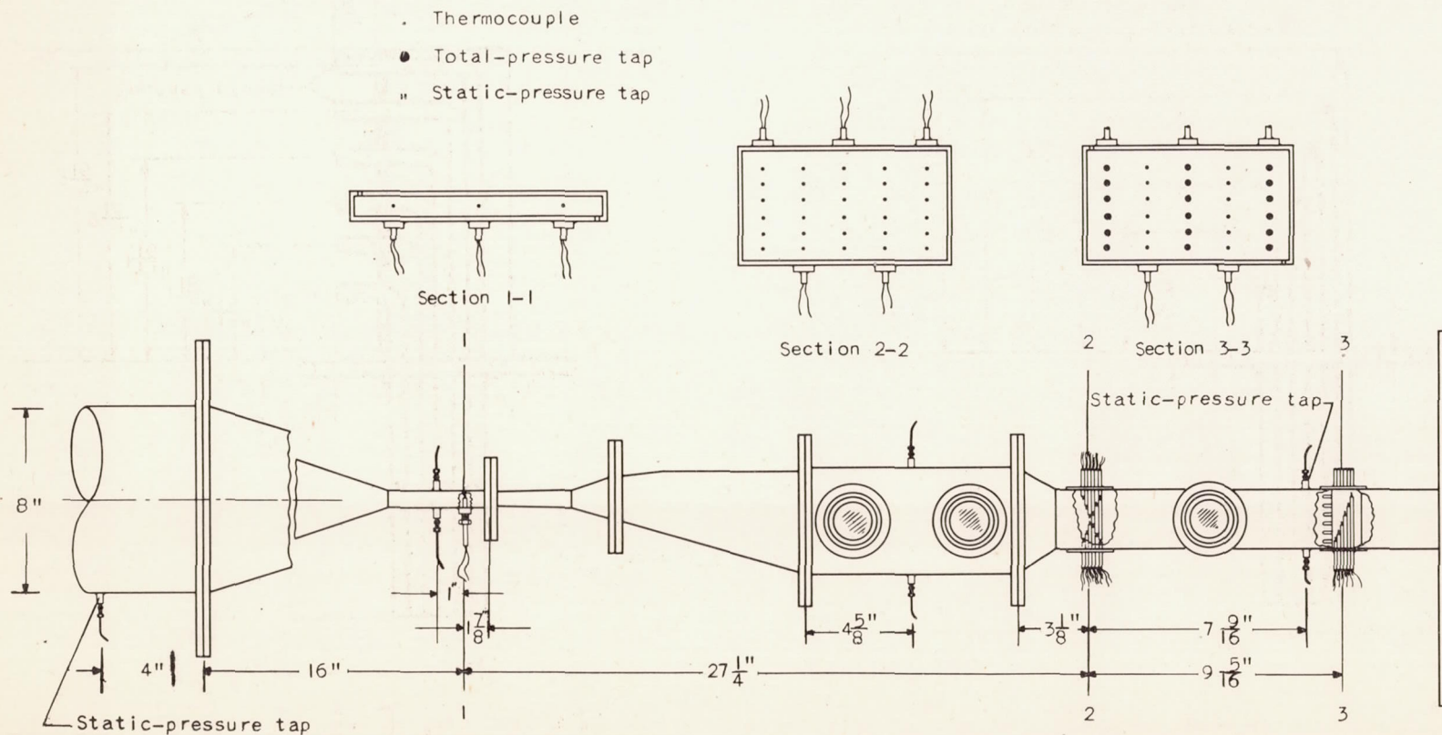
(a) Arrangement of instruments in duct and location of instrument station.
