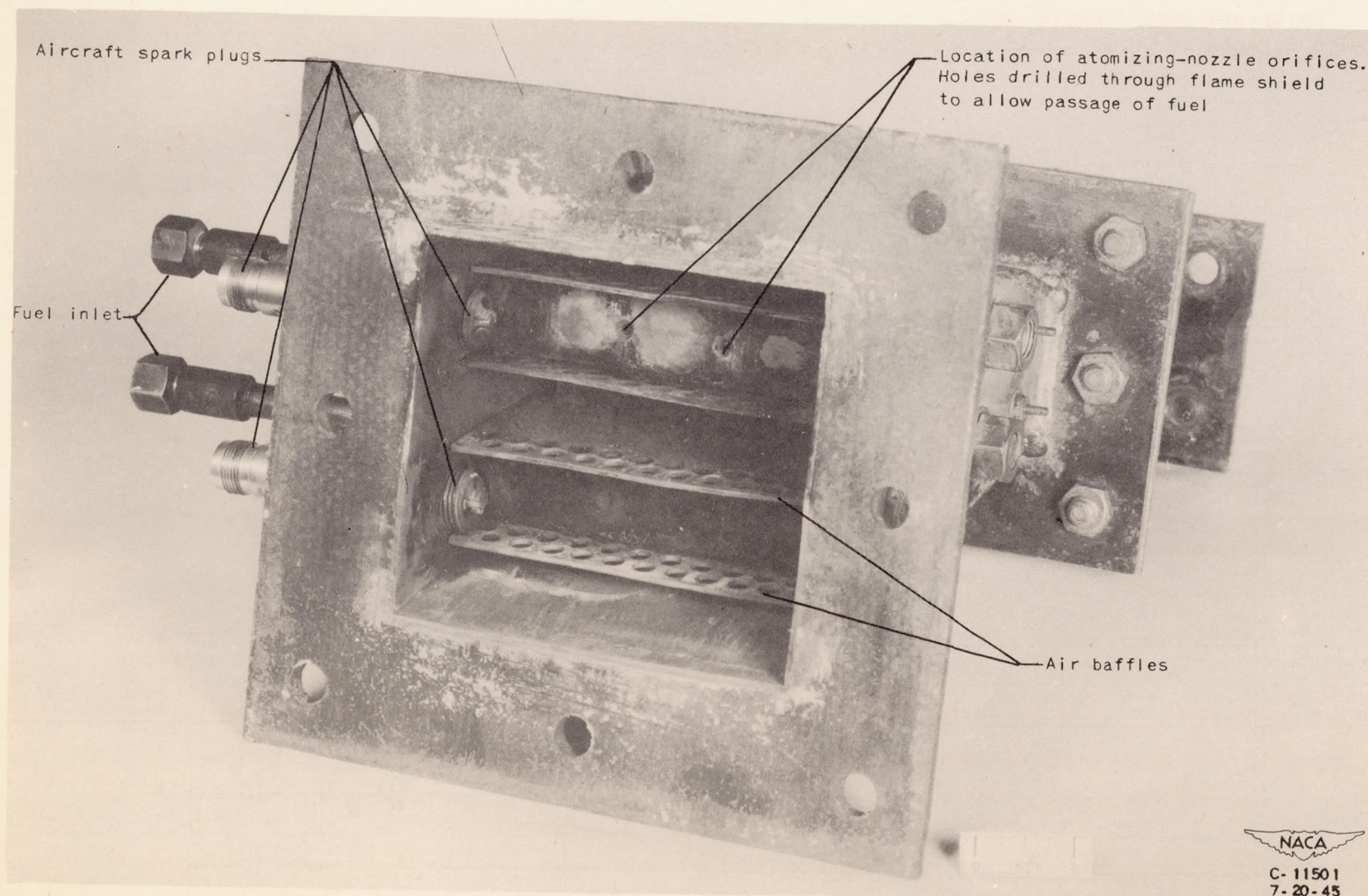
Figure 2. - View of combustor segment showing atomizing nozzles and spark plugs after approximately 200 hours of operation.
