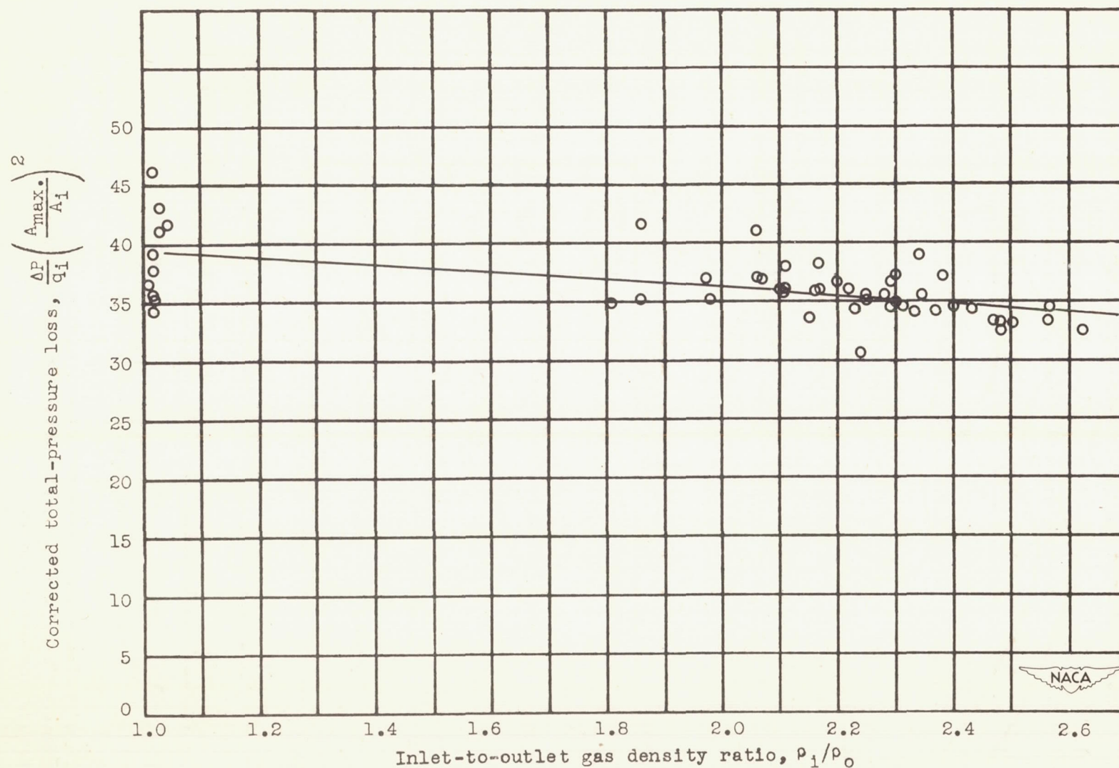
Figure 9. - Total-pressure loss through one-eighth segment of proposed turbojet combustor expressed as fraction of inlet kinetic pressure and as function of inlet-to-outlet gas density ratio.
