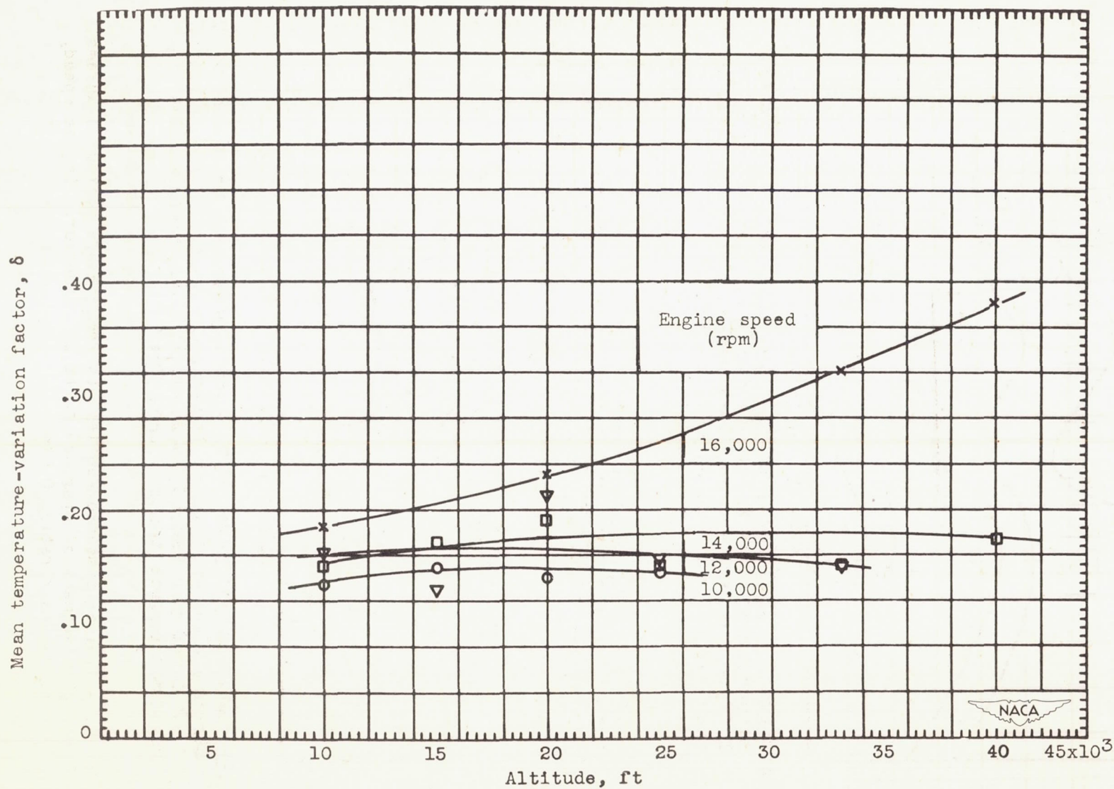
Figure 11. - Effect of various altitudes and engine speeds simulated by inlet conditions on mean outlet-temperature-variation factor, \delta . Fuel-air ratio, 0.015.
