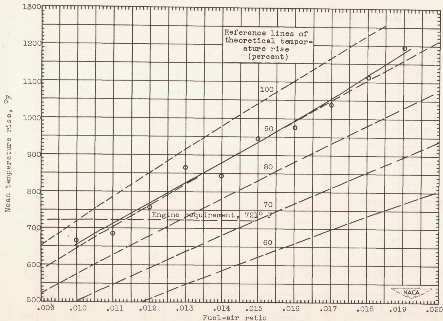
Figure 7. - Effect of fuel-air ratio on mean temperature rise through one-eighth segment of proposed turbojet combustor. Engine speed, 16,000 rpm.
