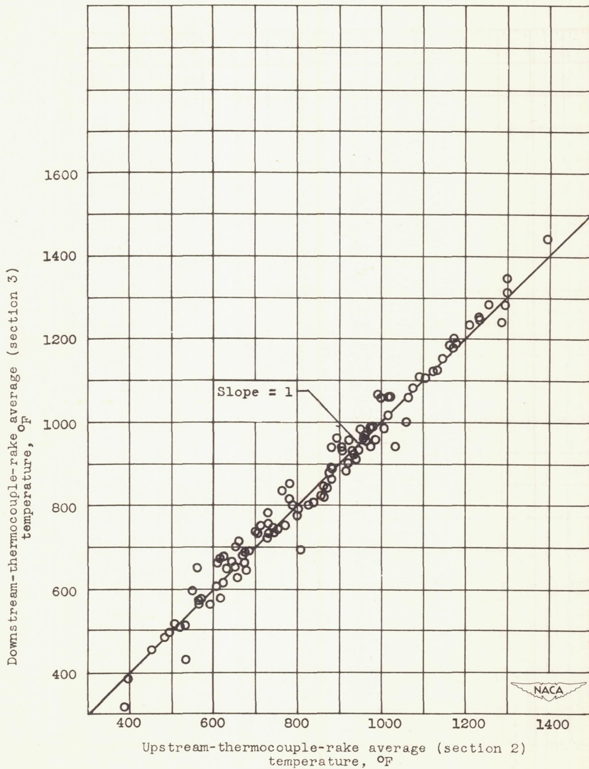
Figure 13. - Comparison of upstream-thermocouple-rake average (section 2) with downstream-thermocouple-rake average (section 3) temperature.
