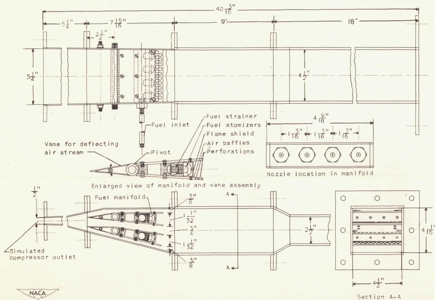
Figure 1. - Diagrammatic sketch of one-eighth segment of proposed turbojet combustor showing air-deflecting vanes, fuel manifolds, fuel atomizers, and housing. Fuel nozzles, fuel manifolds, and ignition plugs as shown in figure 2.
