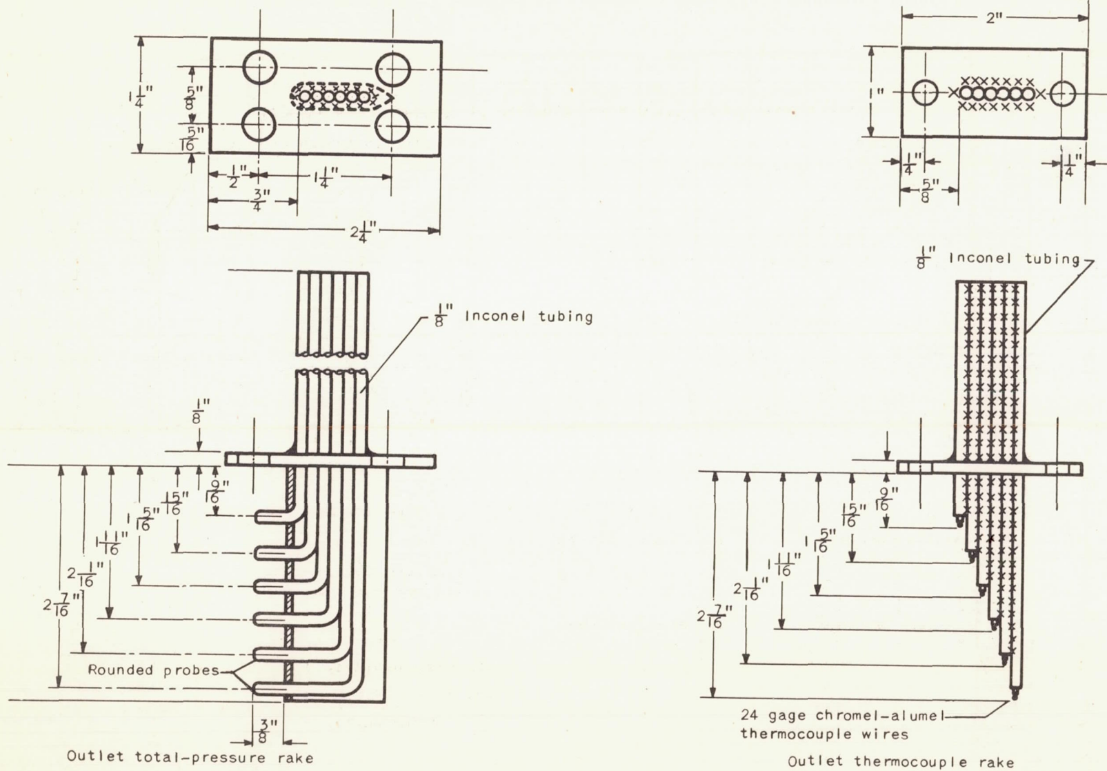
(b) Details of total-pressure rakes and thermocouple rakes. Figure 4. - Concluded. Sketch of combustor-segment instrumentation.
