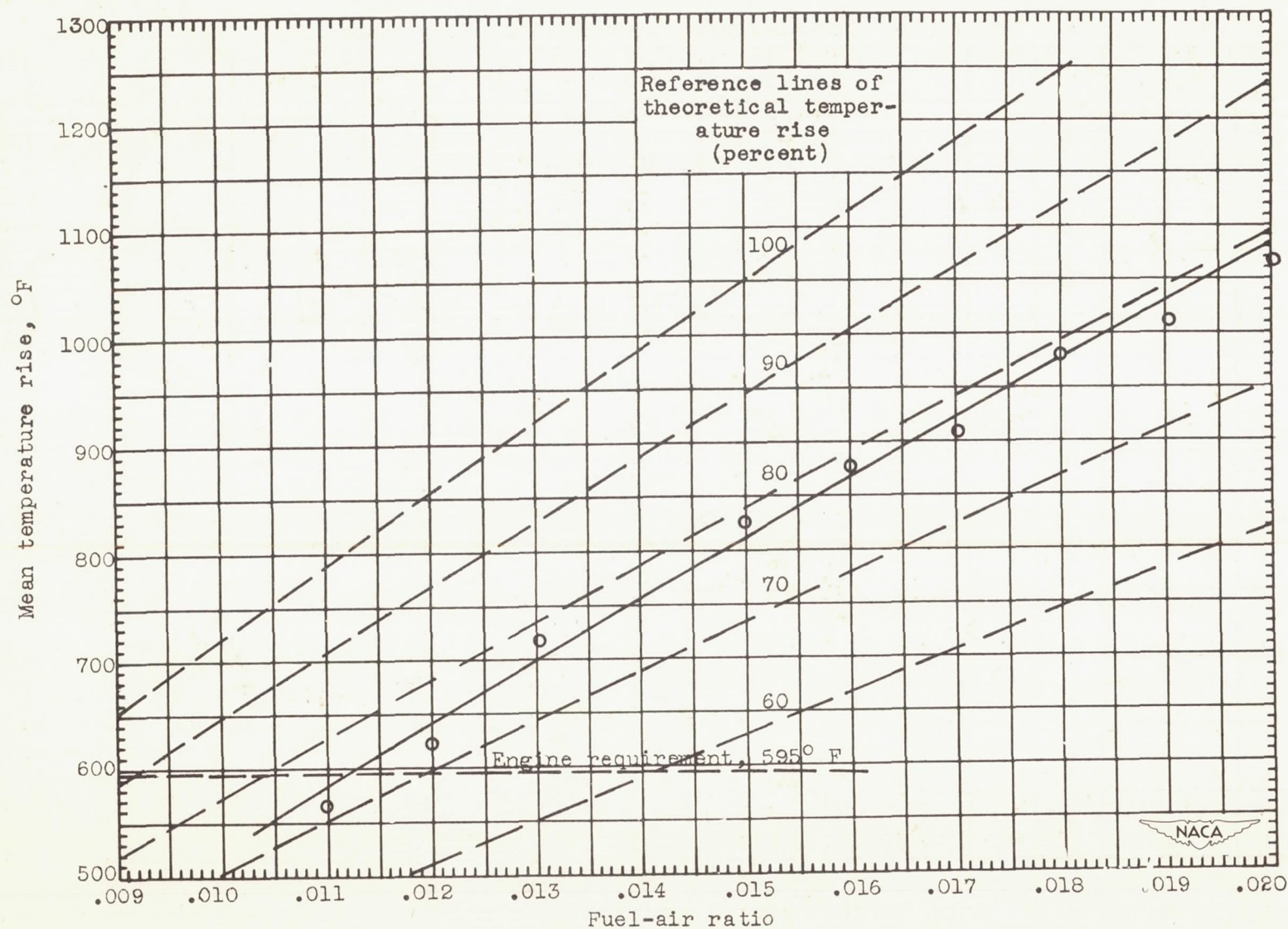
Figure 7. - Concluded. Effect of fuel-air ratio on mean temperature rise through one-eighth segment of proposed turbojet combustor. Engine speed, 16,000 rpm.
