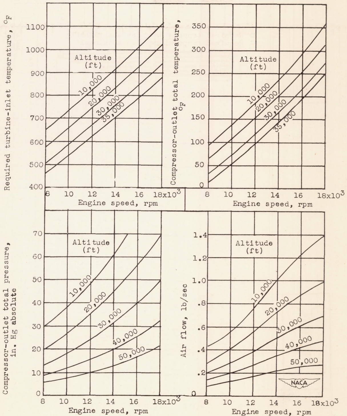
Figure 5. - Estimated inlet conditions of air flow, total pressure, temperature, and required turbine-inlet temperature of one-eighth segment of proposed turbojet combustor. Tail-cone area, 43.3 square inches; flight speed, 470 miles per hour; engine inlet-diffuser efficiency, 100 percent.
