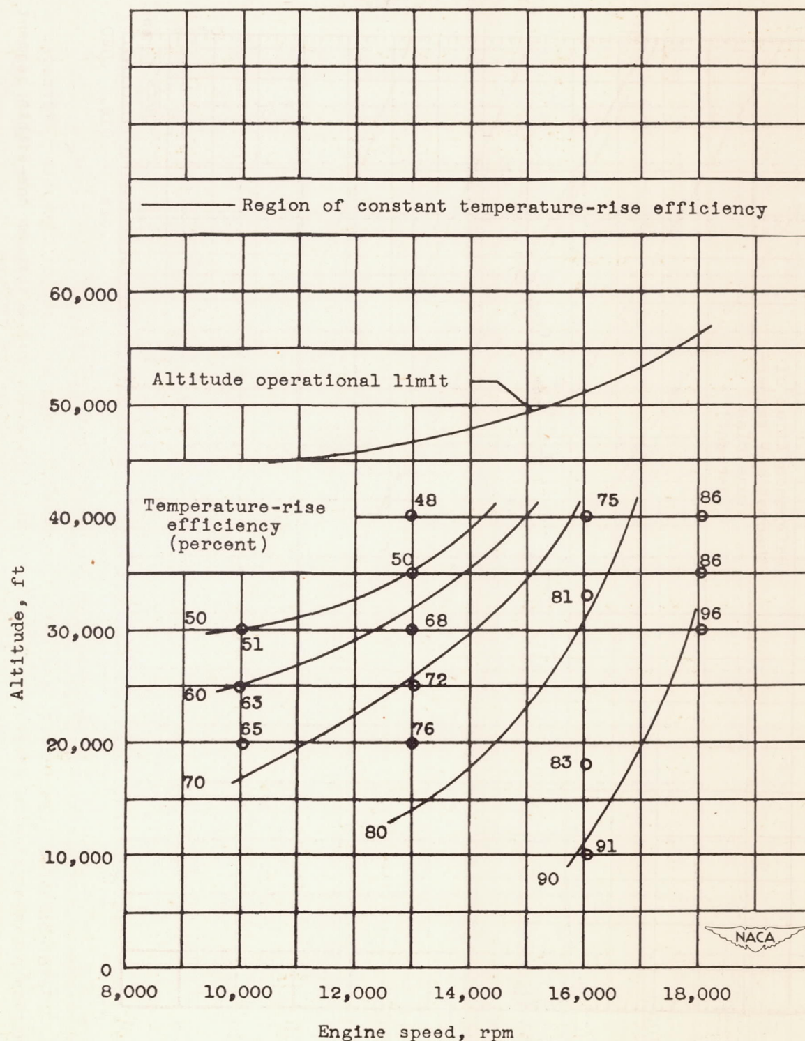
Figure 8. - Temperature-rise-efficiency contour diagram of one-eighth segment of proposed turbojet combustor over operating range below altitude operation limits.
