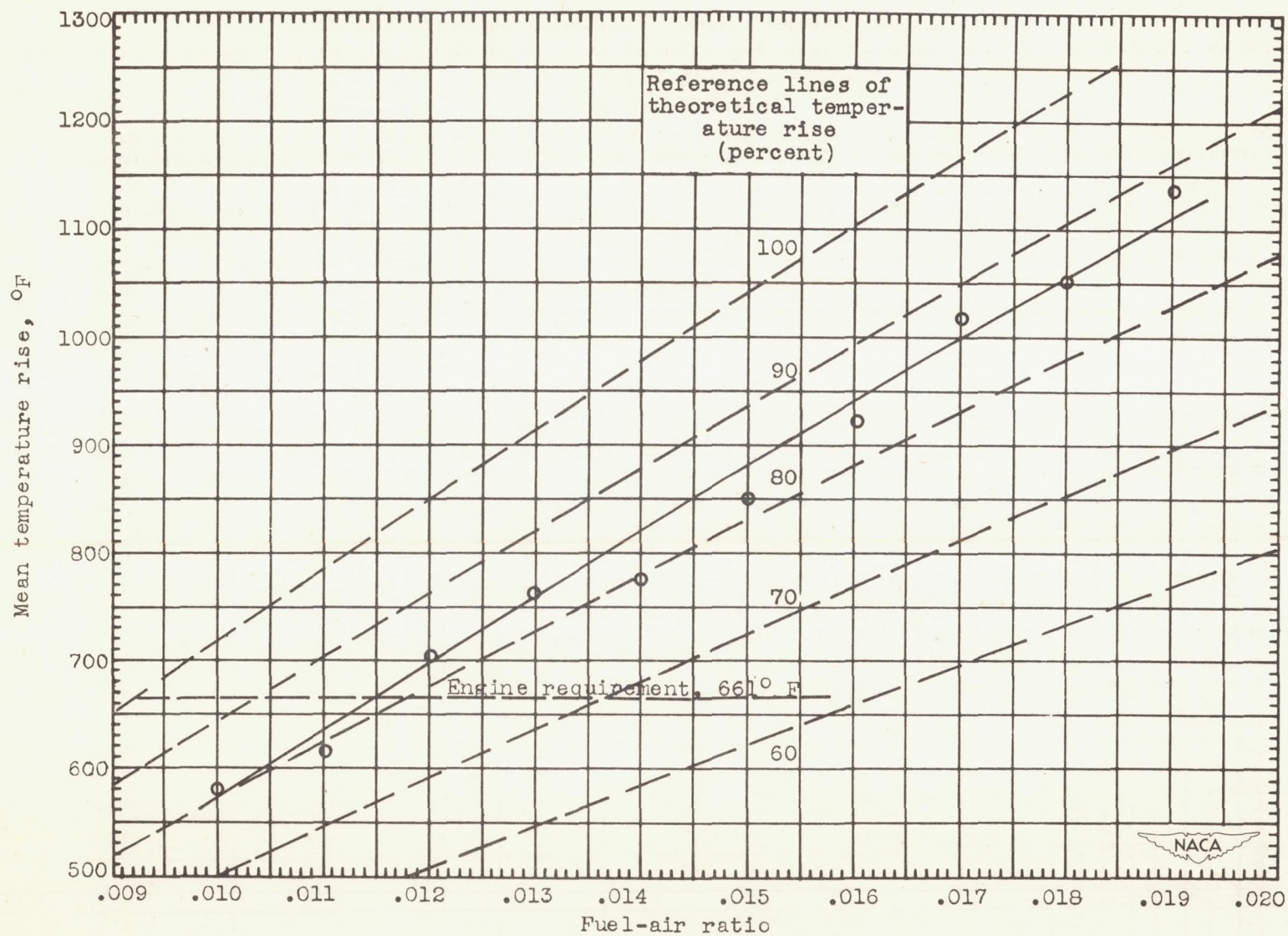
Figure 7. - Continued. Effect of fuel-air ratio on mean temperature rise through one-eighth segment of proposed turbojet combustor. Engine speed, 16,000 rpm.
