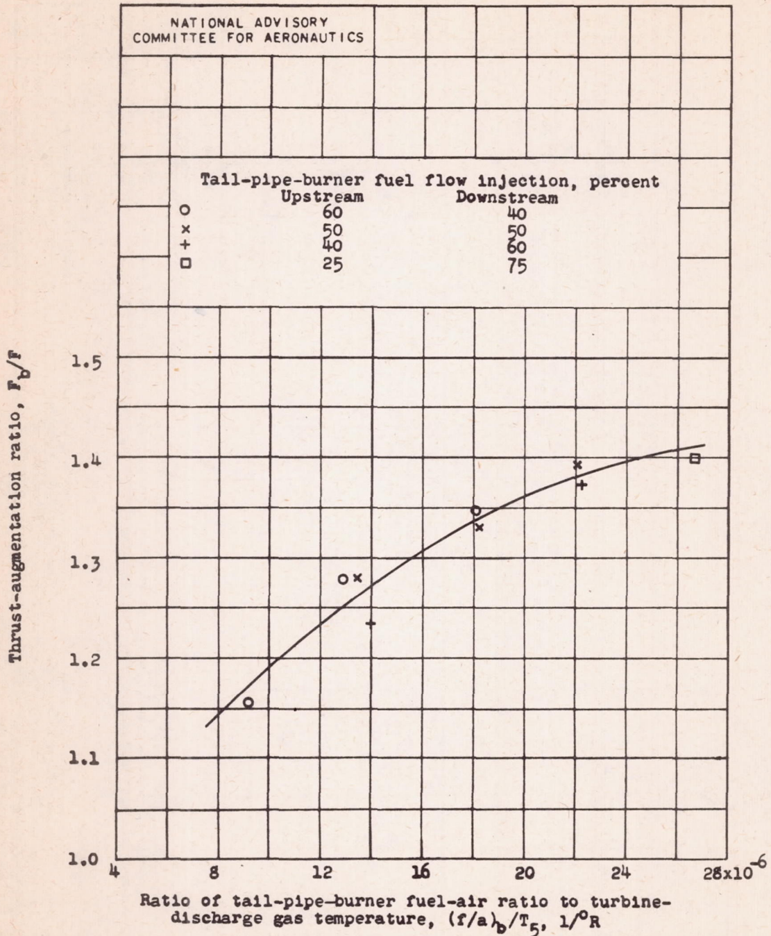
Figure 10. - Variation of thrust augmentation with ratio of tail-pipe-burner fuel-air ratio to turbine-discharge gas temperature at corrected rotor speed of approximately 7500 rpm.
