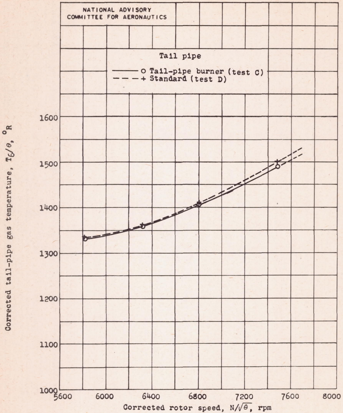
(c) Tail-pipe gas temperature.
