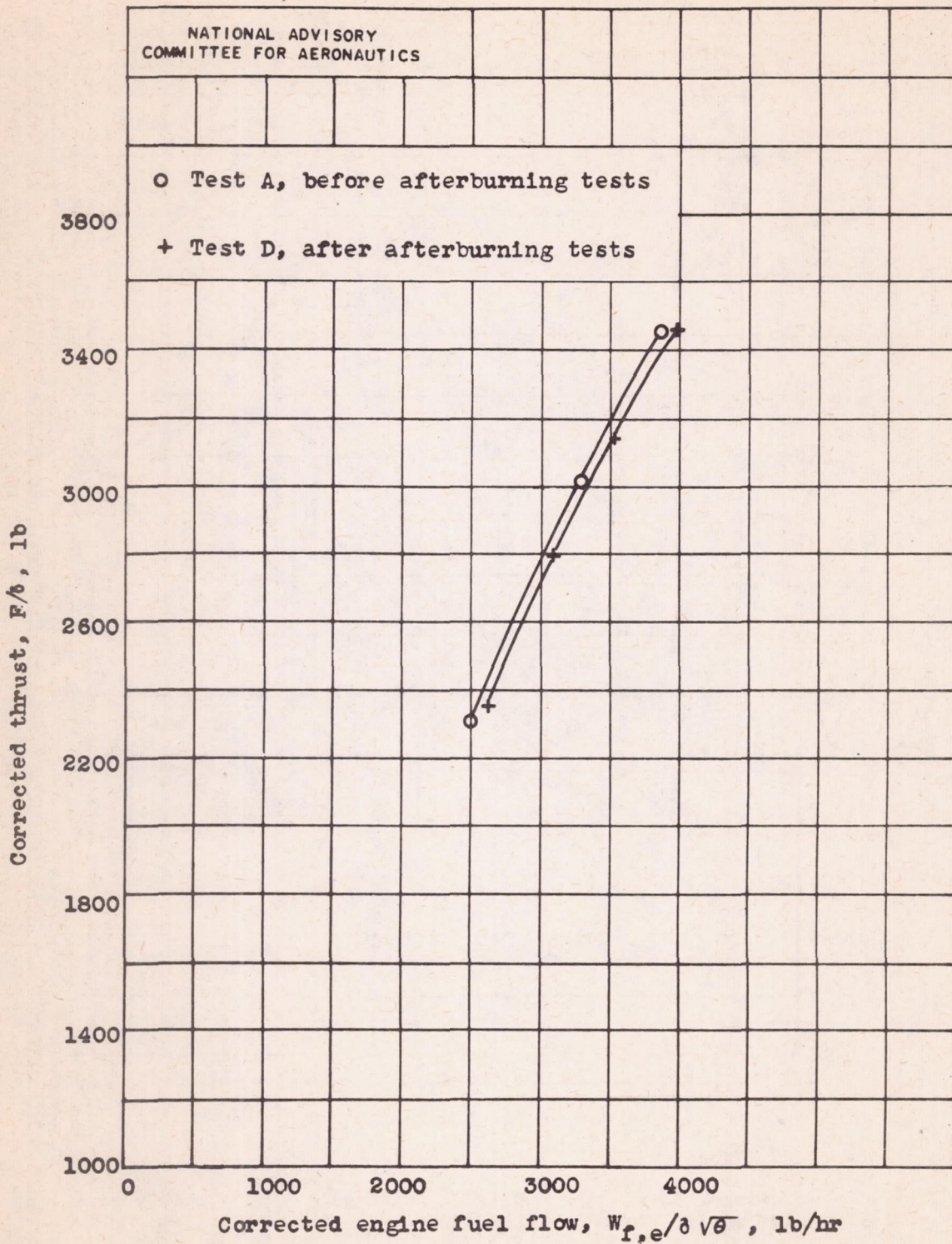
Figure 7. - Comparison of thrust for engine with standard tail pipe from tests A and D at corrected rotor speed of 7500 rpm.
