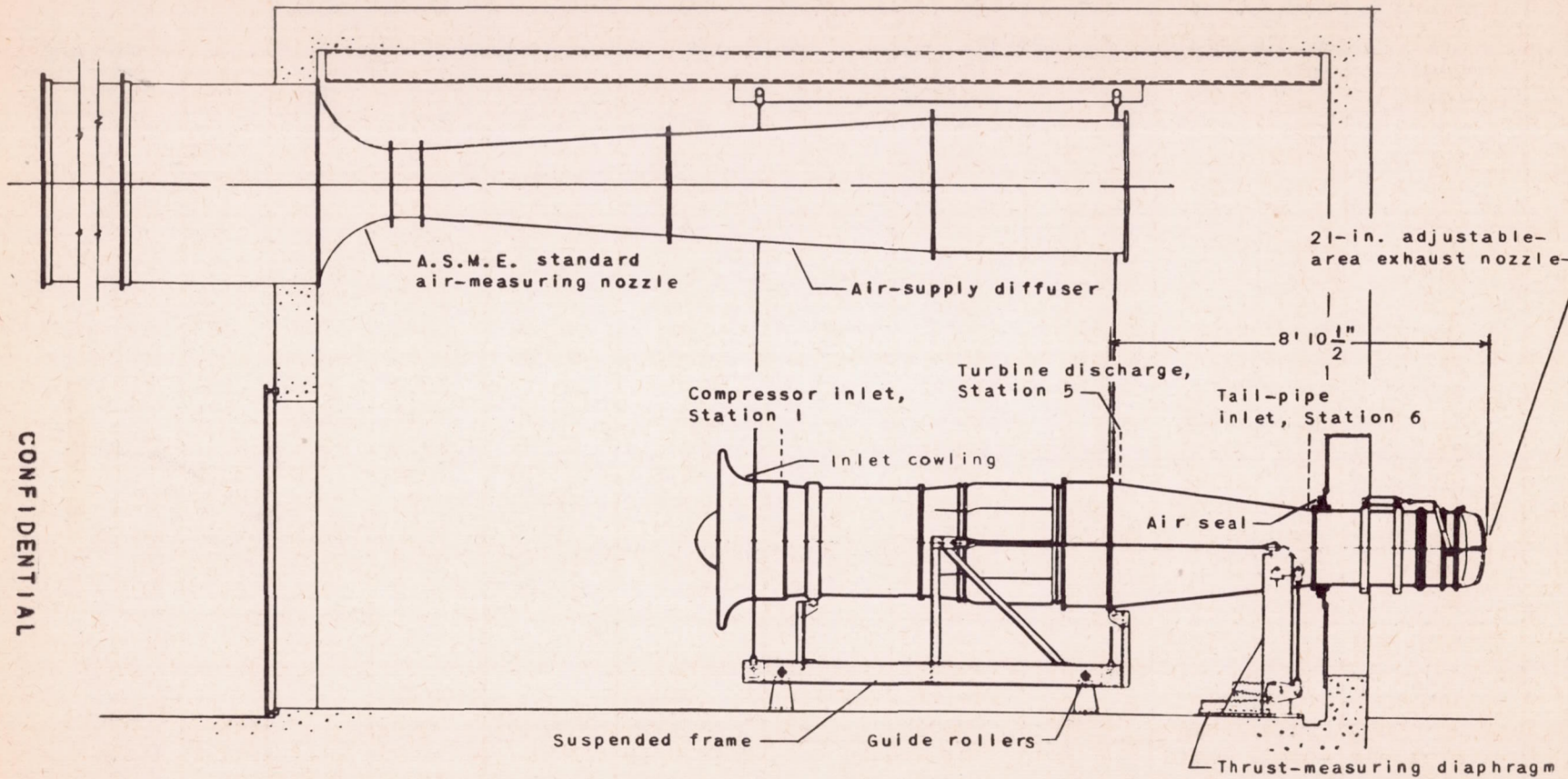
Figure 1. - Schematic diagram of installation of engine with standard tail pipe showing instrumentation stations.
