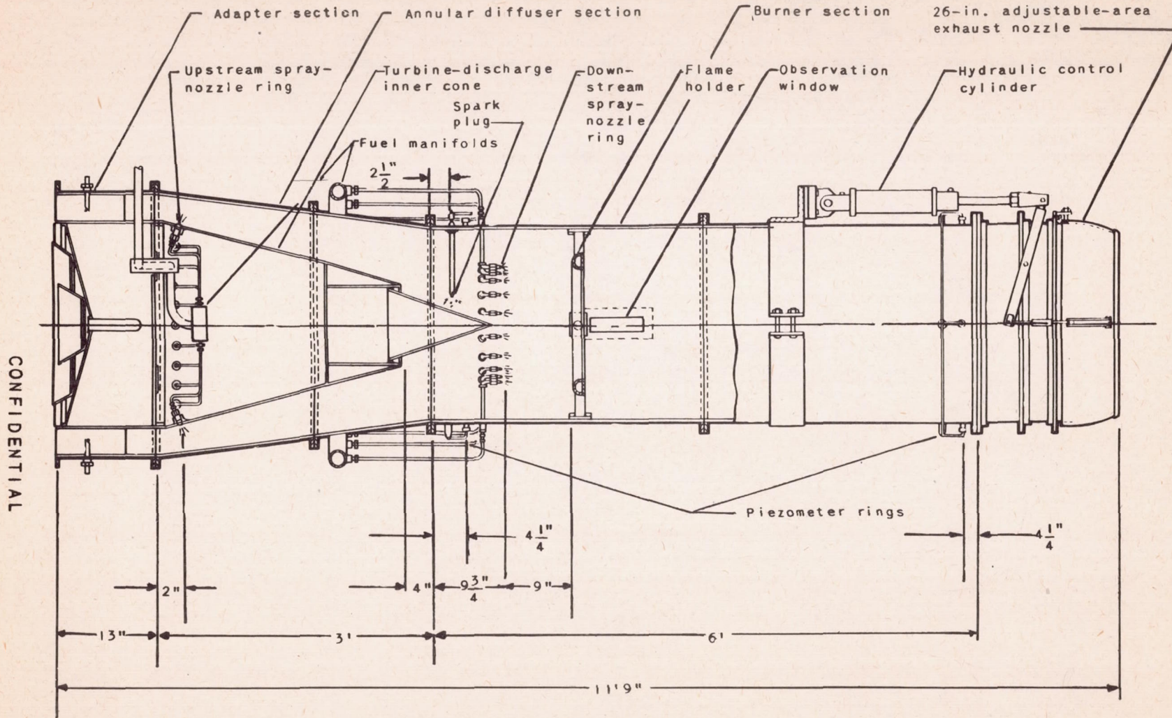
Figure 3. - Sketch of tail-pipe burner for turbojet engine.
