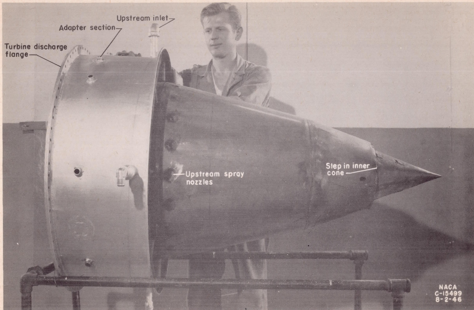
Figure 5. - View of adapter section and turbine-discharge inner cone for tail-pipe burner showing upstream spray nozzles and step in inner cone.
