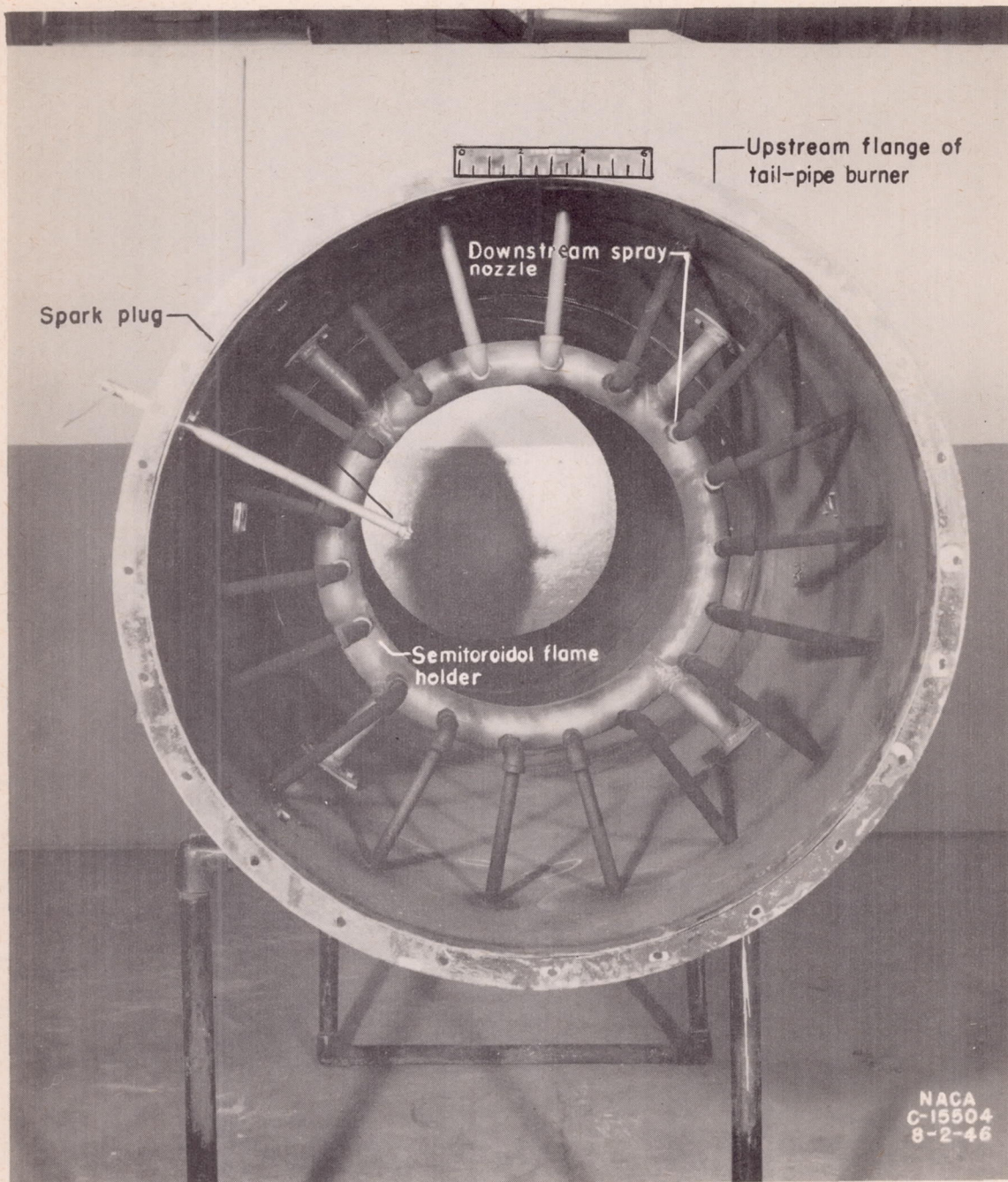
Figure 6. - Upstream view of tail-pipe burner showing downstream spray nozzles and flame holder.
