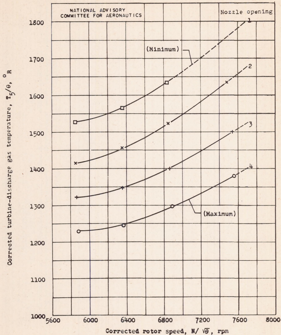
(c) Turbine-discharge gas temperature.
