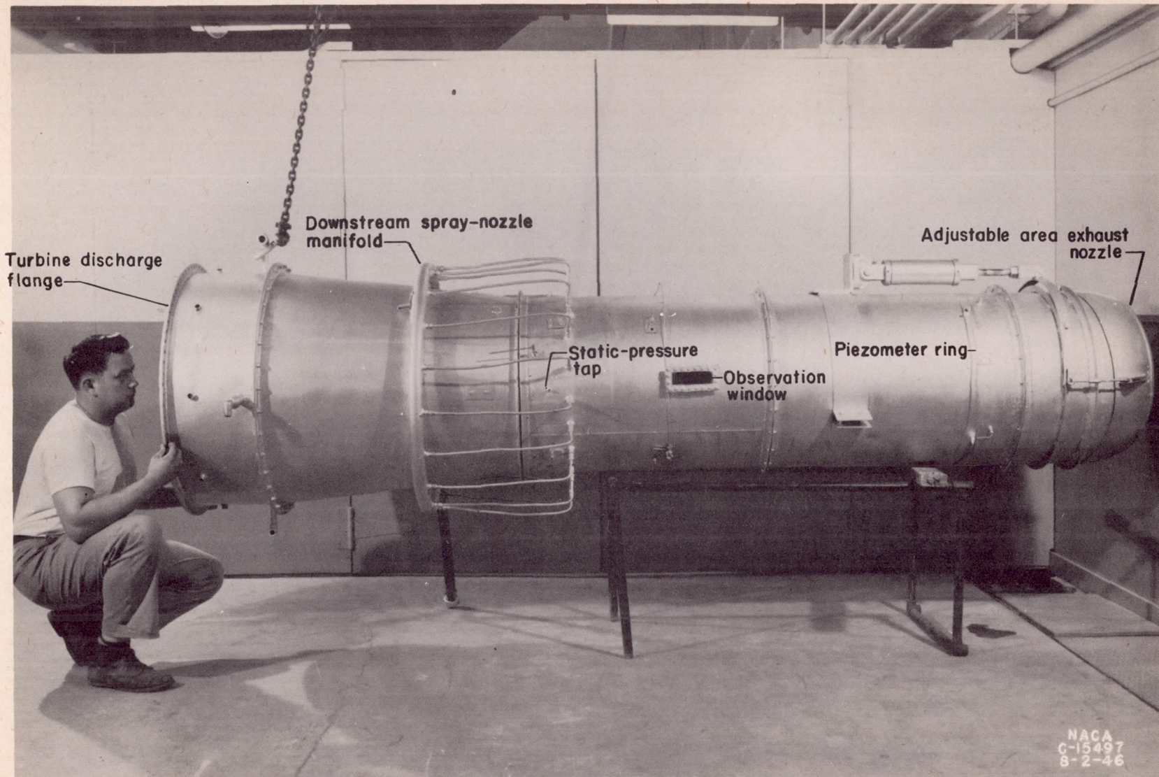
Figure 4. - View of completely assembled tail-pipe burner for turbojet engine.
