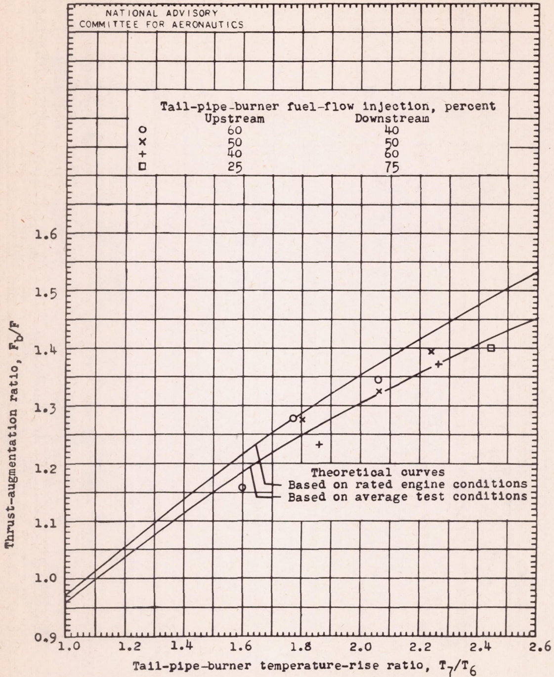
Figure 12. - Variation of thrust augmentation with tail-pipe-burner temperature-rise ratio.
