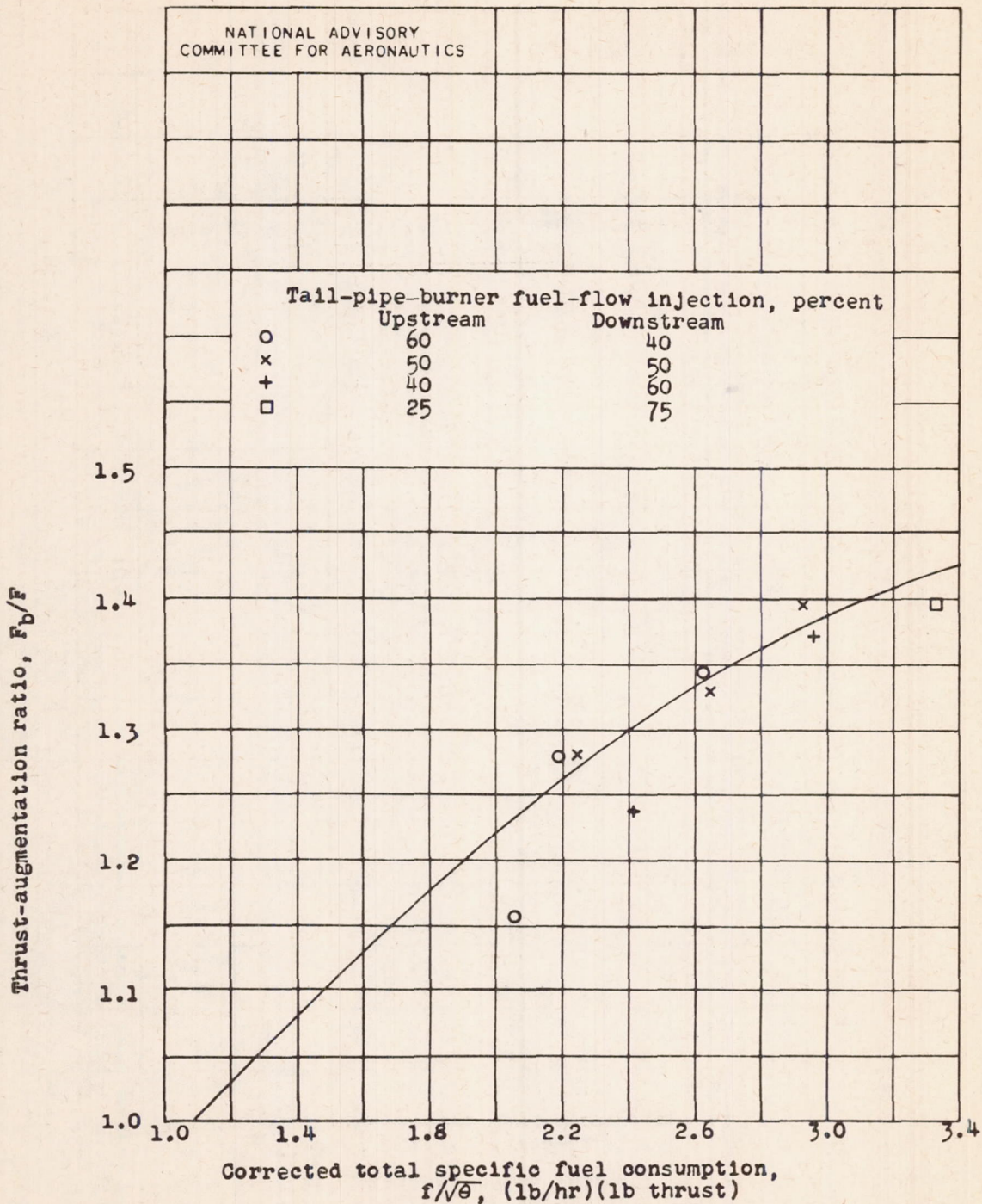
Figure 11. - Variation of thrust augmentation with total specific fuel consumption for corrected rotor speed of approximately 7500 rpm.
