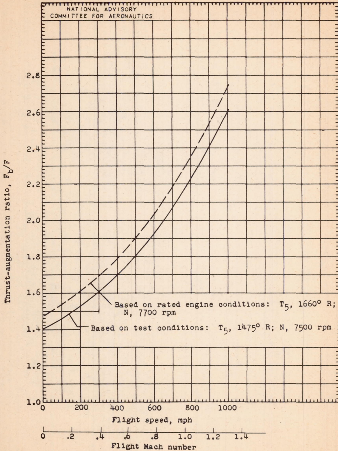
Figure 13. - Variation of calculated thrust augmentation with flight speed for constant turbine-discharge temperature and tail-pipe-burner temperature ratio of 2.34 at sea-level conditions.
