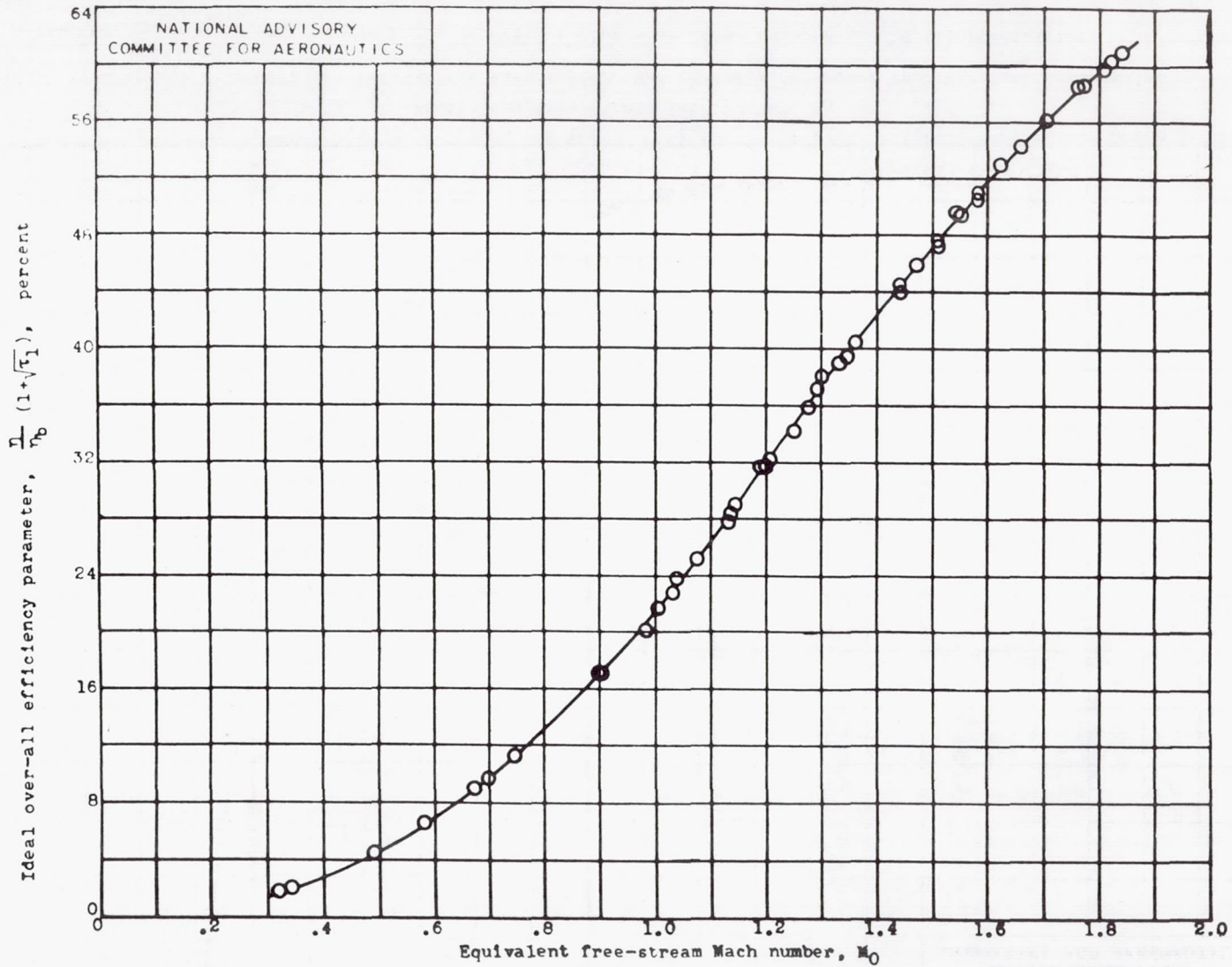
Figure 10.- Effect of equivalent free-stream Mach number M_0 on ideal over-all efficiency parameter \frac{\eta}{\eta_b} (1 + \sqrt{\tau_1}) . 20-inch ram jet with 5-foot combustion chamber and 16.8-inch-diameter exhaust nozzle.
