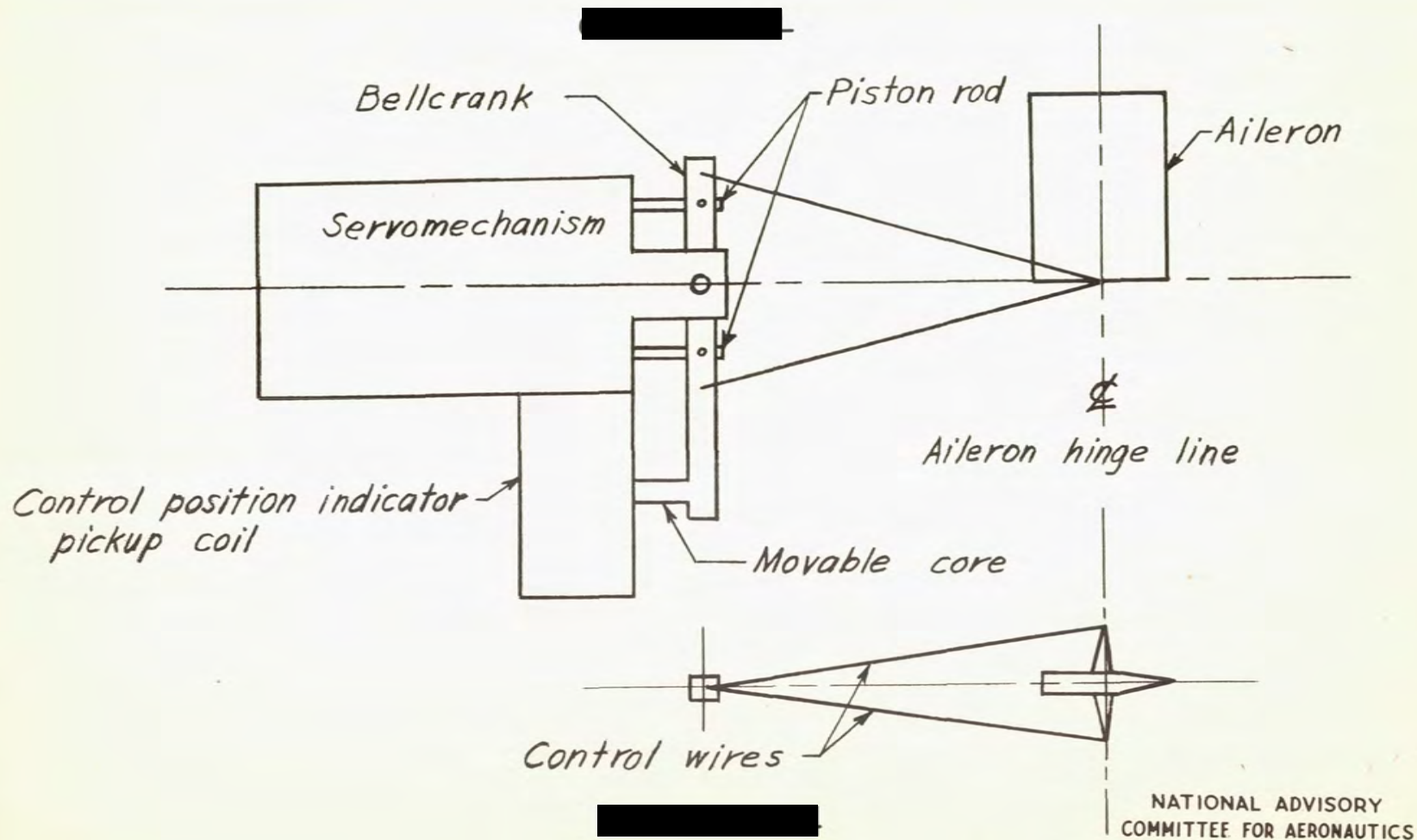
Figure 4.- Schematic sketch of aileron, servomechanism, and control position indicator arrangement.
