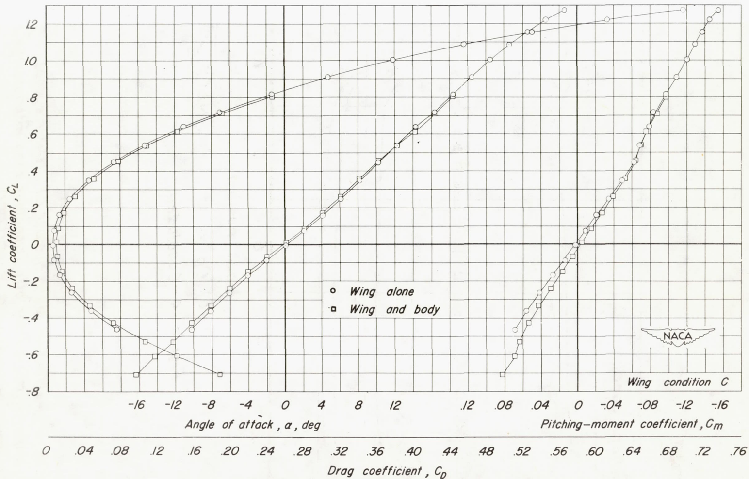
Figure 15.-The effect of the fuselage on the aerodynamic characteristics of a triangular wing at a Mach number of 0.18 and a Reynolds number of 15,000,000.
