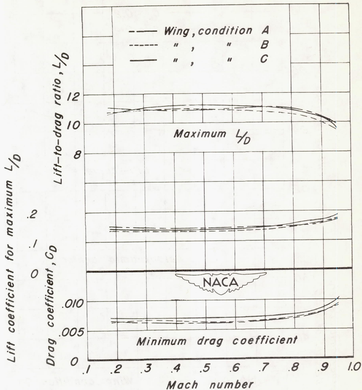
Figure 10.— The effect of Mach number on maximum lift-to-drag ratio and minimum drag of a triangular wing at a Reynolds number of 5,300,000 for three wing-profile conditions.
