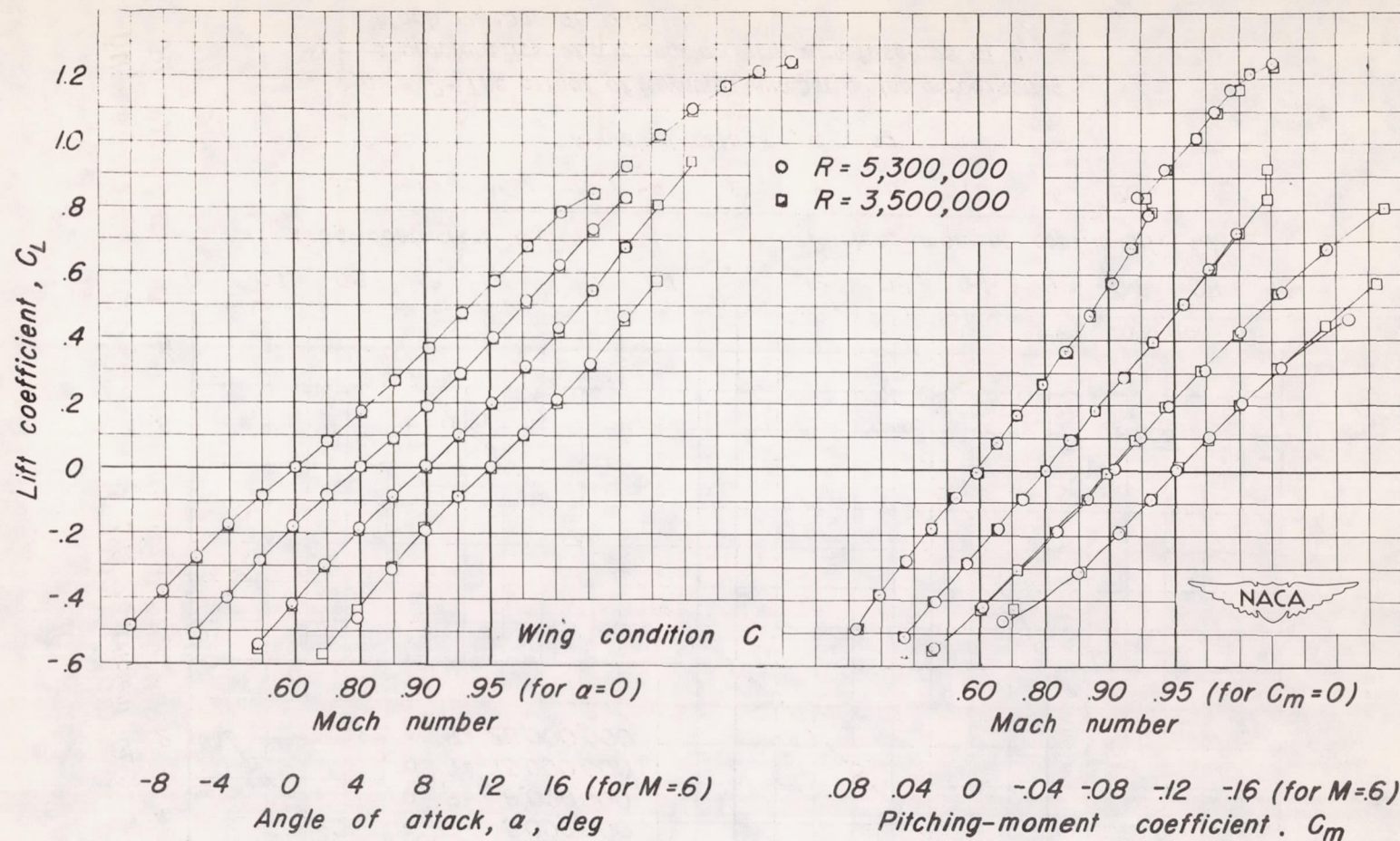
Figure 11.- The effect of Reynolds number on the aerodynamic characteristics of a triangular wing at several high subsonic Mach numbers.
