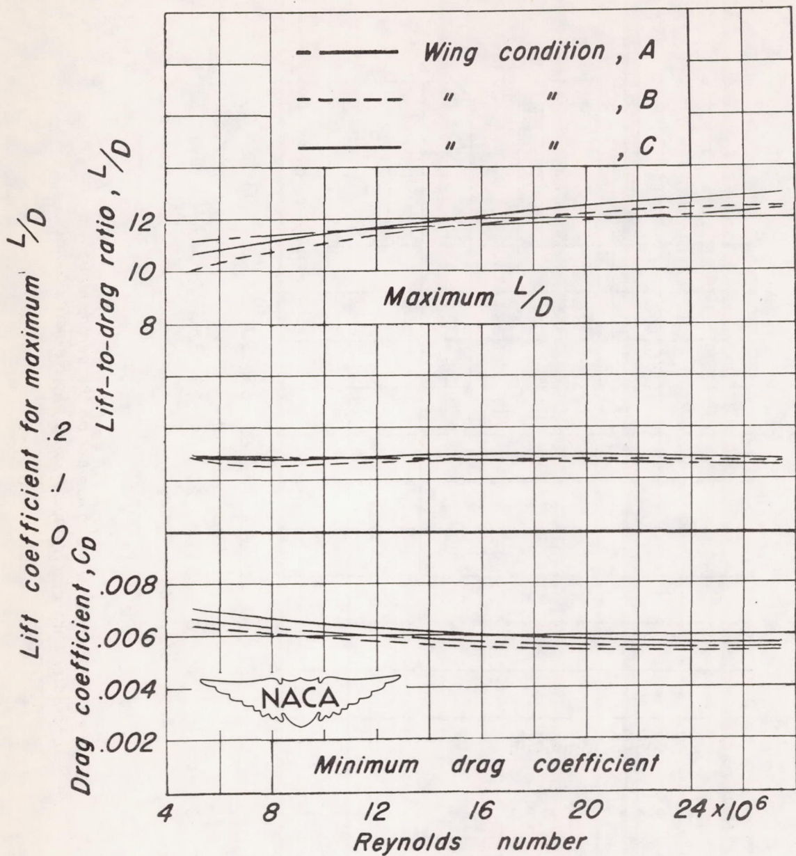
Figure 6.—The effect of Reynolds number on the maximum lift-to-drag ratio and minimum drag of a triangular wing at a Mach number of 0.18 for three wing-profile conditions.
