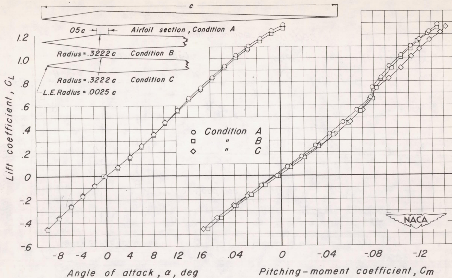
Figure 18.—The effect of minor modifications to the wing profile on the aerodynamic characteristics of a triangular wing at a Mach number of 0.18.
