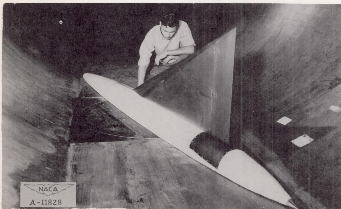
Figure 4.- Semispan wing-body combination mounted in the 12-foot pressure wind tunnel.
