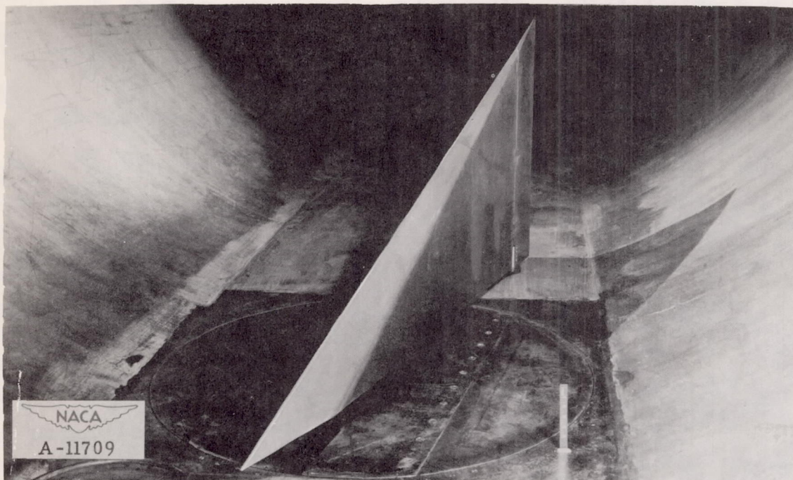
Figure 3.- Semispan wing, condition C, mounted in the 12-foot pressure wind tunnel.
