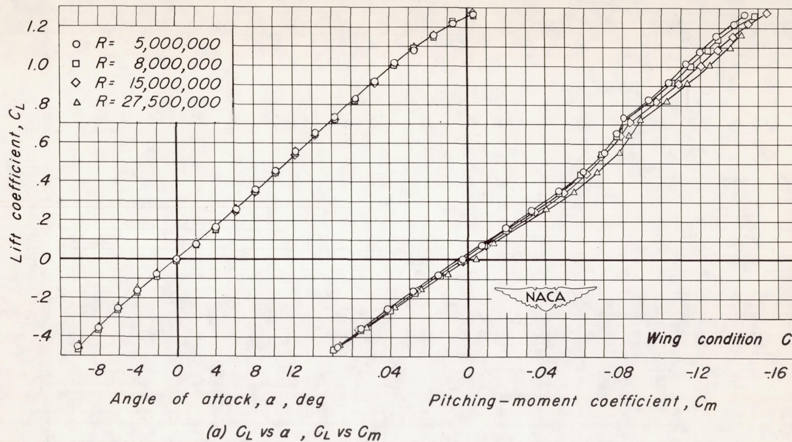
Figure 5.- The effect of Reynolds number on the aerodynamic characteristics of a triangular wing at a Mach number of 0.18.
