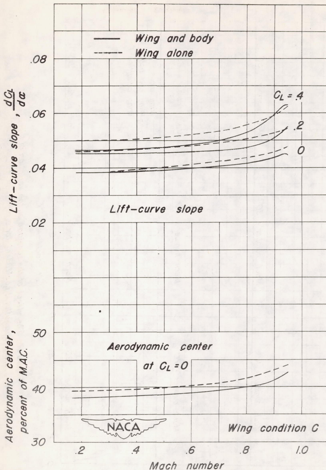
Figure 16.—The effect of Mach number on lift-curve slope and aerodynamic center of a triangular wing with fuselage at a Reynolds number of 5,300,000.
