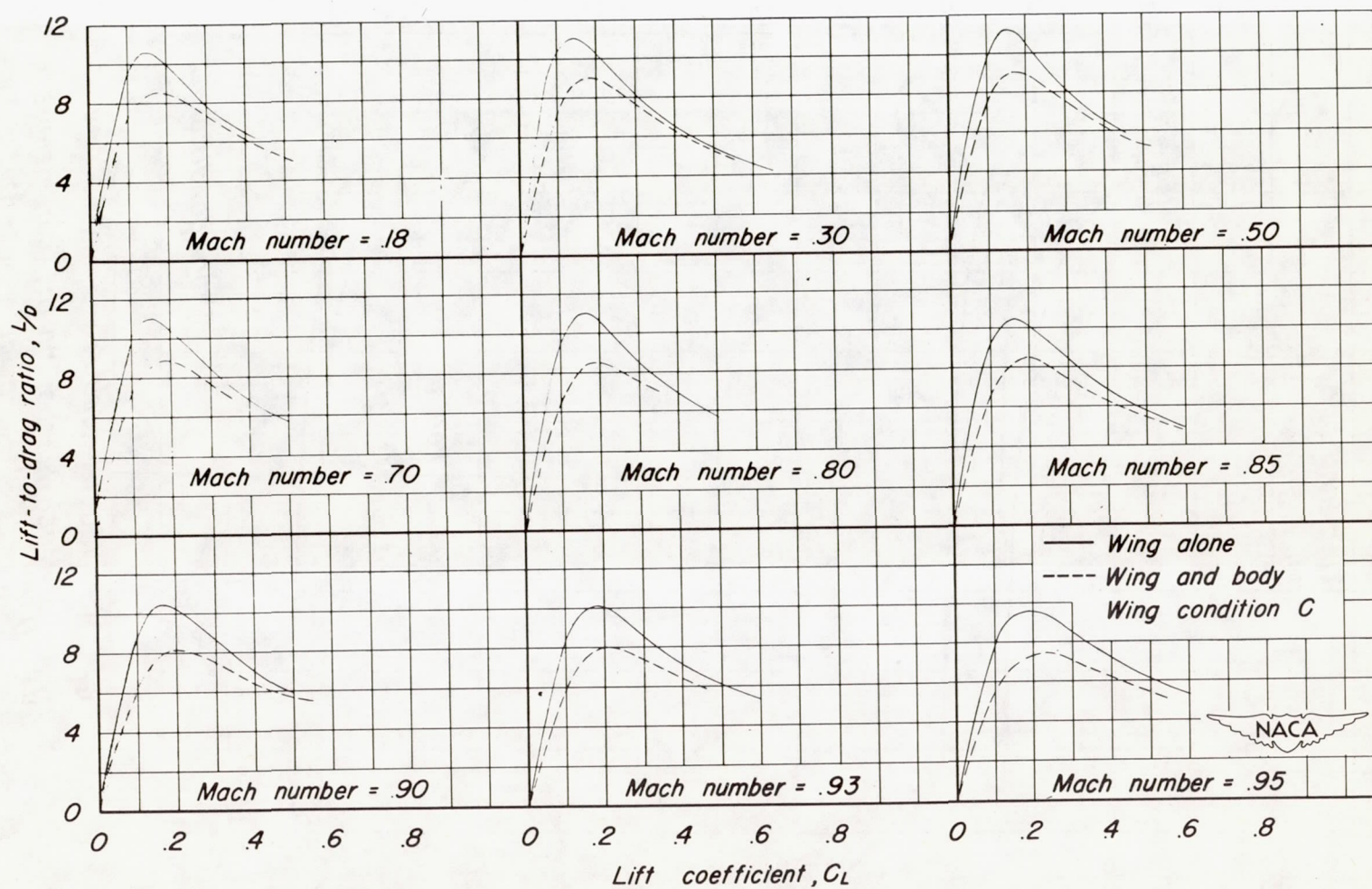
Figure 17 - The effect of the fuselage on the variation of lift-drag ratio with lift coefficient for a triangular wing at several Mach numbers and a Reynolds number of 5,300,000.
