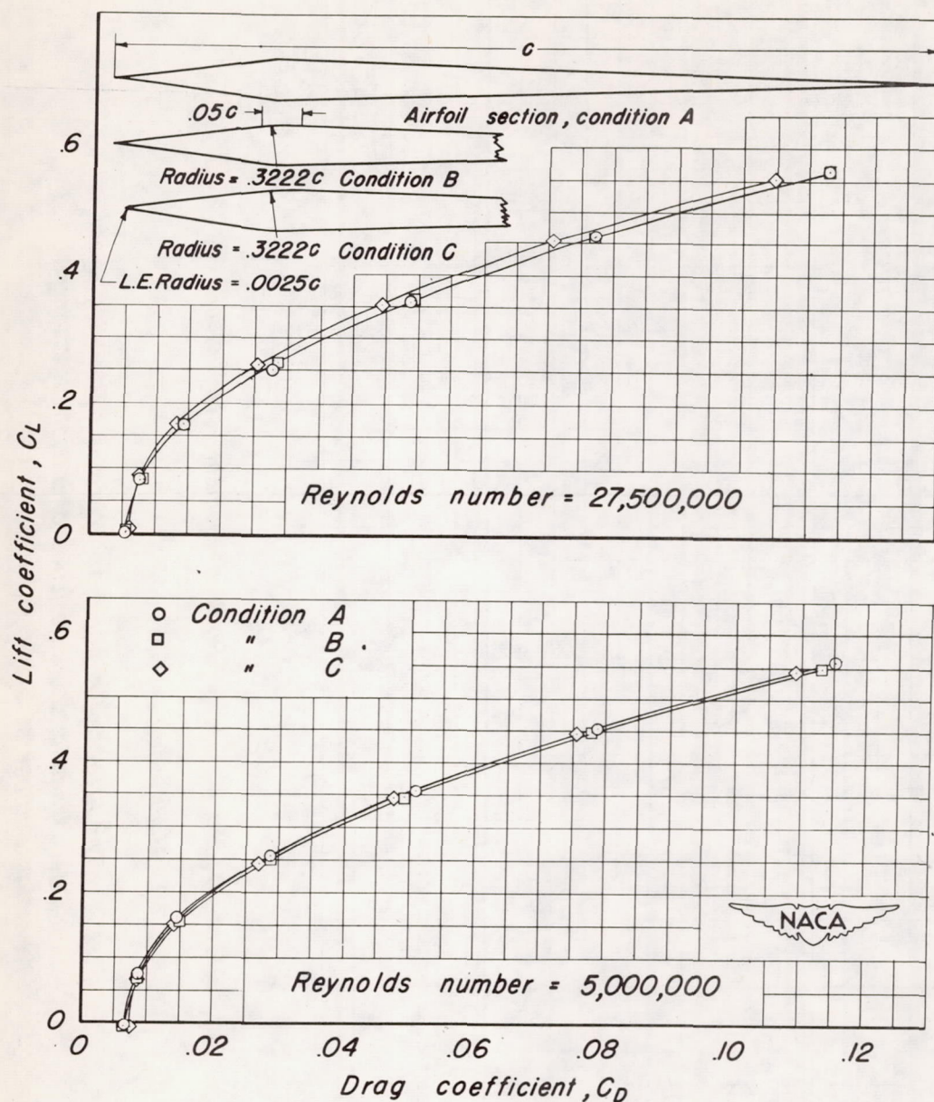
Figure 19.- The effect of minor modifications to the wing profile on the drag characteristics of a triangular wing at a Mach number of 0.18.
