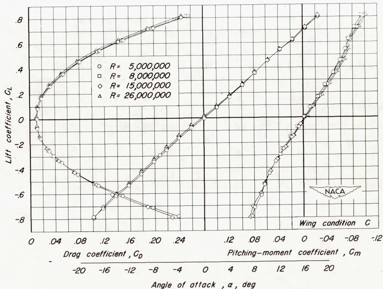
Figure 12.—The effect of Reynolds number on the aerodynamic characteristics of a triangular wing with fuselage at a Mach number of 0.18.
