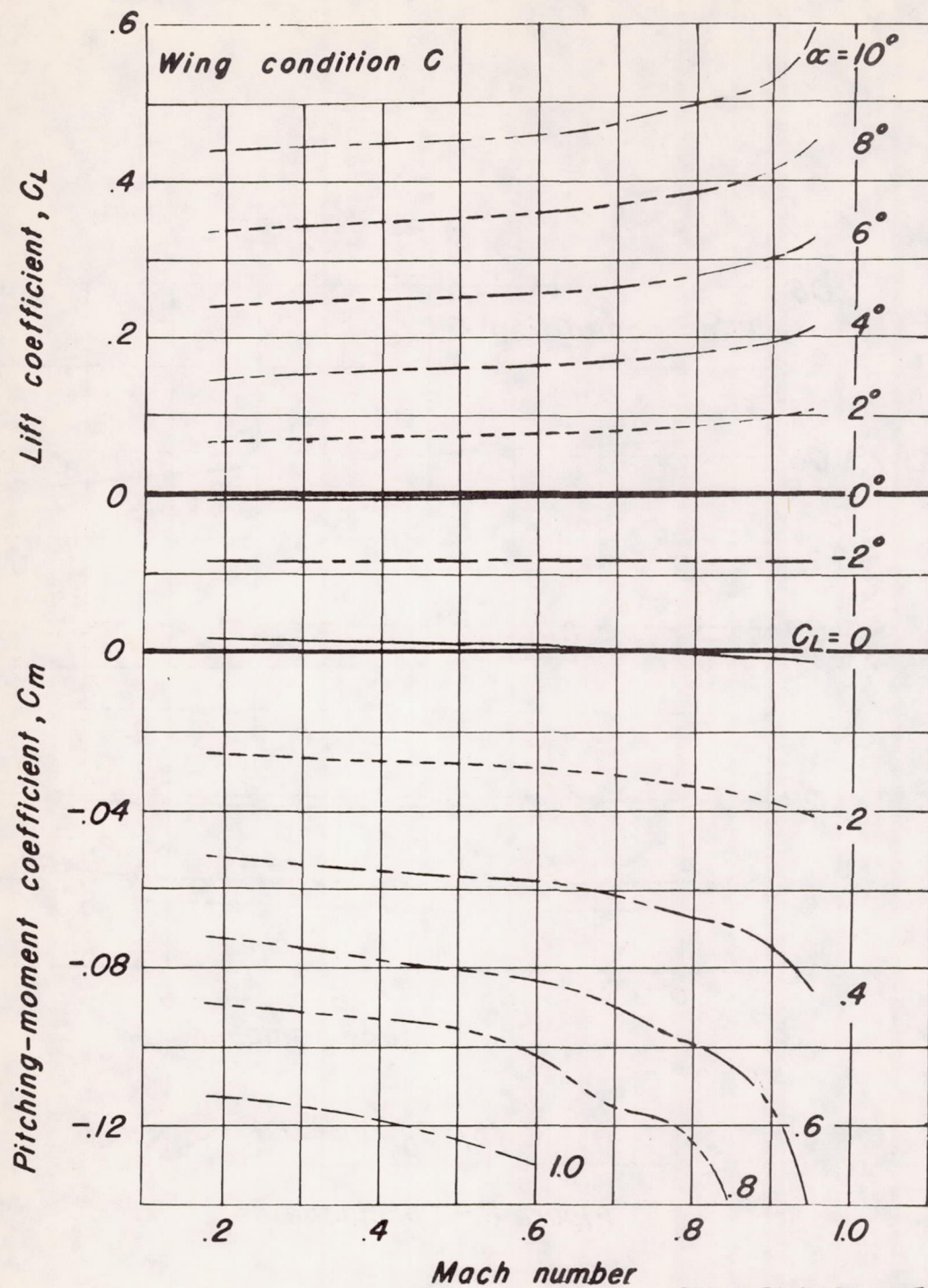
(a) C_L vs M , C_m vs M
