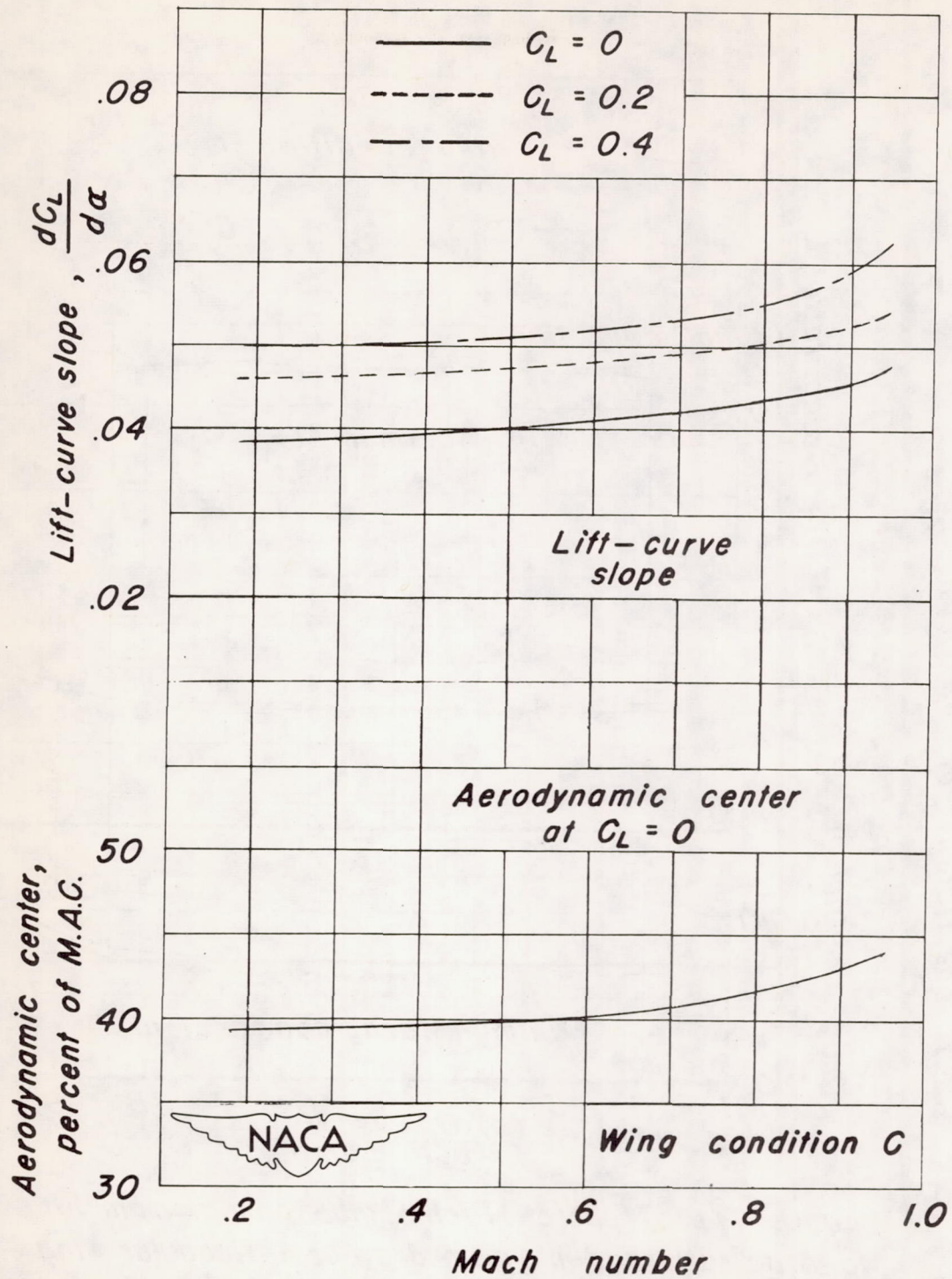
Figure 9.-The effect of Mach number on lift-curve slope and aerodynamic center of a triangular wing at a Reynolds number of 5,300,000.
