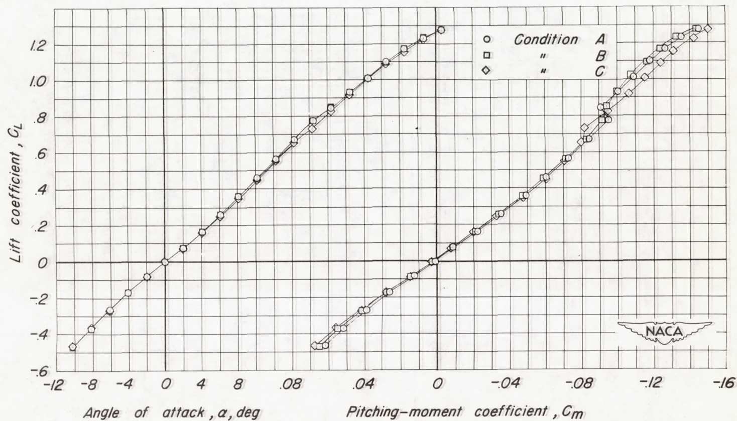
Figure 20.- The effect of minor modifications to the wing profile on the aerodynamic characteristics of a triangular wing at a Reynolds number of 5,300,000.
