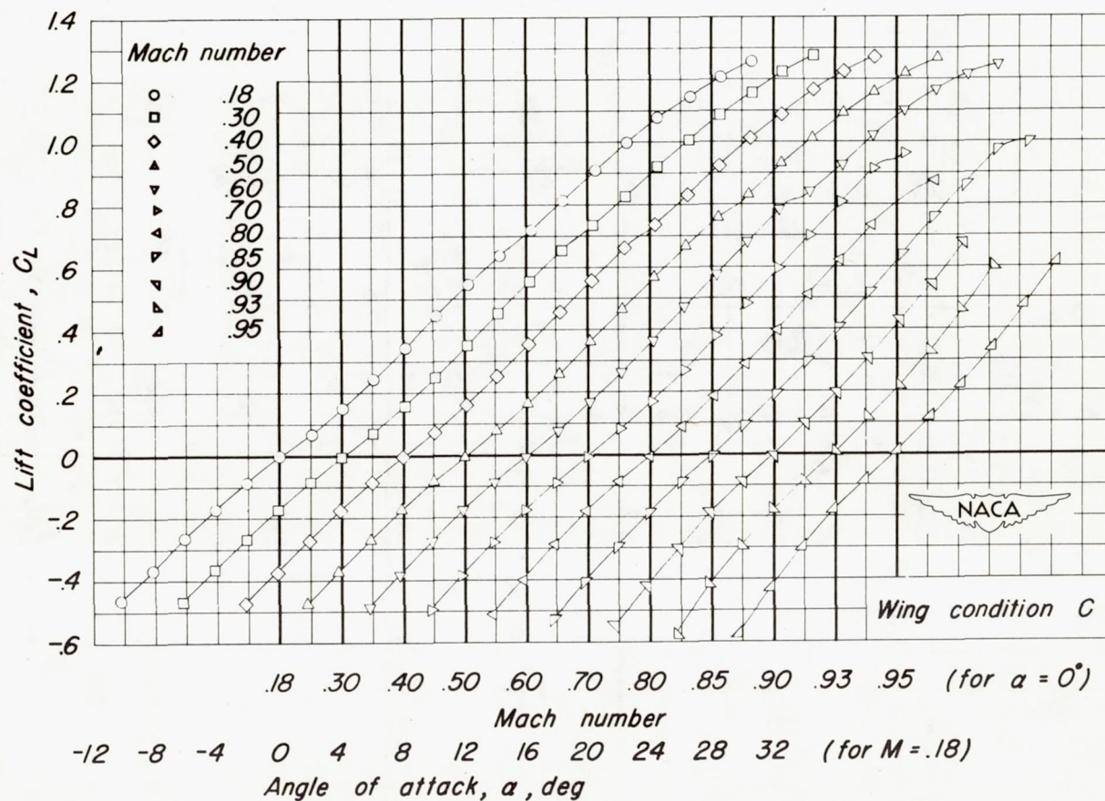
Figure 7.—The effect of Mach number on the aerodynamic characteristics of a triangular wing at a Reynolds number of 5,300,000.
