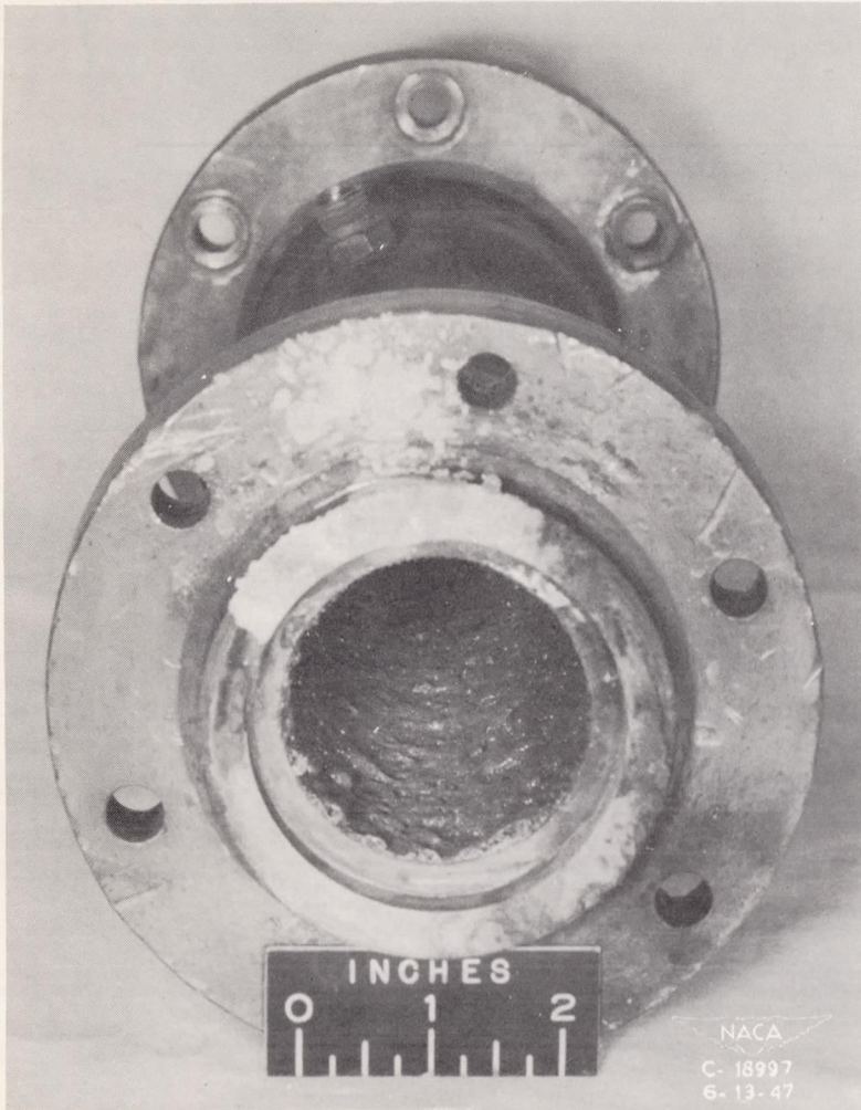
(a) Chamber wall of exhaust end.
