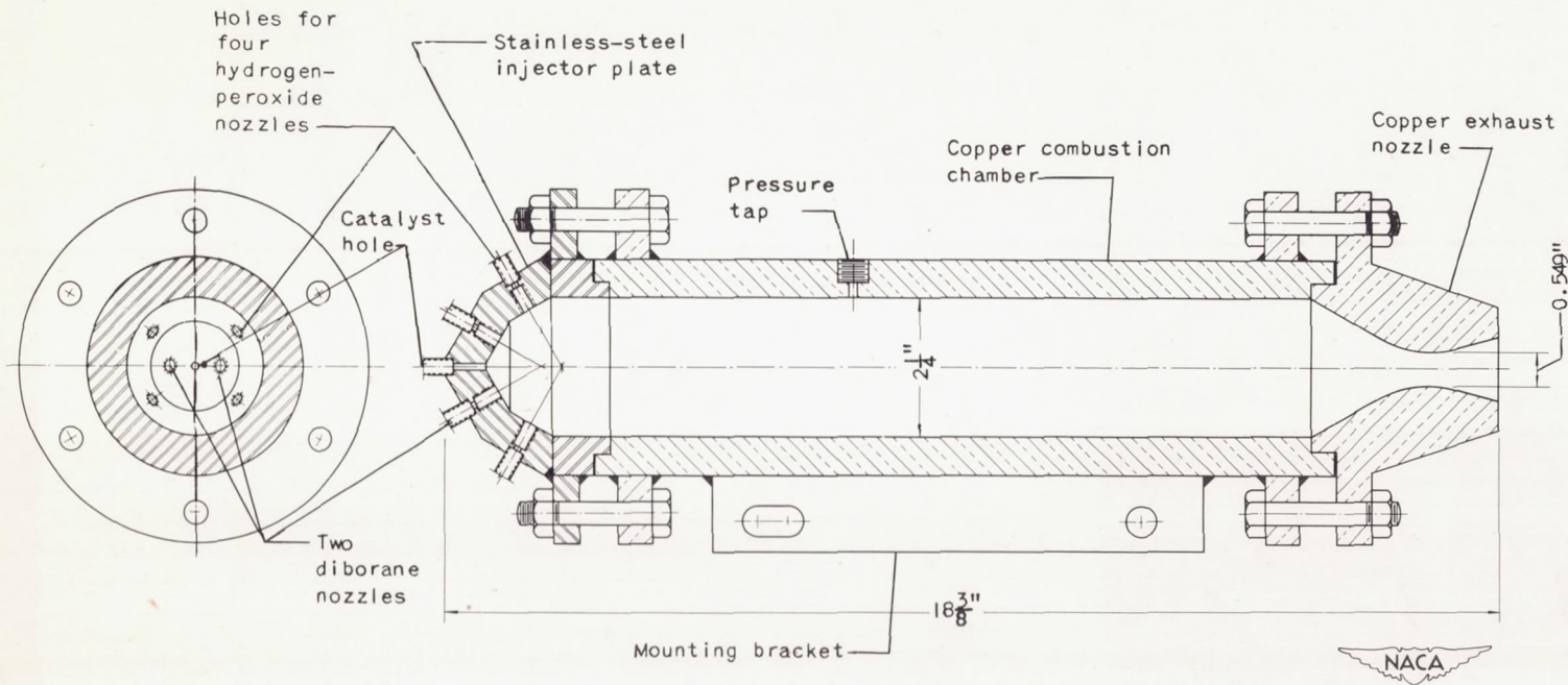
Figure 3. - 100-pound thrust rocket engine.
