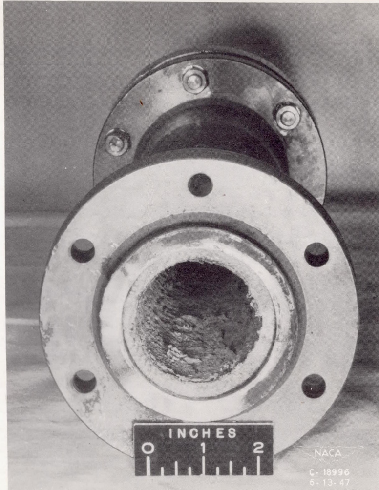
(b) Chamber wall of injection end.
