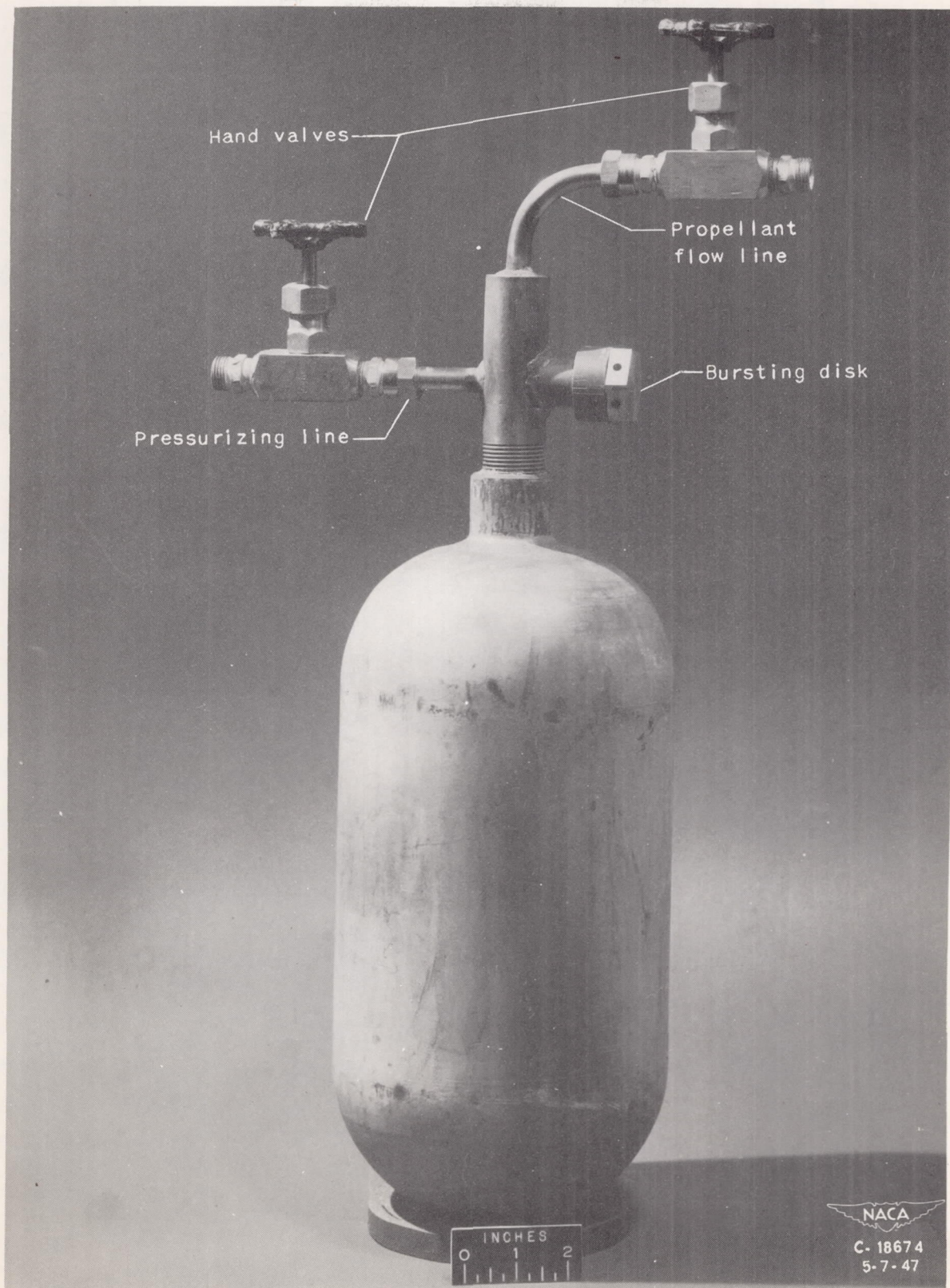
Figure 2. - Chrome-molybdenum steel tank for diborane.
