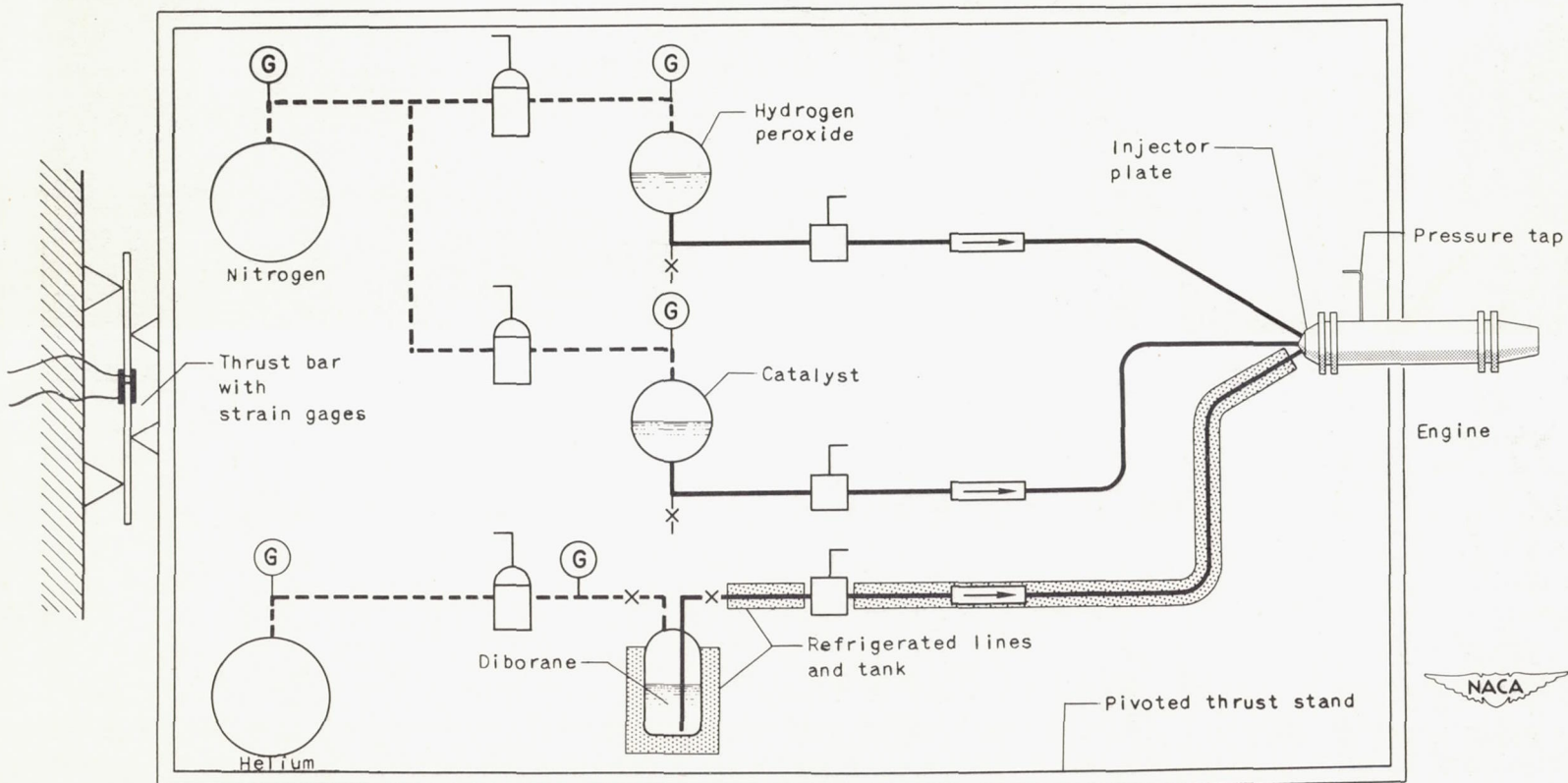
Figure 1. - Diagrammatic sketch of 100-pound-thrust rocket unit.
