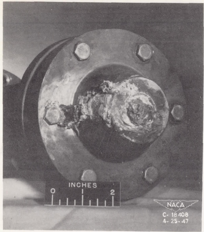
(a) Exhaust nozzle.
