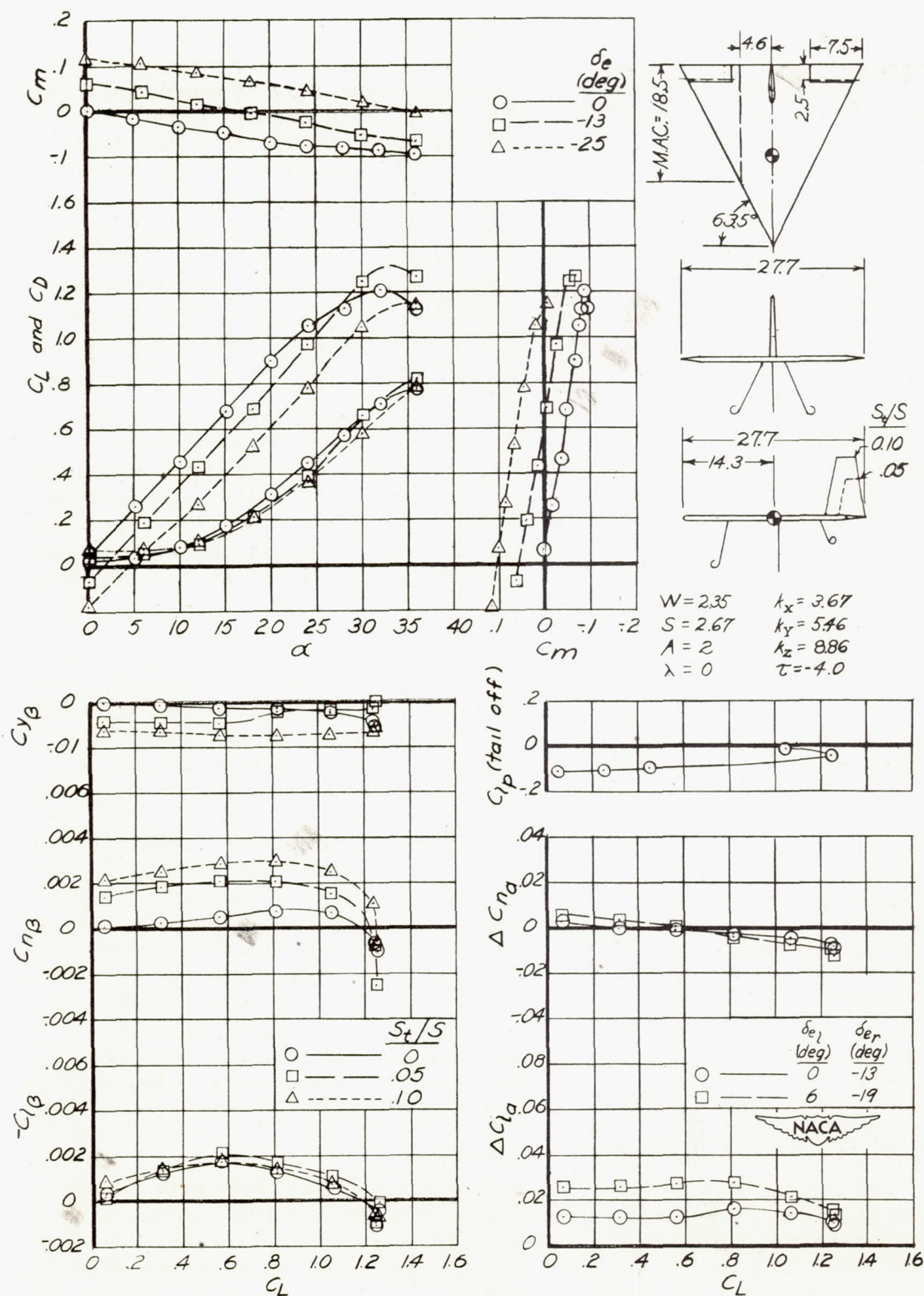
Figure 4.- Aerodynamic characteristics of model 4.
