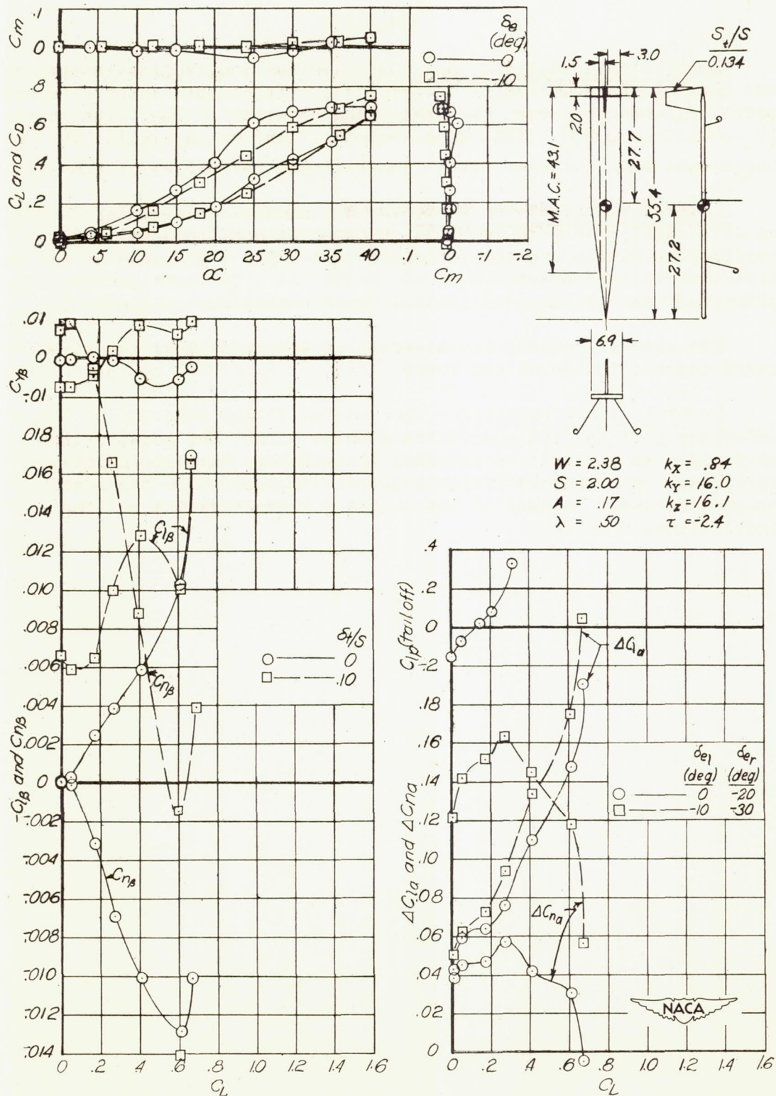
Figure 9.- Aerodynamic characteristics of model 9.
