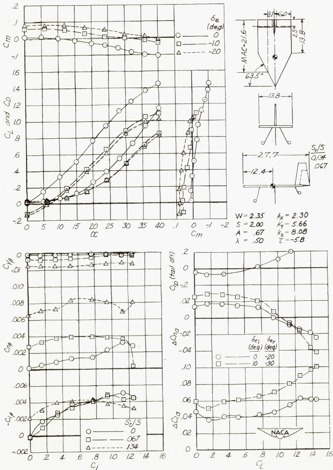
Figure 5.- Aerodynamic characteristics of model 5.
