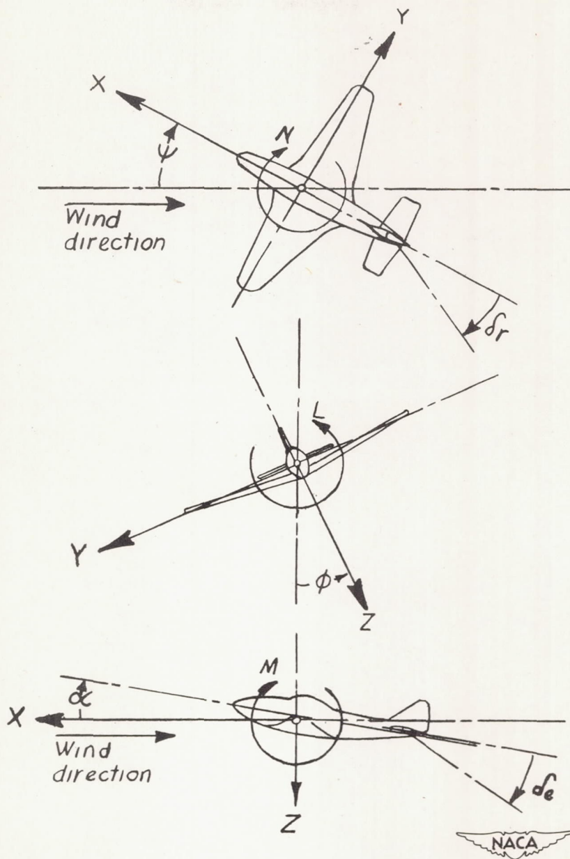
Figure 12: The stability system of axes. Arrows indicate positive directions of moments, forces, and control-surface deflections. This system of axes is defined as an orthogonal system having their origin at the center of gravity and in which the Z-axis is in the plane of symmetry and perpendicular to the relative wind, the X-axis is in the plane of symmetry and perpendicular to the Z-axis, and the Y-axis is perpendicular to the plane of symmetry.
