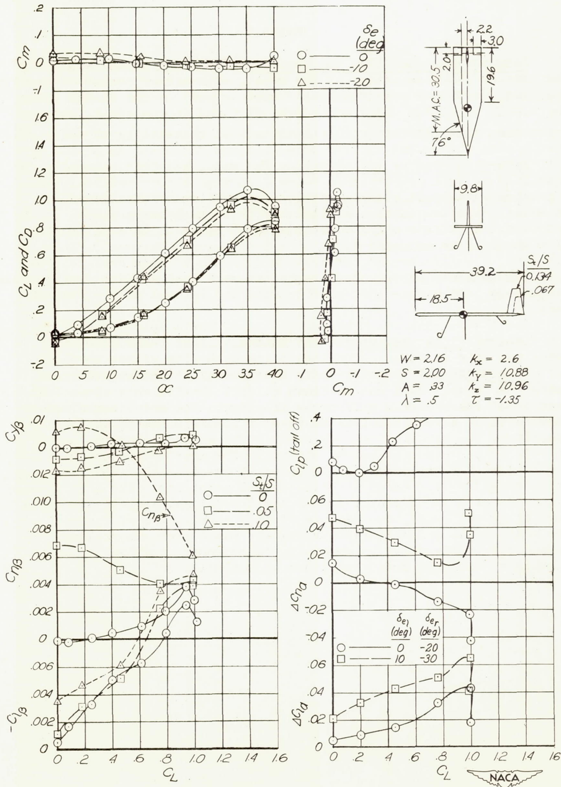
Figure 7.- Aerodynamic characteristics of model 7.
