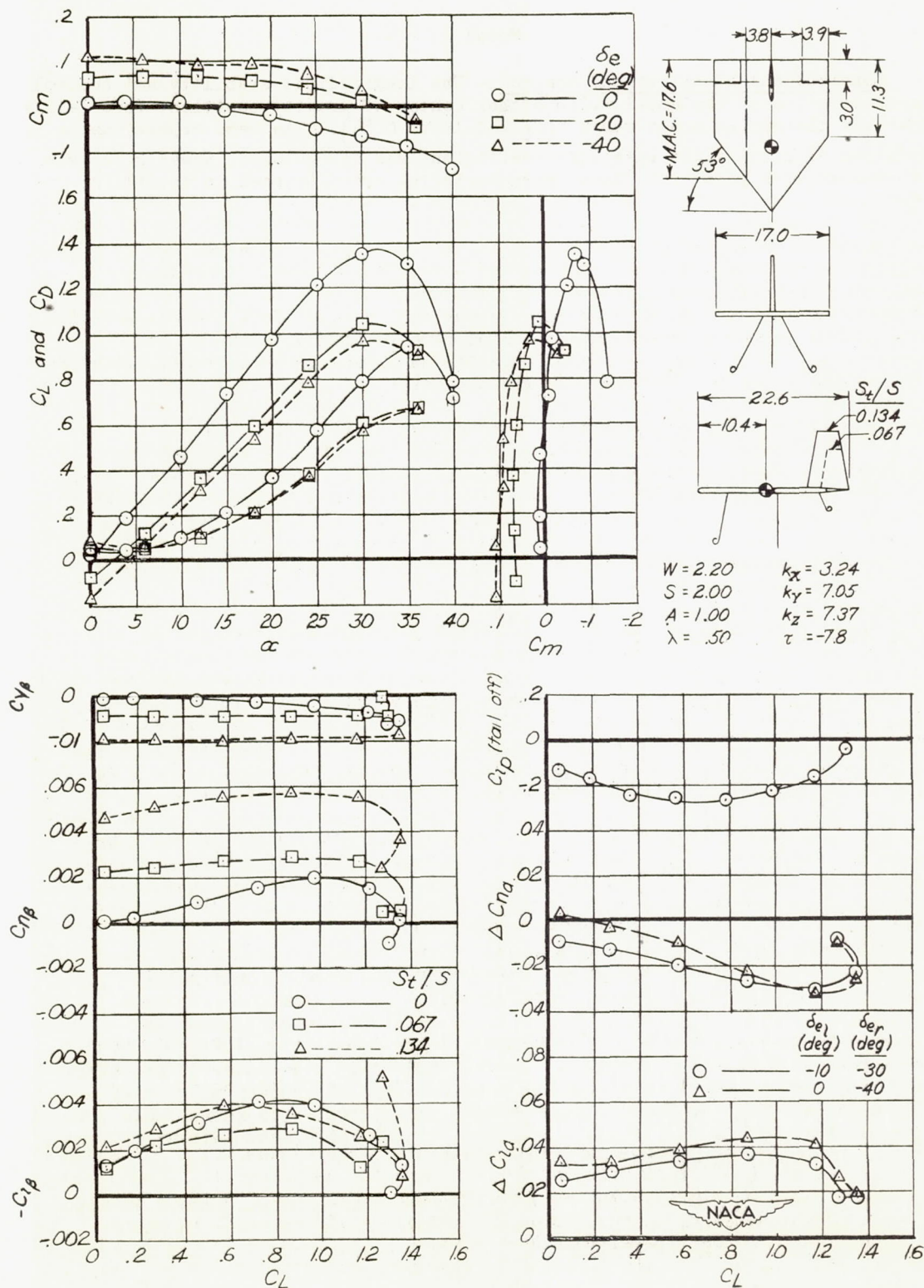
Figure 3.- Aerodynamic characteristics of model 3.
