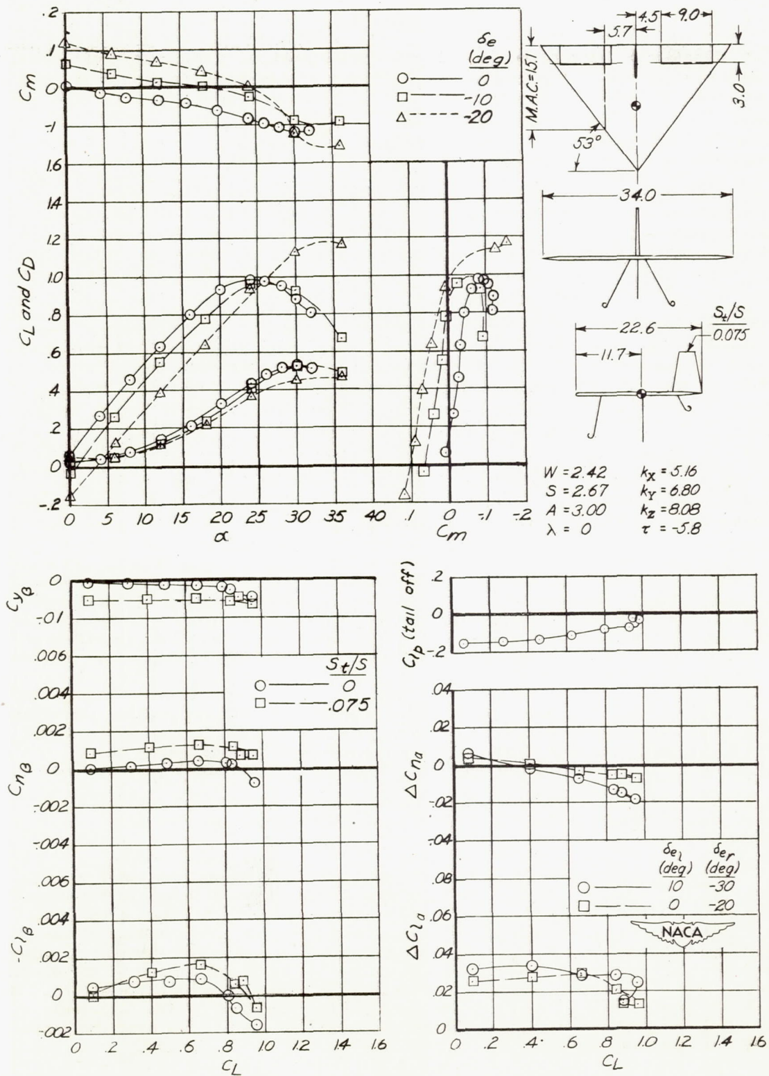
Figure 1.- Aerodynamic characteristics of model 1.
