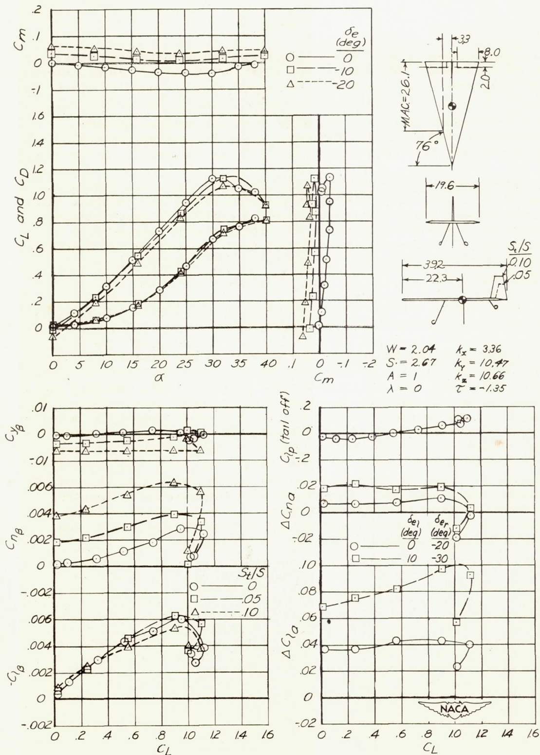
Figure 6.- Aerodynamic characteristics of model 6.
