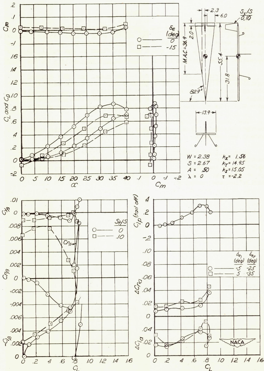
Figure 8.- Aerodynamic characteristics of model 8.
