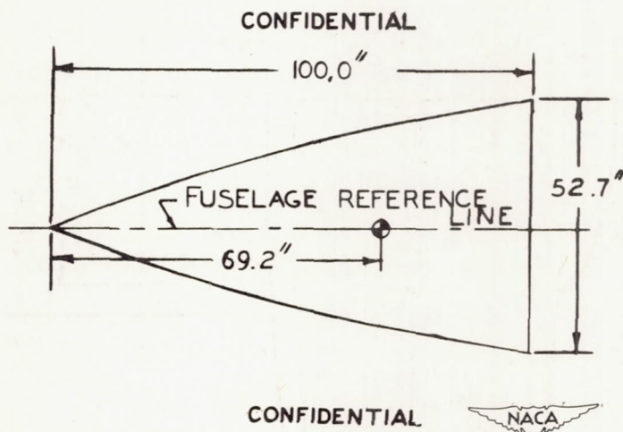
FIGURE 4.-SKETCH OF THE \frac{1}{12} -SCALE MODEL OF THE JETTISONABLE NOSE SECTION OF THE DOUGLAS D-558, PHASE II, AIRPLANE TESTED IN THE FREE-SPINNING TUNNEL. CENTER OF GRAVITY IS SHOWN FOR THE ORIGINAL LOADING CONDITION. DIMENSIONS ARE FULL-SCALE VALUES.
