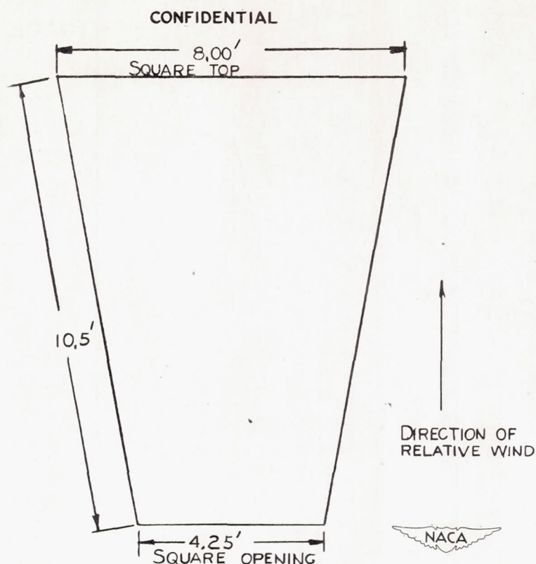
FIGURE 8.-SKETCH OF BOX-TYPE PARACHUTE A, USED AS STABILIZING PARACHUTE FOR THE \frac{1}{12} -SCALE MODEL OF THE D-558, PHASE II, AIRPLANE NOSE SECTION IN THE FREE-SPINNING TUNNEL. PARACHUTE IS SHOWN FULLY OPENED. EIGHT SHROUD LINES AVERAGING 10.6 FEET IN LENGTH WERE ATTACHED TO THE BOTTOM OF THE PARACHUTE AT THE CORNERS AND MIDWAY OF EACH SIDE. DIMENSIONS ARE FULL-SCALE.
