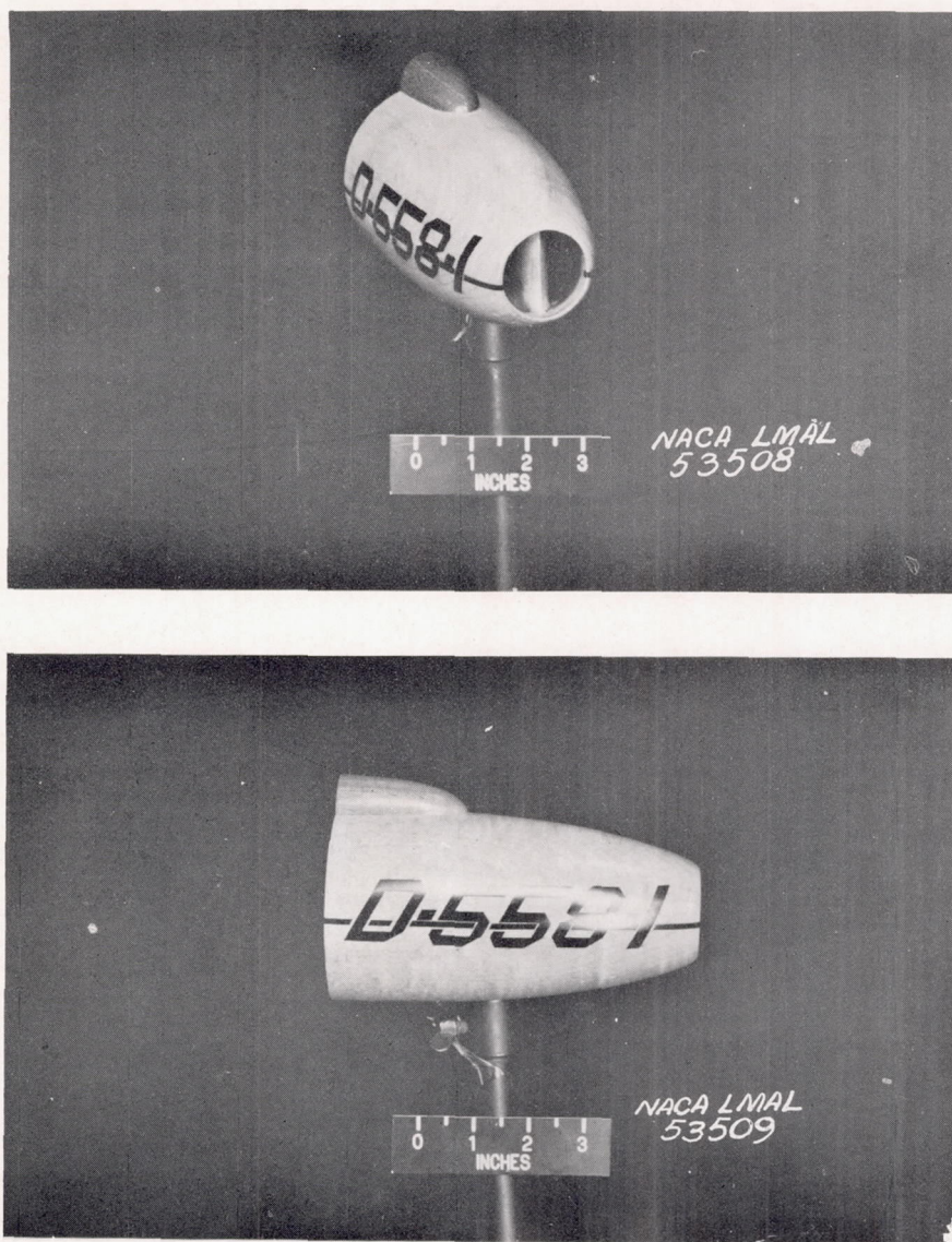
Figure 1.- Photographs of the \frac{1}{14} -scale model of the jettisonable nose section of the Douglas D-558, phase I, airplane tested in the free-spinning tunnel.
