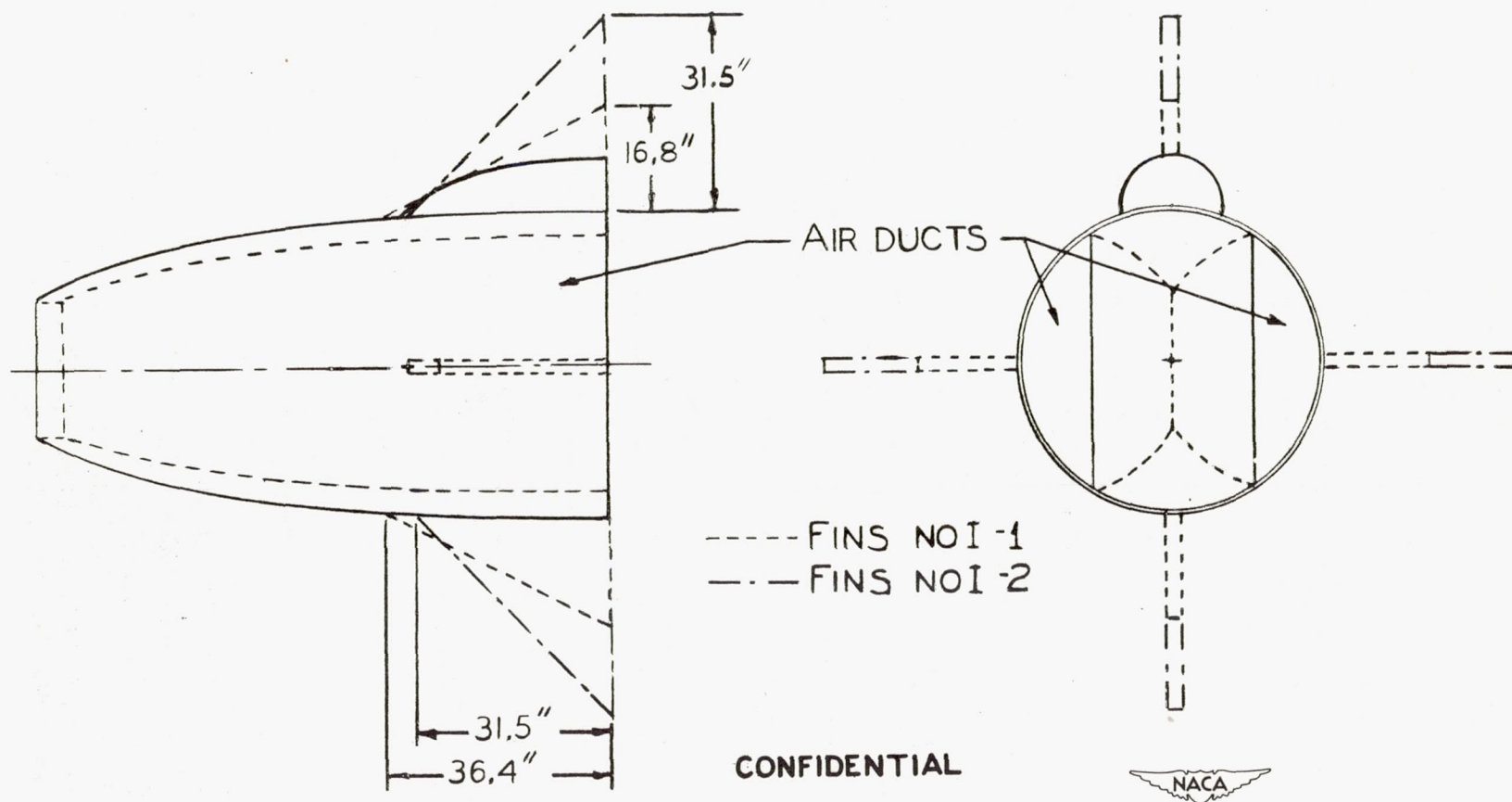
FIGURE 5.-SKETCH SHOWING FINS TESTED ON THE \frac{1}{4} -SCALE MODEL OF THE JETTISONABLE NOSE SECTION OF THE DOUGLAS D-558, PHASE I, AIRPLANE. DIMENSIONS ARE FULL-SCALE VALUES.
