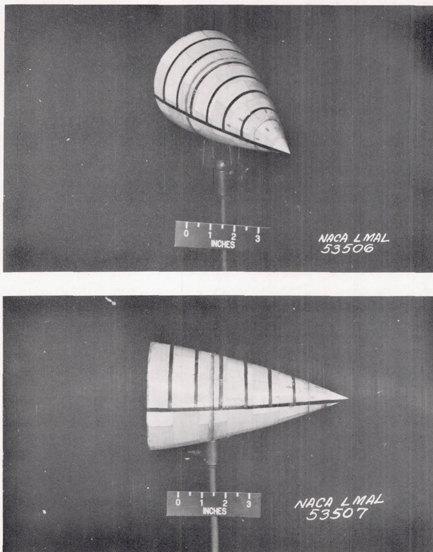
Figure 2.- Photographs of the \frac{1}{12} -scale model of the jettisonable nose section of the Douglas D-558, phase II, airplane tested in the free-spinning tunnel.
