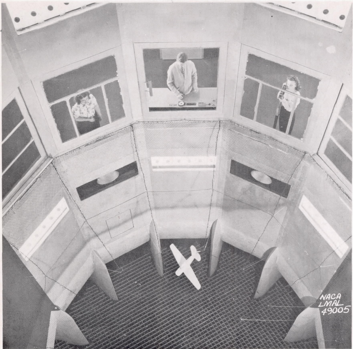
Figure 10.- Photograph showing the test section of the Langley 20-foot free-spinning tunnel. A typical spin-tunnel airplane model is shown spinning in the tunnel.
