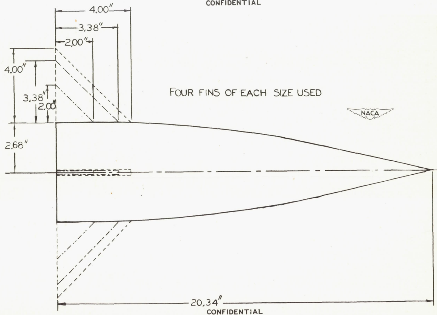
FIGURE 7. - SKETCH OF THE \frac{1}{2} -SCALE MODEL OF THE NOSE SECTION OF THE RM-11 TEST VEHICLE TESTED IN THE FREE-SPINNING TUNNEL. VARIOUS FINS TESTED ON THE MODEL ARE SHOWN. DIMENSIONS SHOWN ARE MODEL VALUES.
