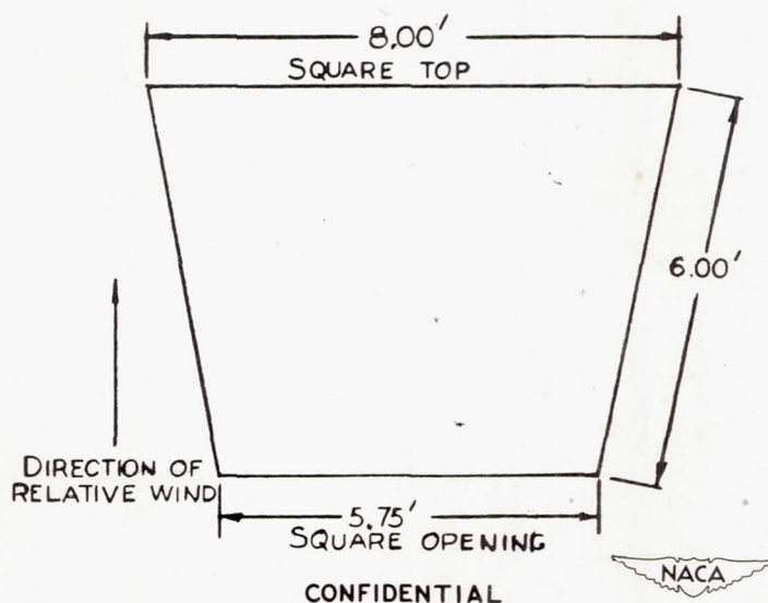
FIGURE 9.-SKETCH OF BOX-TYPE PARACHUTE B, USED AS STABILIZING PARACHUTE FOR THE \frac{1}{12} -SCALE MODEL OF THE D-558, PHASE II, AIRPLANE NOSE SECTION IN THE FREE-SPINNING TUNNEL. PARACHUTE IS SHOWN FULLY OPENED. EIGHT SHROUD LINES AVERAGING 10.3 FEET IN LENGTH WERE ATTACHED TO THE BOTTOM OF THE PARACHUTE AT THE CORNERS AND MIDWAY OF EACH SIDE. DIMENSIONS ARE FULL-SCALE.
