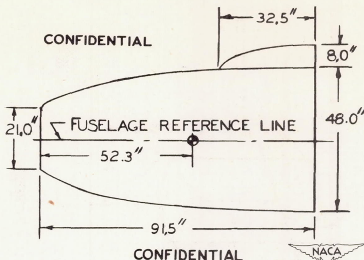
FIGURE 3.-SKETCH OF THE \frac{1}{14} -SCALE MODEL OF THE JETTISONABLE NOSE SECTION OF THE DOUGLAS D-558, PHASE I, AIRPLANE TESTED IN THE FREE-SPINNING TUNNEL. CENTER OF GRAVITY IS SHOWN FOR THE ORIGINAL LOADING CONDITION. DIMENSIONS ARE FULL-SCALE VALUES. MODEL AIR DUCTS ARE NOT SHOWN.
