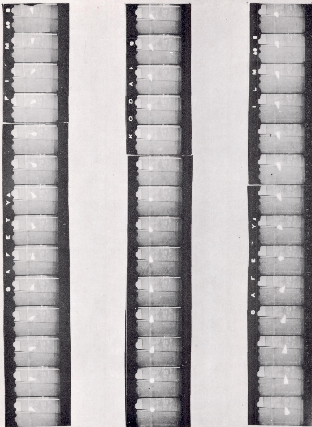
Figure 11.- Moving picture strip of tests of the \frac{1}{12} -scale model of the jettisonable nose section of the D-558, phase II, airplane in its original loading with no fins installed. The model is shown tumbling in the Langley 20-foot free-spinning tunnel.
