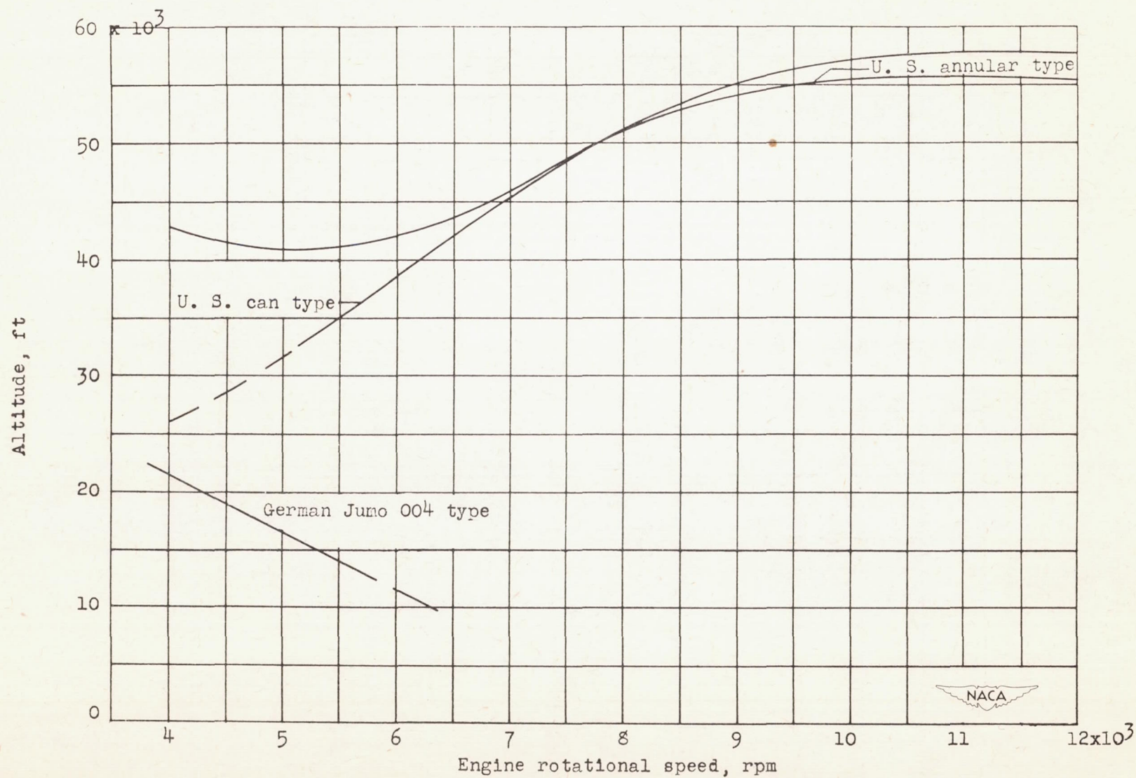
Figure 10. - Comparison of altitude operational limits of combustors with air flows based on included areas.
