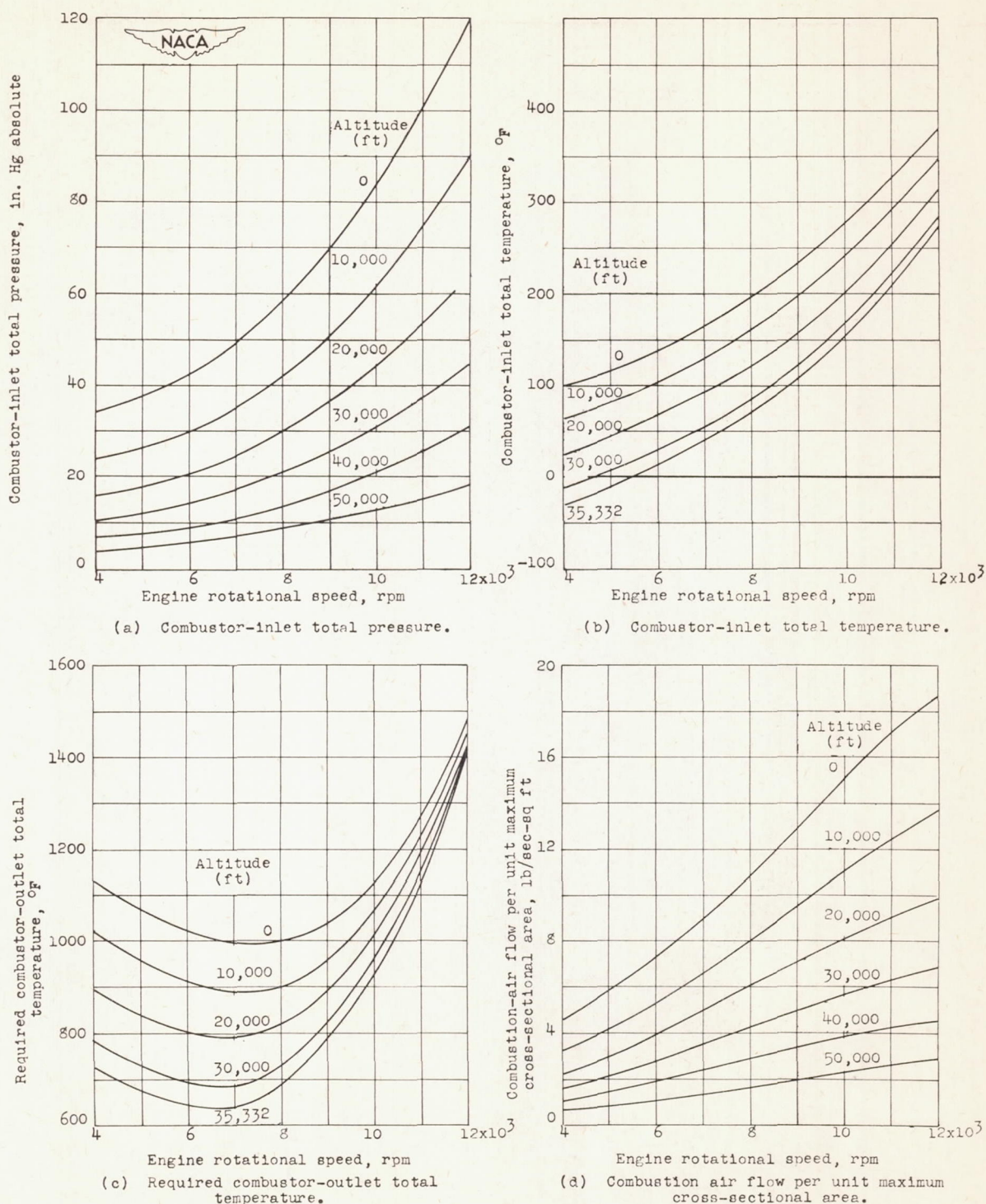
Figure 6. - Variation of combustor operating conditions with engine speed for various altitudes based on performance of reference turbo-jet engine. Flight speed, 0 mile per hour; compressor-pressure ratio, 4.
