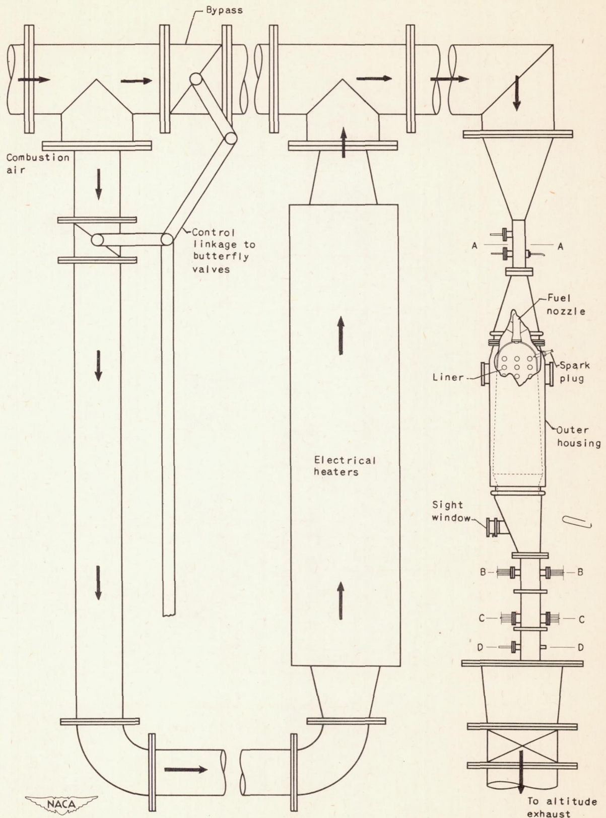
Figure 2. - Schematic sketch of U. S. can-type combustor installed in test rig.
