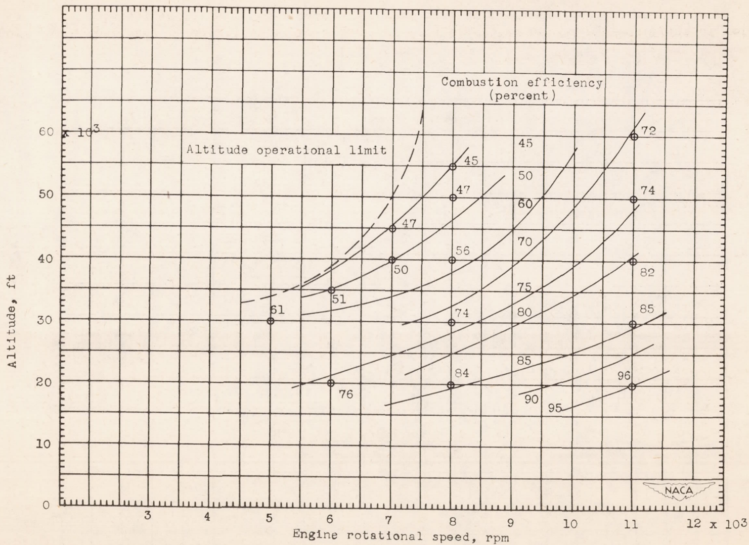
Figure 11. - Combustion efficiency at various simulated operating conditions of reference engine for air flows based on actual maximum cross-sectional area.
