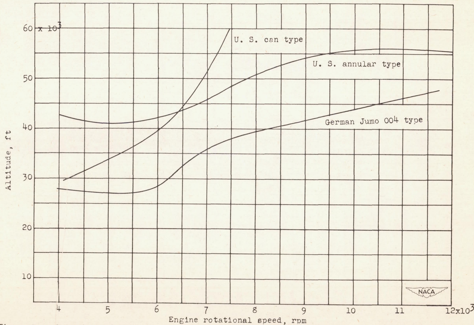
Figure 8. - Comparison of altitude operational limits of combustors with air flow based on actual maximum cross-sectional areas.
