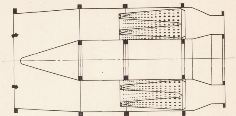
Annular type
