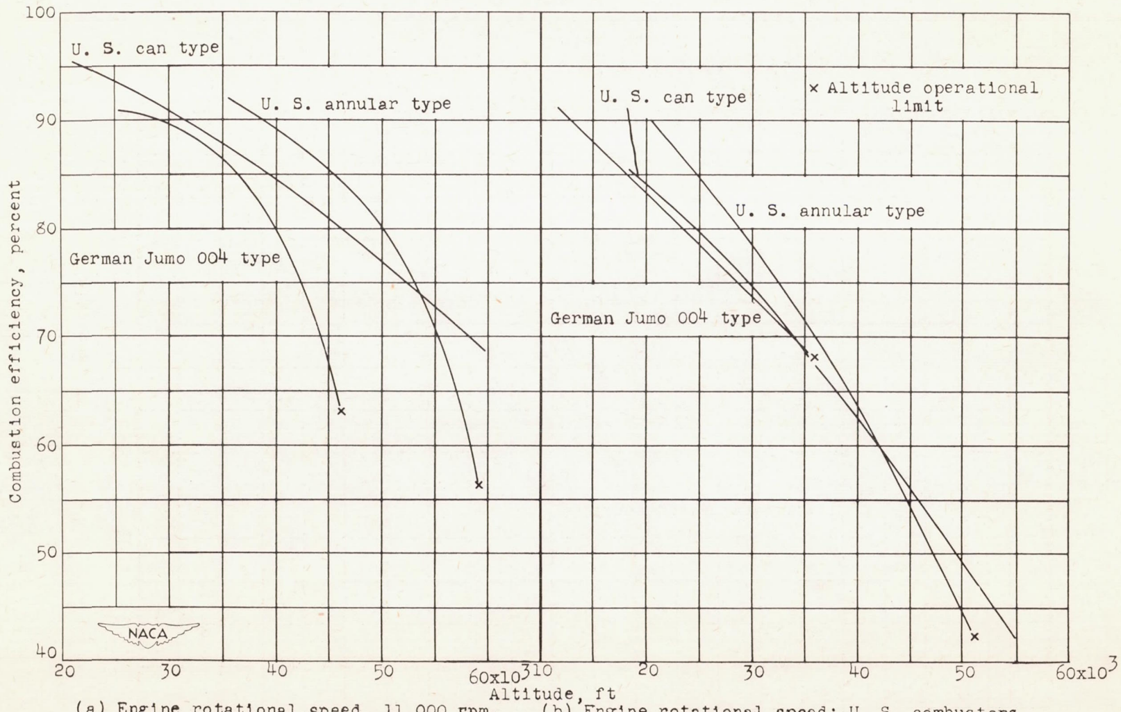
Figure 12. - Variation of combustion efficiency with altitude for air flows based on actual maximum cross-sectional areas.
