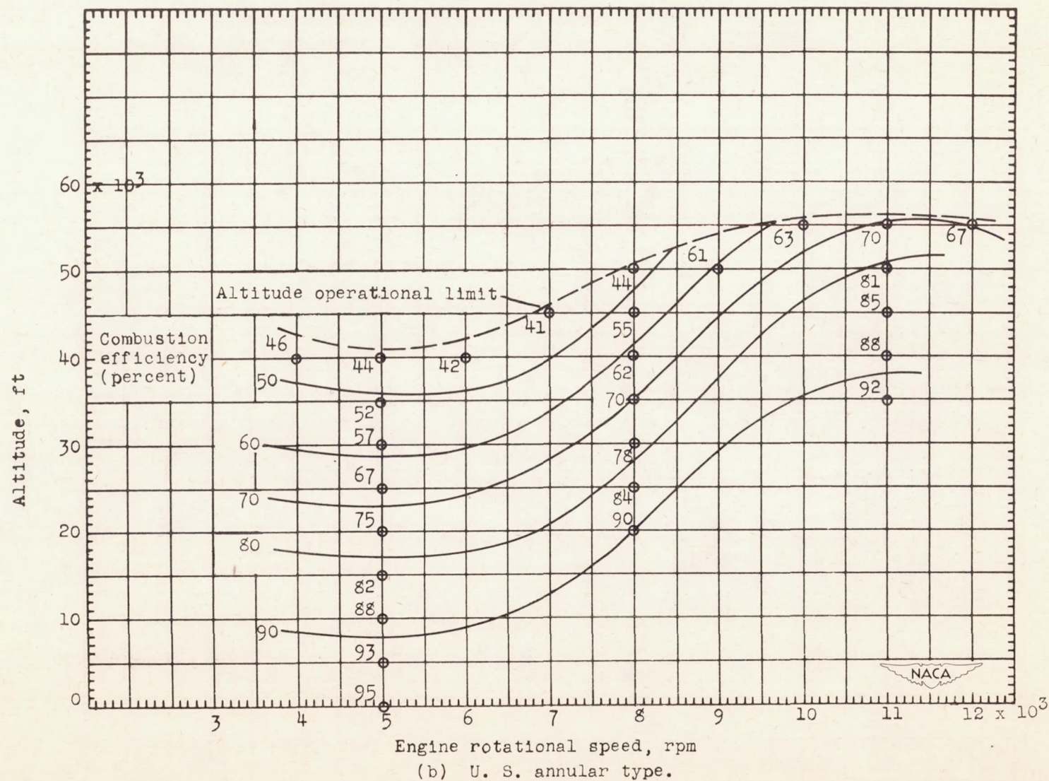
Figure 11. - Continued. Combustion efficiency at various simulated operating conditions of reference engine for air flows based on actual maximum cross-sectional area.
