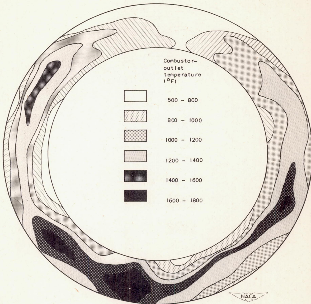
Figure 17. - Concluded. Temperature profile of U. S. annular-type combustor at combustor outlet for air flows based on actual maximum cross-sectional area. Engine speed, 11,000 rpm.
