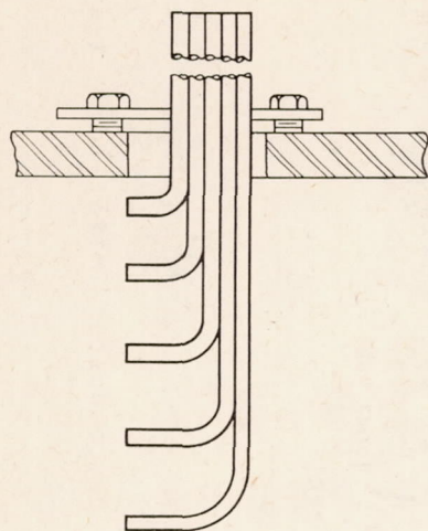
Total-pressure rake
