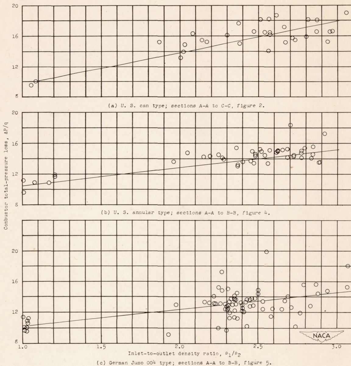
Figure 15. - Correlation of combustor inlet-to-outlet total-pressure-loss data.
