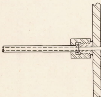
Static-pressure orifice
