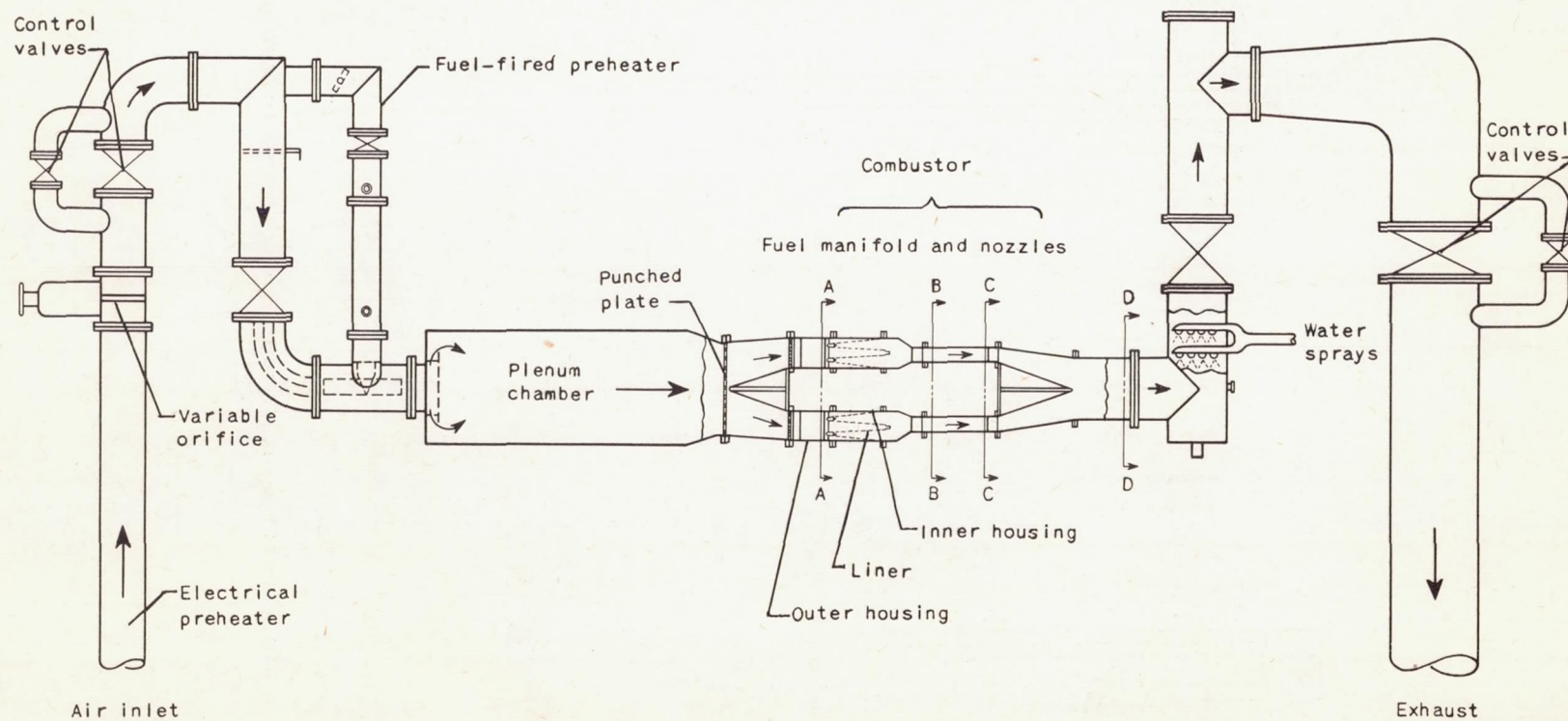
Figure 4. - Schematic sketch of U. S. annular-type combustor installed in test rig.
