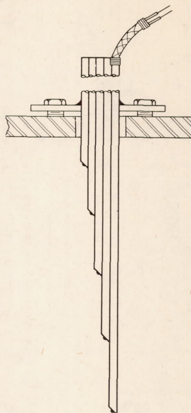
Thermocouple rake
