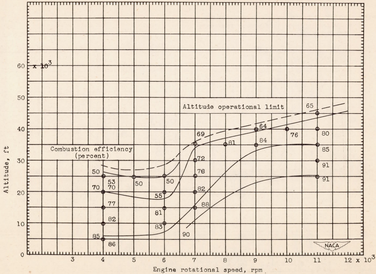
Figure 11. - Concluded. Combustion efficiency at various simulated operating conditions of reference engine for air flows based on actual maximum cross-sectional area.
