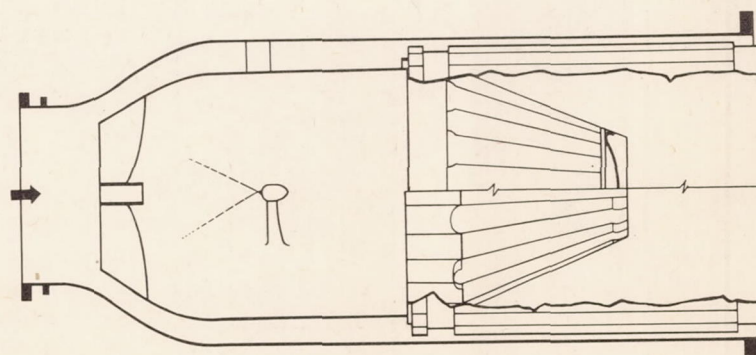
German can type (Jumo 004)
