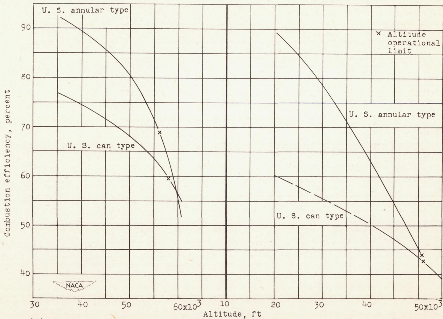
Figure 14. - Variation of combustion efficiency with altitude for air flows based on included annular areas.
