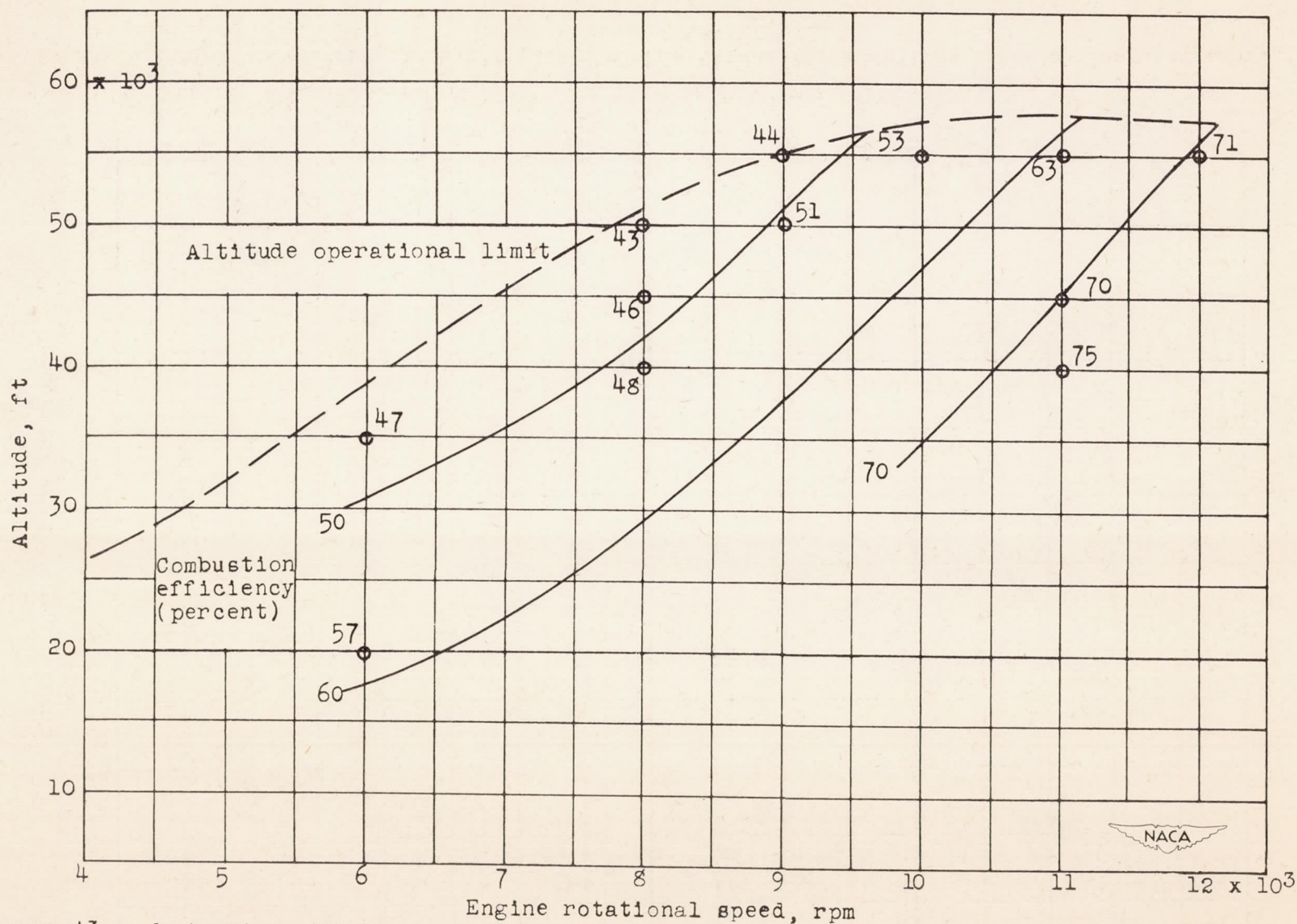
Figure 13. - Combustion efficiency at various simulated operating conditions of reference engine for U. S. can-type combustor; air flows based on included annular area.
