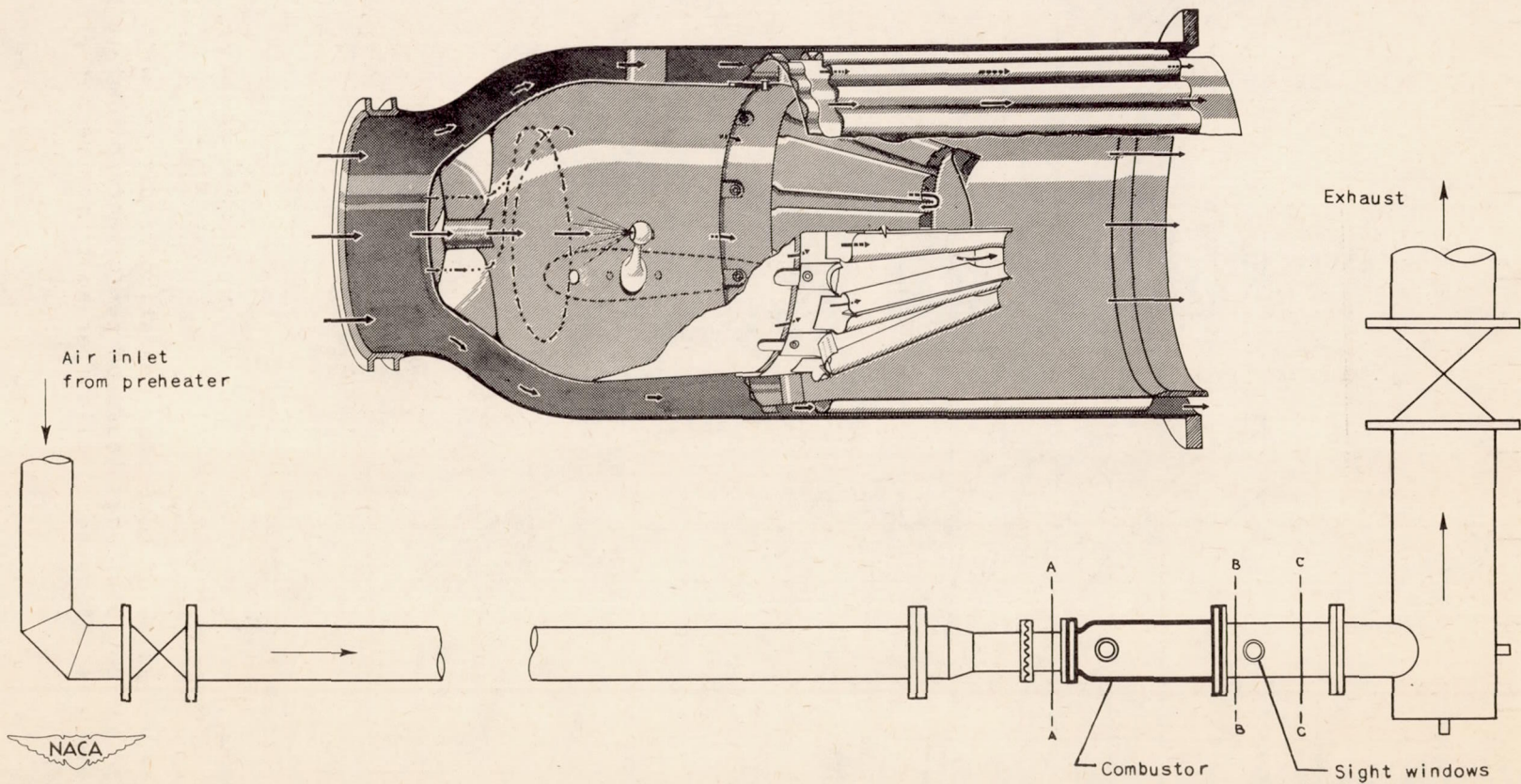
Figure 5. - Schematic sketch of German Jumo 004 can-type combustor and test-rig installation.
