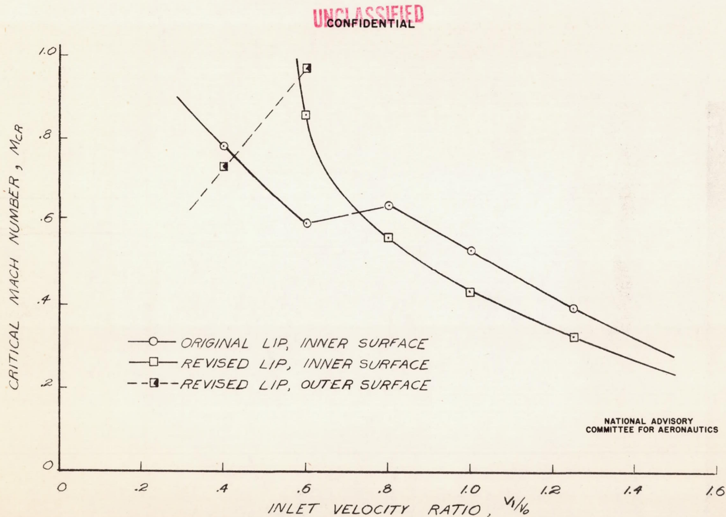
FIGURE 10.— VARIATION OF CRITICAL MACH NUMBER WITH INLET-VELOCITY RATIO FOR ORIGINAL INSTALLATION AND WITH REVISED LIP AND DEFLECTORS, \alpha = 0^\circ , MODIFIED FIGHTER AIRPLANE.
