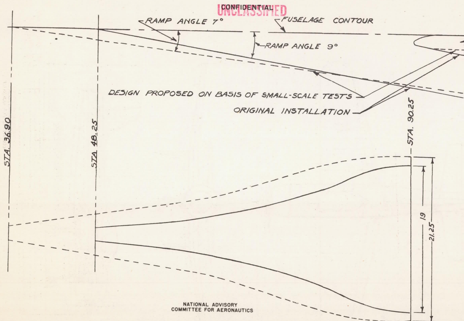
FIGURE 1.- COMPARISON OF ORIGINAL AND PROPOSED INSTALLATION OF SUBMERGED DUCT ENTRANCE ON MODIFIED FIGHTER AIRPLANE.
