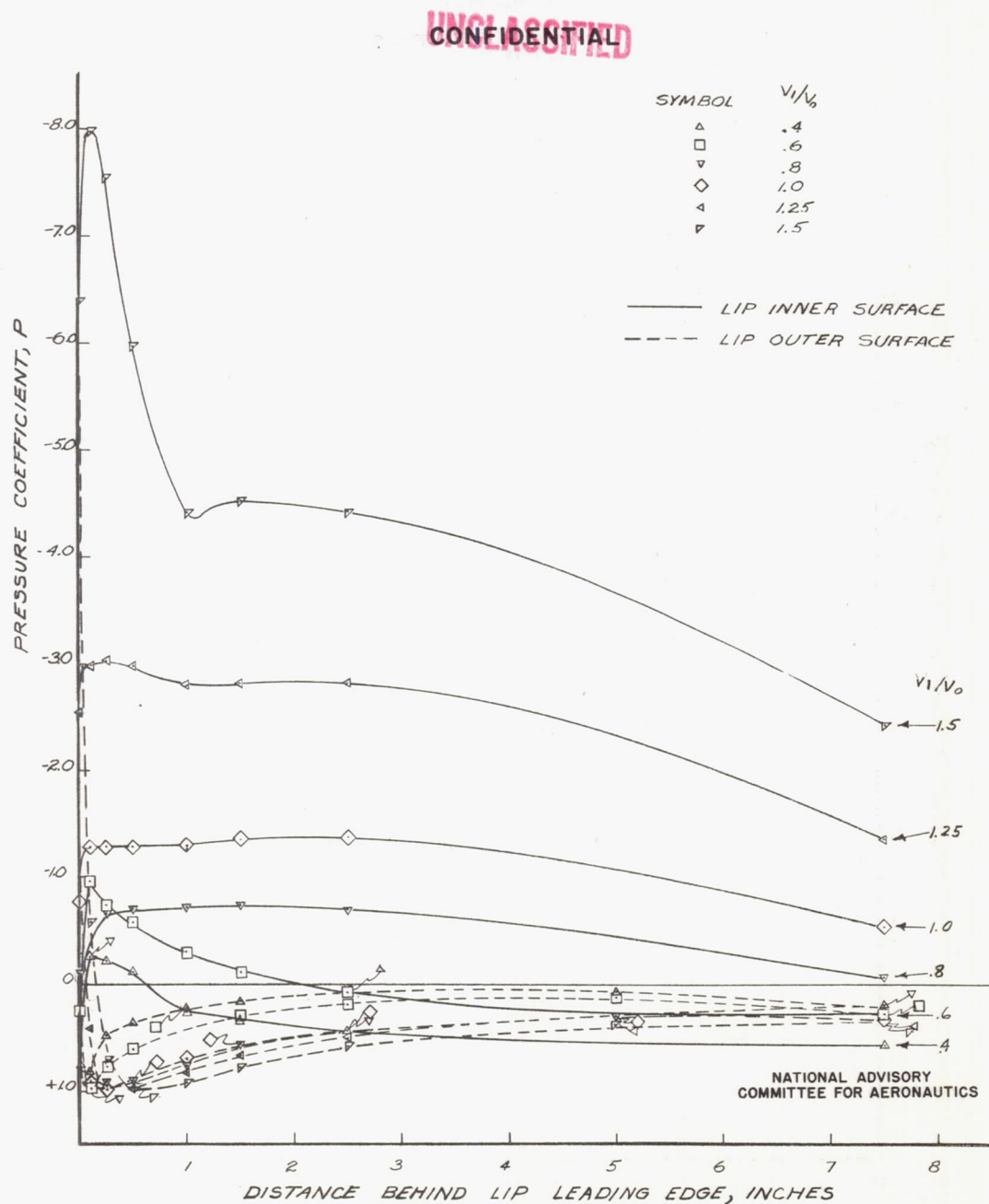
(a) ORIGINAL LIP
