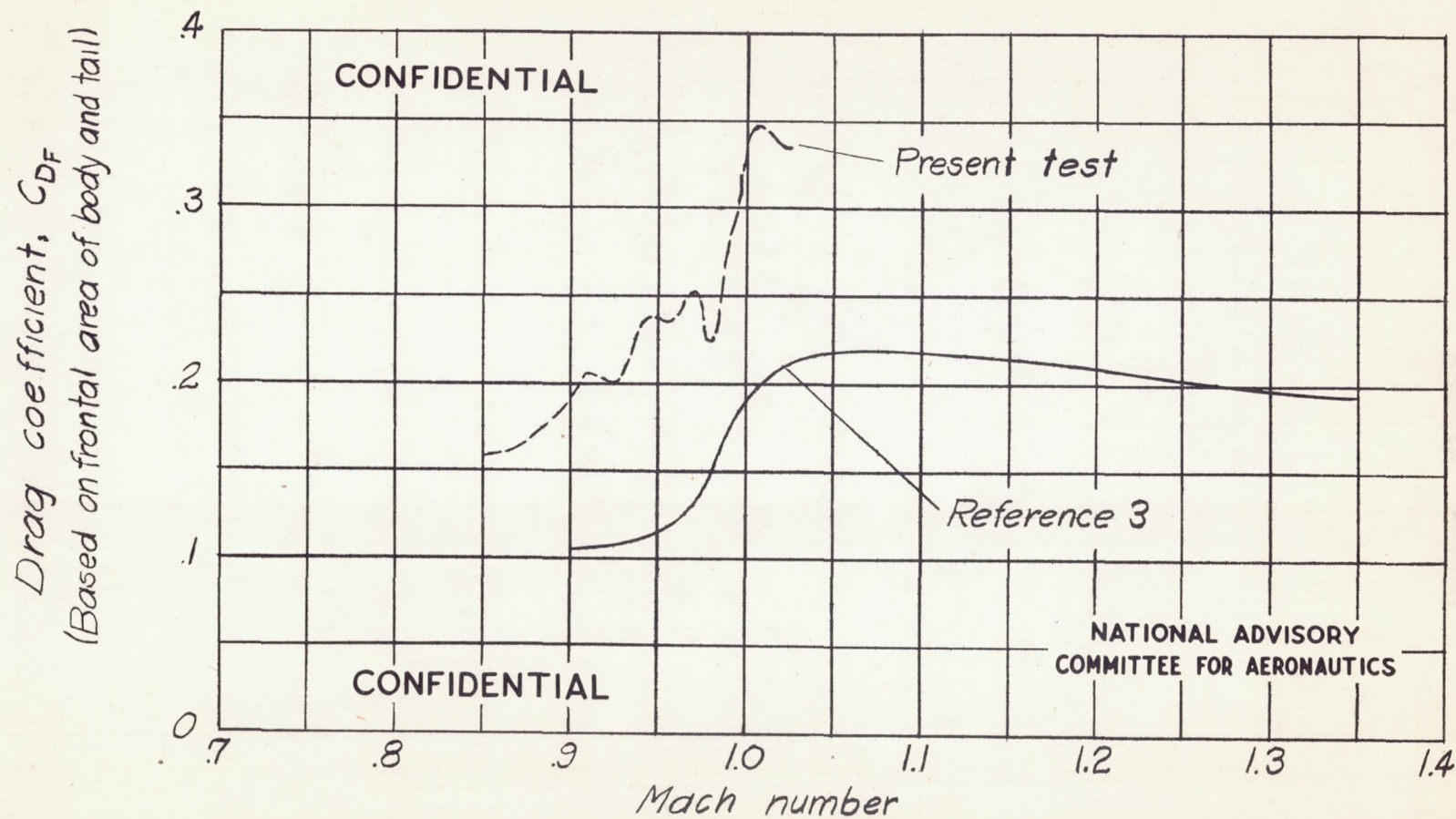
Figure 7.- Comparison of drag results for the body-tail combination with those of previous tests.
