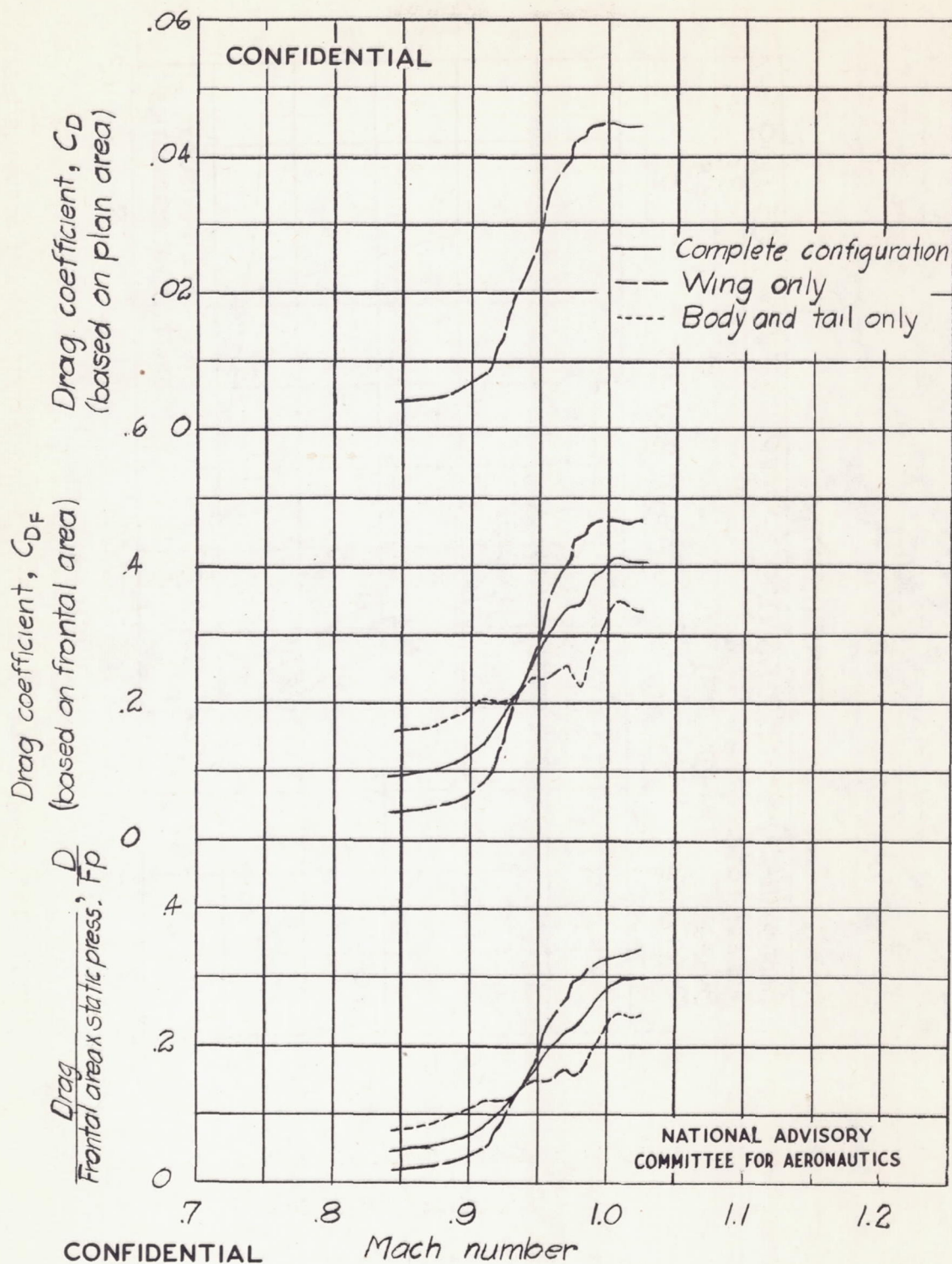
Figure 5.- Variation with Mach number of drag coefficients and D/F_p ratios for the complete configuration and its component parts. For each curve the drag parameter is based on the area of the specified component.
