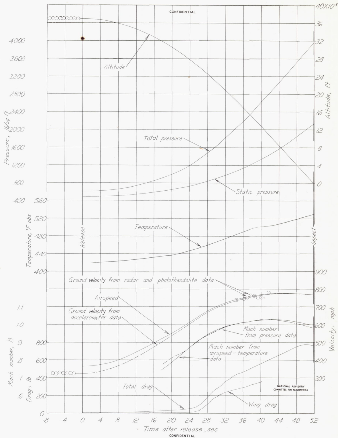
Figure 4.- Time history of free fall of test configuration.
