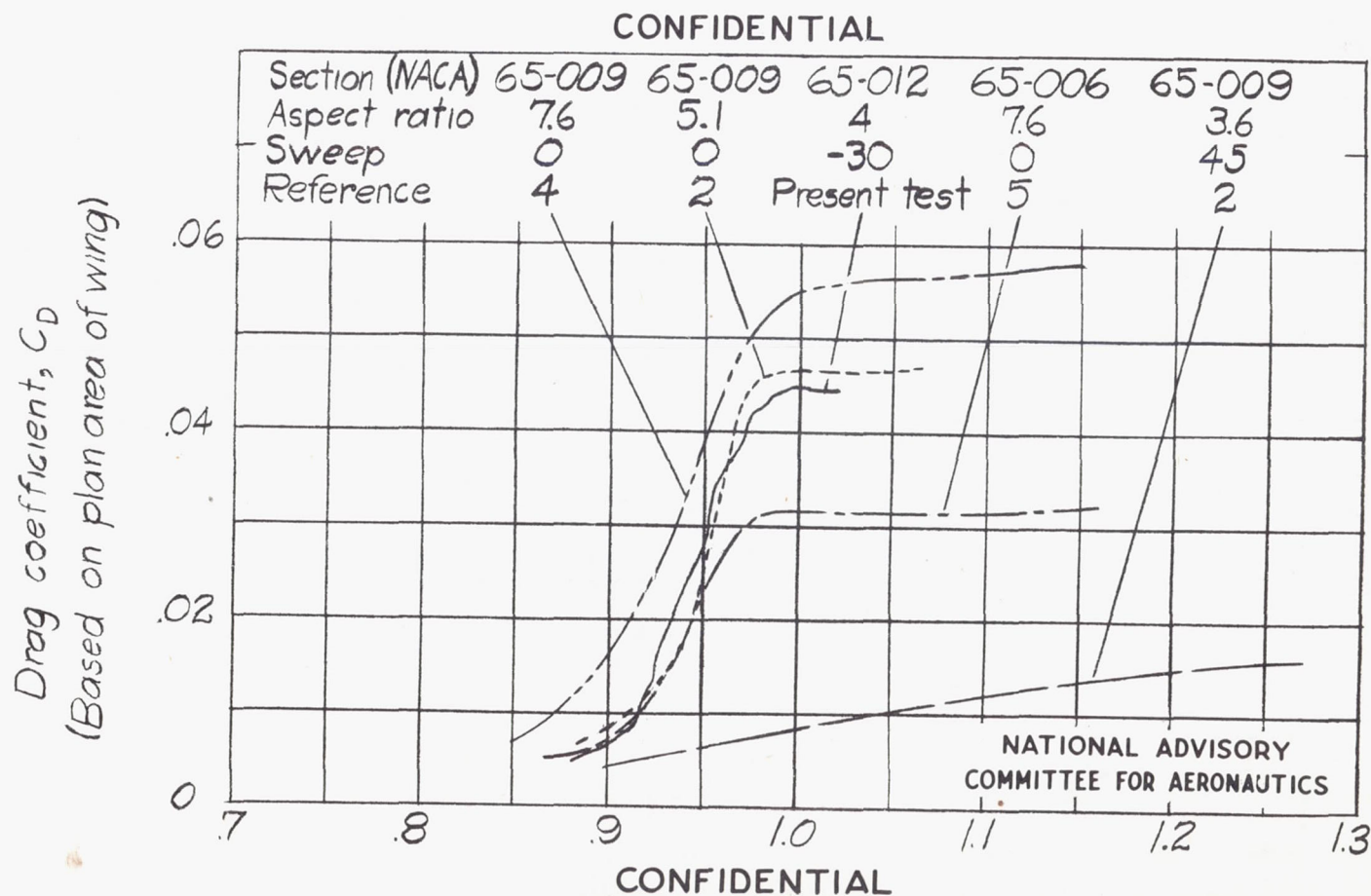
Figure 6.- Comparison of wing drag results with those of previous tests.
