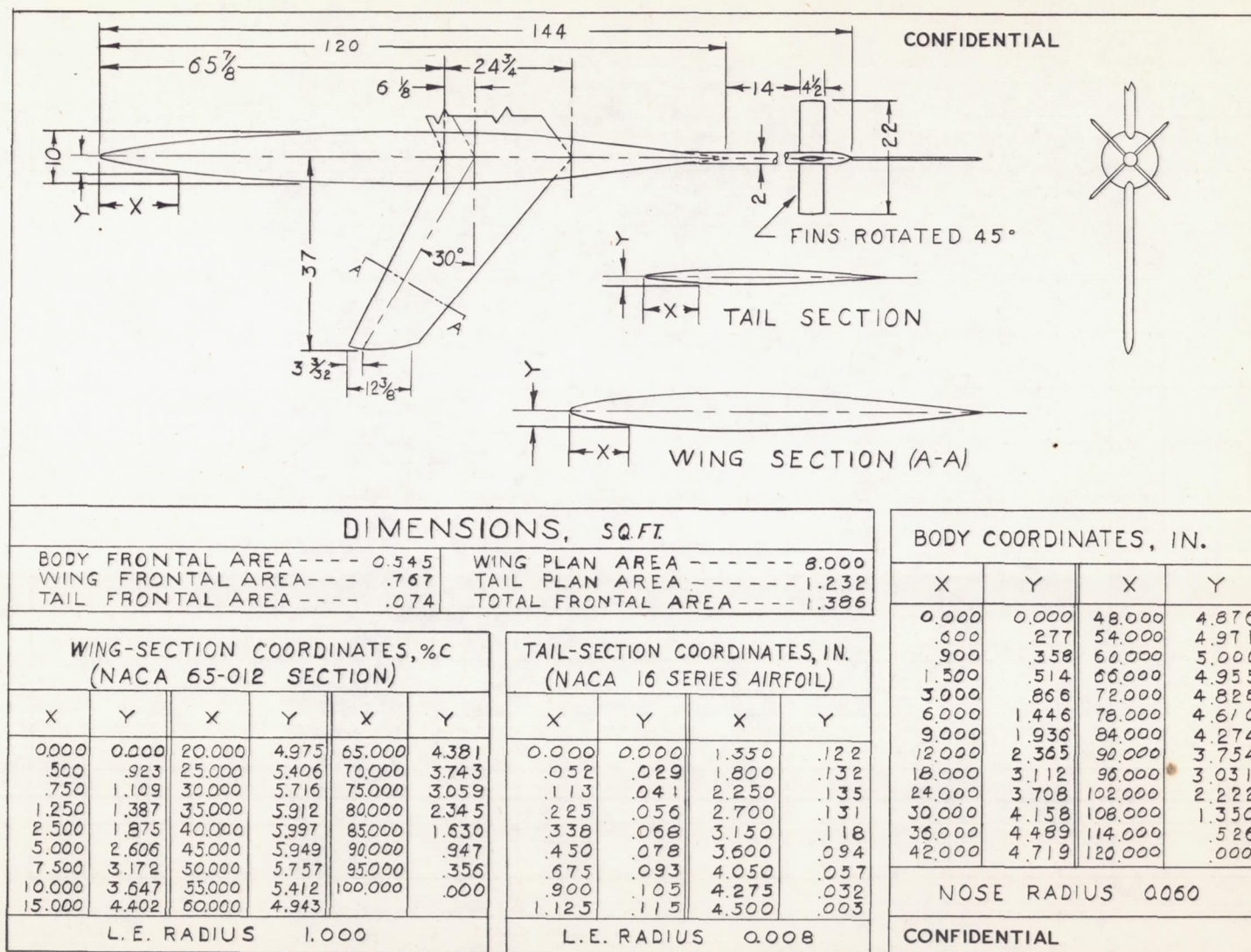
Figure 3.- General arrangement and dimensions of test configuration. All dimensions are in inches.
