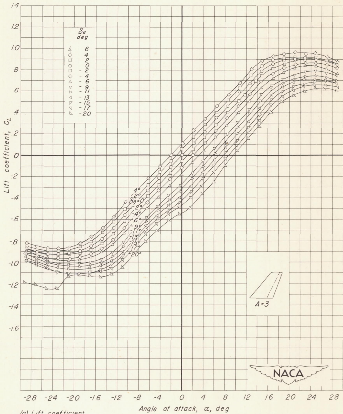
(a) Lift coefficient. Figure 10.- Lift, hinge-moment, and pitching-moment coefficients of the 35° swept-back tail. Aspect ratio 3; R, 3.0 \times 10^6 .
