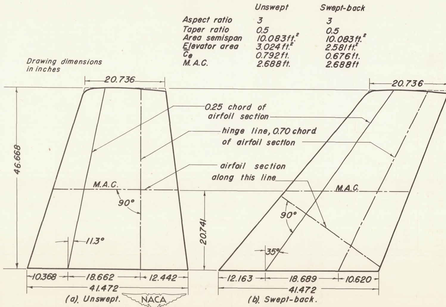
Figure 1.- Plan forms of the horizontal tail models of aspect ratio 3.
