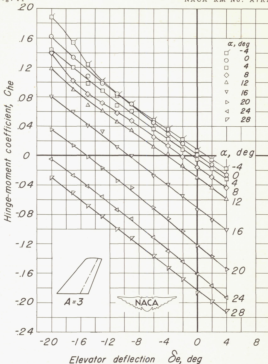
Figure 11.- Variation of hinge-moment coefficients with elevator deflection for various angles of attack of the 35^\circ swept-back tail. Aspect ratio 3; R, 3.0 \times 10^6 .
