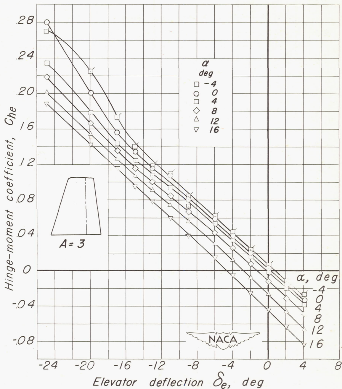
Figure 5.- Variation of hinge-moment coefficient with elevator deflection for various angles of attack of the unswept tail. Aspect ratio, 3; R, 3.0 \times 10^6 .
