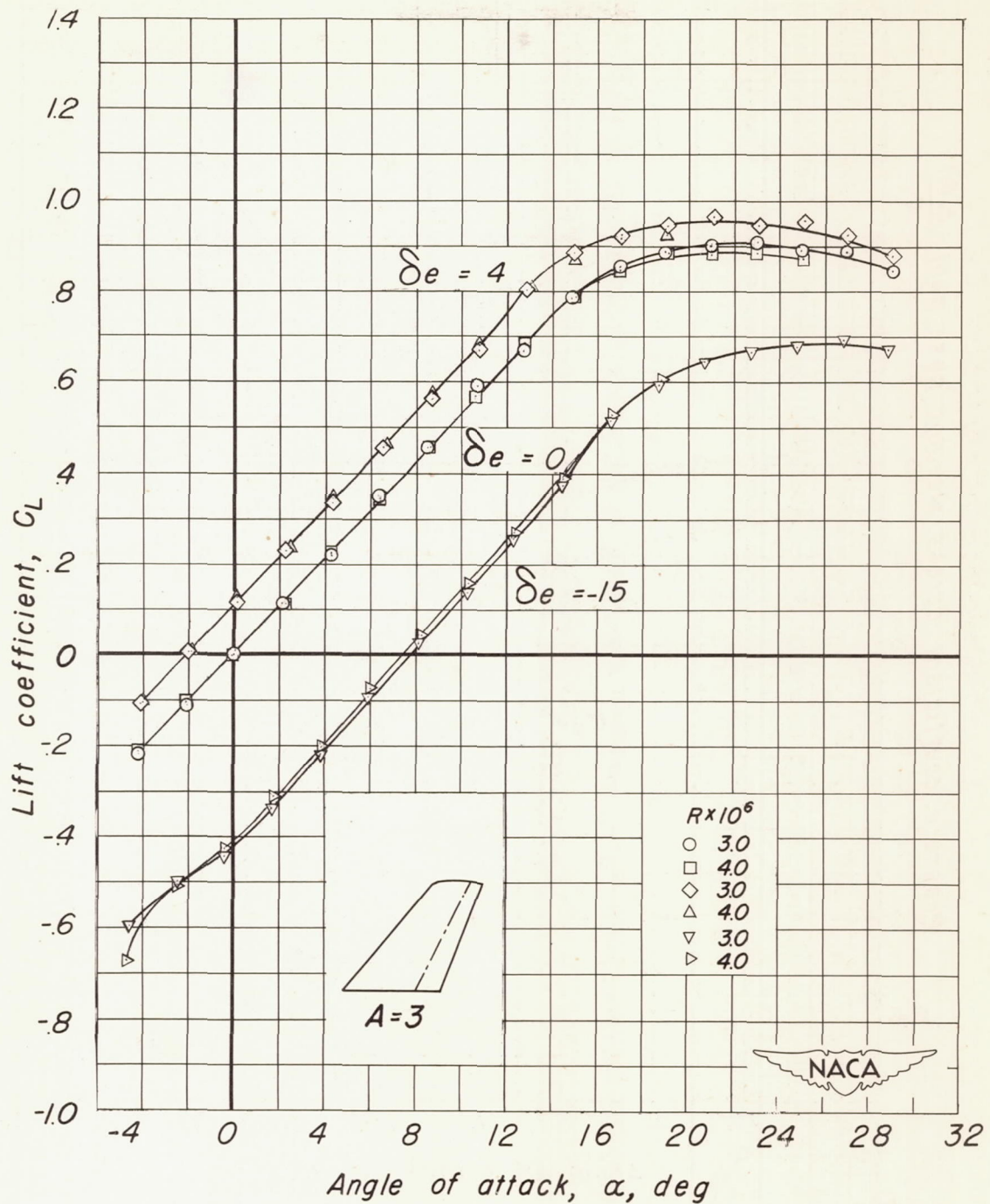
Figure 13.- Comparison of the lift and hinge-moment coefficients at R=3.0 \times 10^6 and 4.0 \times 10^6 for the 35^\circ swept-back tail. Aspect ratio 3.
