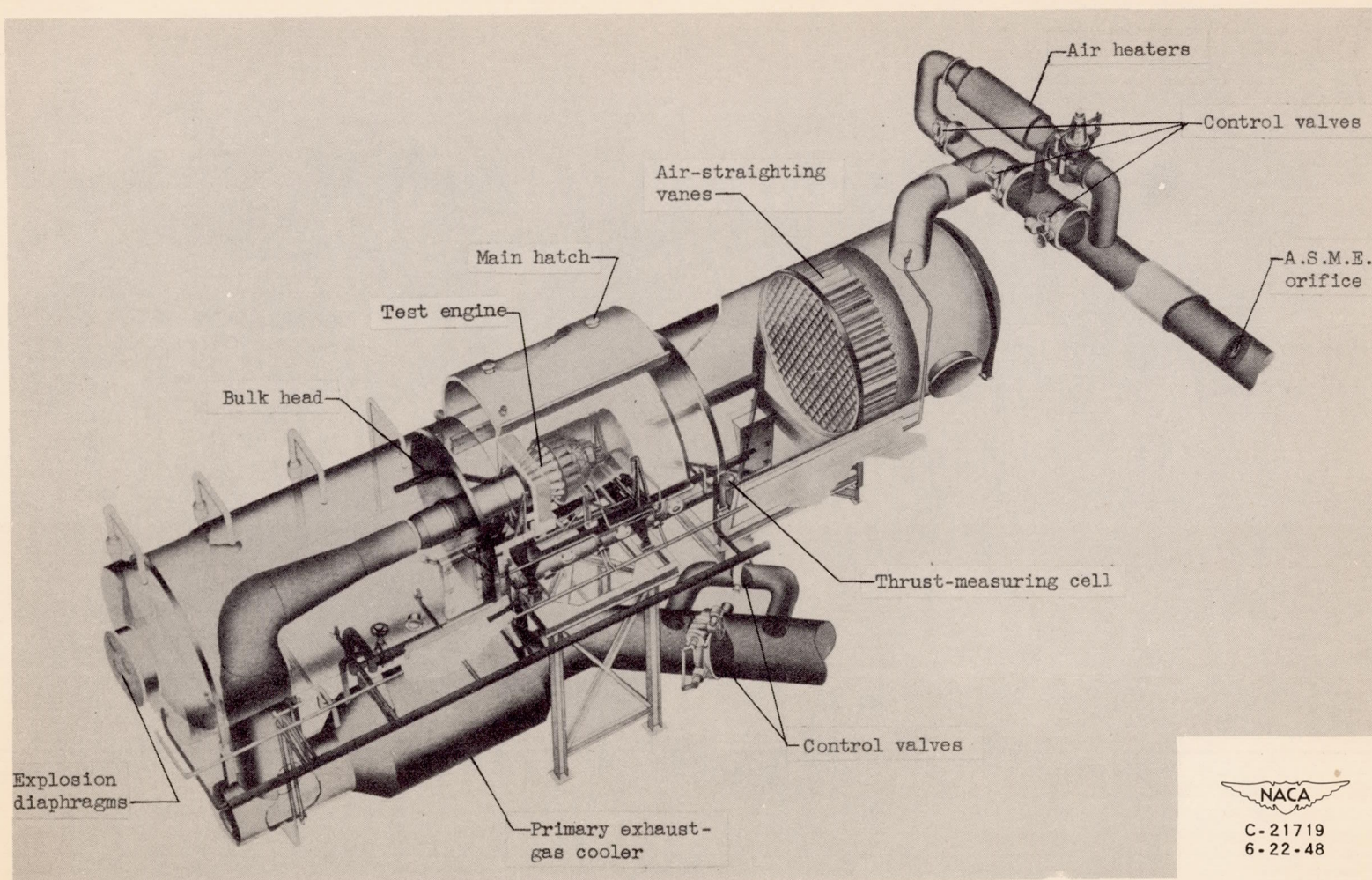
Figure 1. - Altitude chamber showing engine installation.
