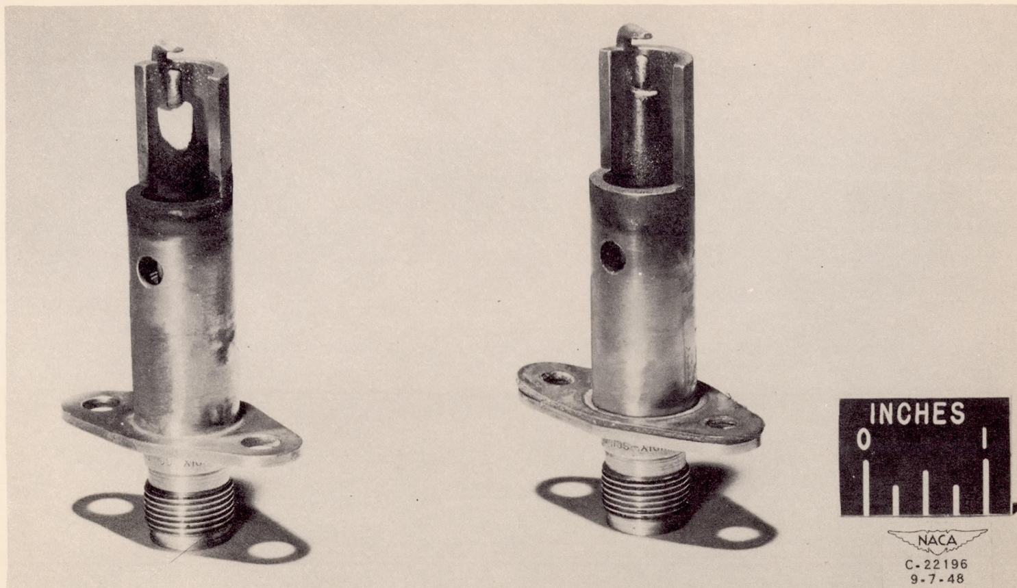
(b) Operating time, 11 hours; fuel, AN-F-32.
