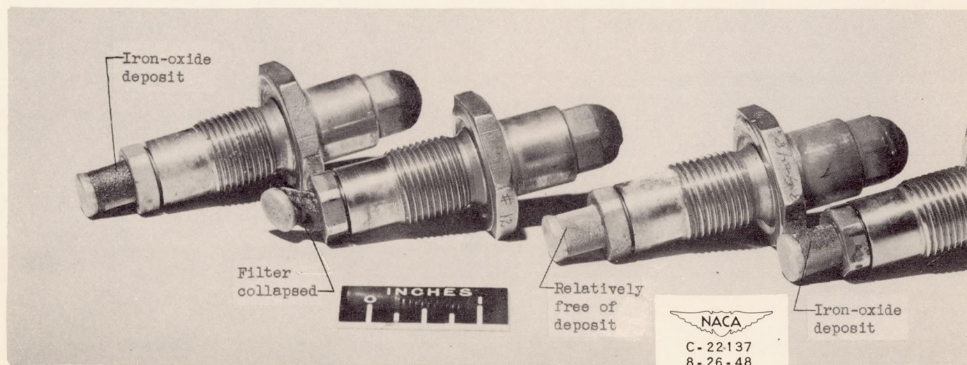
Figure 13. - Fuel injectors showing iron oxide deposits on injector-inlet filters.
