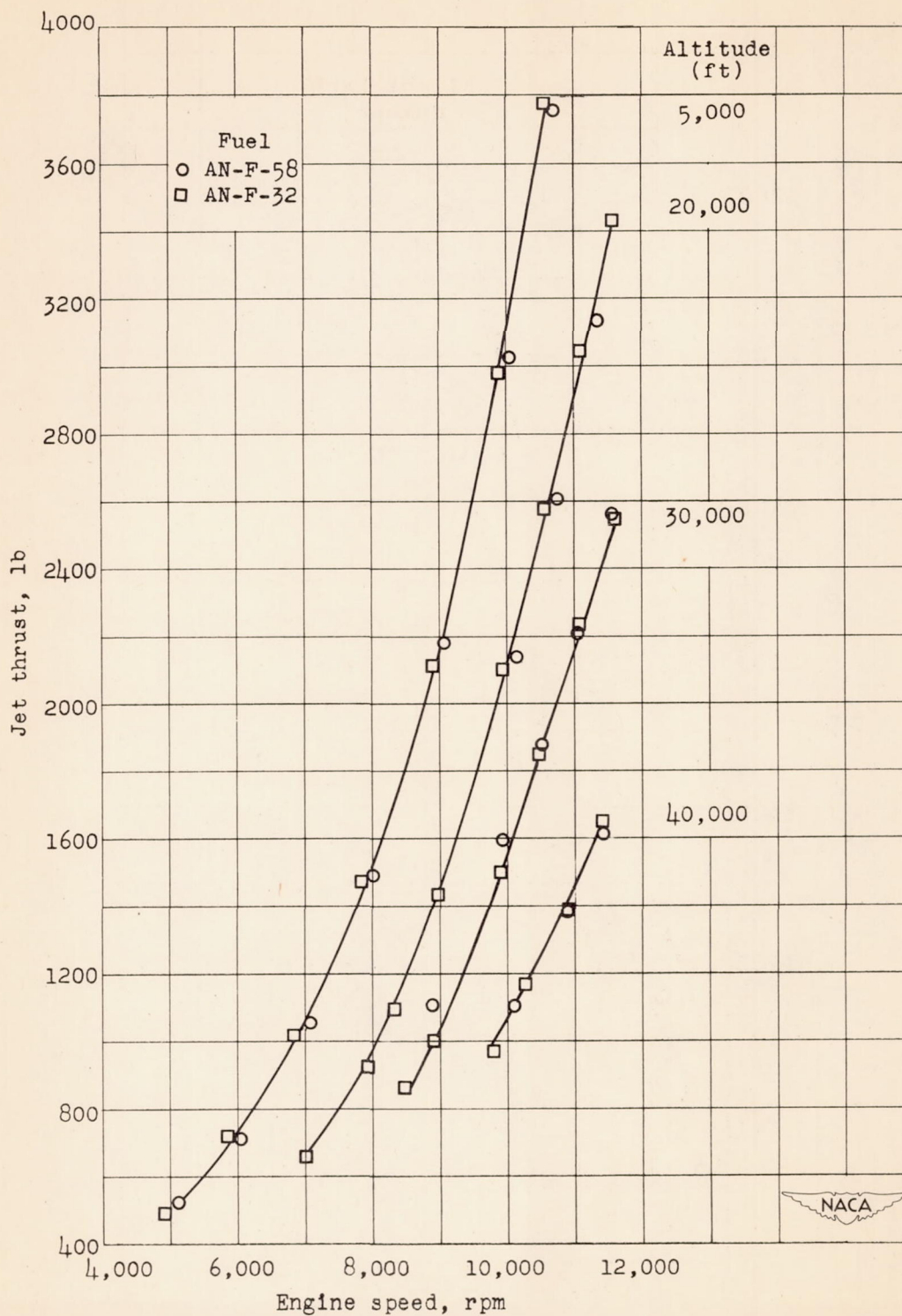
Figure 2. - Jet thrust using AN-F-58 and AN-F-32 fuels at various altitudes. Flight Mach number, 0.60.
