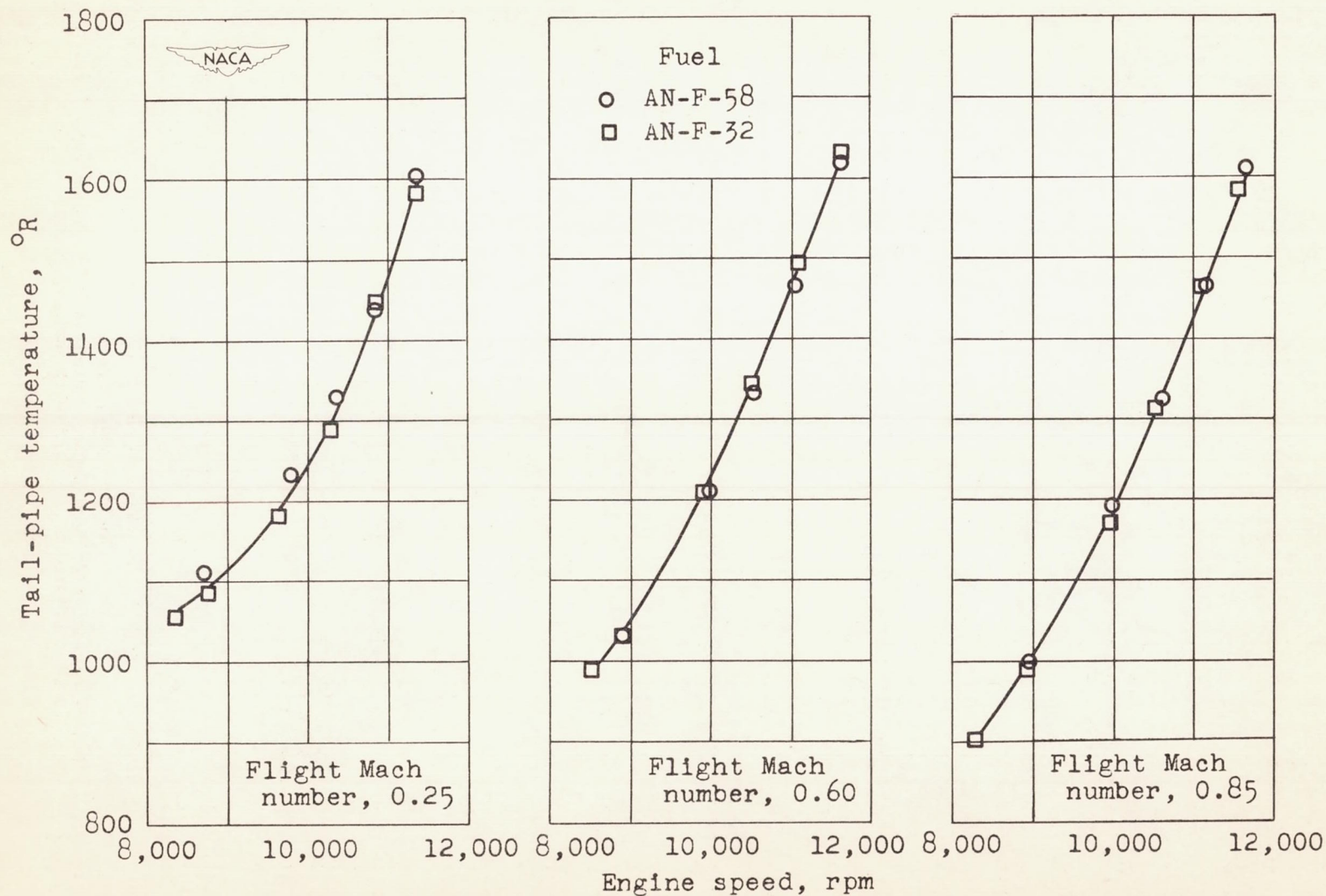
Figure 7. - Indicated tail-pipe temperature of AN-F-58 and AN-F-32 fuels at various flight Mach numbers. Altitude, 30,000 feet.
