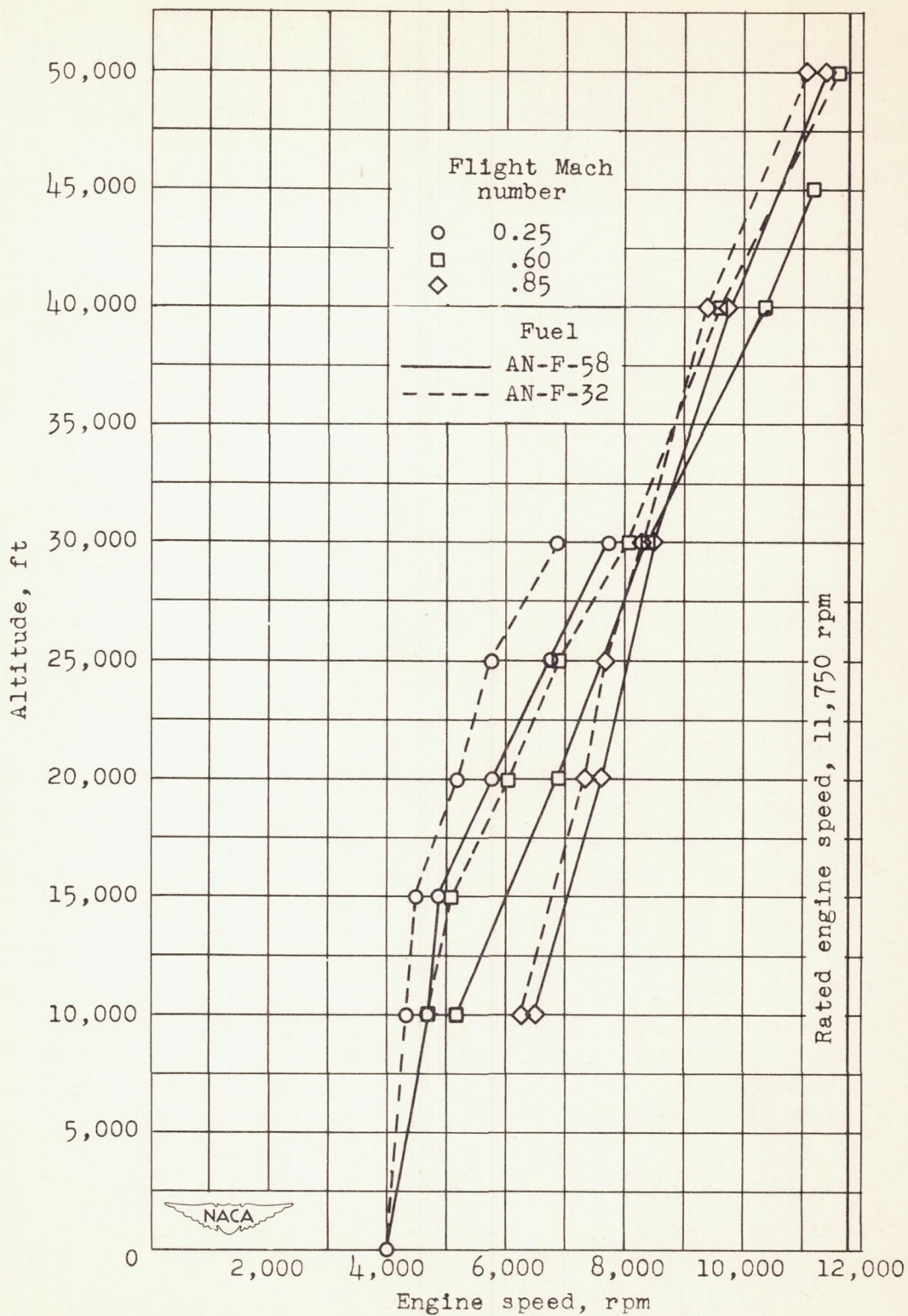
Figure 9. - Idling limits of fuel-metering control using AN-F-58 and AN-F-32 fuels.
