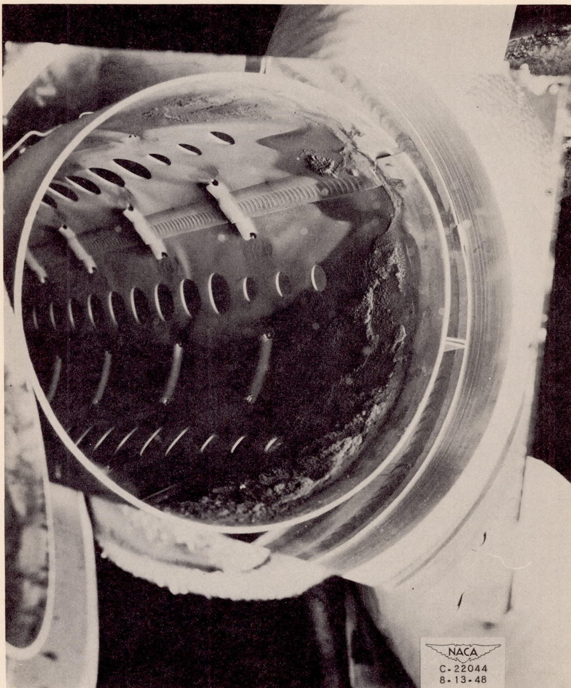
Figure 12. - Typical carbon deposits in burner liner from J33-A-23 turbojet engine operating time, 45\frac{1}{4} hours.
