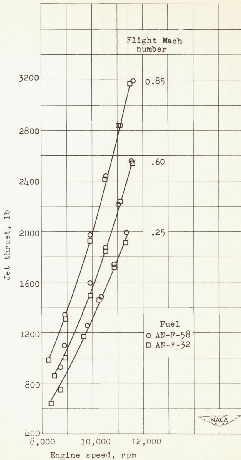
Figure 3. - Jet thrust using AN-F-58 and AN-F-32 fuels at various flight Mach numbers. Altitude, 30,000 feet.
