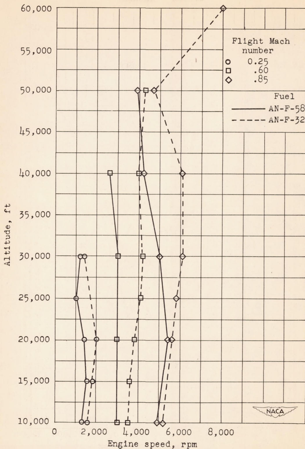
Figure 8. - Low-speed blow-out limits of AN-F-58 and AN-F-32 fuels.
