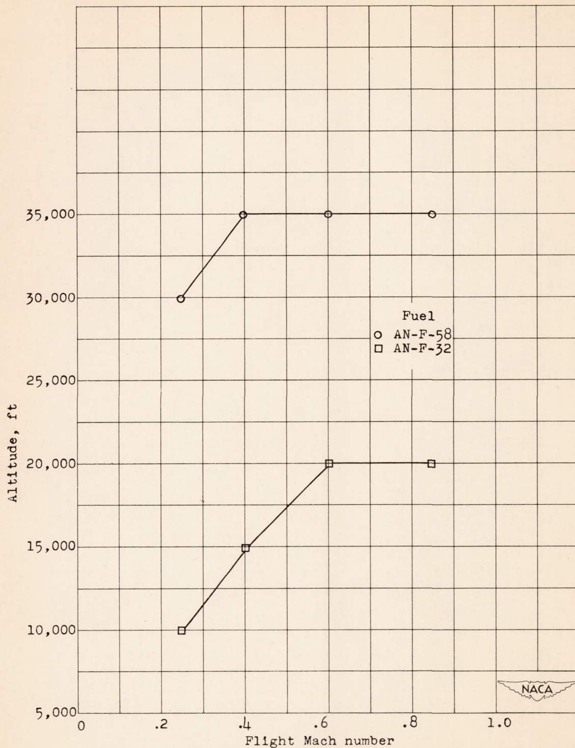
Figure 10. - Maximum altitudes at which windmilling starts were possible (using manual controls) with AN-F-58 and AN-F-32 fuels.
