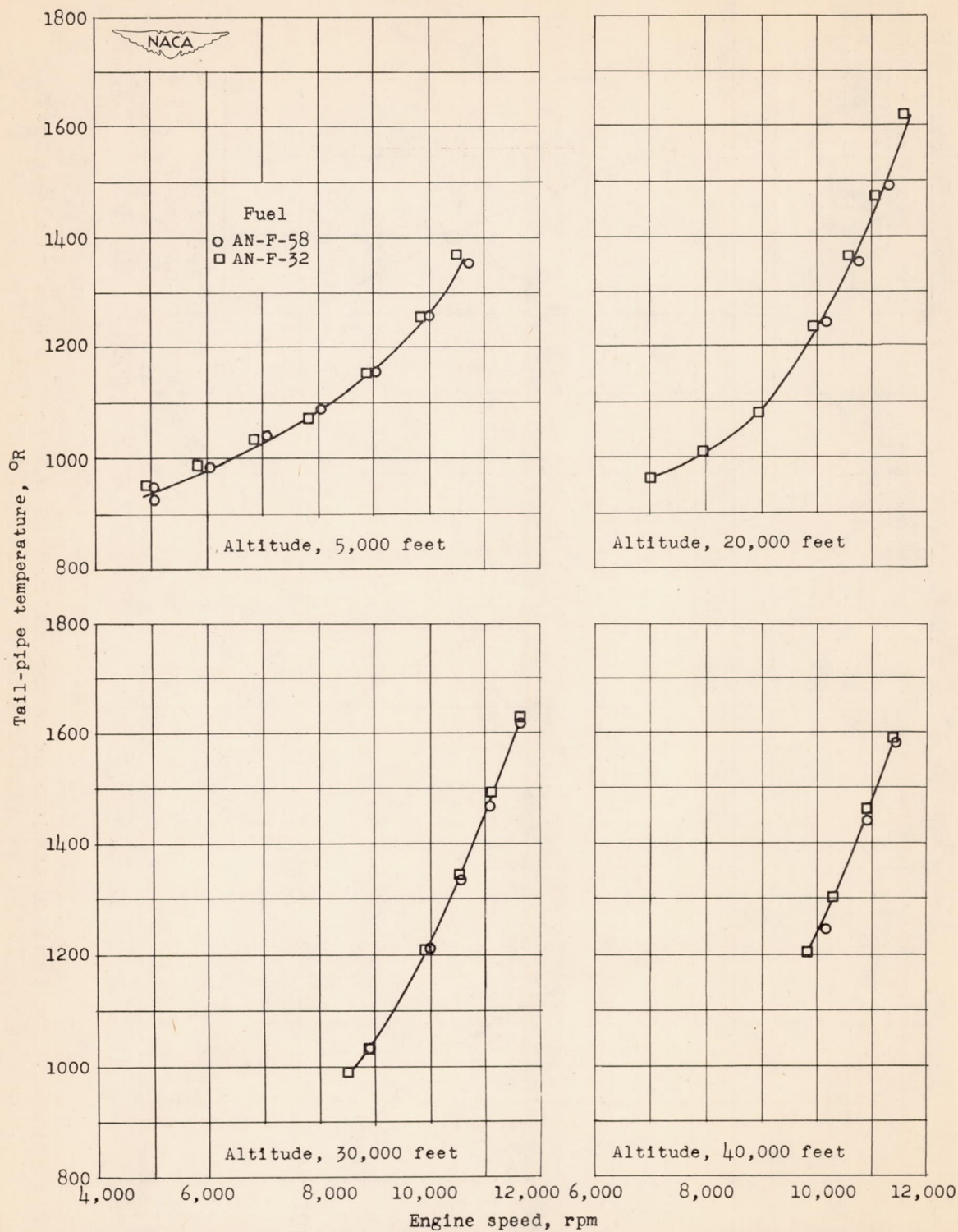
Figure 6. - Indicated tail-pipe temperature using AN-F-58 and AN-F-32 fuels at various altitudes. Flight Mach number, 0.60.
