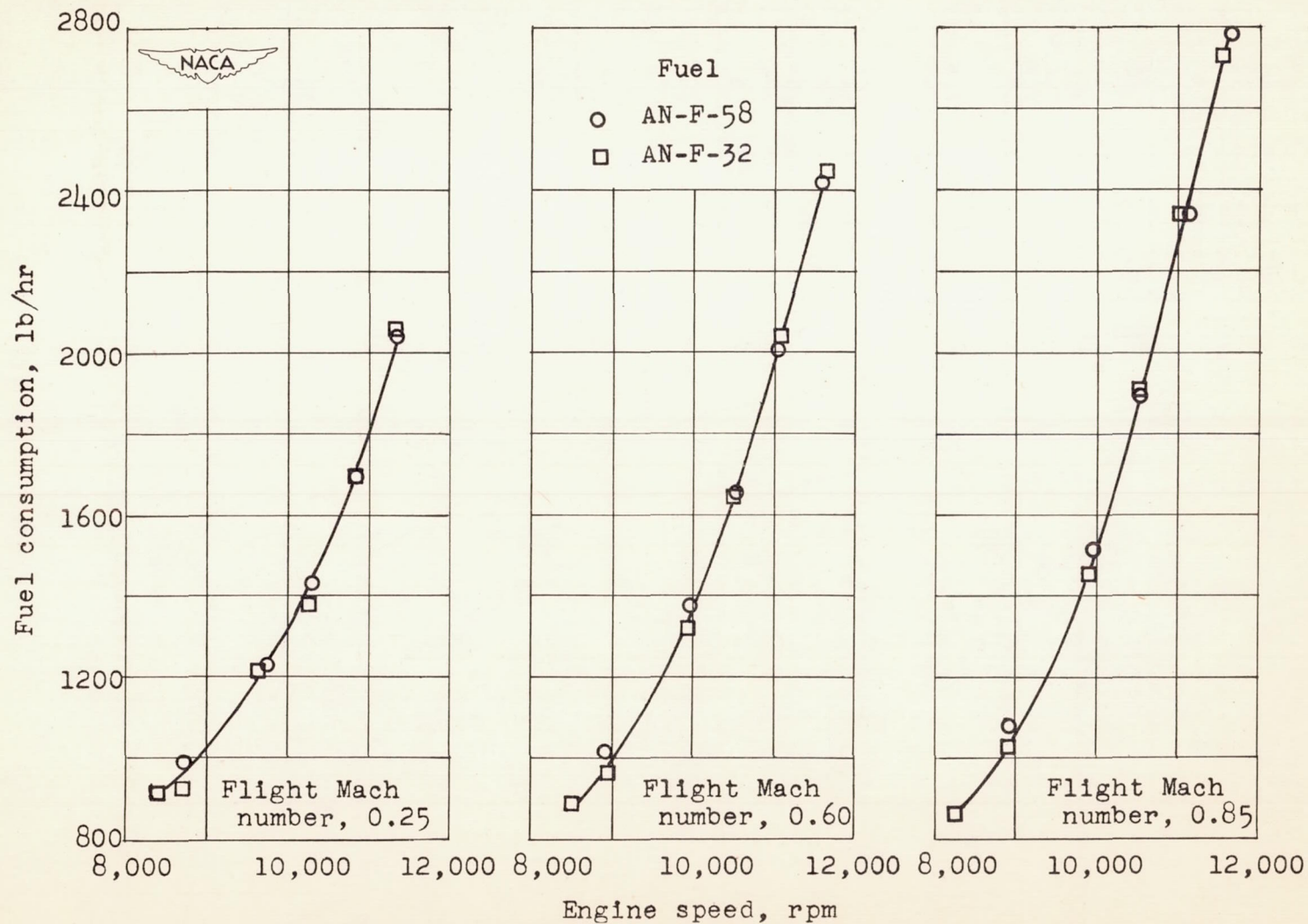
Figure 5. - Fuel consumption using AN-F-58 and AN-F-32 fuels at various flight Mach numbers. Altitude, 30,000 feet.
