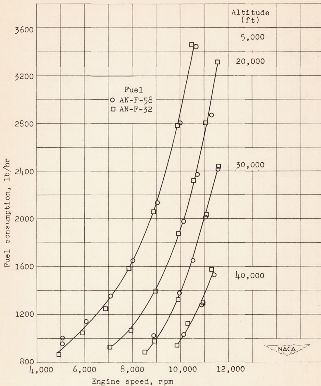
Figure 4. - Fuel consumption using AN-F-58 and AN-F-32 fuels at various altitudes. Flight Mach number, 0.60.
