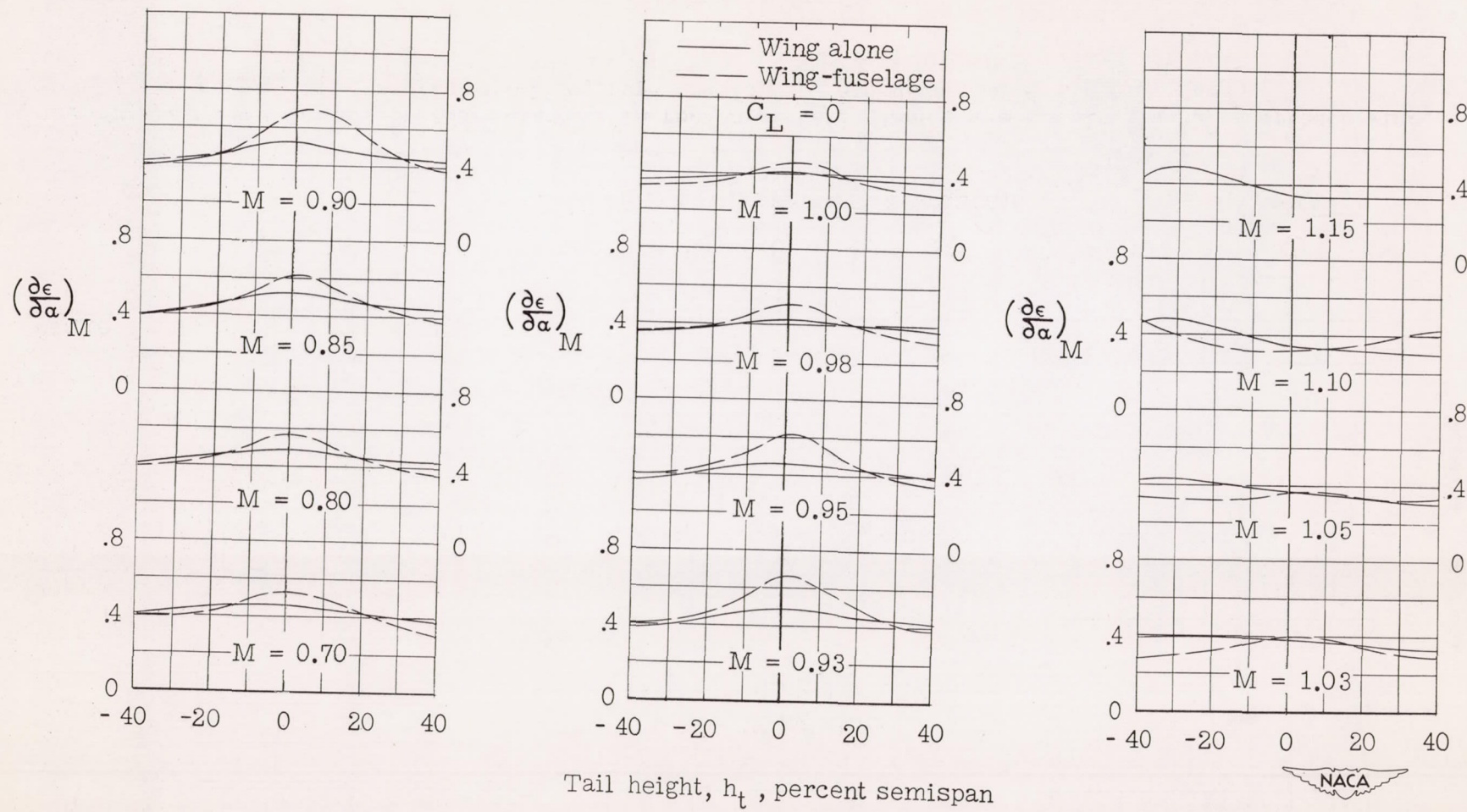
Figure 11.— Variation of downwash gradient with tail height and Mach number for a model with 35^\circ sweptback wing, aspect ratio 4, taper ratio 0.6, and NACA 65A006 airfoil.
