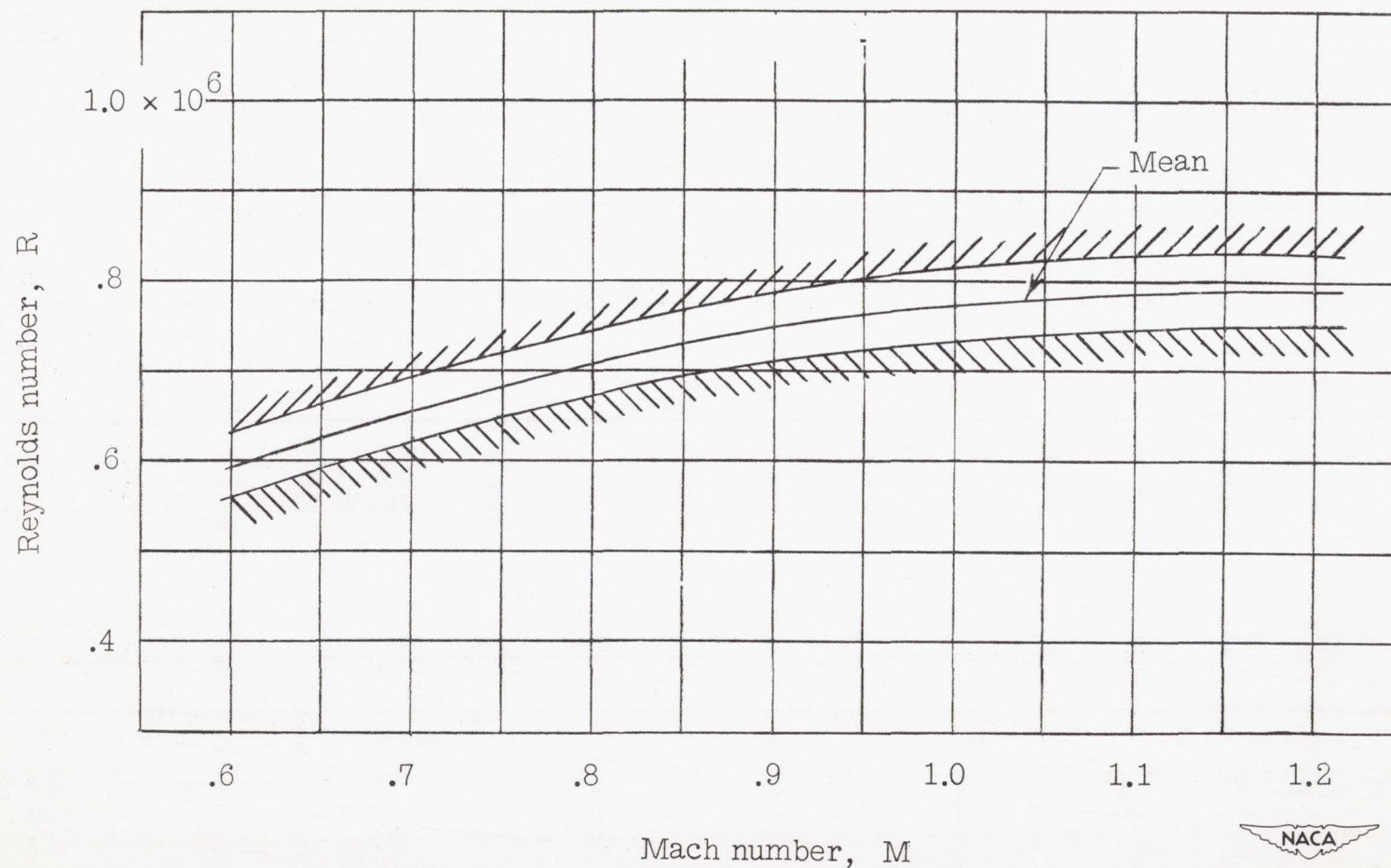
Figure 6.— Variation of test Reynolds number with Mach number for a model with 35^\circ sweptback wing, aspect ratio 4, taper ratio 0.6, and NACA 65A006 airfoil.
