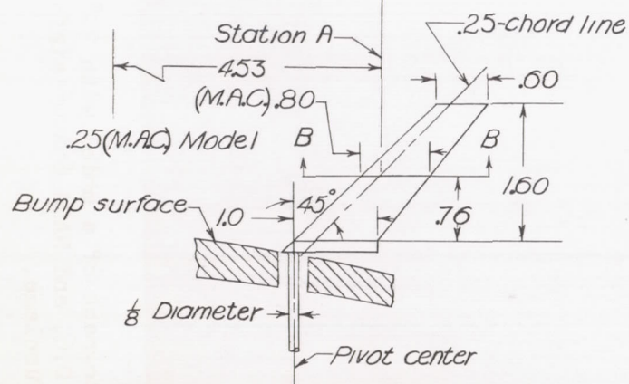
Figure 3.— Details of free-floating tails used in surveys behind a model with 35^\circ sweptback wing, aspect ratio 4, taper ratio 0.6, and NACA 65A006 airfoil.
