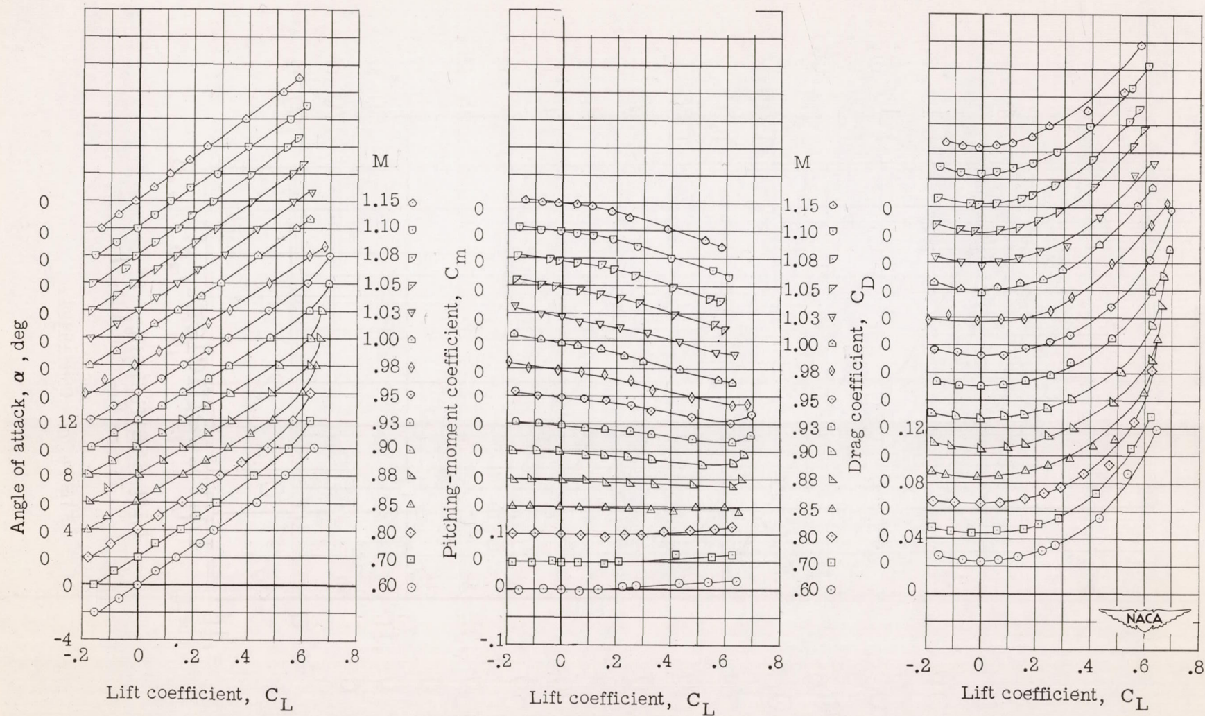
Figure 8.— Wing-fuselage aerodynamic characteristics for a model with 35^\circ sweptback wing, aspect ratio 4, taper ratio 0.6, and NACA 65A006 airfoil.
