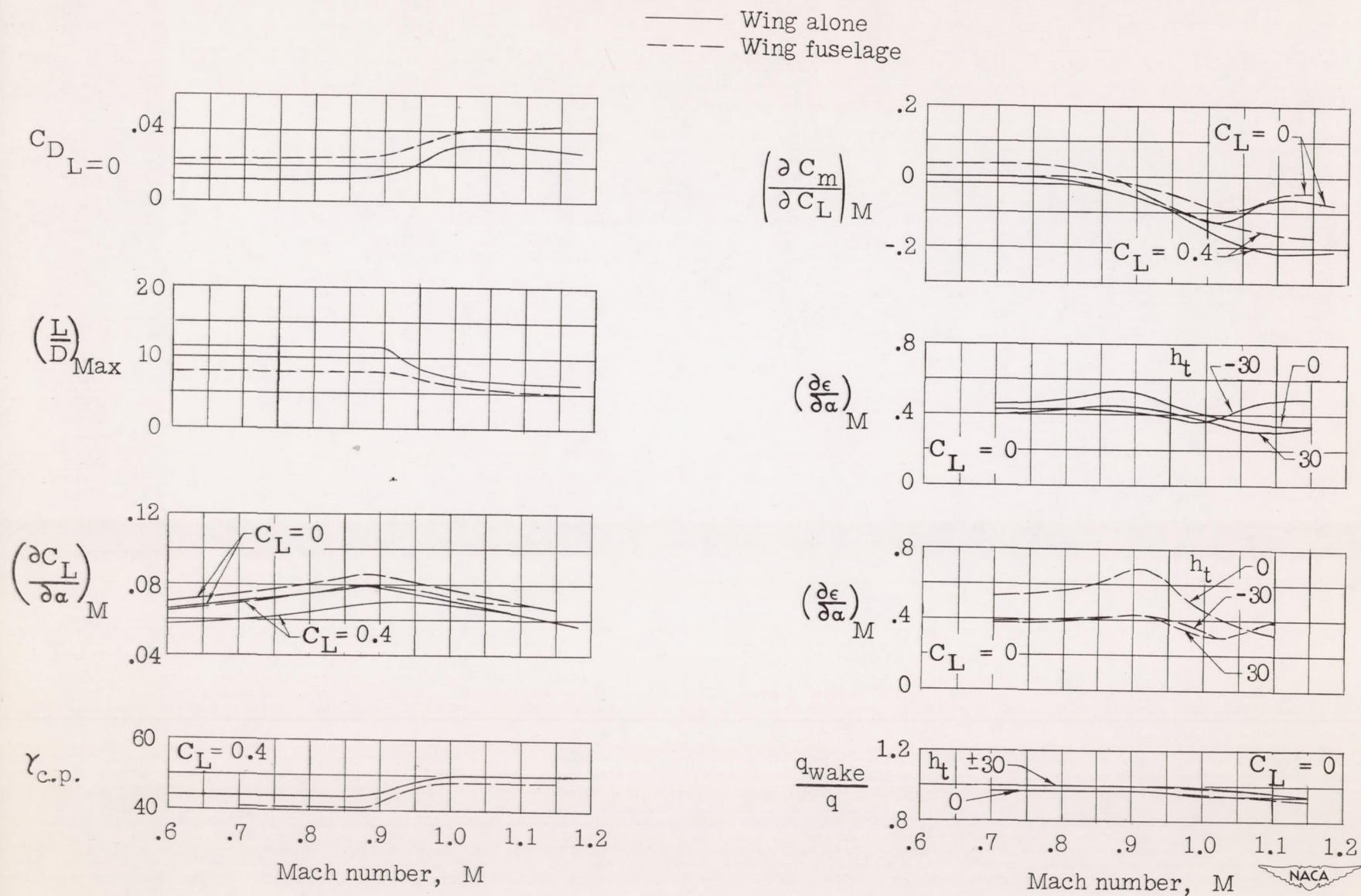
Figure 13.— Summary of aerodynamic characteristics for a model with 35° sweptback wing, aspect ratio 4, taper ratio 0.6, and NACA 65A006 airfoil.
