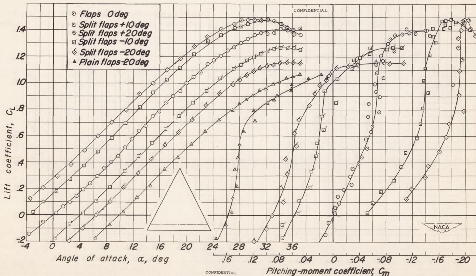
Figure 8.—The lift and pitching-moment characteristics of the flat-plate wing with a constant-chord flap.
