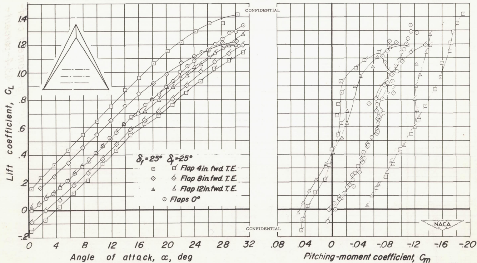
Figure 9.—The lift and pitching-moment characteristics of the 5-percent thick wing with a 43.4-percent-span constant-chord split flap at various chordwise locations.
