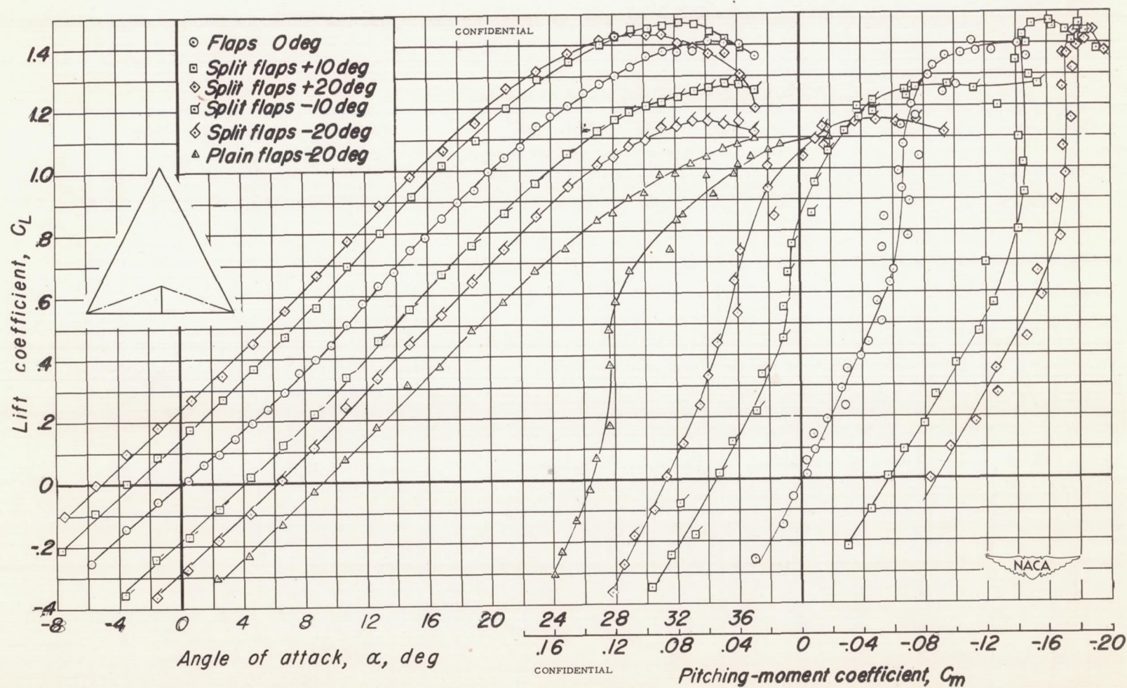
Figure 7.—The lift and pitching-moment characteristics of the flat-plate wing with a constant-percent chord flap.
