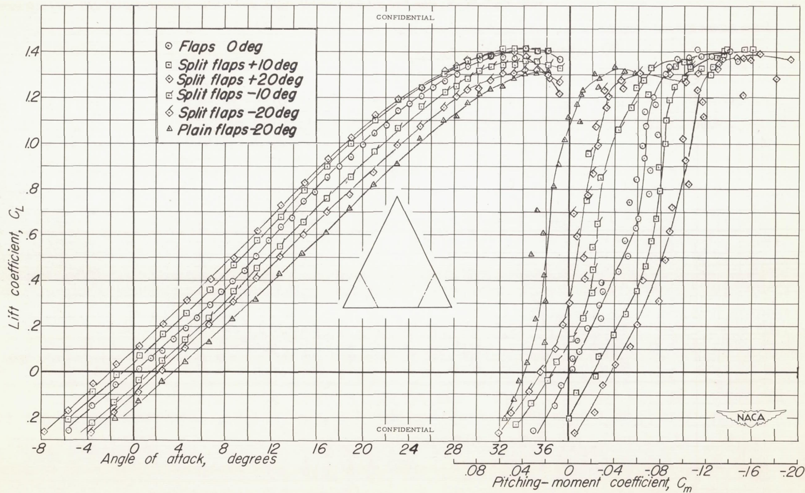
Figure 5.—The lift and pitching-moment characteristics of the flat-plate wing with a skewed tip flap.
