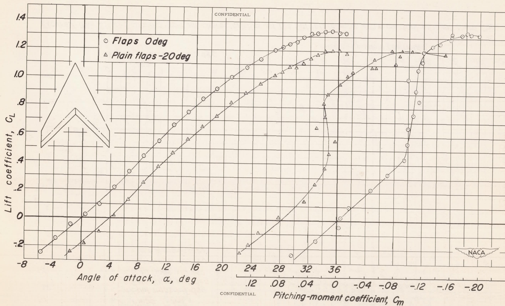
Figure 6.—The lift and pitching-moment characteristics of the flat-plate wing with a swept-back constant-chord flap.
