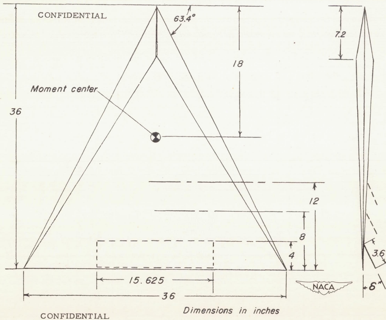
Figure 3.- The chordwise locations of the split flap tested on the 5-percent thick wing.
