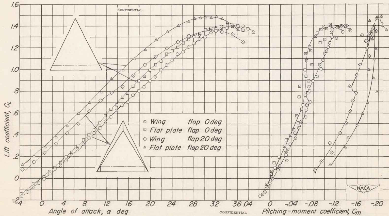
Figure 4.- The lift and pitching-moment characteristics of the flat-plate model and the 5-percent thick double wedge wing with split flaps.
