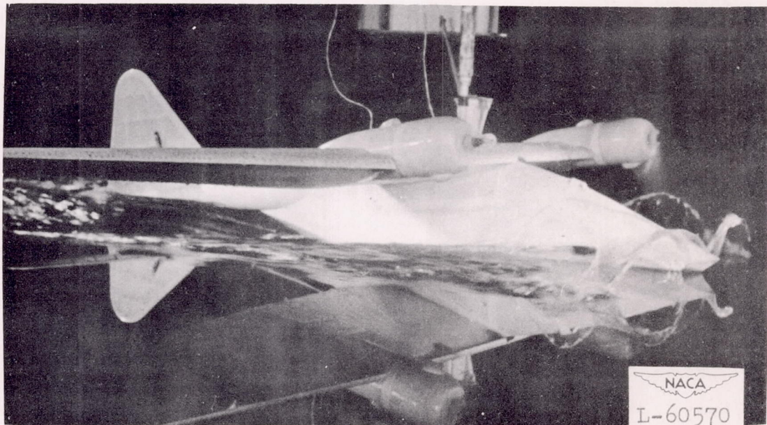
(b) Final spray strip used throughout investigation.
