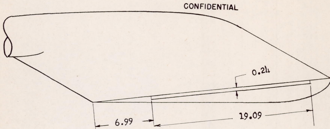
(a) Spray strip similar to that on unswept model.
