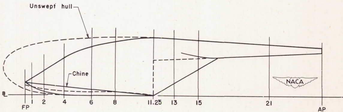
Figure 3.— Hull lines of Langley tank model 237-6SB.
