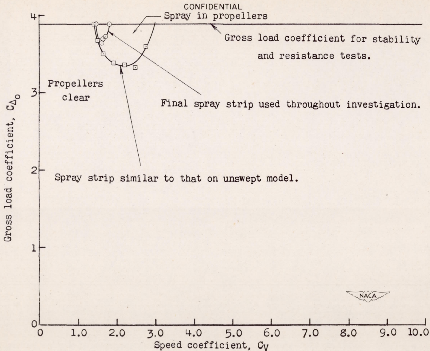
Figure 6.—Gross load coefficients at which spray entered propellers for two spray-strip arrangements.
