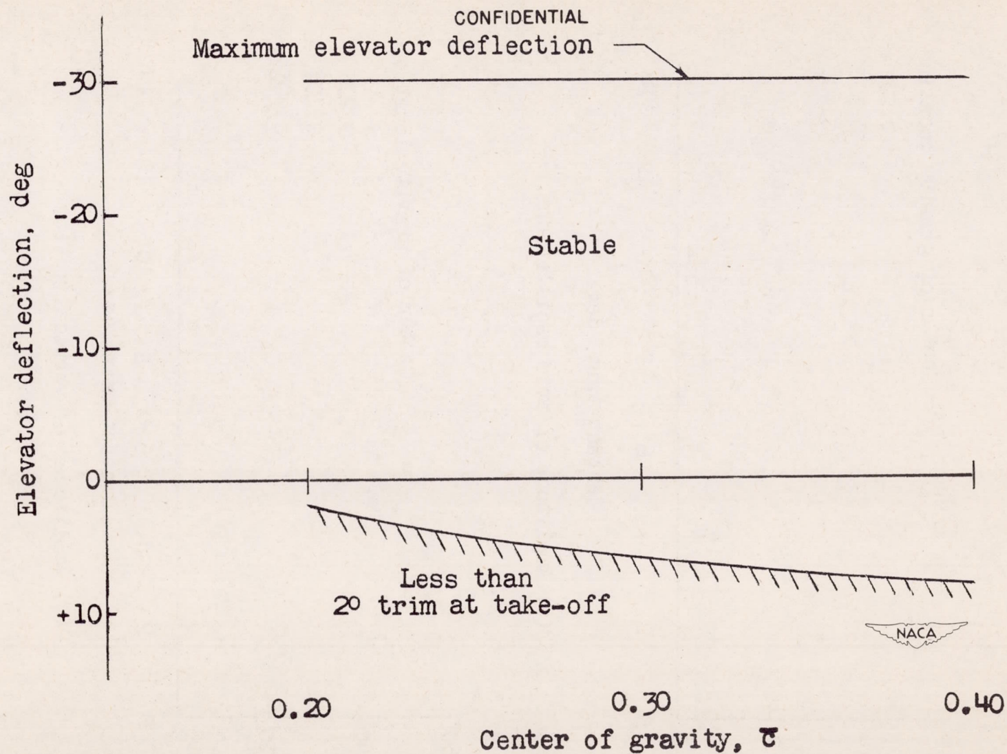
Figure 11.— Elevator limits for various center-of-gravity locations. Gross load coefficient, 3.87, full power.
