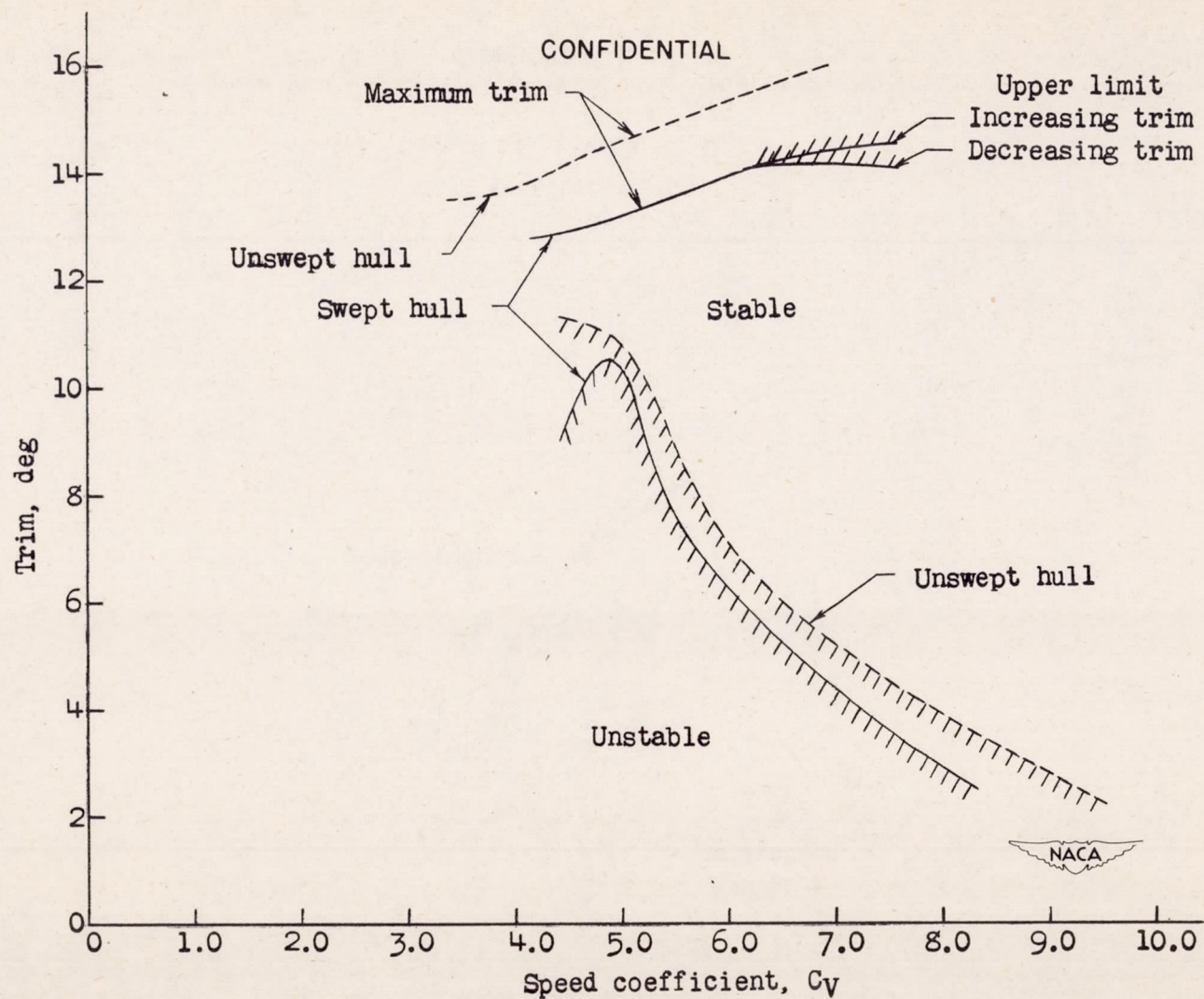
Figure 8.— Trim limits of stability. CONFIDENTIAL
