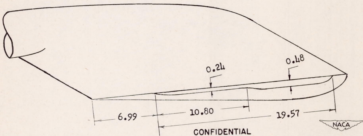
(b) Final spray strip used throughout investigation.
