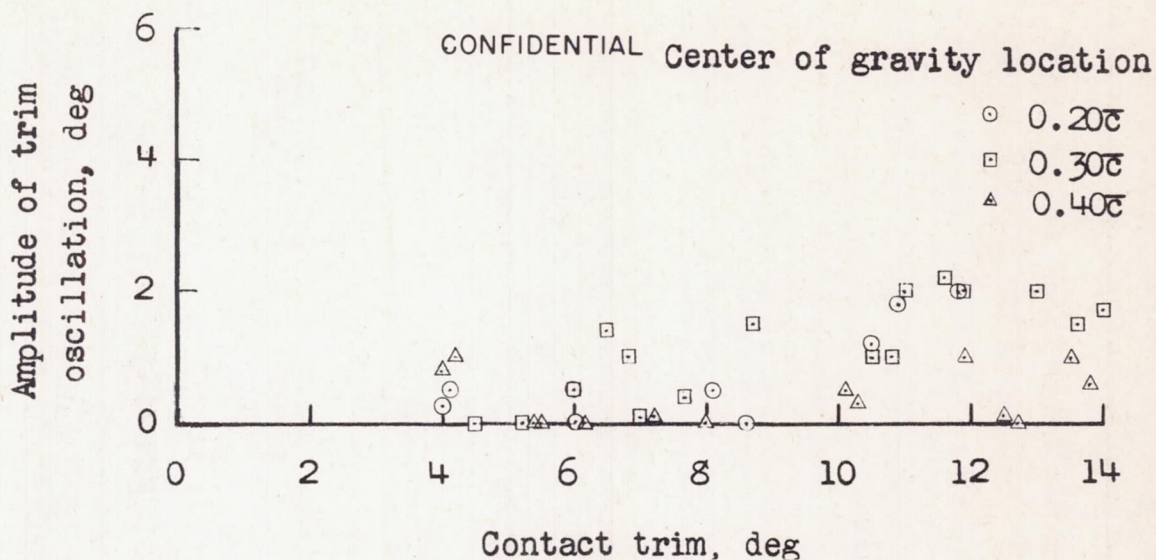
(a) Amplitude of trim oscillations.
