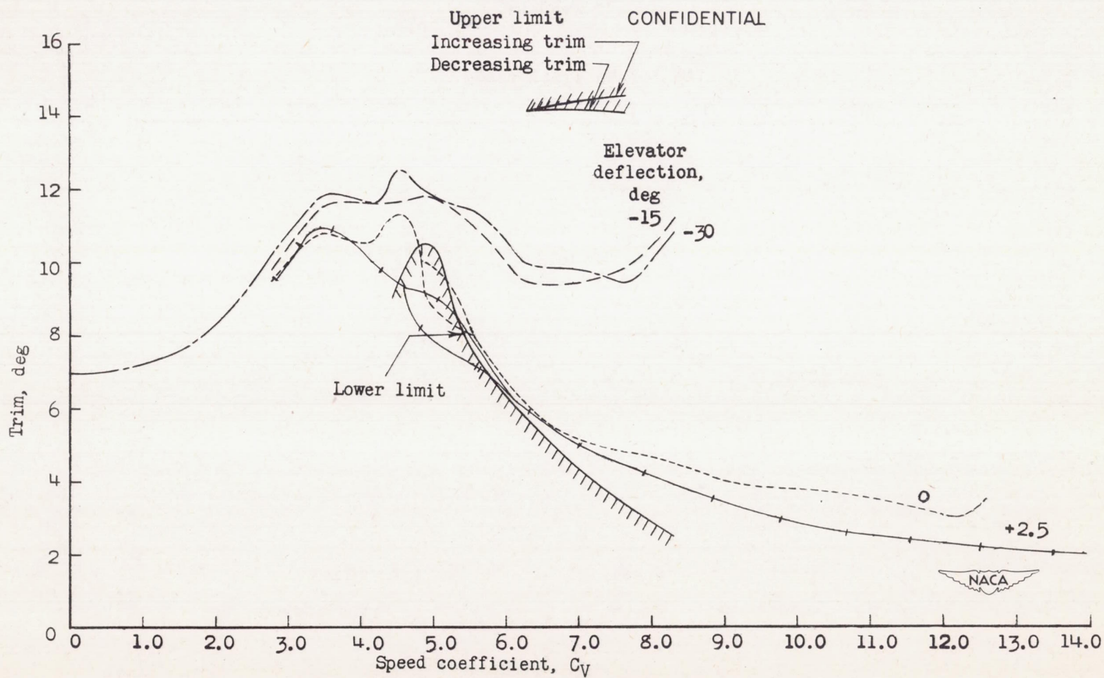
Figure 9.— Variation of trim with speed coefficient.
