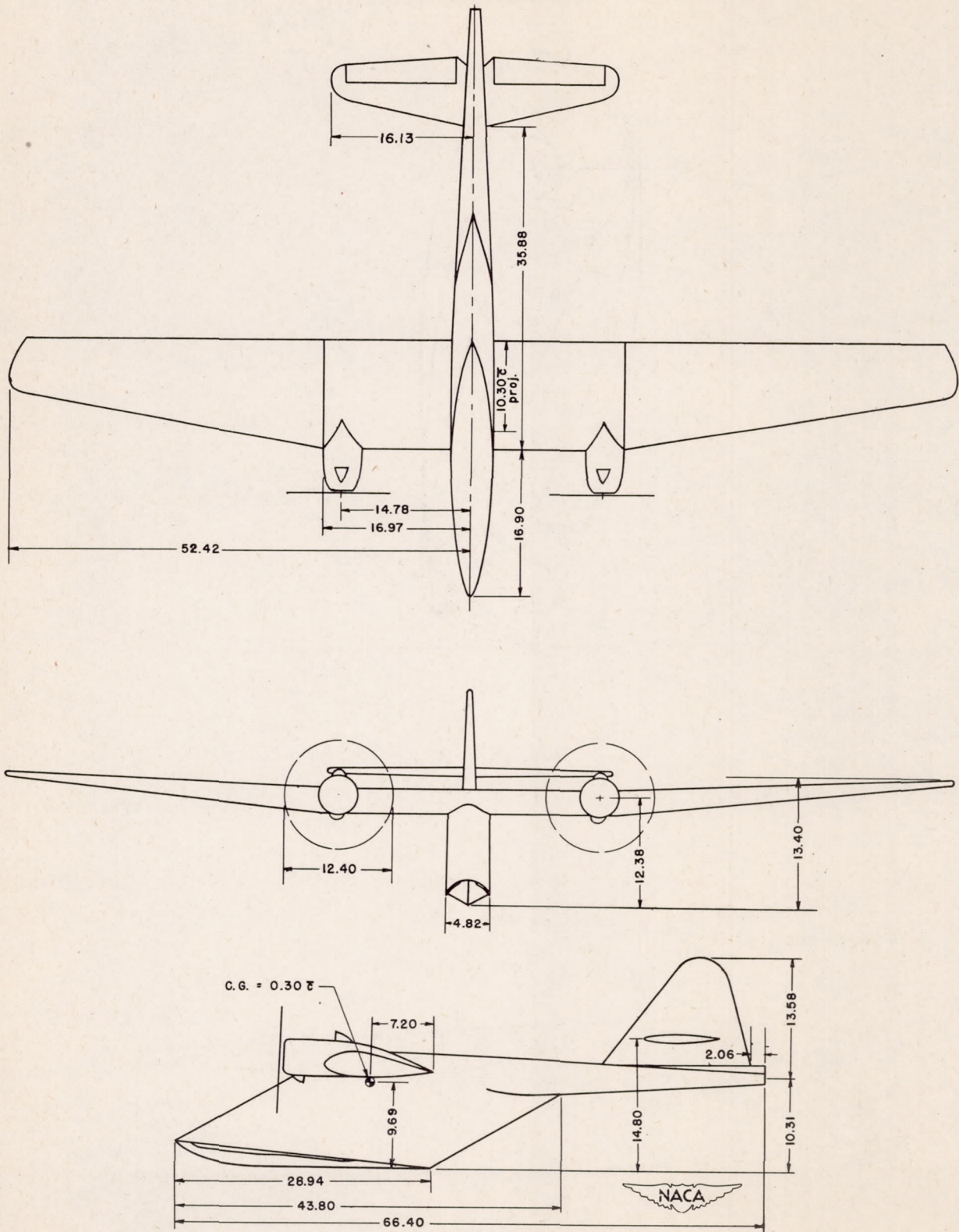
Figure 2.— General arrangement of Langley tank model 237-6SB. (All dimensions in inches.)
