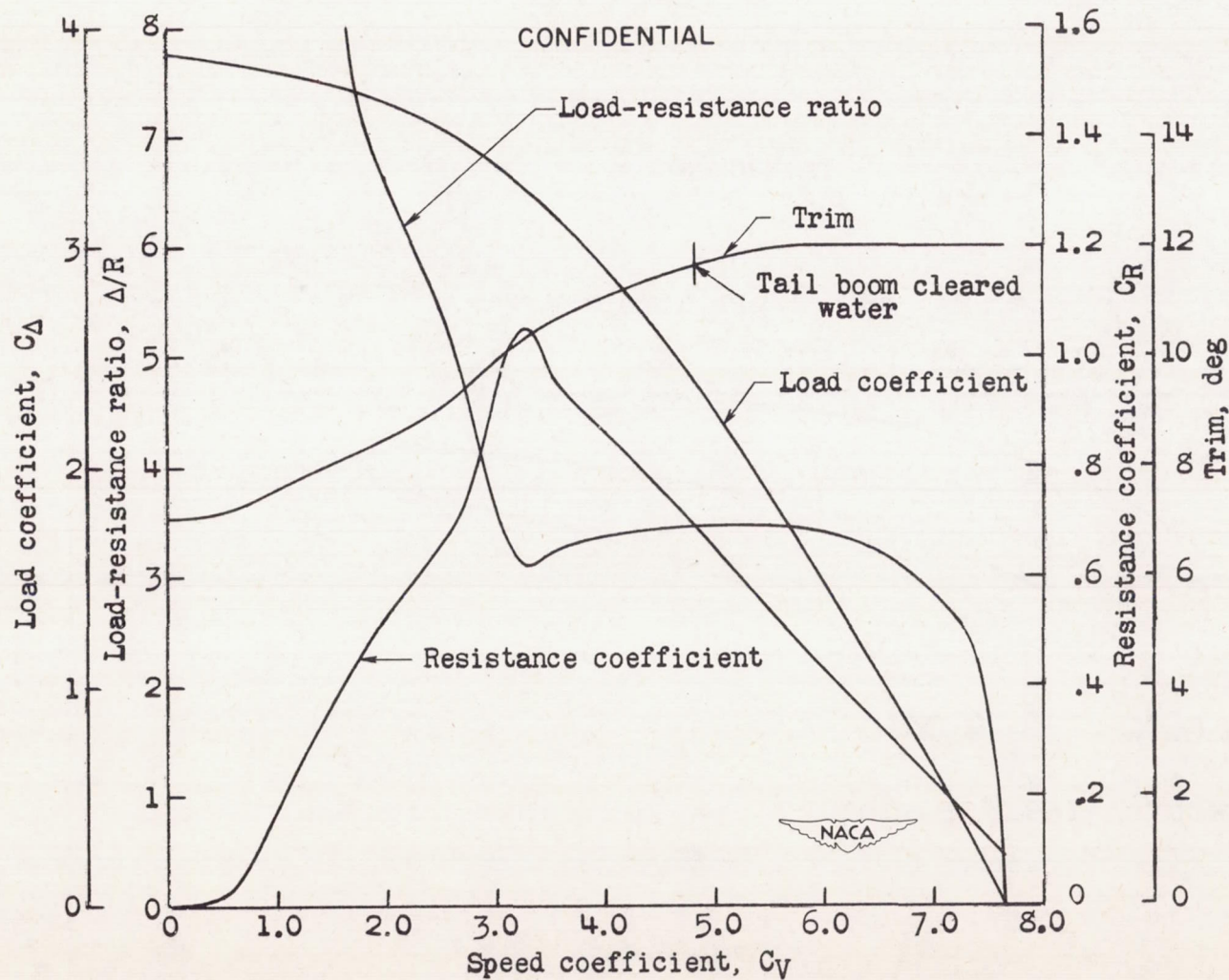
Figure 14.— Resistance coefficient, load-resistance ratio, trim and load coefficient for minimum stable resistance.
