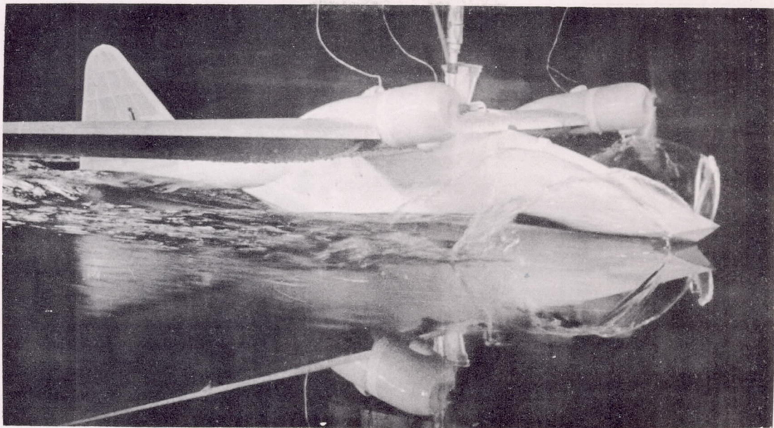
(a) Spray strip similar to that on unswept model.
