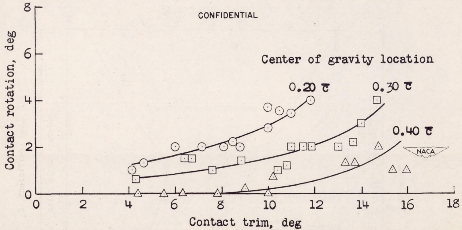
Figure 13.- Change in trim at contact.
