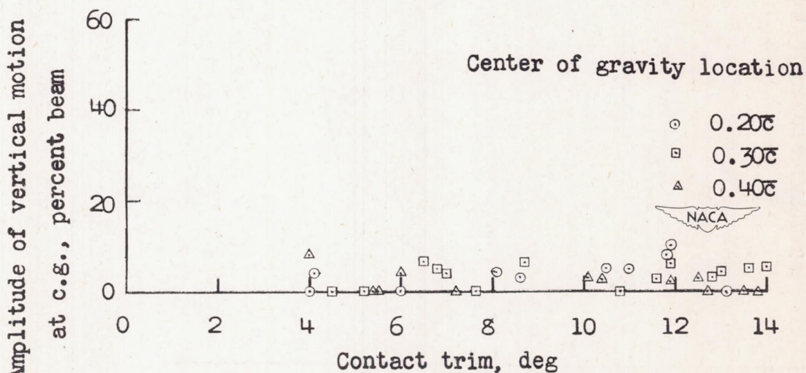
(b) Amplitudes of vertical motion.
