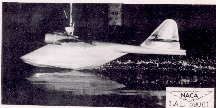
(c) C_V = 11.08 ; \tau = 3.5^\circ ; \delta_e = 0^\circ .
