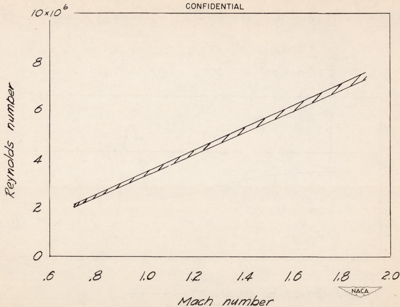
Figure 3.— Variation of Reynolds number with Mach number for range of climatic conditions encountered during tests. CONFIDENTIAL
