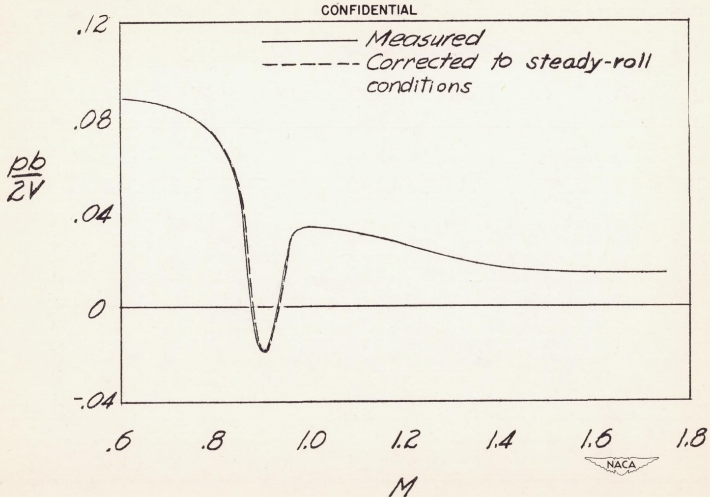
Figure 4.— Effect of moment of inertia about roll axis on measured variation of \frac{pb}{2V} with Mach number. CONFIDENTIAL
