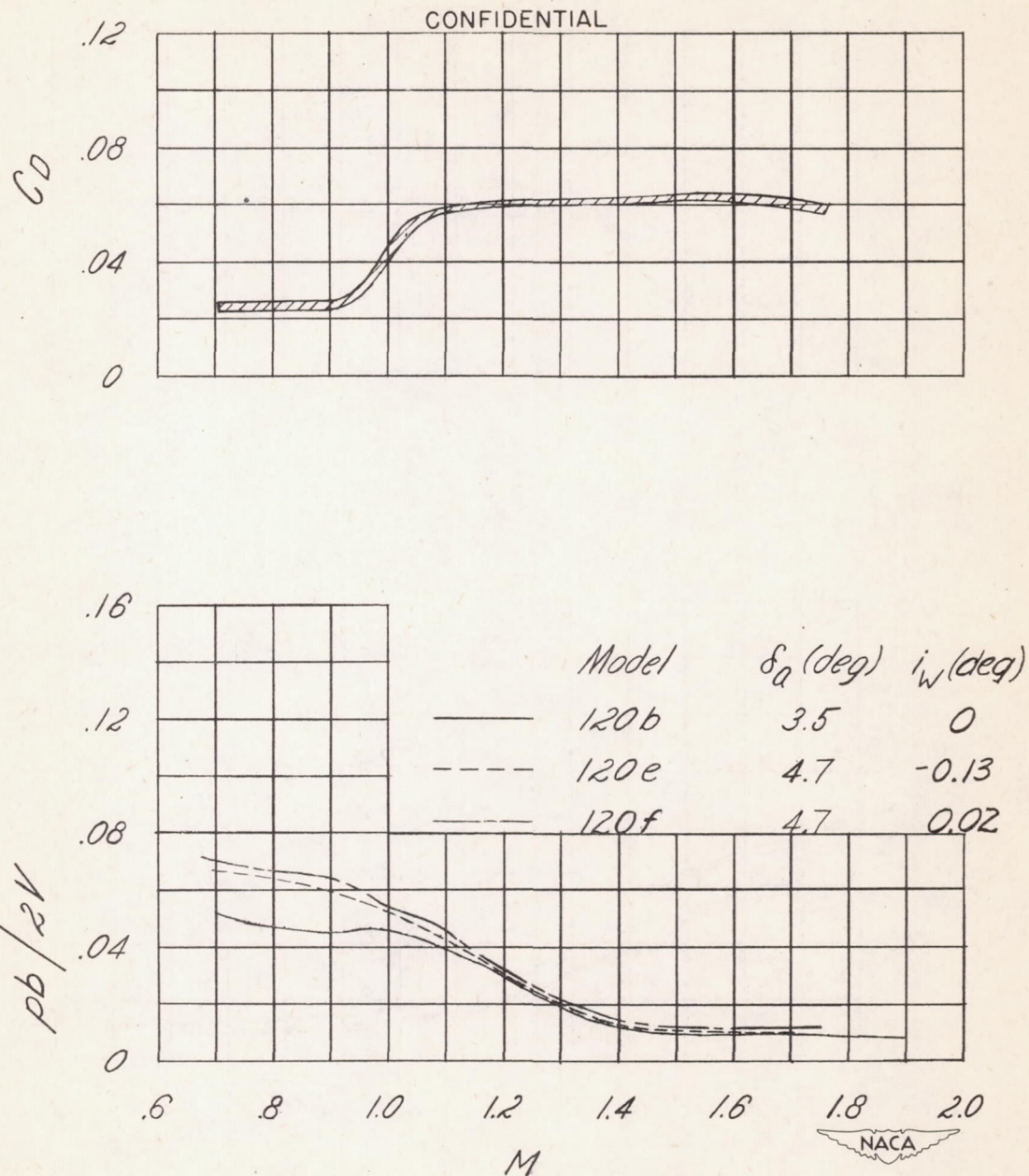
(b) 9-percent-thick double-wedge airfoil section.
