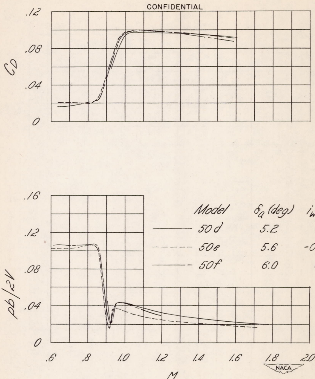
(a) NACA 65A009 airfoil section.
