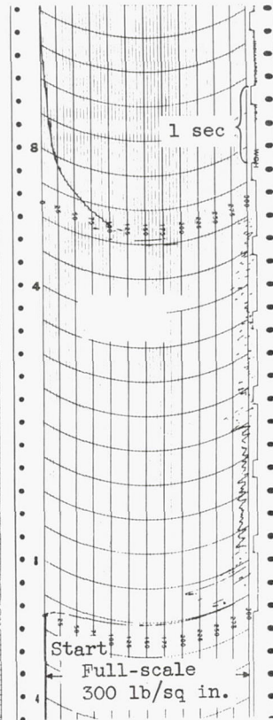
Combustion-chamber pressure
