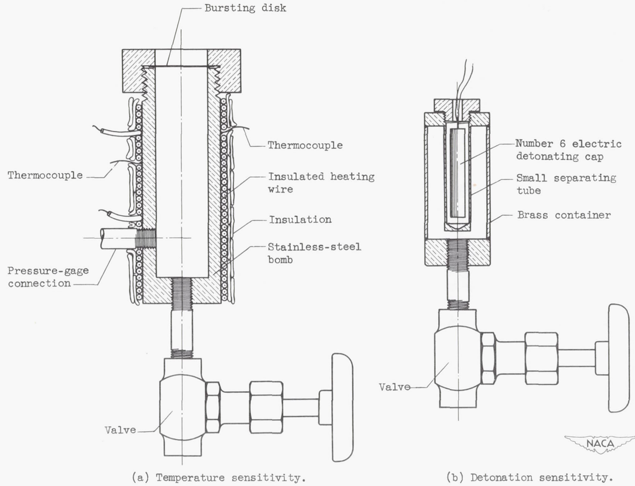
Figure 9. - Sensitivity apparatus.
