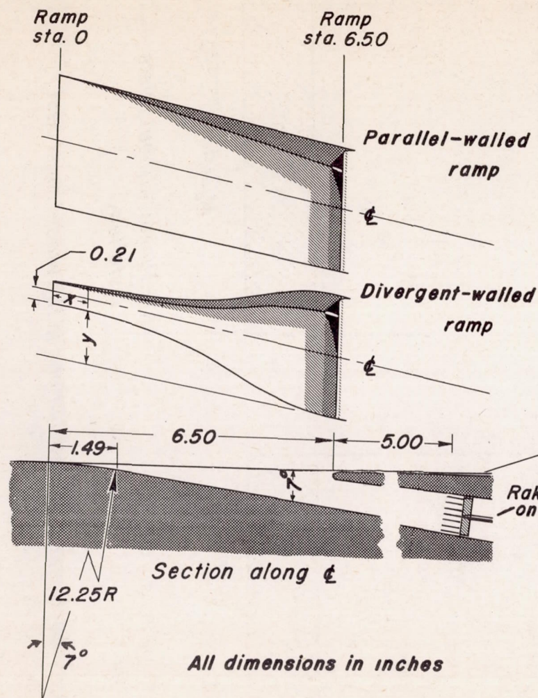
Figure 3.— General arrangement and dimensions of the submerged-type inlets.
