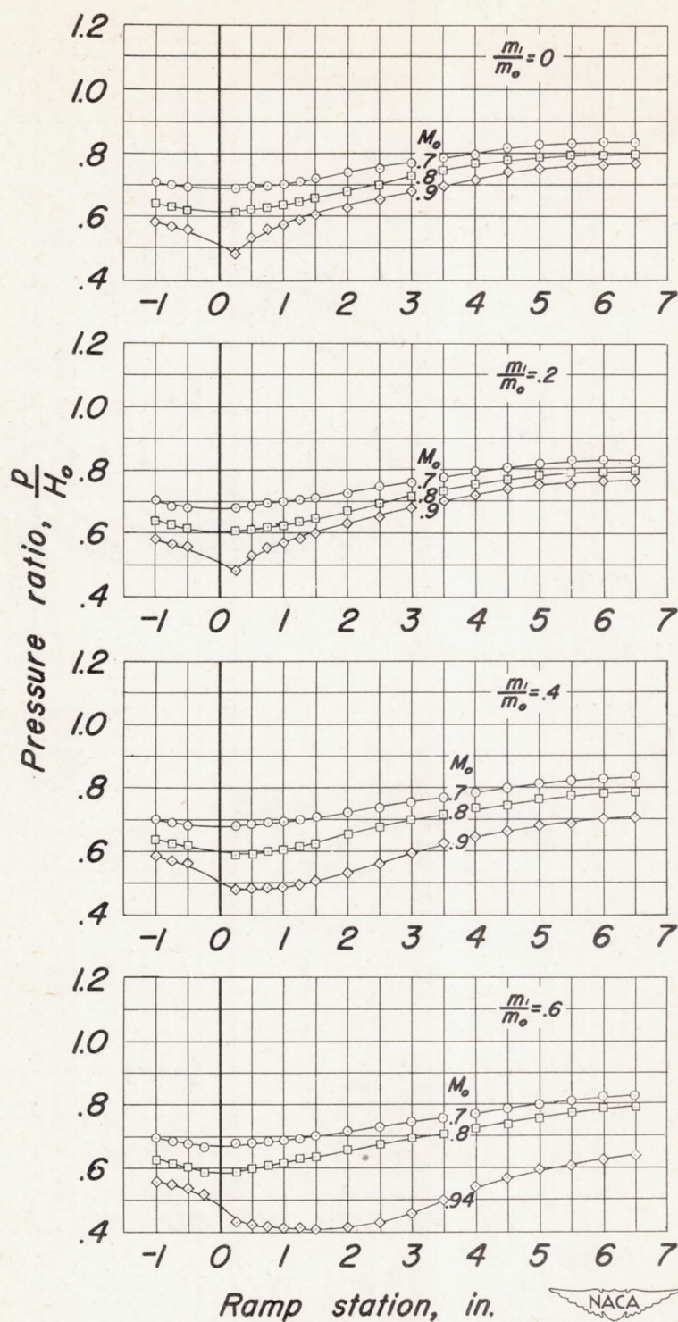
Figure 8.— Pressure distribution along the ramp center line for various free-stream Mach numbers.
