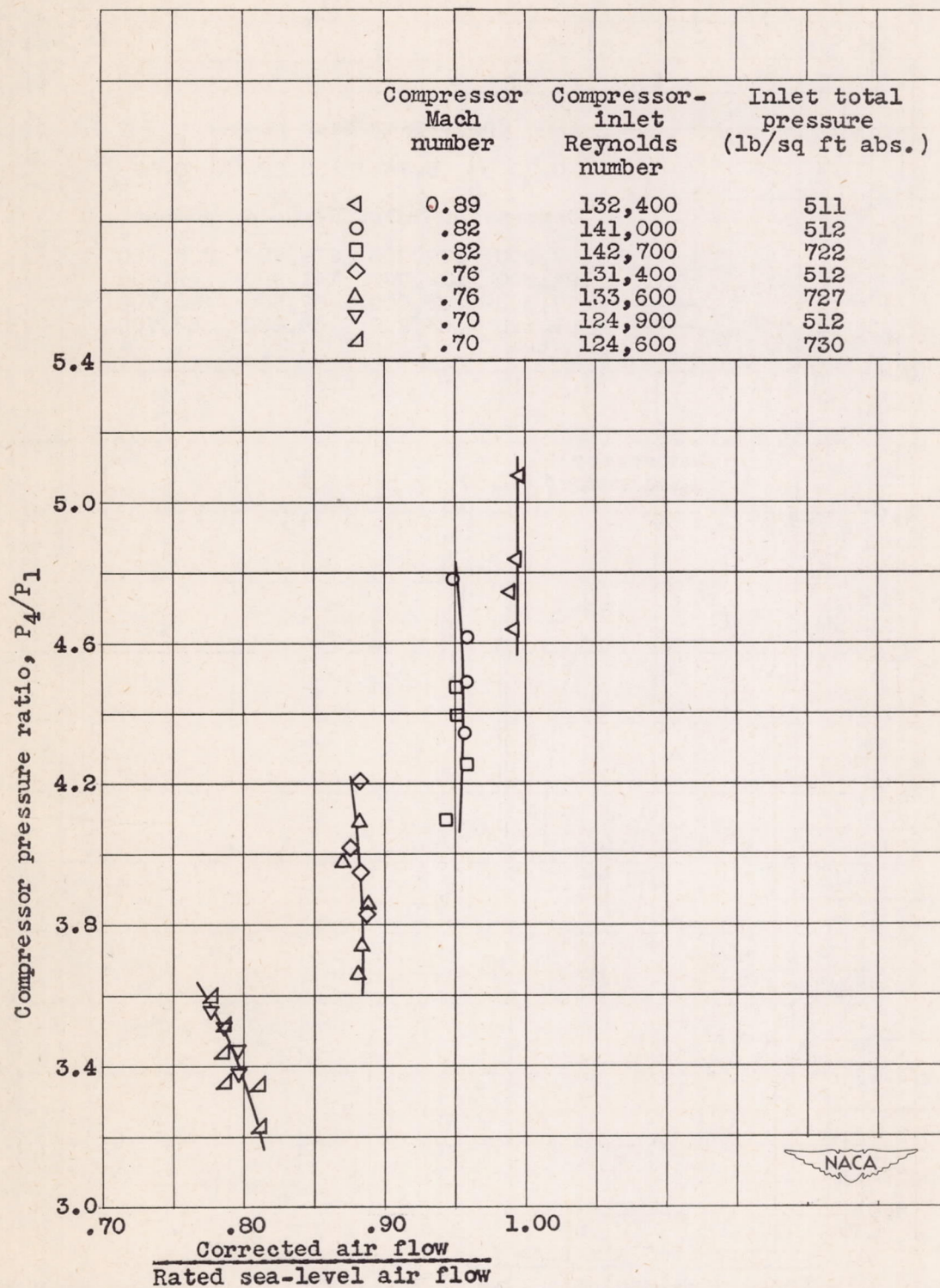
Figure 8. - Variation of compressor pressure ratio with fraction of rated sea-level air flow for constant values of compressor Mach number and compressor-inlet Reynolds number.
