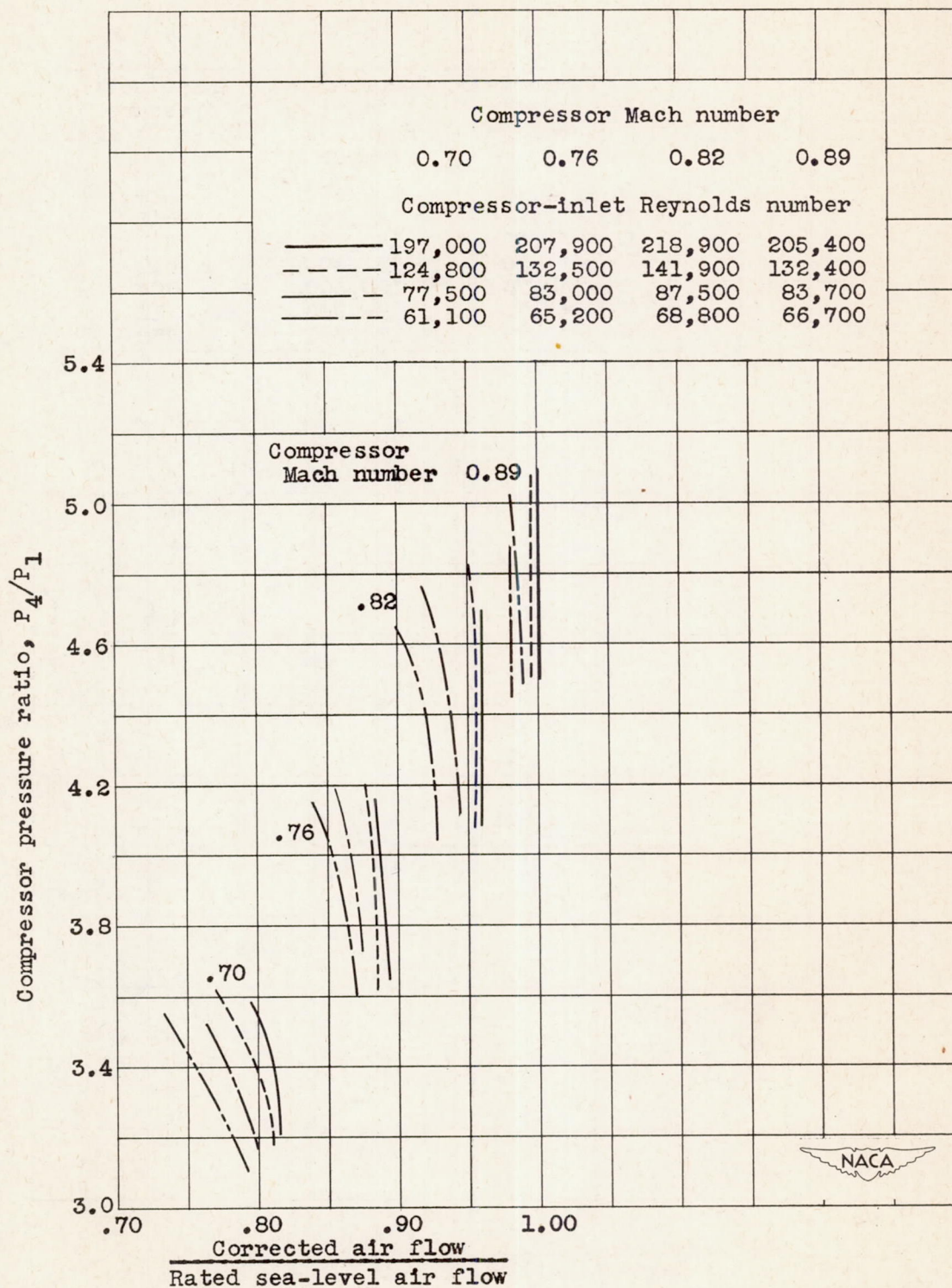
Figure 9. - Effect of compressor-inlet Reynolds number on relation between compressor pressure ratio and fraction of rated sea-level air flow.
