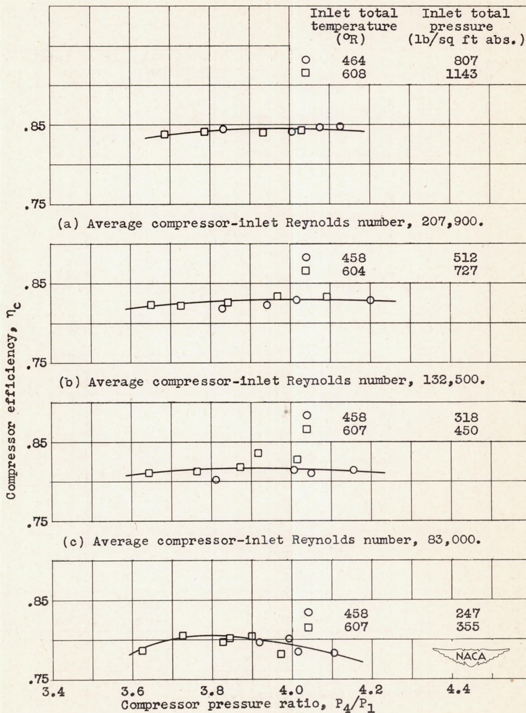
Figure 5. - Variation of compressor efficiency with compressor pressure ratio at compressor Mach number of 0.76.
