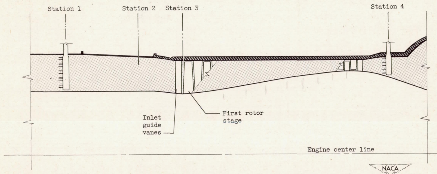
Figure 1. - Schematic view of compressor showing measuring stations.
