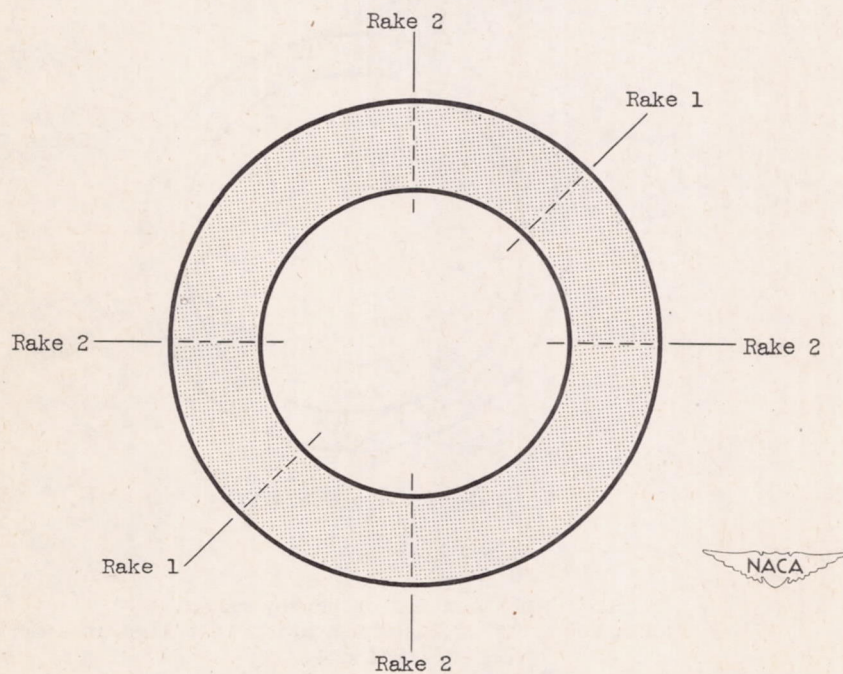
Figure 2. - Location and details of instrumentation installed at engine inlet, station 1.
