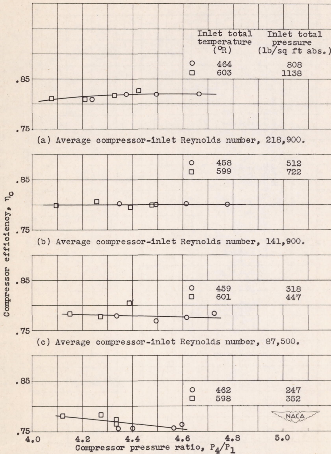
Figure 6. - Variation of compressor efficiency with compressor pressure ratio at compressor Mach number of 0.82.
