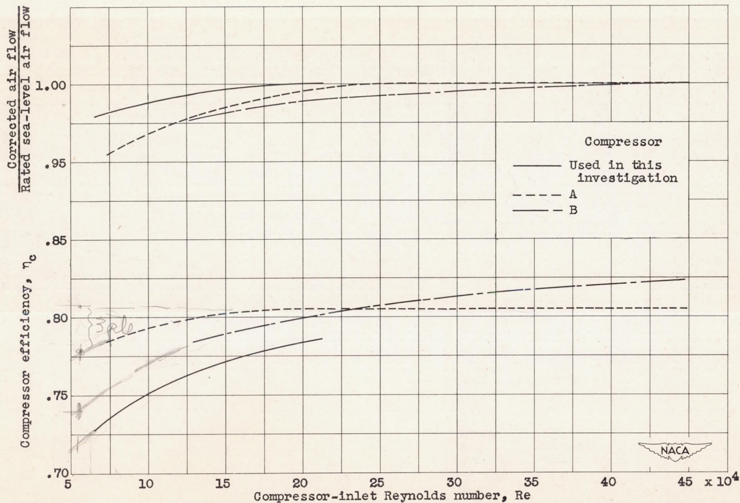
Figure 11. - Comparison of Reynolds number effect at rated Mach number on performance of compressor studied in this investigation and compressors of two other current turbojet engines.
