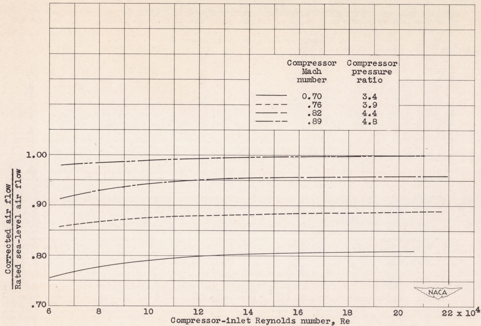
Figure 10. - Effect of compressor-inlet Reynolds number on fraction of rated sea-level air flow.
