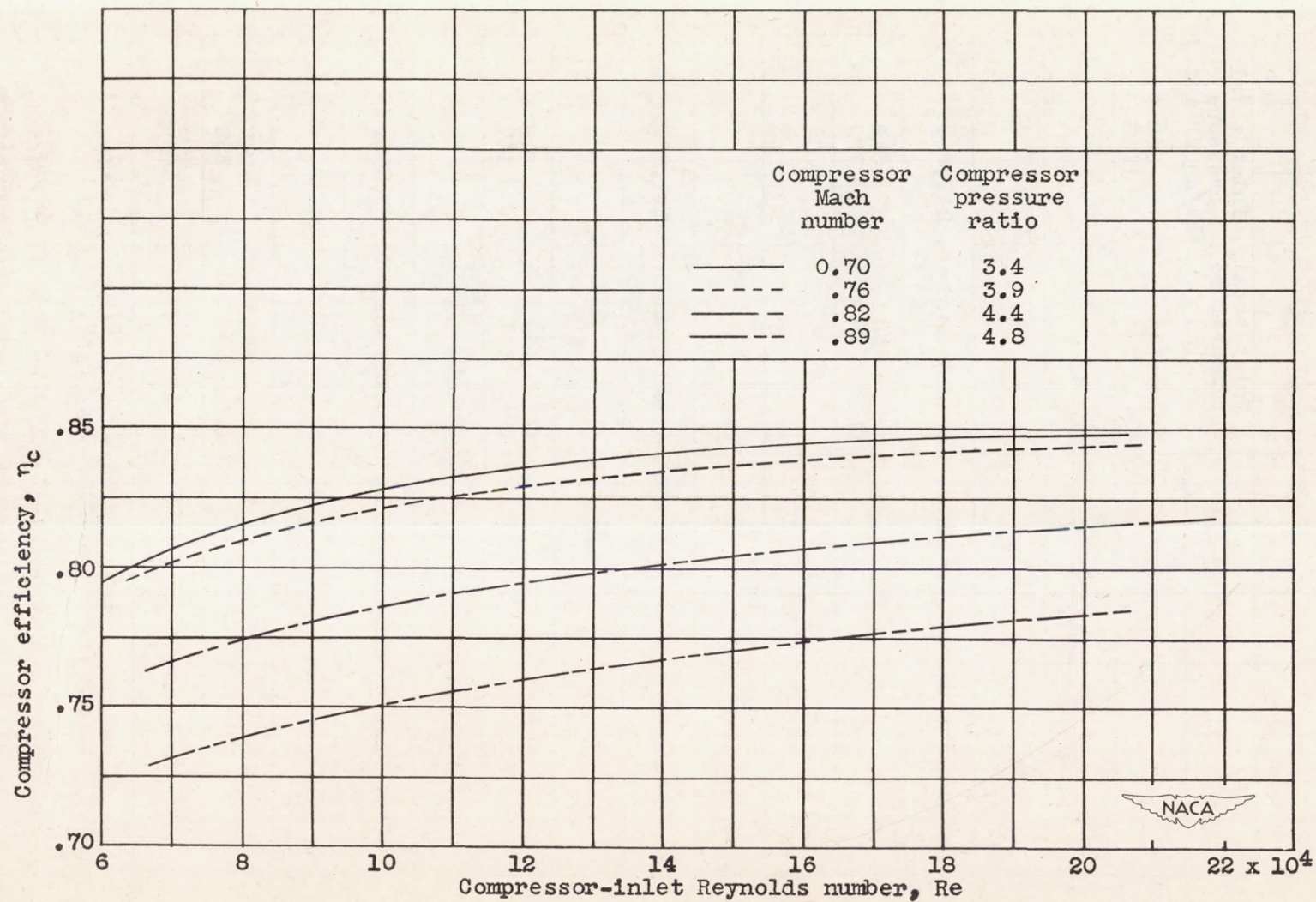
Figure 7. - Effect of compressor-inlet Reynolds number on compressor efficiency.
