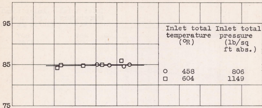
(a) Average compressor-inlet Reynolds number, 197,000.
