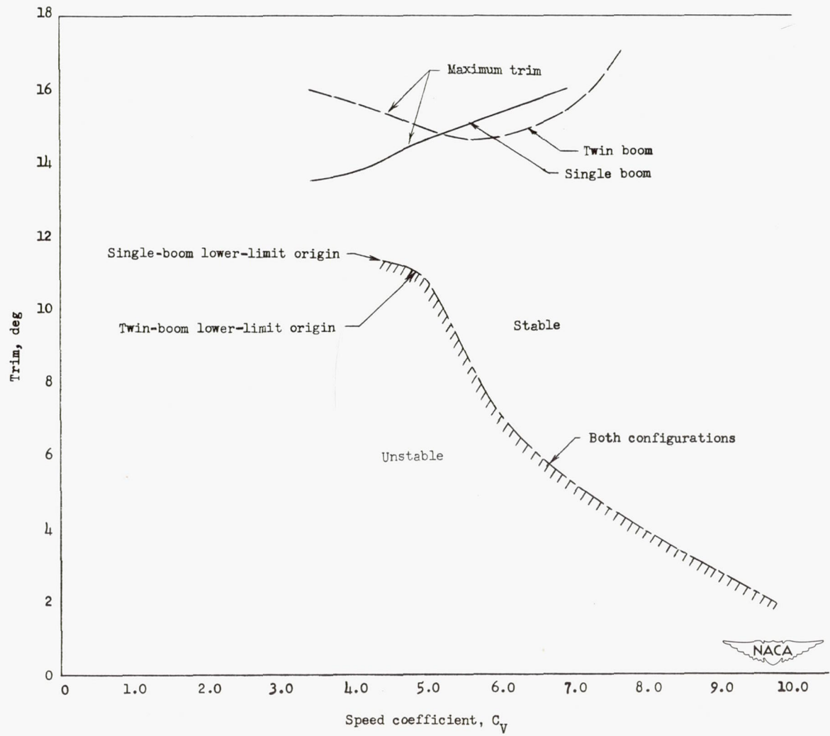
Figure 9.- Trim limits of stability.
