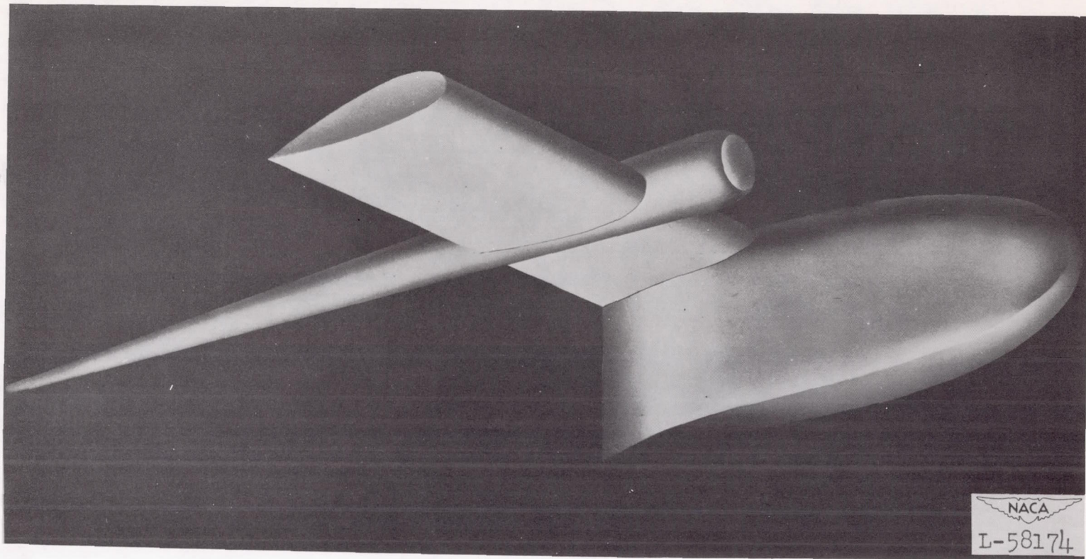
(b) With twin booms. (Langley tank model 237-7TB.)
