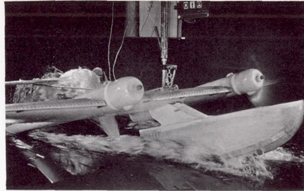
(b) C_V = 2.92 ; trim = 10.4^\circ .
