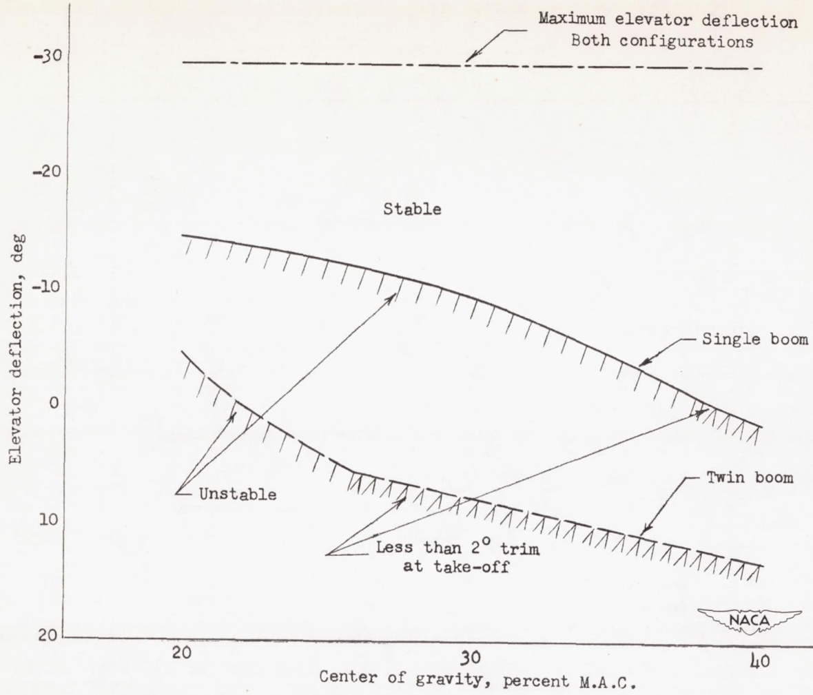
Figure 8.- Center-of-gravity limits of stability. Gross load coefficient 3.87; full power.
