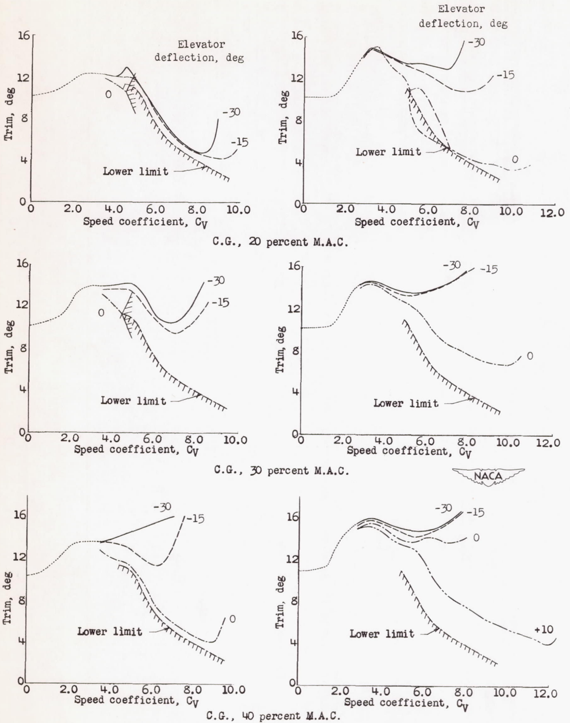
(a) Single boom.
