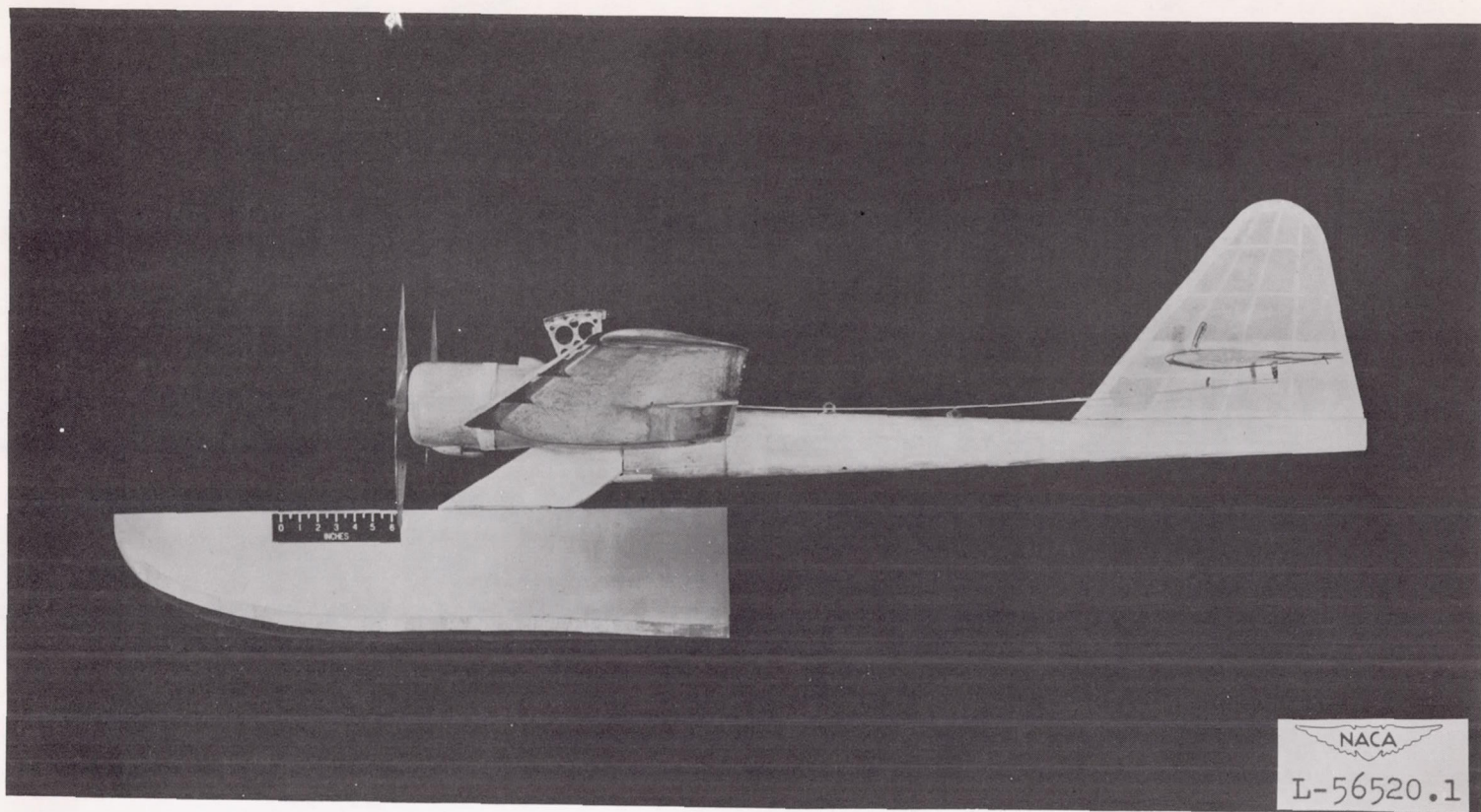
(a) Profile view.
