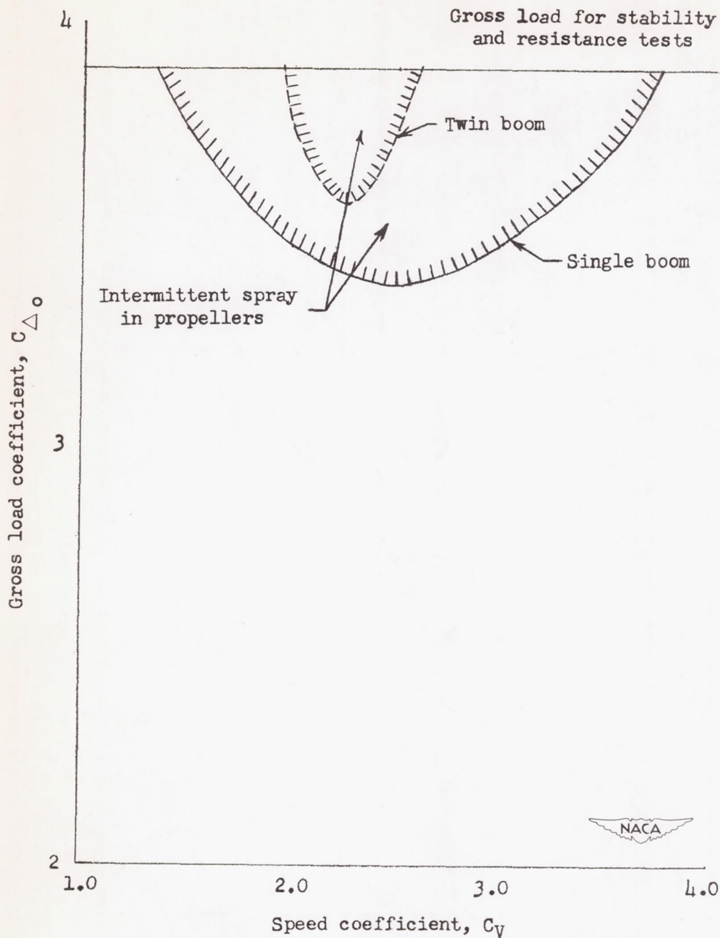
Figure 15.- Gross load coefficient at which spray enters propellers.
