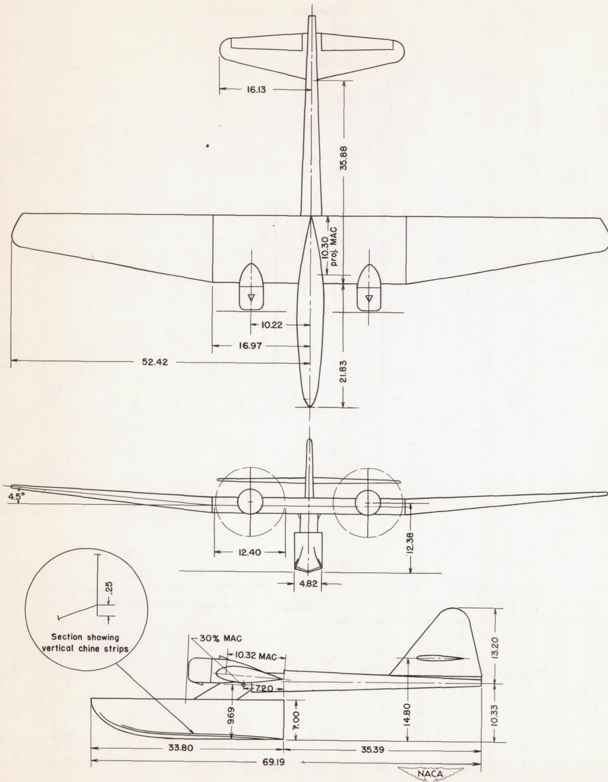
Figure 3.- General arrangement of model 237-7B. (All dimensions are in inches.)
