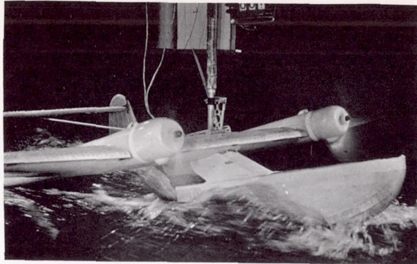
(a) C_V = 2.12 ; trim = 13.2^\circ .
