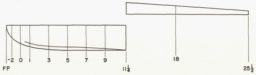
Figure 7.- Hull lines of model 237-7TB.
