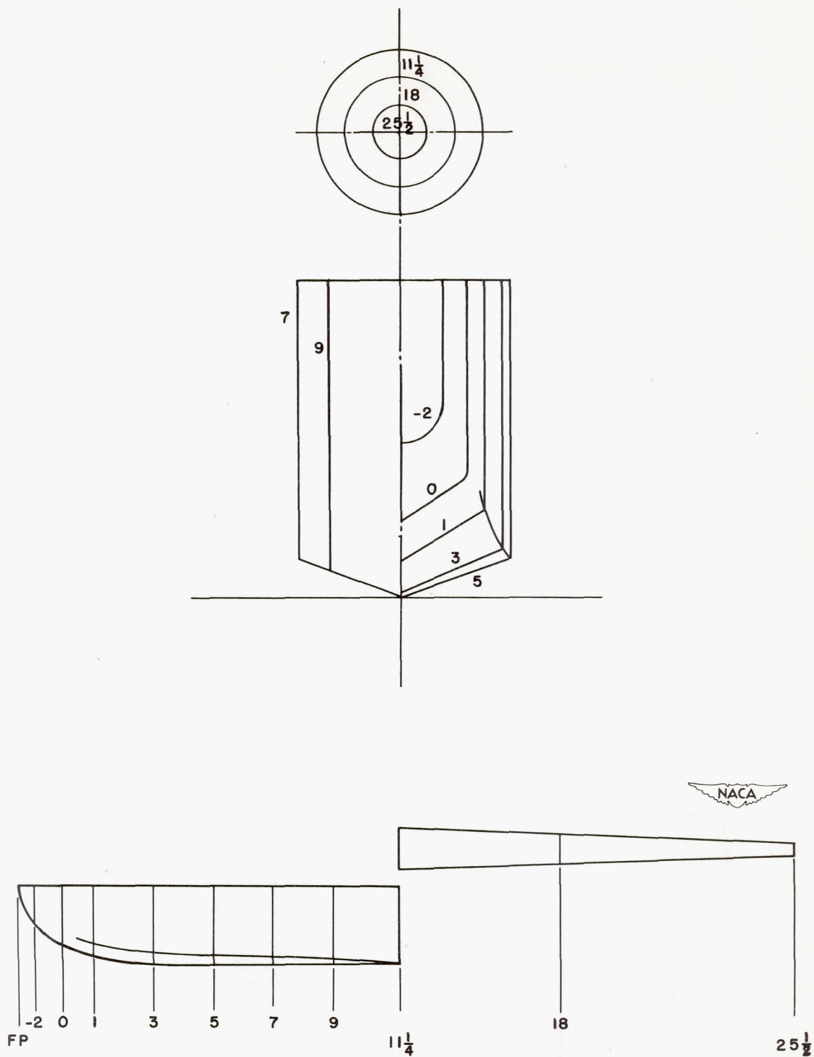
Figure 4.- Hull lines of model 237-7B.
