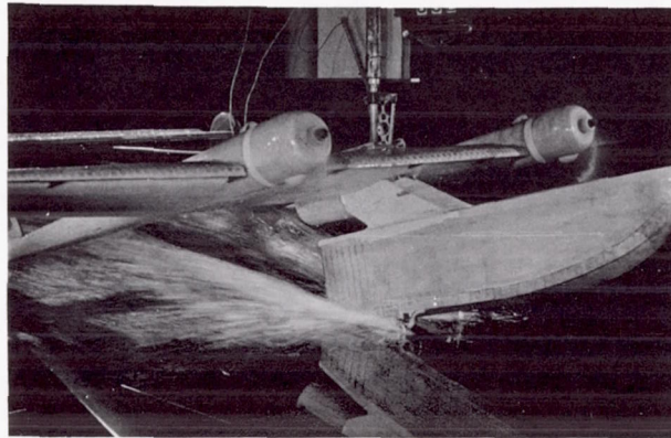
(c) C_V = 6.26 ; trim = 13.6^\circ .
