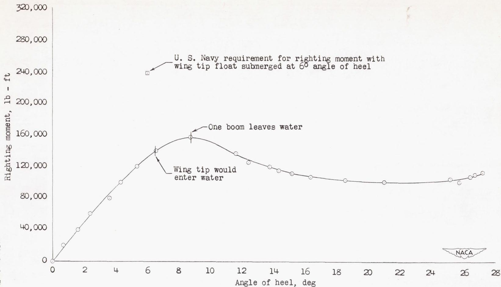
Figure 17.- Righting moment of twin-boom configuration without tip floats.
