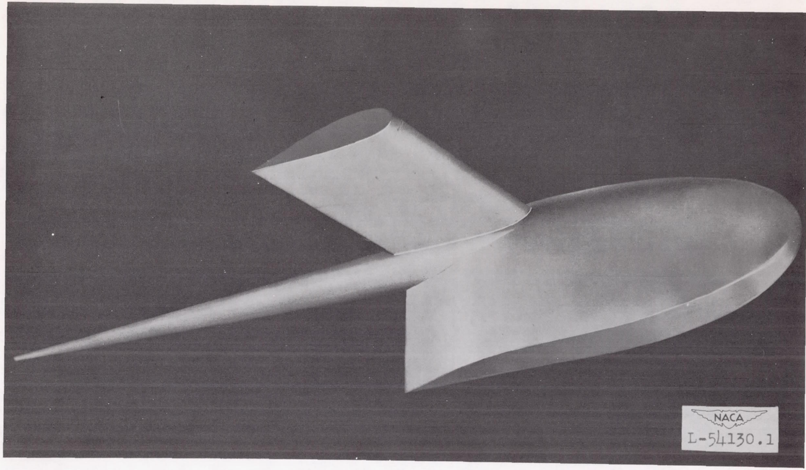
(a) With single boom. (Langley tank model 237-7B.)
