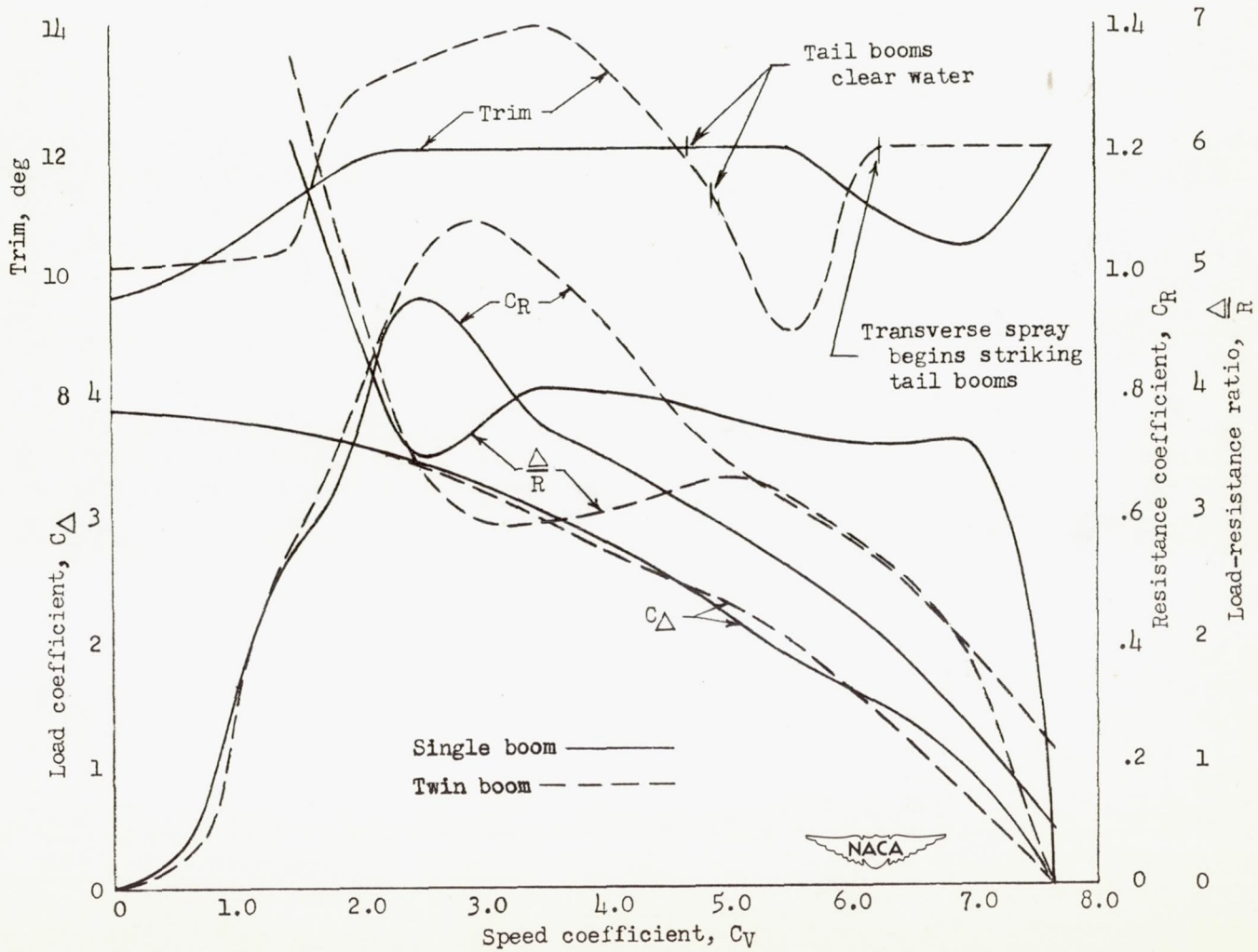
Figure 16.- Minimum stable resistance characteristics for single-boom and twin-boom hulls.
