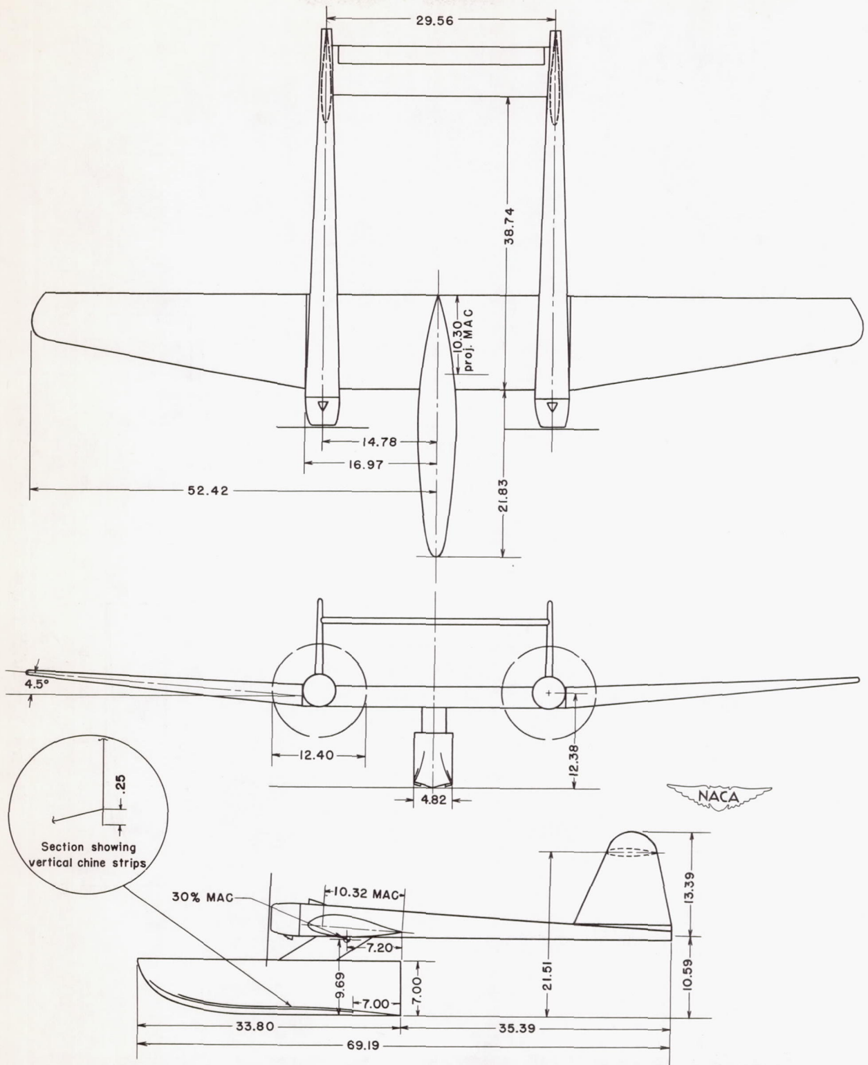
Figure 6.- General arrangement of model 237-7TB. (All dimensions are in inches.)
