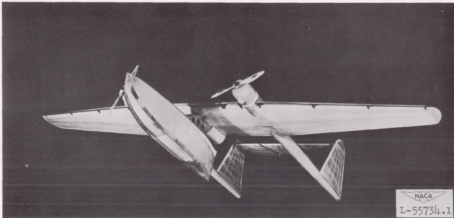
(a) Three-quarter bottom view.
