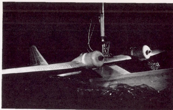
(b) C_V = 1.94 ; trim = 11.4°.
