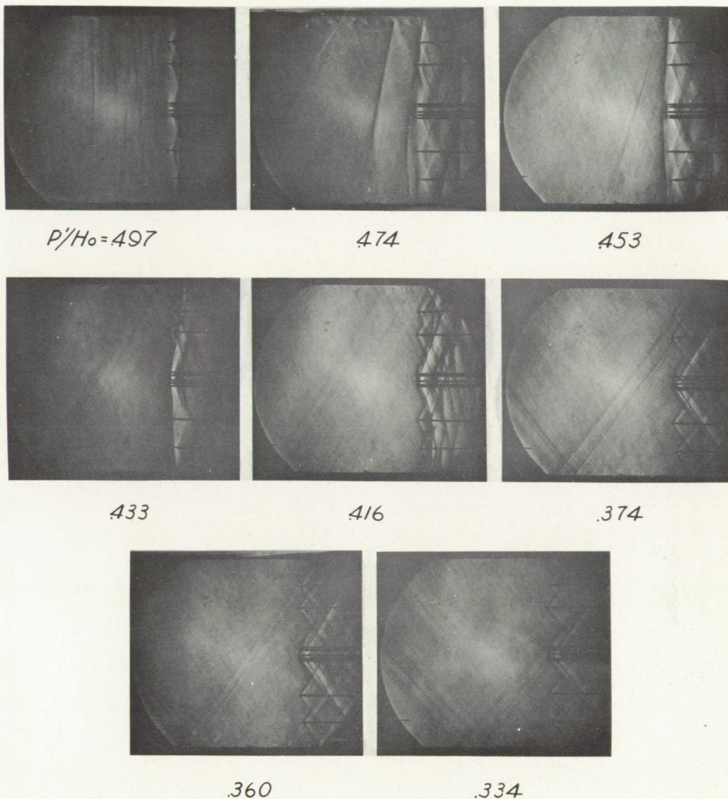
(a) Schlieren photographs. Slotted wall at top. L-59008
