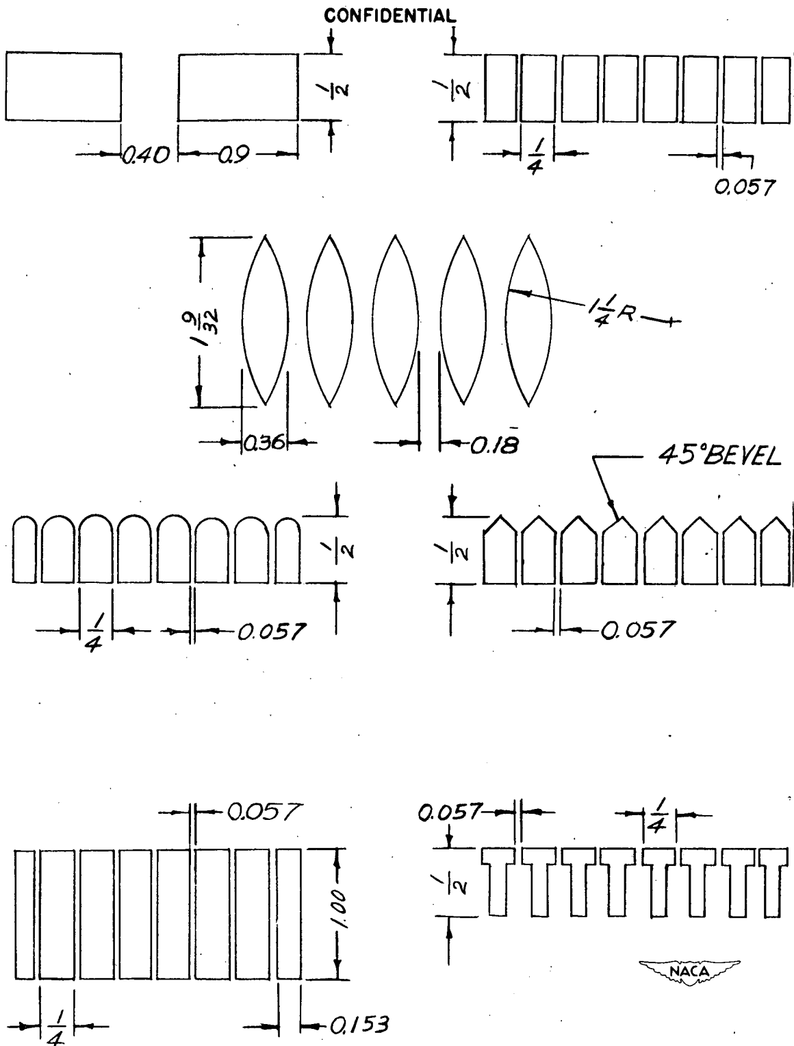
(b) Slot profiles.
