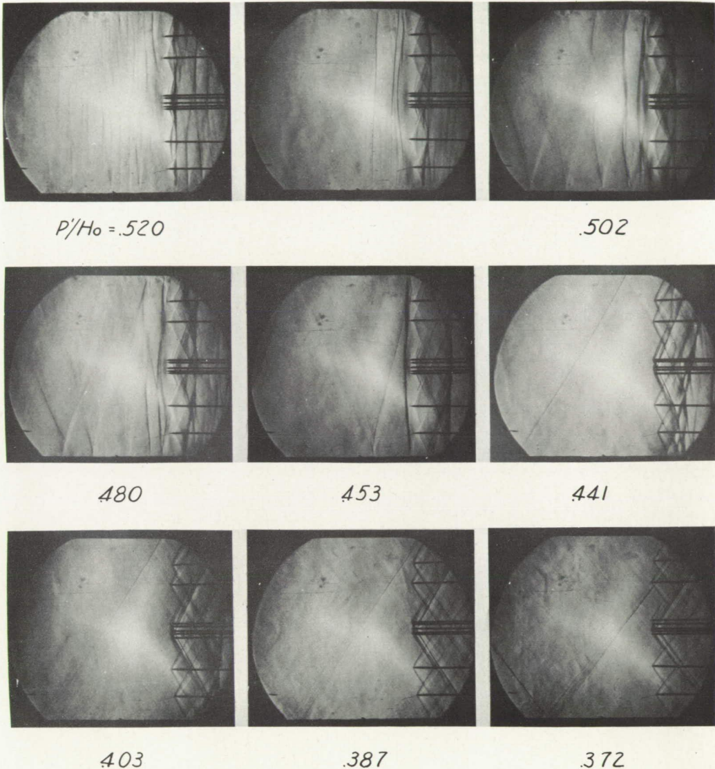
(a) Schlieren photographs. Slotted wall at top. L-59014
