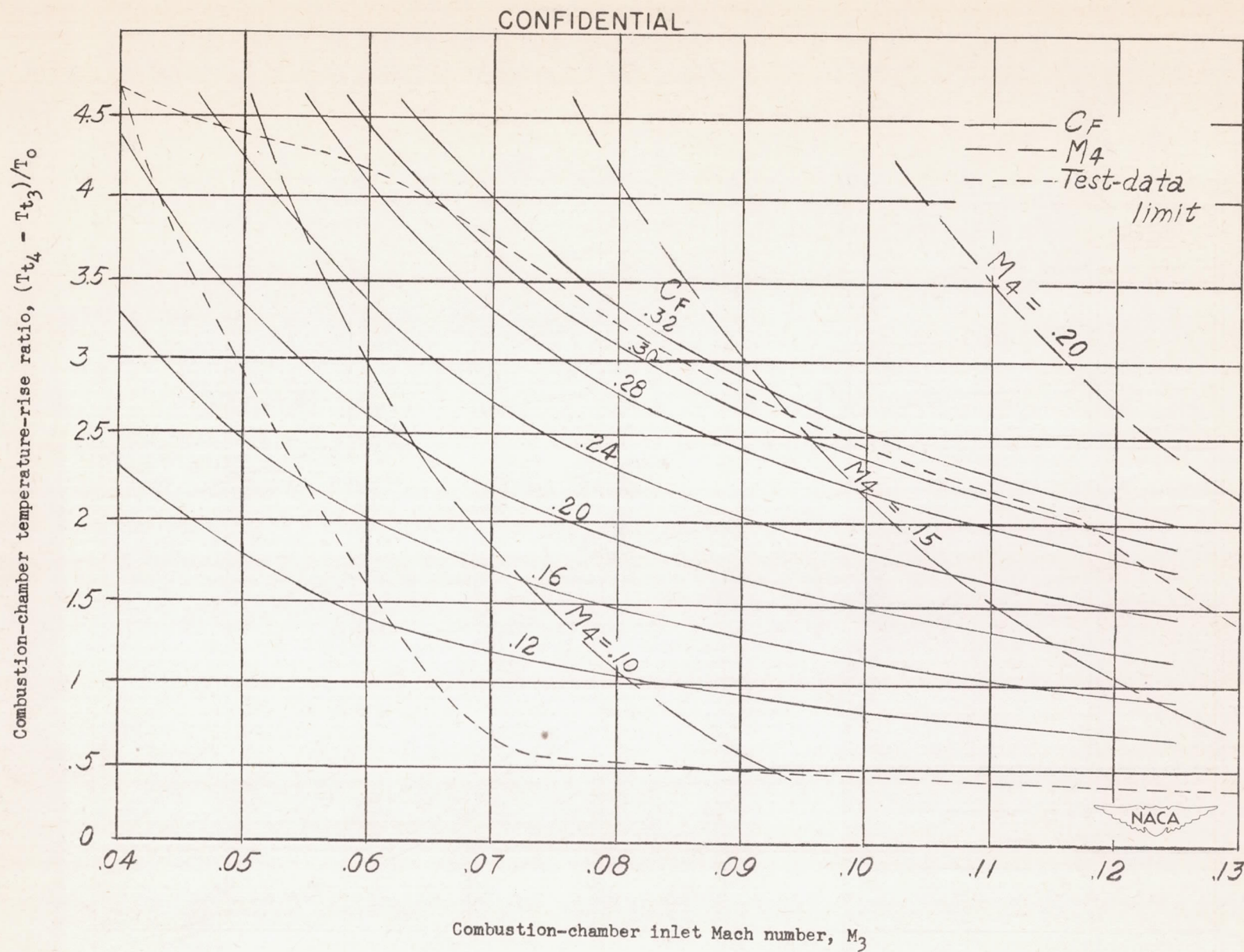
Figure 27.— Calculated thrust coefficient. M_0 = 2.0 ; \frac{P_{t3}}{P_{t0}} = 1.0 . CONFIDENTIAL
