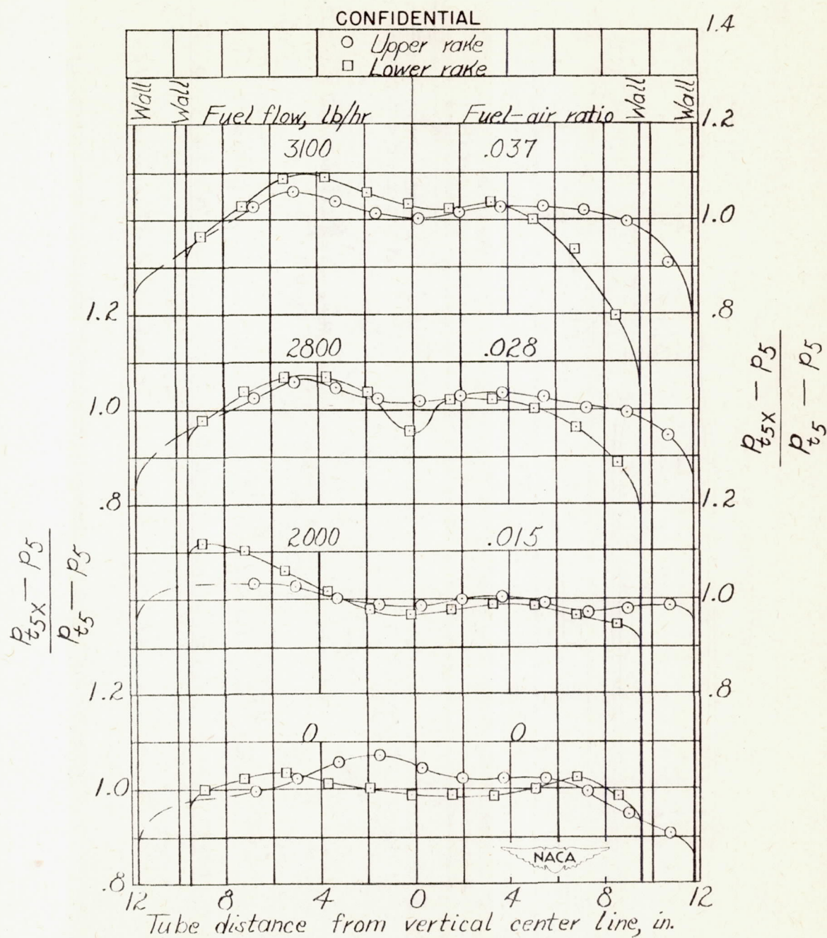
Figure 8.— Horizontal dynamic-pressure gradients from rake readings at station 5. (See fig. 7.)
