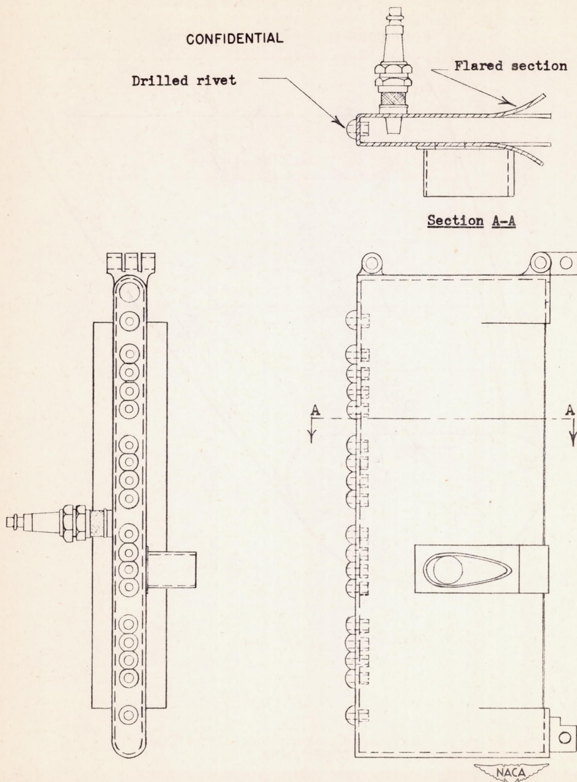
Figure 3.- Modified nonvaporizing pilot-burner housing.
