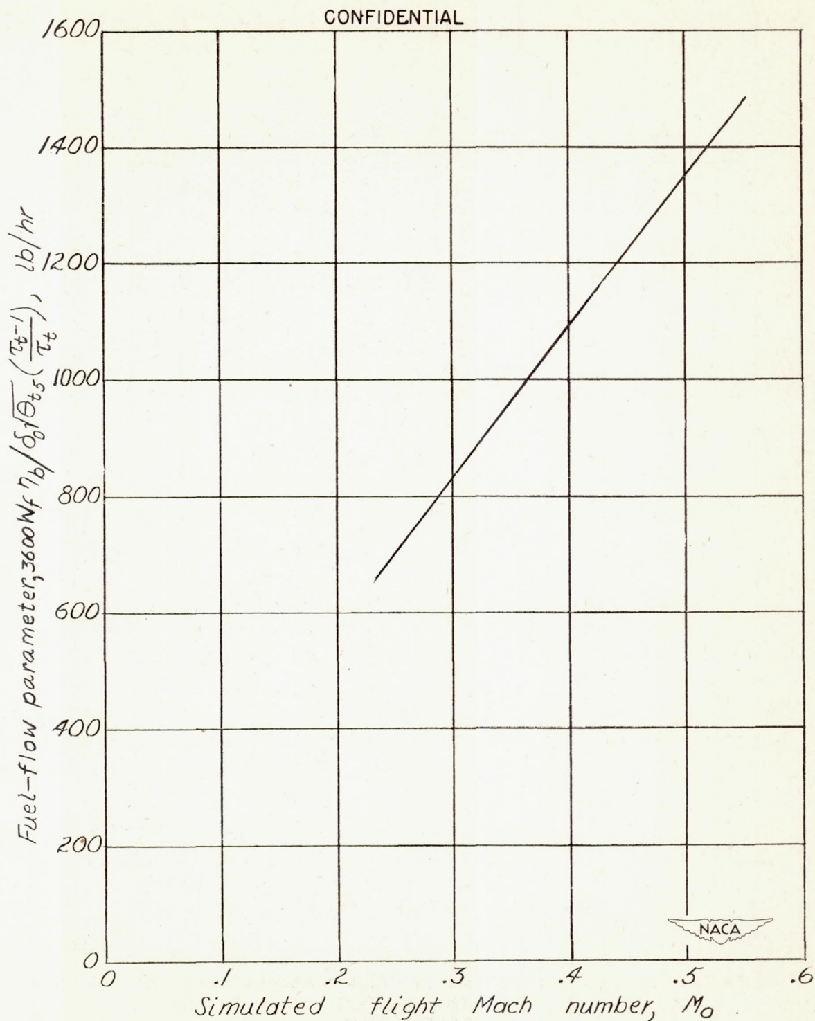
Figure 16.— Variation of fuel-flow parameter with simulated flight Mach number.
