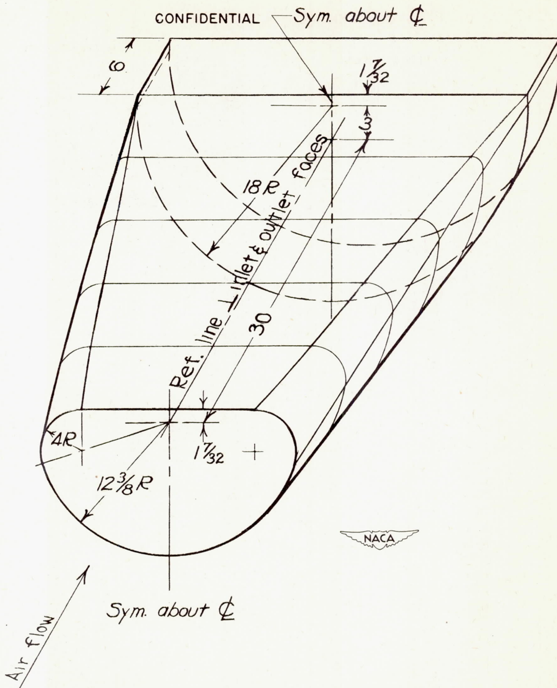
Figure 4.- Diagrammatic sketch of inlet diffuser.
