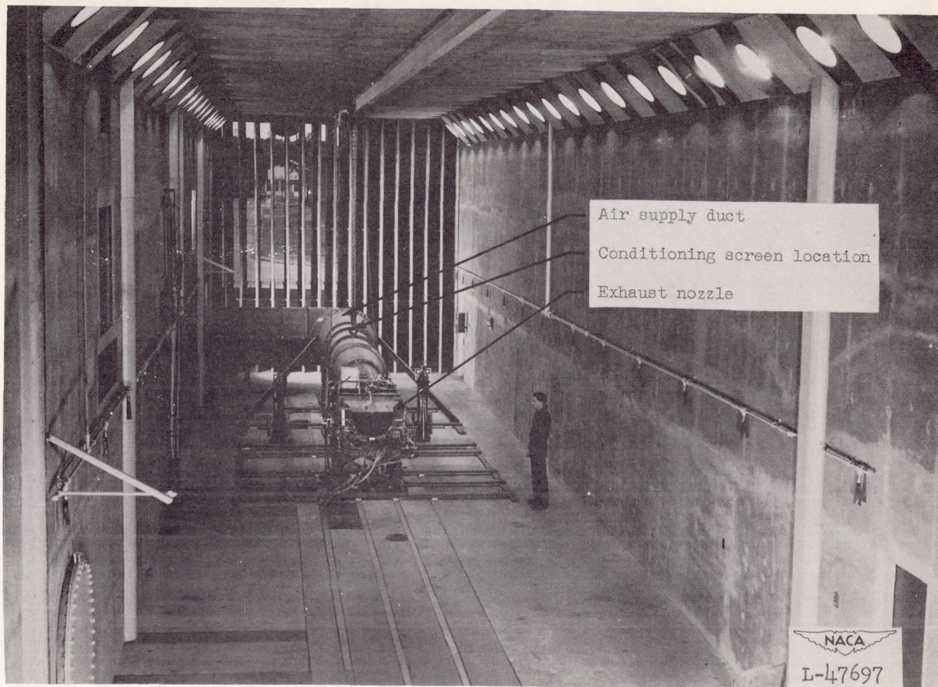
Figure 6.- View from test-cell exit of ram-jet test installation.
