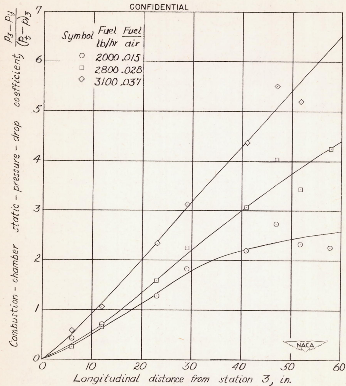
Figure 21.- Combustion-chamber longitudinal-wall static-pressure variations. CONFIDENTIAL
