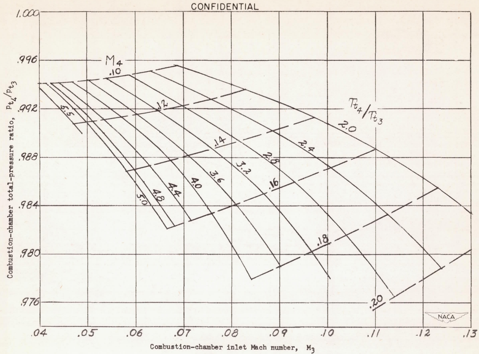
Figure 23.- Test combustion-chamber characteristics.
