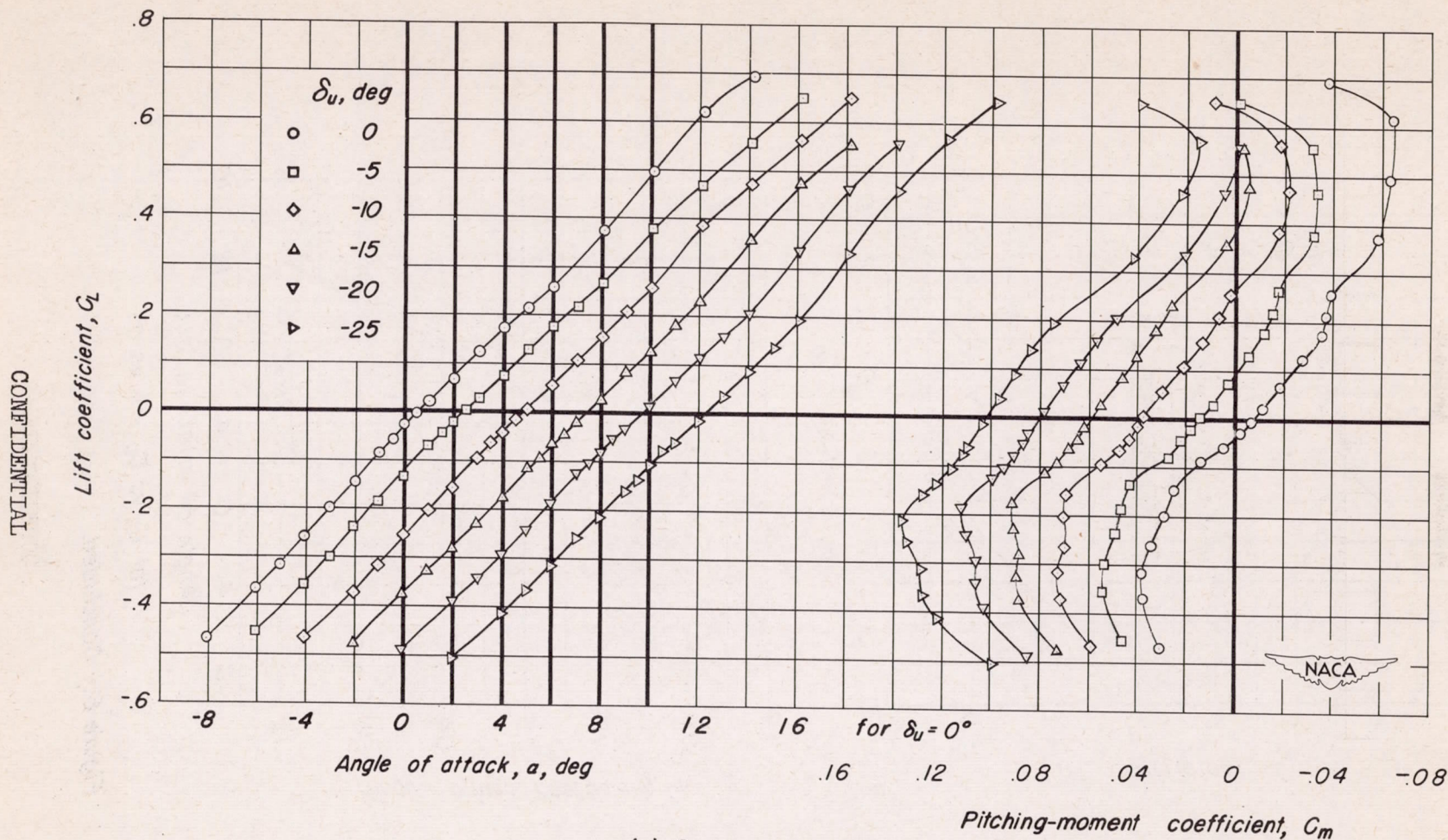
Figure 6.- The effect of elevon deflection on the aerodynamic characteristics of the wing-fuselage combination and on the elevon hinge-moment coefficients at a Mach number of 0.80.
