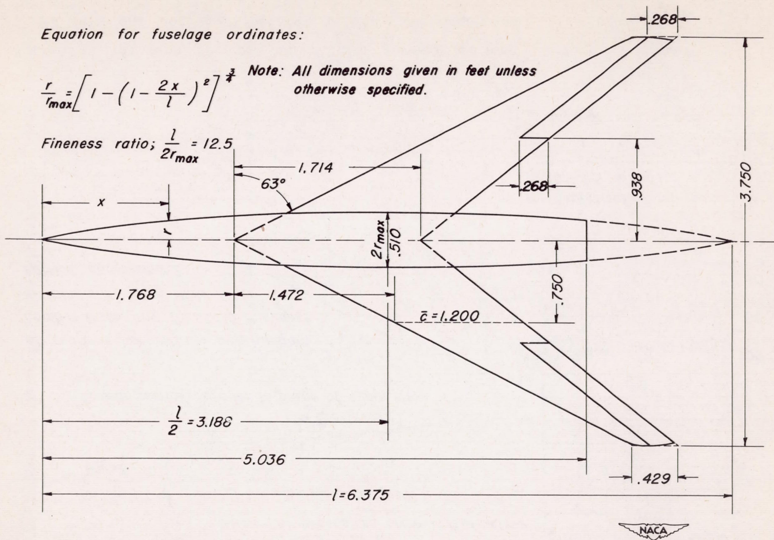
Figure 2.— Dimensions of wing and fuselage.
