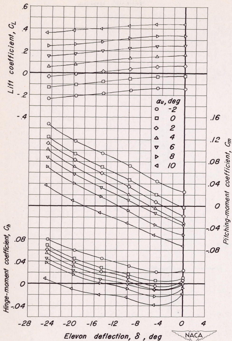
Figure 9. - The variation of lift, pitching-moment, and hinge-moment coefficients with elevon deflection for various angles of attack at several Mach numbers.
