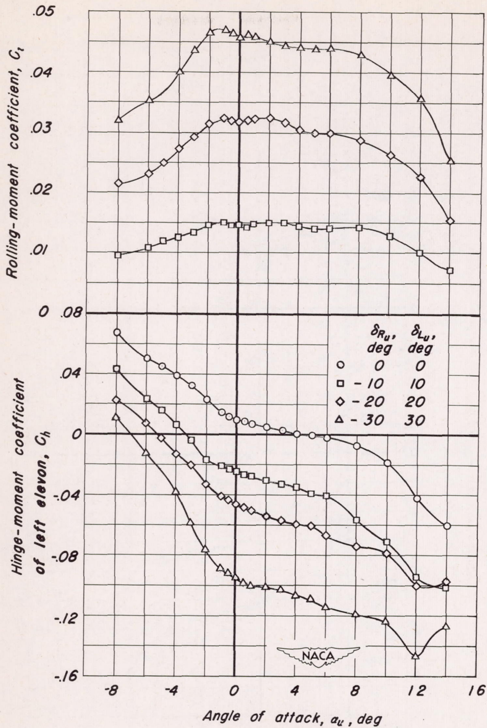
Figure 12.- The variation of rolling-moment and hinge-moment coefficients with angle of attack for various elevon deflections at several Mach numbers.
