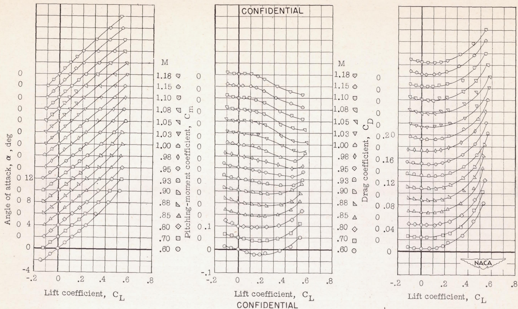
Figure 8.— Aerodynamic characteristics for a model with 45° sweptback wing, aspect ratio 6, taper ratio 0.6, and NACA 65A006 airfoil section. Wing alone.
