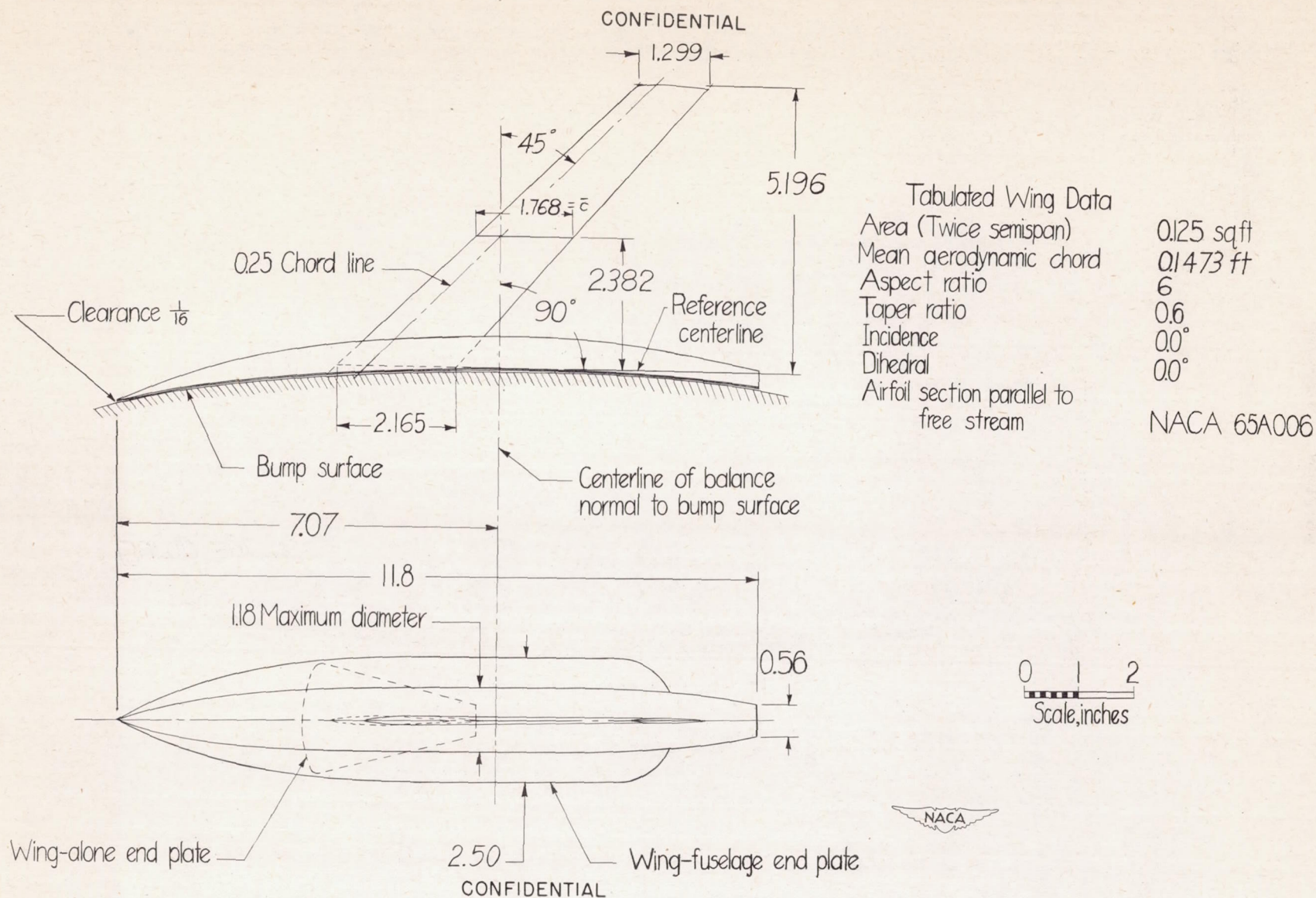
Figure 1.— General arrangement of a model with 45° sweptback wing, aspect ratio 6, taper ratio 0.6, and NACA 65A006 airfoil section.
