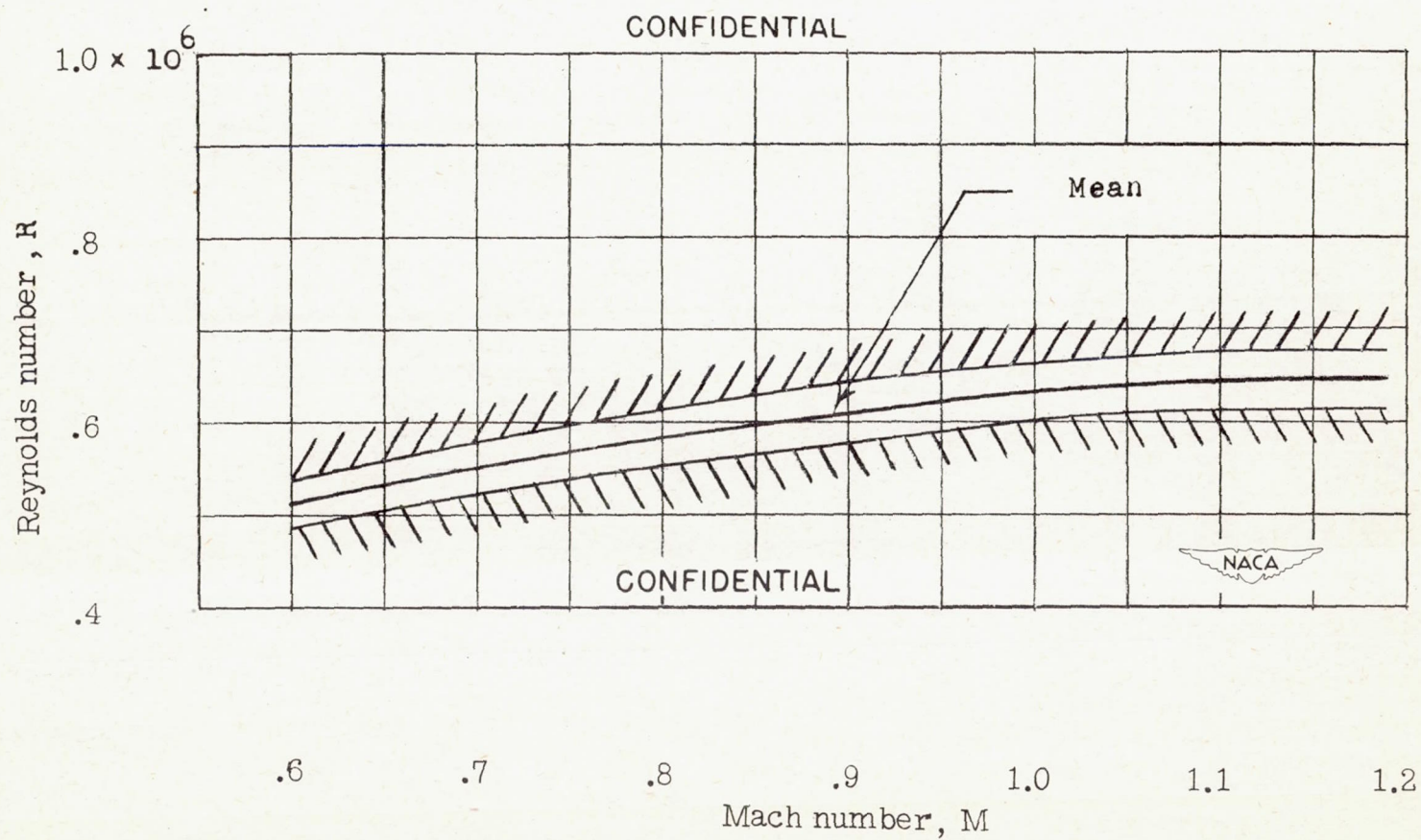
Figure 7.— Variation of test Reynolds number with Mach number for a model with 45^\circ sweptback wing, aspect ratio 6, taper ratio 0.6, and NACA 65A006 airfoil section.
