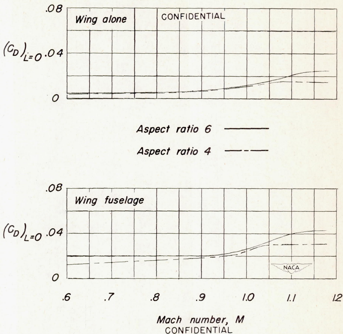
Figure 15.— Effect of aspect ratio on the minimum drag characteristics obtained from tests using a sponge-wiper seal for wings with 45^\circ sweepback, taper ratio 0.6, and NACA 65A006 airfoil section.
