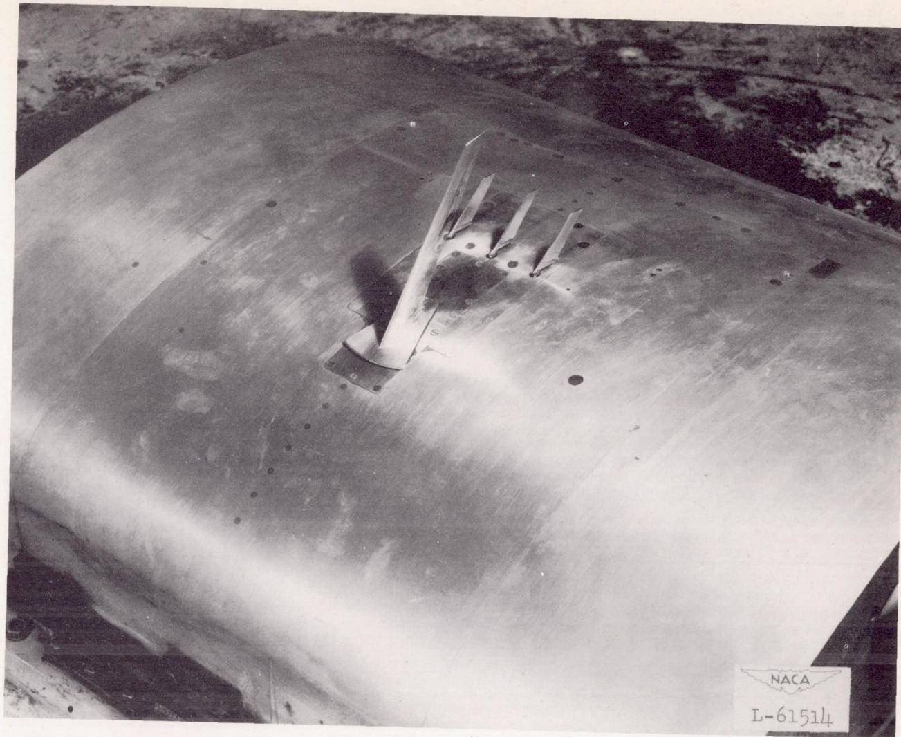
Figure 4.— Photograph of a model with 45^\circ sweptback wing, aspect ratio 6, taper ratio 0.6, and NACA 65A006 airfoil mounted on the bump.
