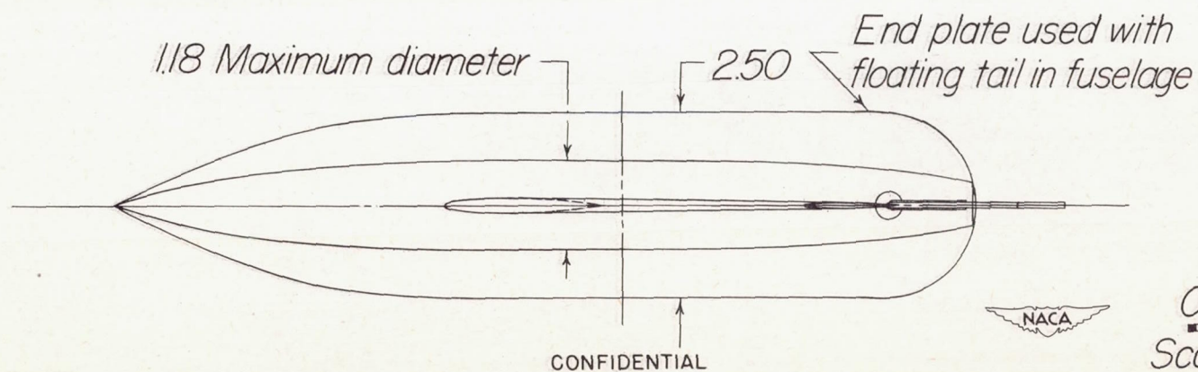
Figure 2.- Details of free-floating tail mounted in fuselage of a model with 45° sweptback wing, aspect ratio 6, taper ratio 0.6, and NACA 65A006 airfoil section.
