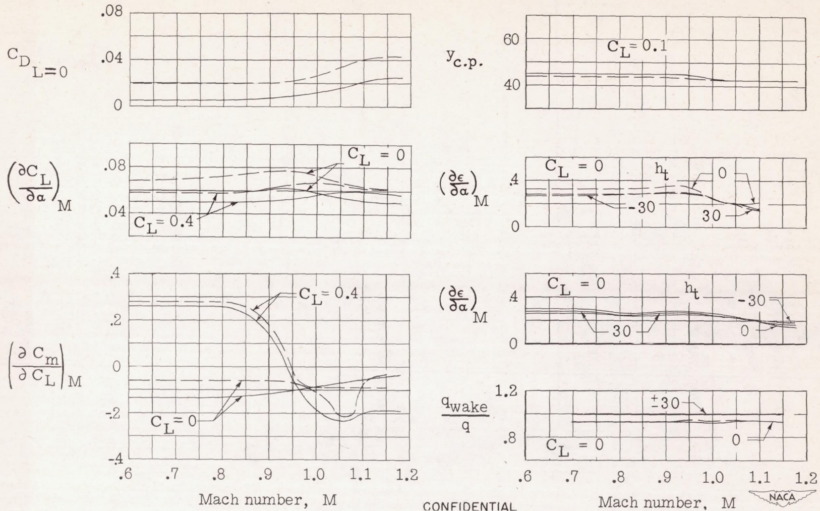
Figure 14.— Summary of aerodynamic characteristics for a model with 45° sweptback wing, aspect ratio 6, taper ratio 0.6, and NACA 65A006 airfoil section.
