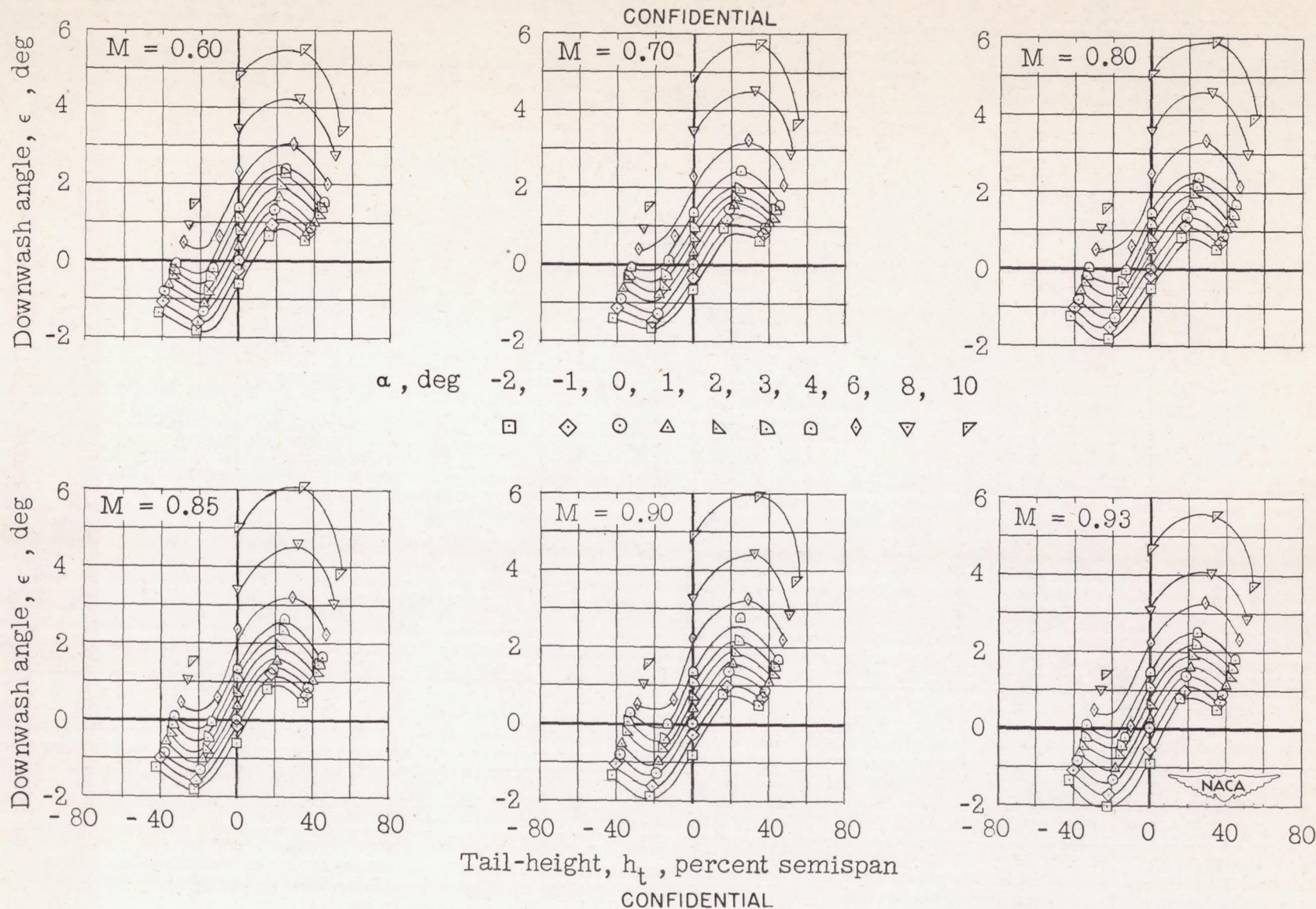
Figure 11.— Effective downwash angles in region of tail plane for a model with 45^\circ sweptback wing, aspect ratio 6, taper ratio 0.6, and NACA 65A006 airfoil section. Wing fuselage.
