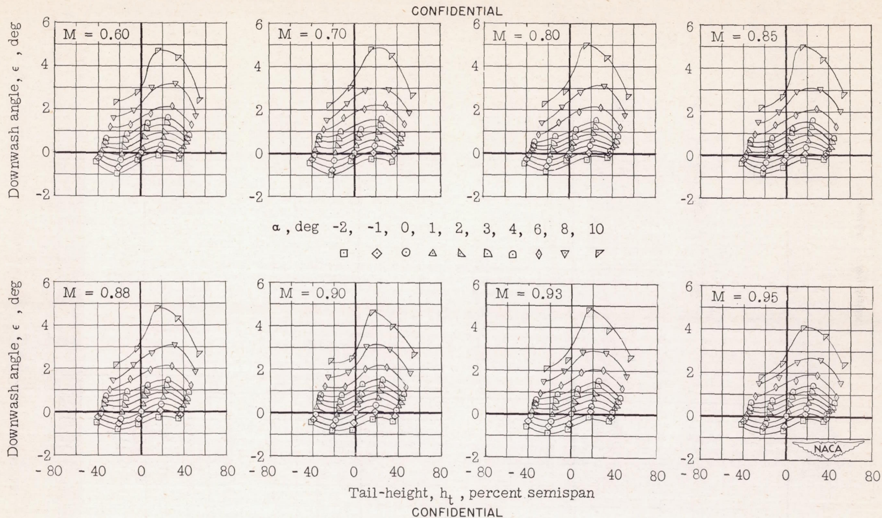
Figure 10.— Effective downwash angles in region of tail plane for a model with 45^\circ sweptback wing, aspect ratio 6, taper ratio 0.6, and NACA 65A006 airfoil section. Wing alone.
