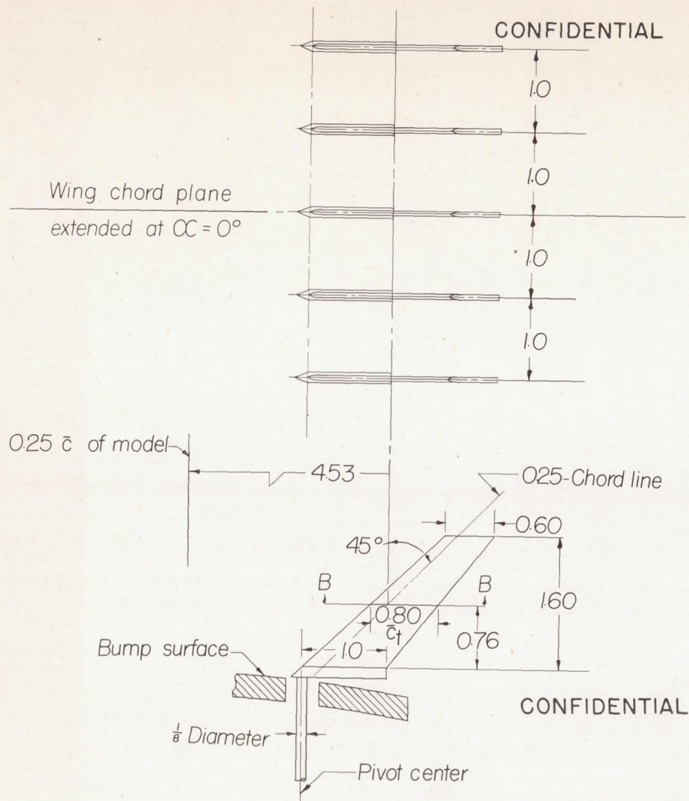
Figure 3.— Details of free-floating tails used in surveys behind model with 45^\circ sweptback wing, aspect ratio 6, taper ratio 0.6, and NACA 65A006 airfoil section.
