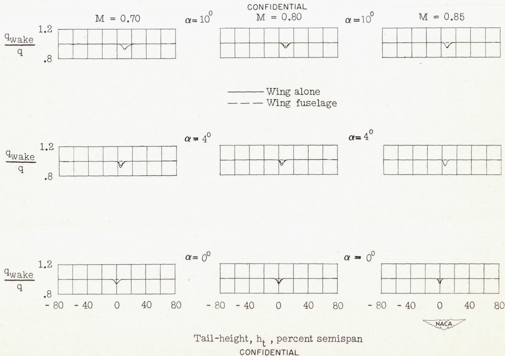
Figure 13.— Dynamic-pressure surveys in region of tail plane for a model with 45^\circ sweptback wing, aspect ratio 6, taper ratio 0.6, and NACA 65A006 airfoil section.
