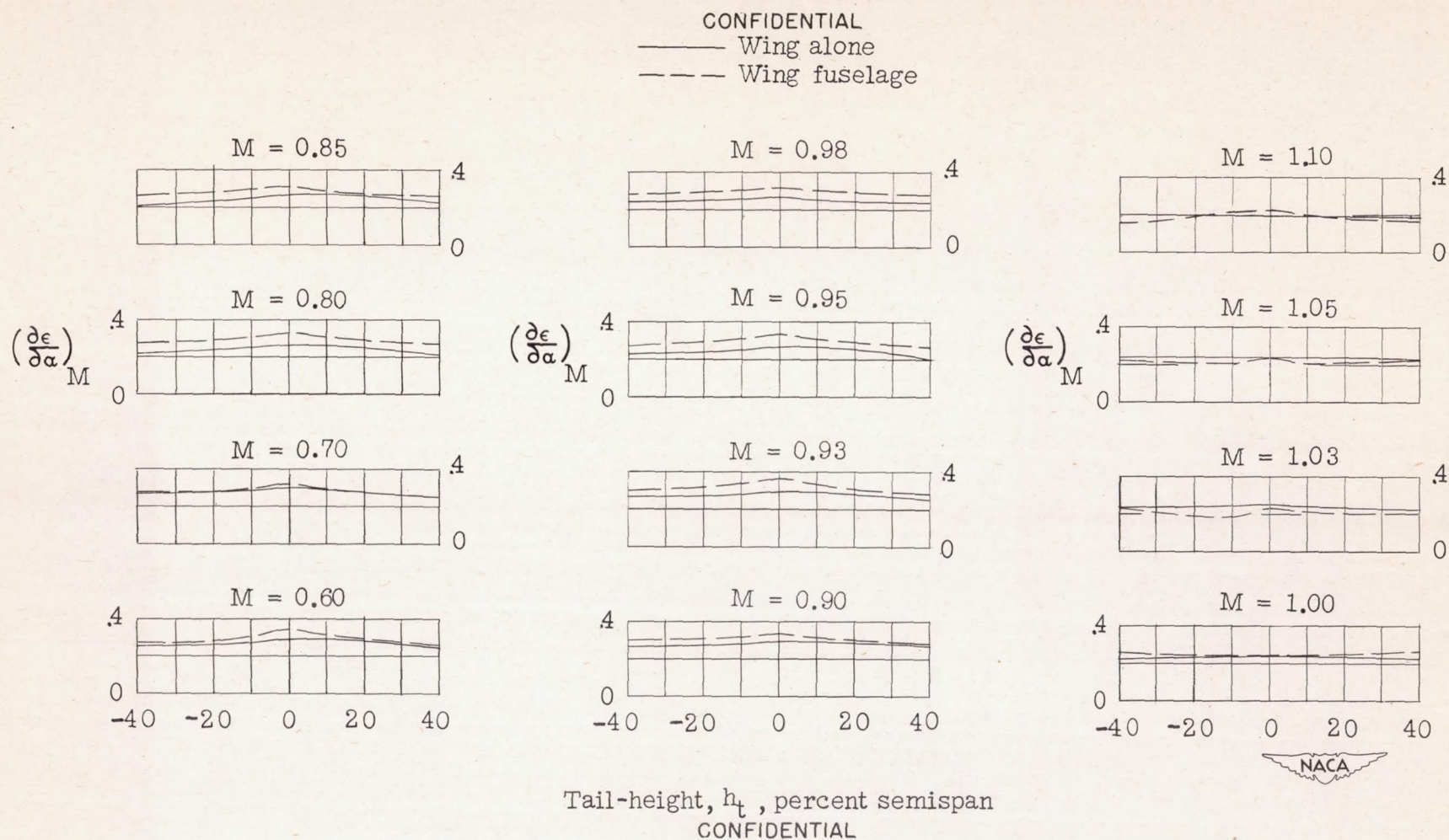
Figure 12.— Variation of downwash gradient with tail height and Mach number for a model with 45^\circ sweptback wing, aspect ratio 6, taper ratio 0.6, and NACA 65A006 airfoil section. C_L = 0 .
