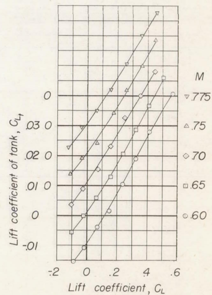
(c) A_{t/A_i} = 0.232 .
