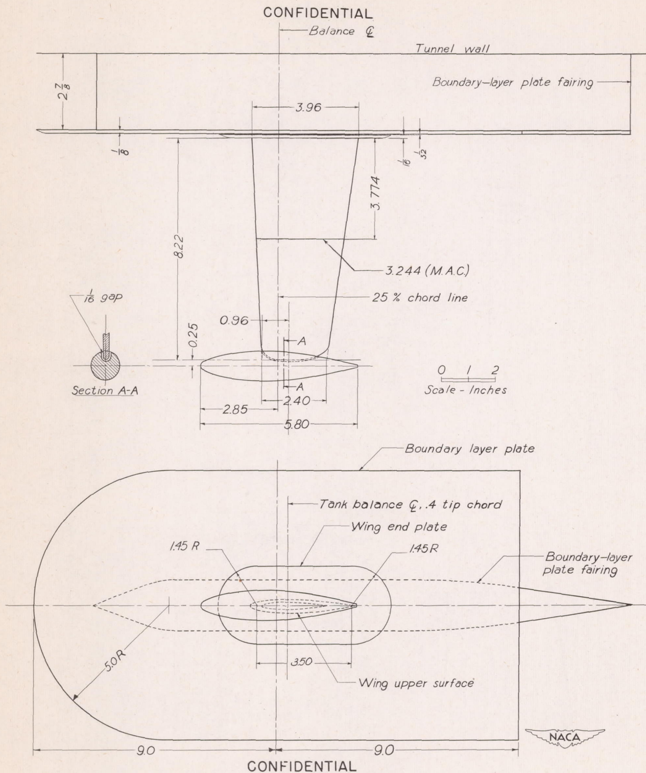
Figure 1 - Drawing of test models with tip tank attached.
