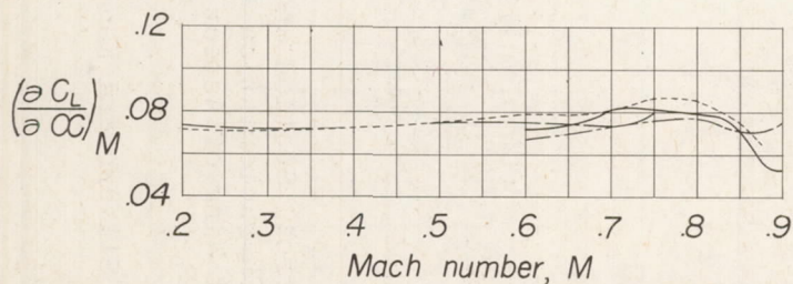
(a) Effect of trailing edge modifications.
