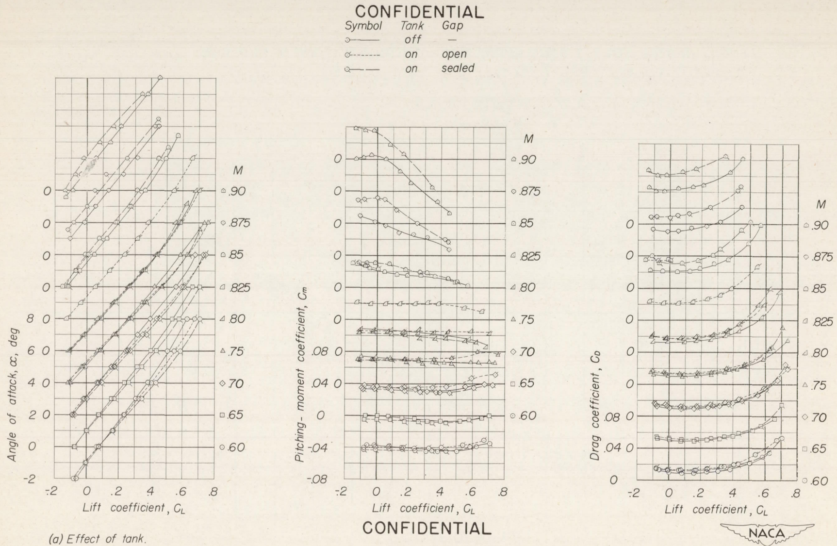
Figure 6.—Effect of a tip-mounted auxiliary fuel tank installation on the aerodynamic characteristics of the wing with section A.
