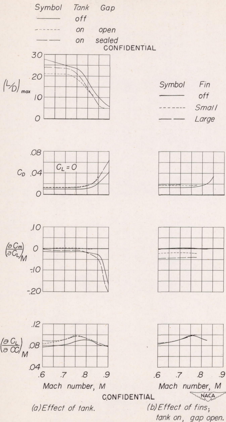
Figure 11.—Effect of Mach number on the aerodynamic characteristics of the wing with section A and a tip-mounted auxiliary fuel tank installation.
