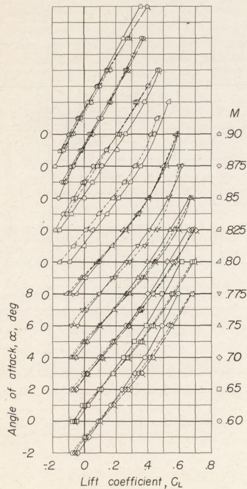
(a) Effect of tank.
