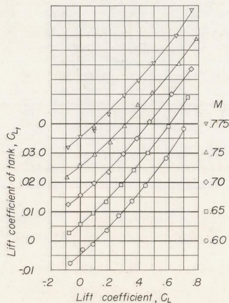
(b) A_{t/A_i} = 0.675 .
