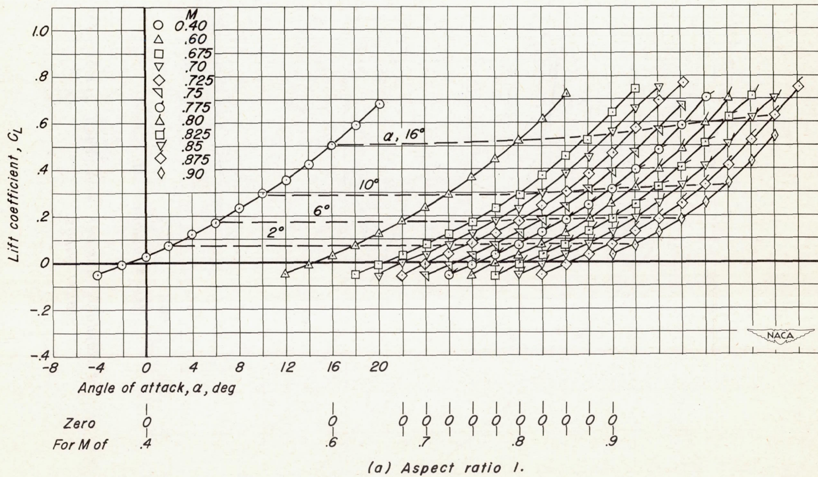
Figure 4.— Variation of lift coefficient with angle of attack.
