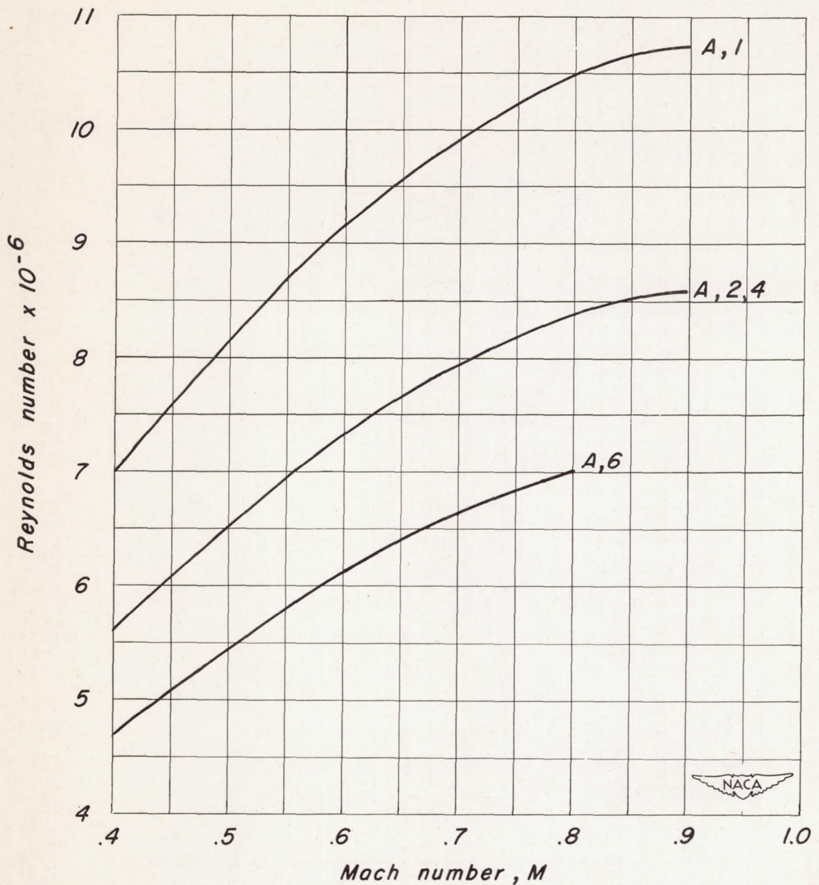
Figure 3.—Variation of Reynolds number with Mach number for the model wings.
