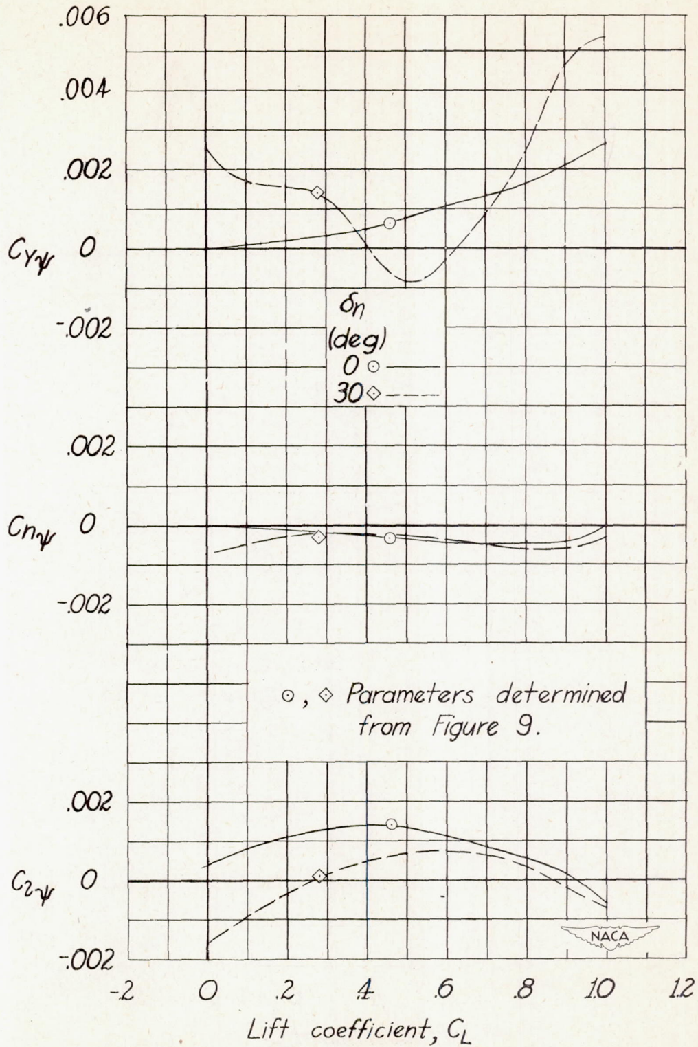
Figure 11.— The lateral-stability parameters of a 60° delta wing with full-span beveled leading-edge flaps.
