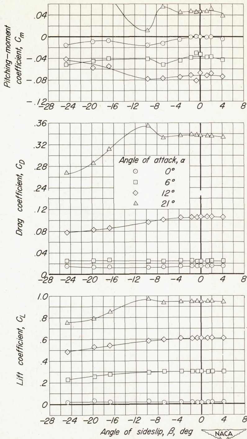
(a) C_m, C_D, C_L vs \beta .
