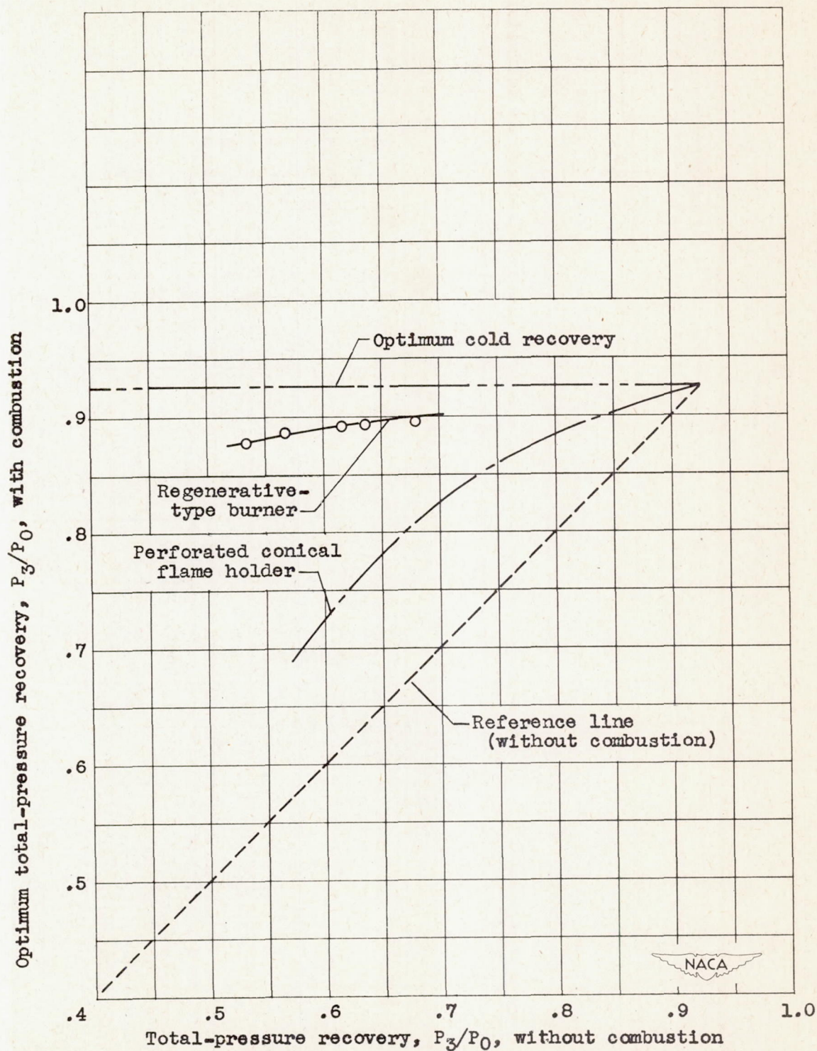
Figure 7. - Comparative diffuser performance with regenerative-type burner and perforated conical flame holder.
