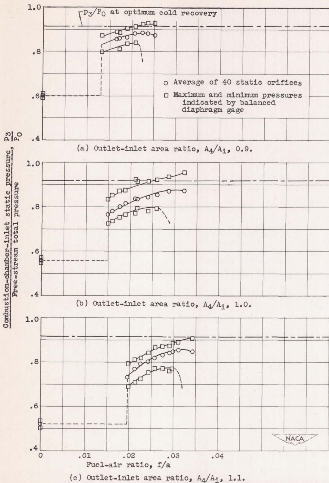
Figure 6. - Effect of fuel-air ratio on combustion-chamber-inlet static pressure. Regenerative-type burner.
