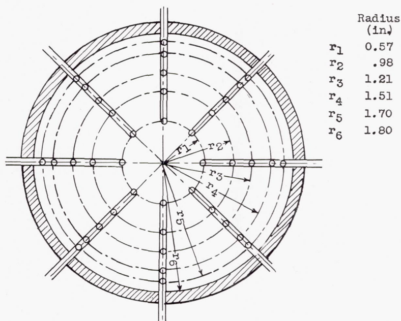
(d) Pitot-static survey rake located at cross section A-A (fig. 1(a)).
