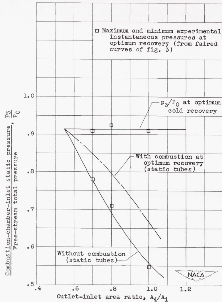
Figure 4. - Variation of maximum and minimum combustion-chamber-inlet static pressures with outlet-inlet area ratio at optimum mean static pressure. Perforated conical flame holder.
