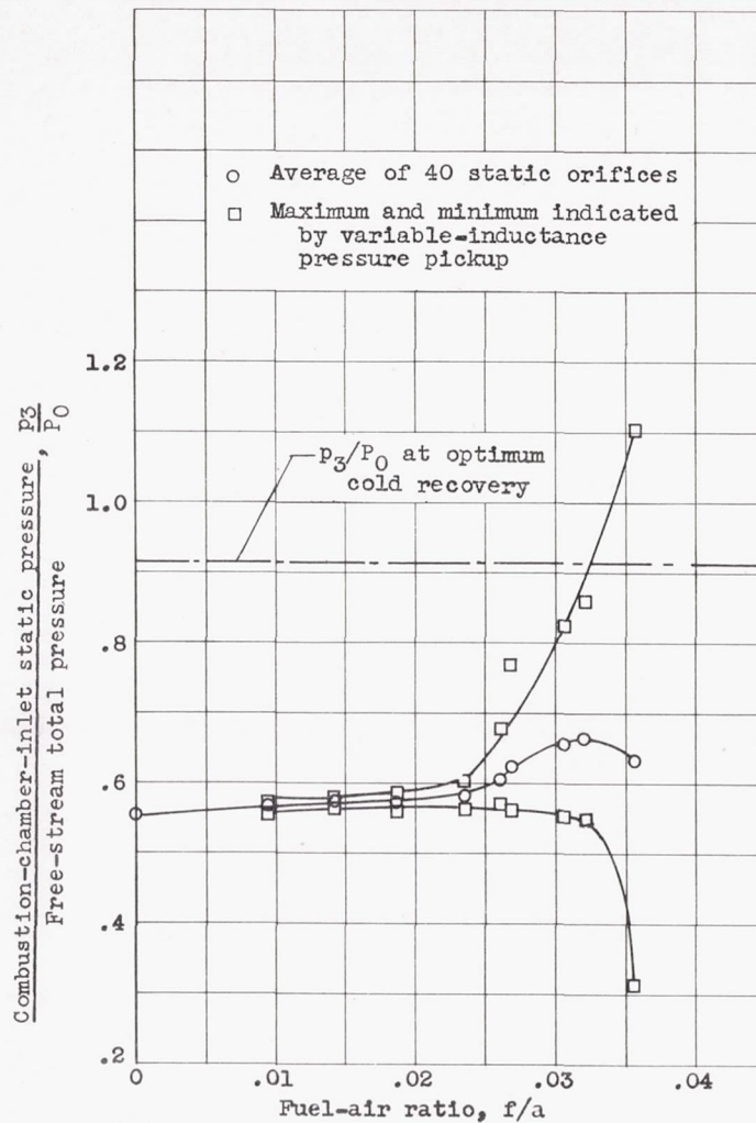
Figure 3. - Concluded. Effect of fuel-air ratio on combustion-chamber-inlet static pressure. Perforated conical flame holder.
