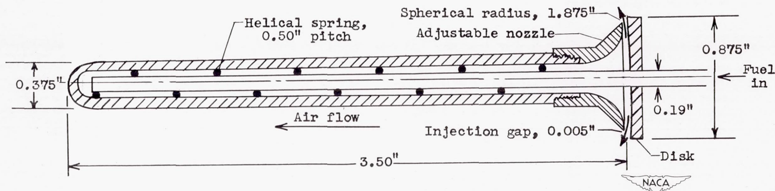
(b) Details of regenerative-type burner.
