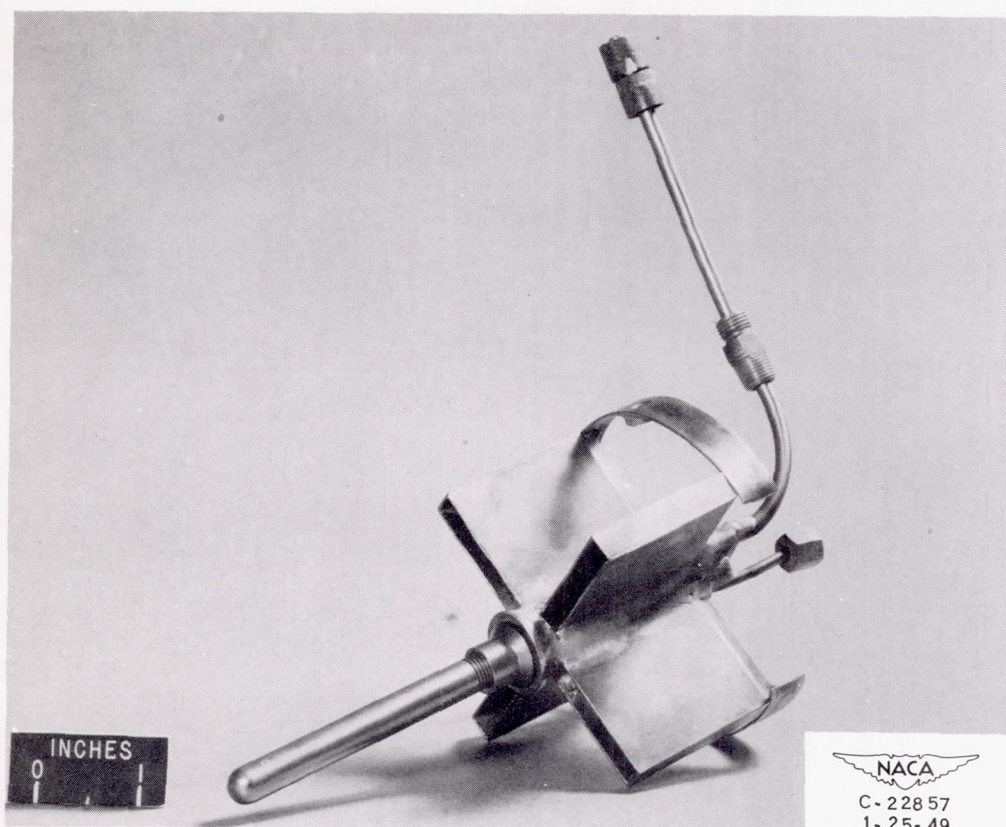
(c) Regenerative burner with acetylene pilot.
