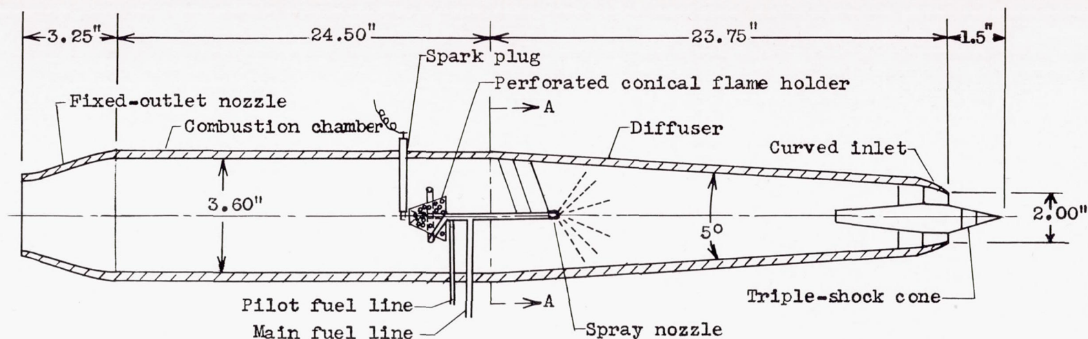
(a) Schematic drawing of combustion model with perforated conical flame holder.
