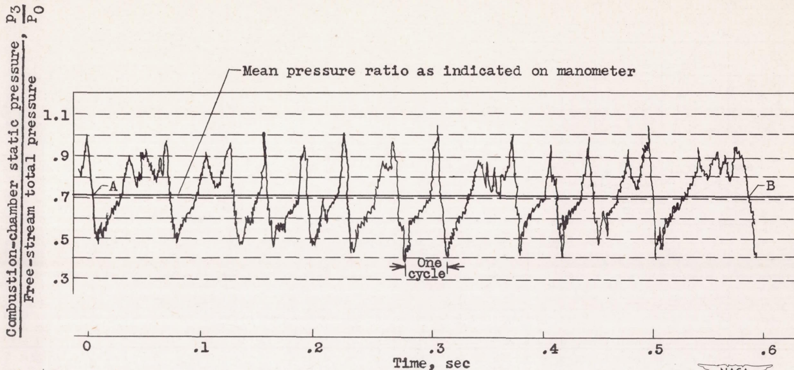
Figure 2. - Typical signal from variable-inductance pressure pickup showing wave form of pressure fluctuations at combustion-chamber inlet when ram jet is operating with shock oscillating in and out of diffuser inlet. Shock diffuser with triple-shock projecting cone; fundamental frequency, approximately 22 cycles per second.
