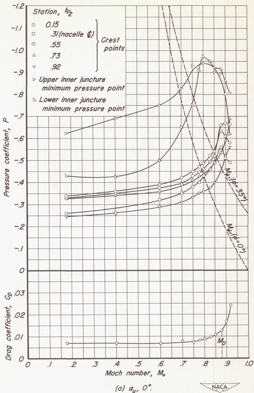
Figure 22.—The variation with Mach number of the drag coefficient and of the pressure coefficients at several points on the wing-nacelle combination.
