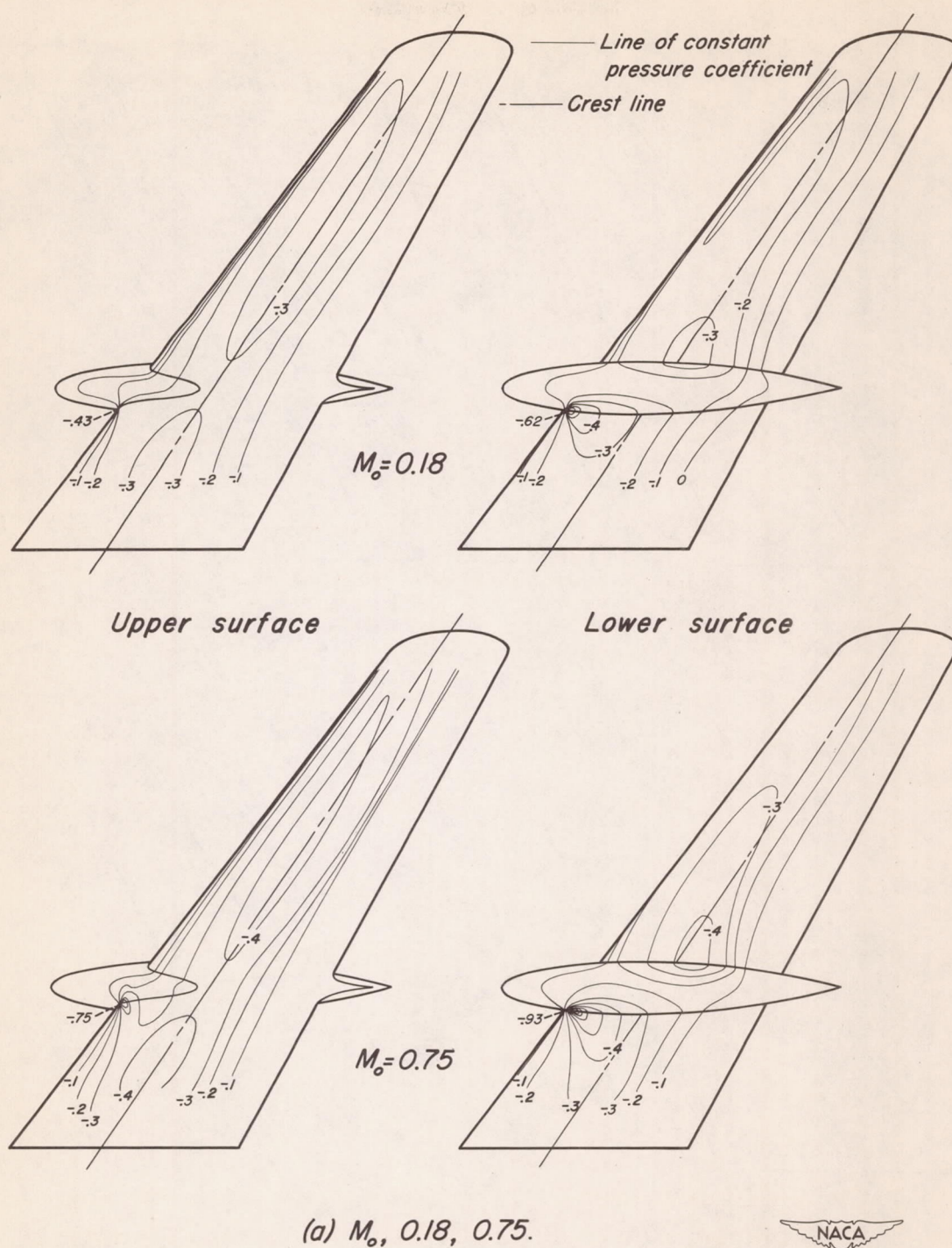
Figure 17.—The lines of constant pressure coefficient on the upper and lower surfaces for several Mach numbers. \alpha_u, 0^\circ ; R_w, 2,000,000 .
