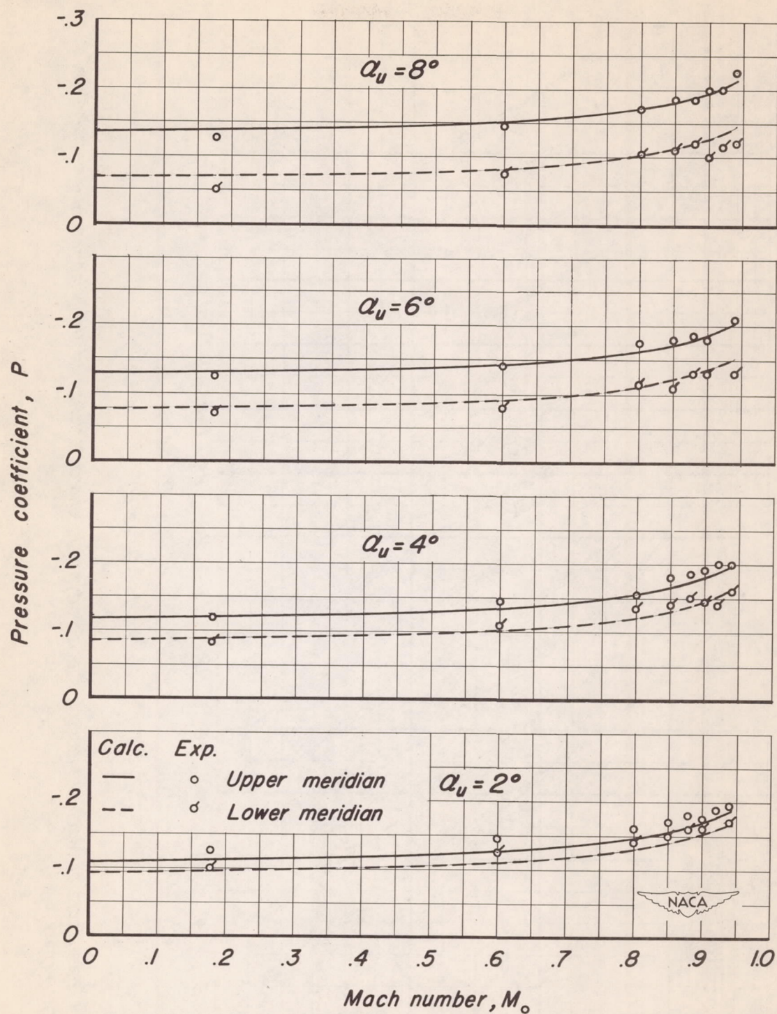
Figure 11.- A comparison of the effect of Mach number on the pressure coefficient on the upper and lower surfaces at 26.9-percent length at several angles of attack with that calculated by linear theory.
