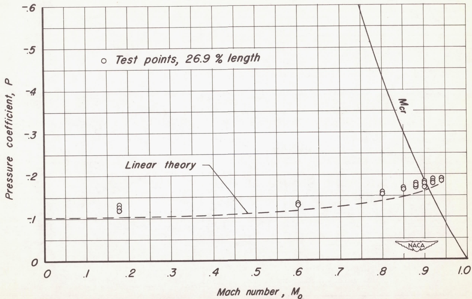
Figure 10.—The effect of Mach number on the pressure coefficients at the minimum-pressure station on the body of revolution. \alpha_u, 0^\circ
