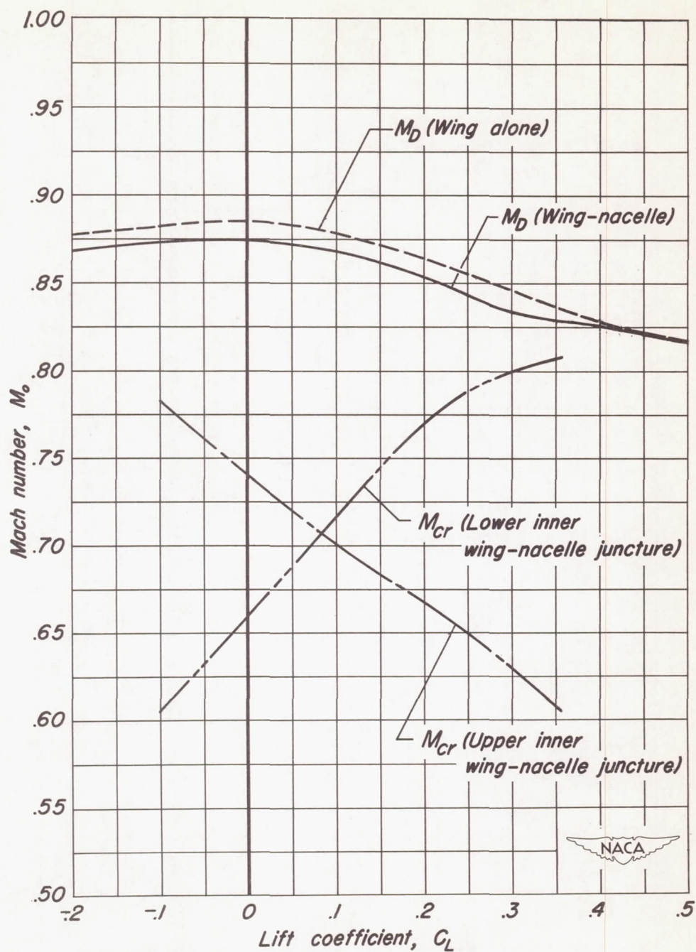
Figure 23.-The variation with lift coefficient of the drag-divergence Mach number and the critical Mach numbers in the wing-nacelle junctures.
