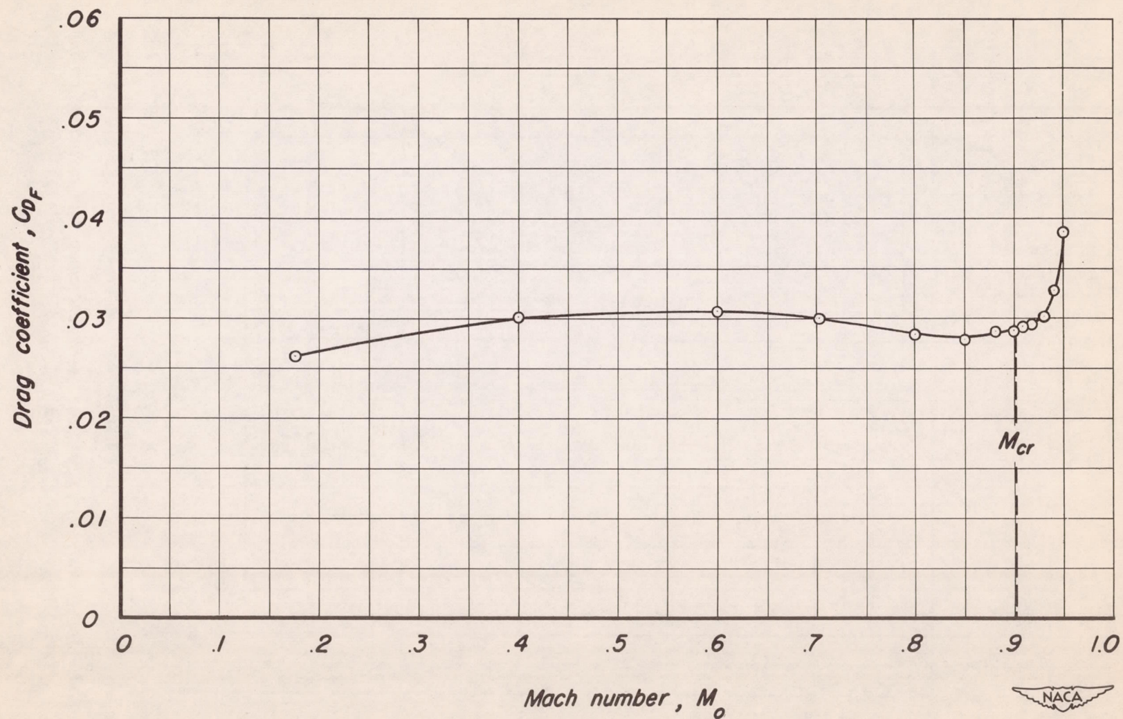
Figure 3.—The variation of drag coefficient with Mach number for the body of revolution at 0^\circ angle of attack. R_b , 3,760,000.
