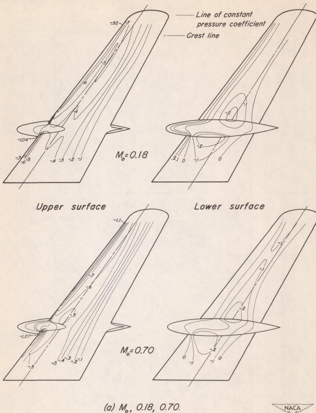
Figure 19.-The lines of constant pressure coefficient on the upper and lower surfaces for several Mach numbers. \alpha_u, 4^\circ ; R_w, 2,000,000.
