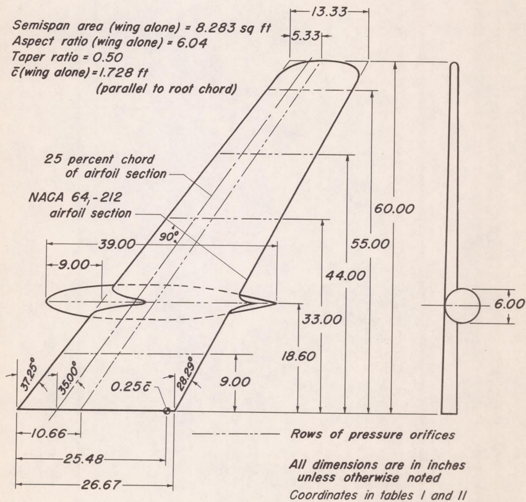
(b) Semispan wing and nacelle.
