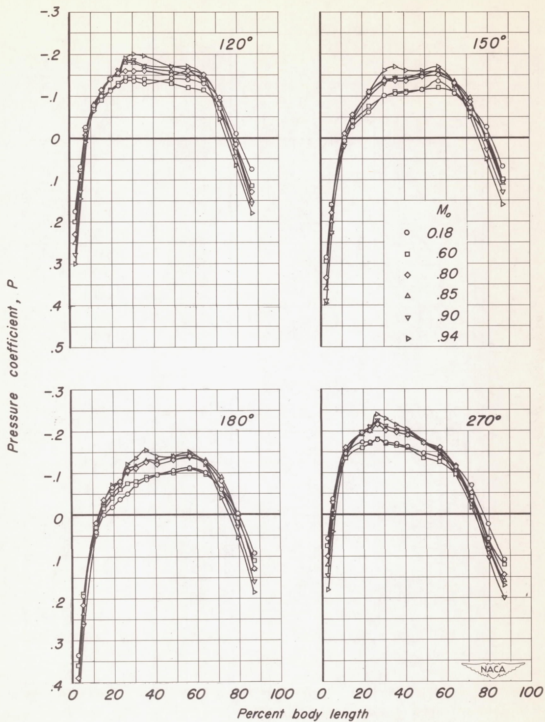
(b) Meridians, 120^\circ , 150^\circ , 180^\circ , 270^\circ
