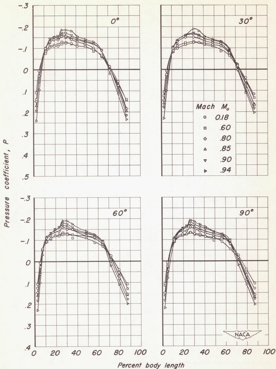
Figure 4.- The distribution of pressure coefficient along four meridians on the body of revolution at several Mach numbers. a_u , 0°.
