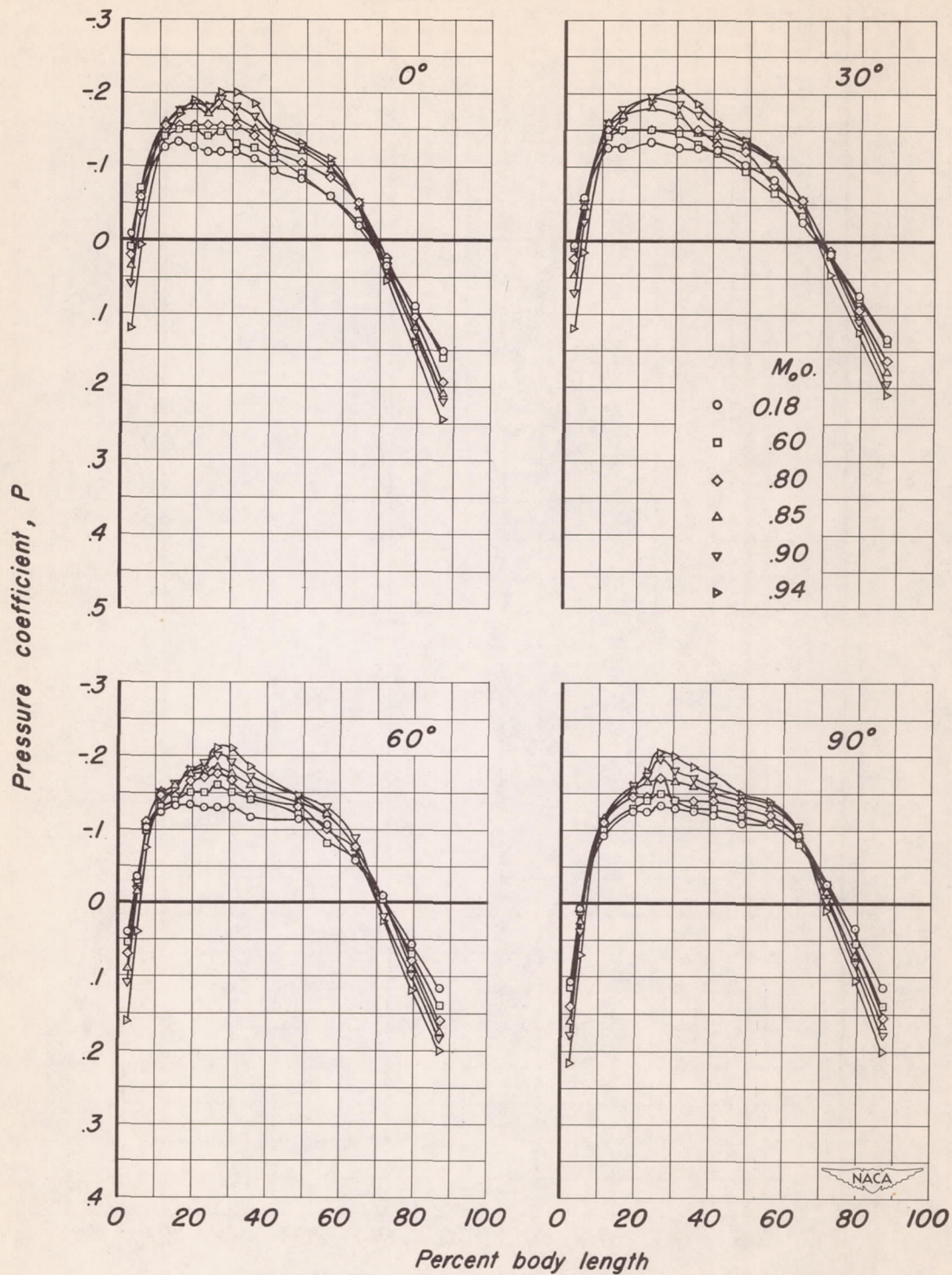
(a) Meridians, 0^\circ , 30^\circ , 60^\circ , 90^\circ .
