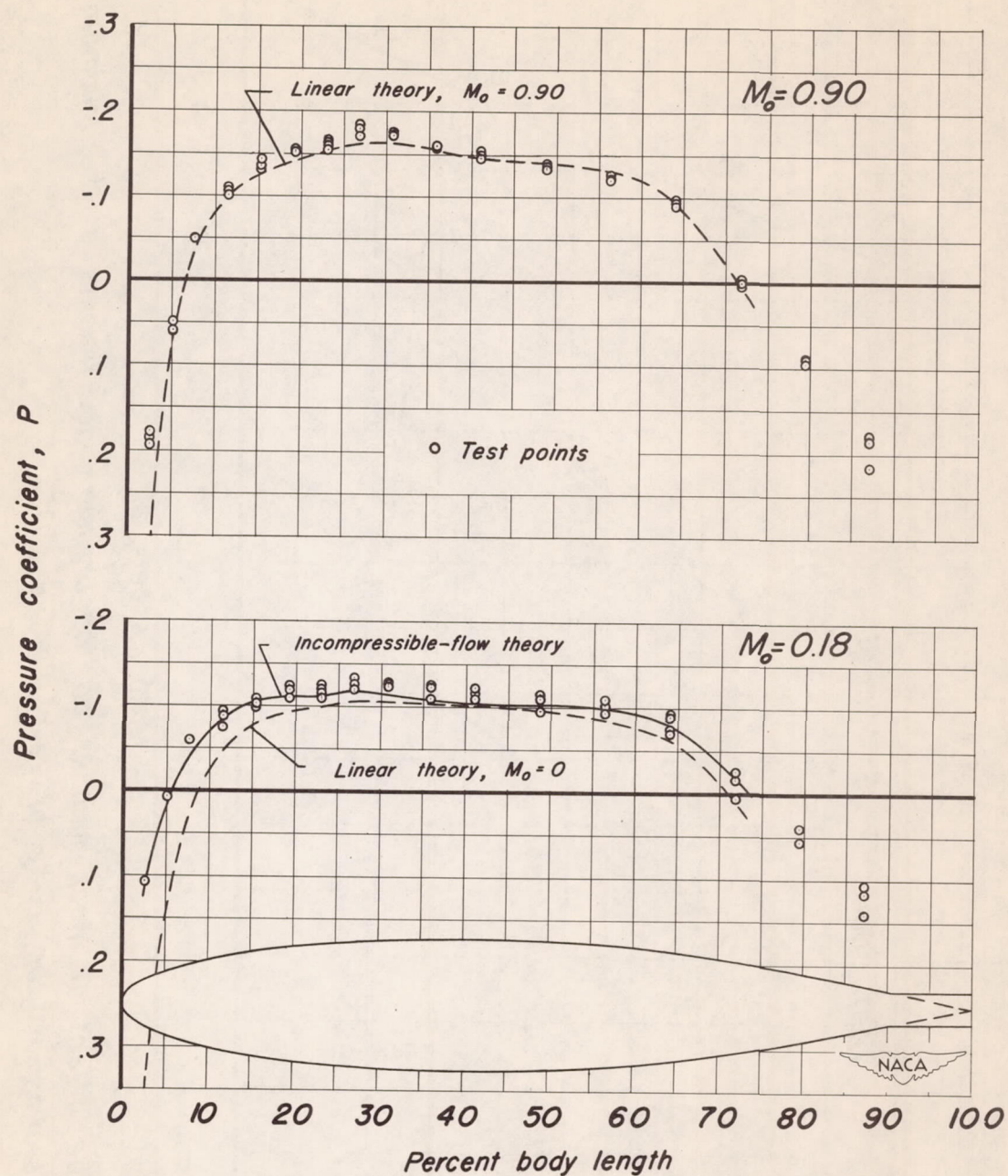
Figure 9.-A comparison of the lengthwise distribution of pressure coefficient obtained experimentally at Mach numbers of 0.18 and 0.90 with that calculated by theory. \alpha_u, 0^\circ .
