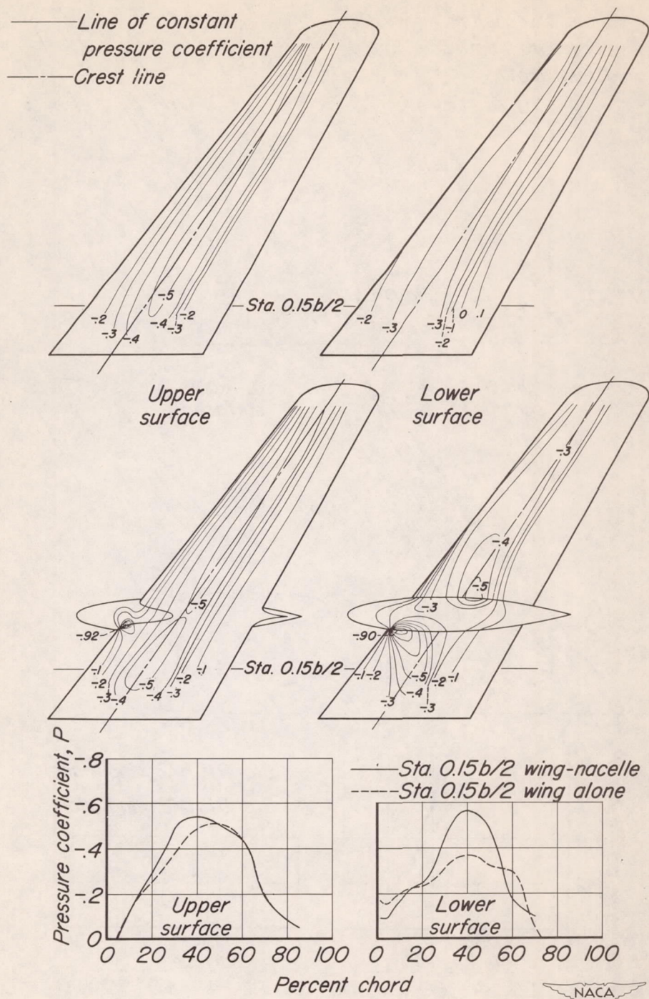
Figure 20.-A comparison of the pressures on the wing alone with those on the wing-nacelle combination. R_w, 2,000,000 .
