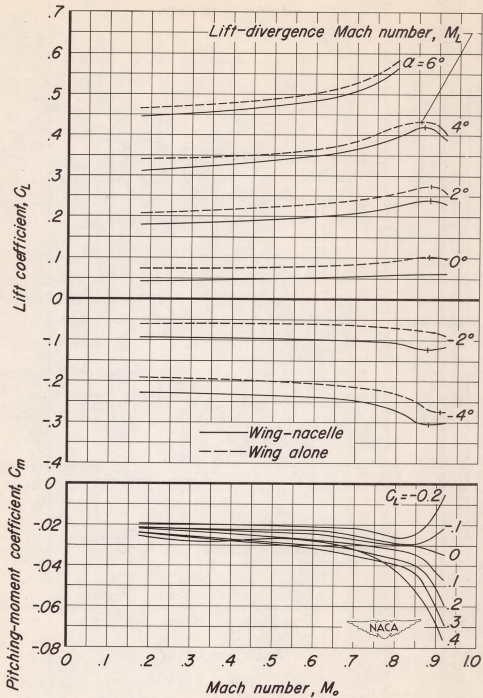
Figure 13.-The variation with Mach number of the lift coefficient at several angles of attack and of the pitching-moment coefficient at several values of lift coefficient.
