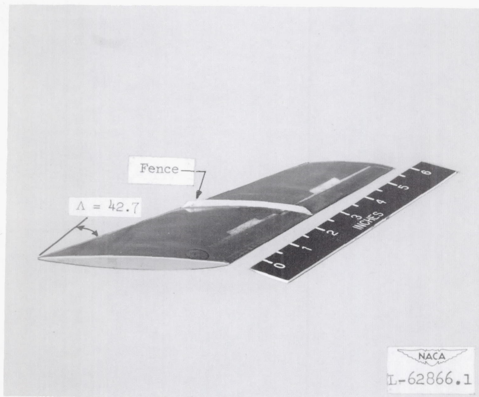
Figure 1.- Photograph of model 4 showing fence installed.
