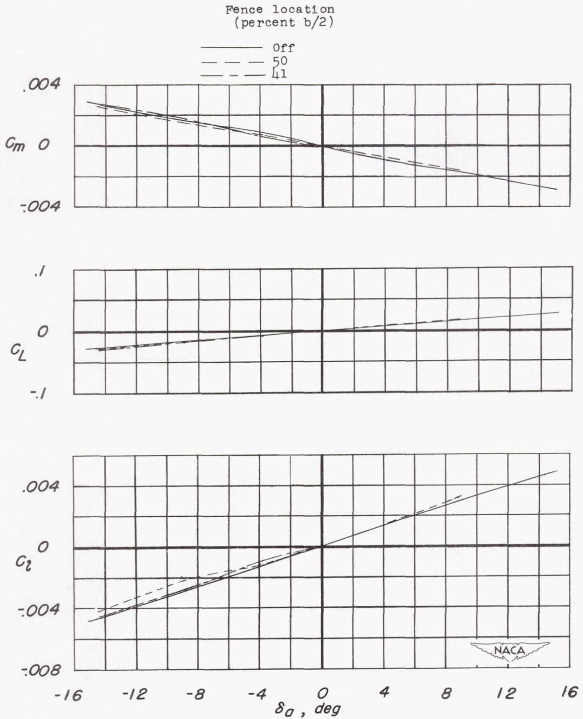
(b) C_m , C_L , and C_l against \delta_a . \alpha = 0 .
