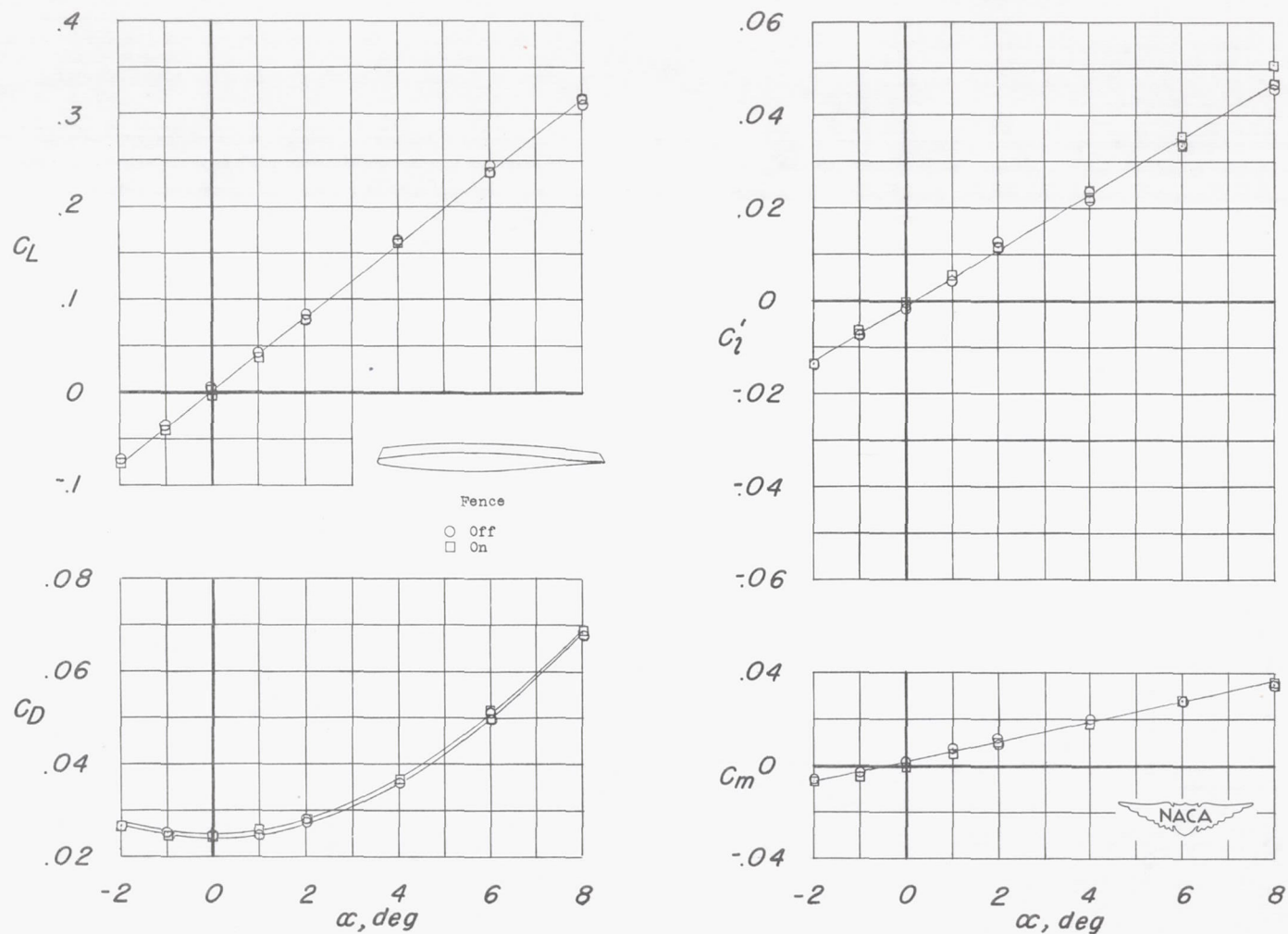
Figure 5.- Effects of a fence on the aerodynamic characteristics of model 3 at a Mach number of 1.9. Leading-edge sweepback = 45^\circ ; aspect ratio = 1.8.
