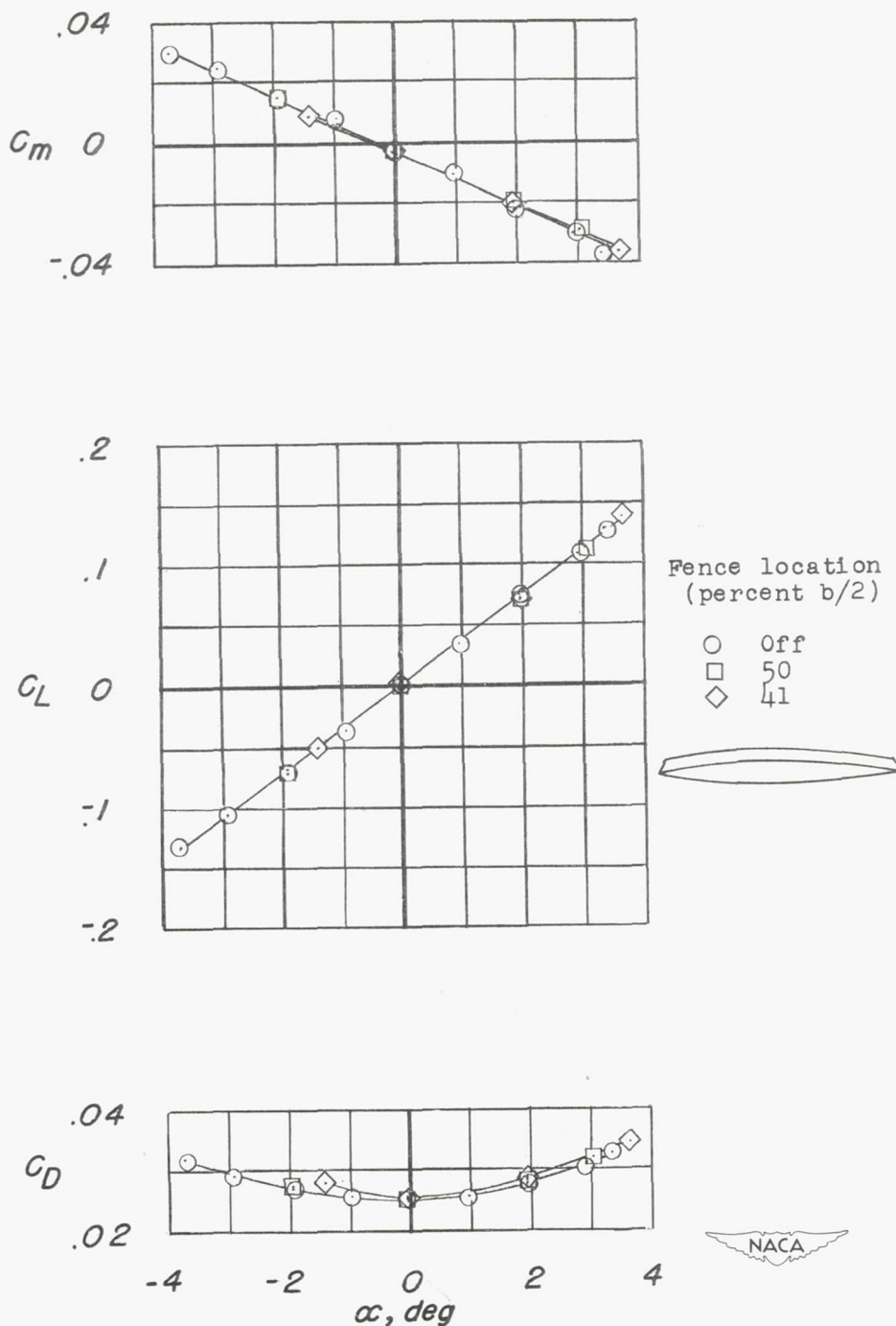
(a) C_m , C_L , and C_D against \alpha . \delta_a = 0 .
