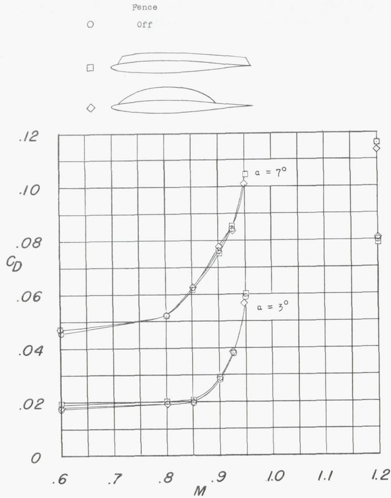
Figure 4.- Effects of fences on the aerodynamic characteristics of model 2 at Mach numbers from 0.6 to 0.95 and 1.2. Leading-edge sweepback = 38.8^\circ ; aspect ratio = 3.6.
