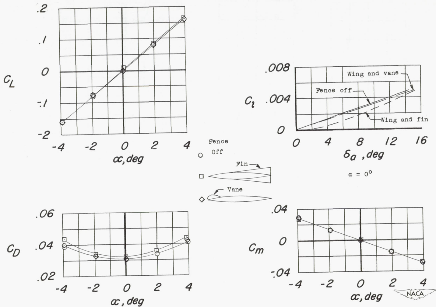
Figure 7.- Effects of a stall-control vane and fin at 50 percent b/2 on the aerodynamic characteristics of model 4 at a Mach number of 1.9; leading-edge sweepback = 42.7^\circ ; aspect ratio = 4.0.
