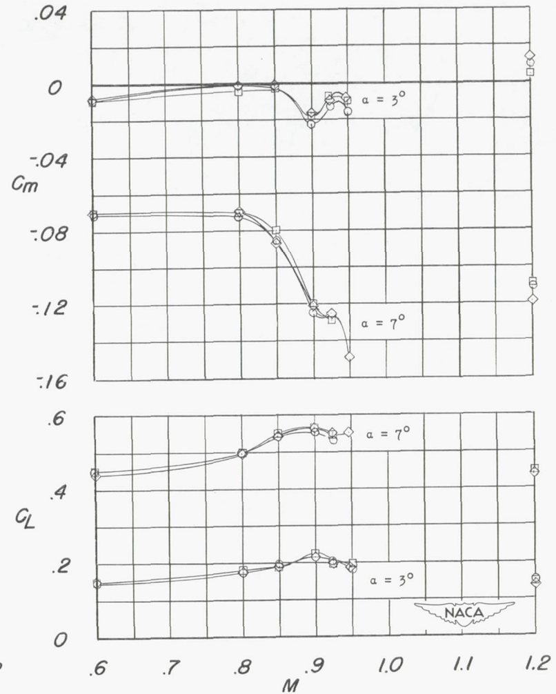
Figure 4.- Effects of fences on the aerodynamic characteristics of model 2 at Mach numbers from 0.6 to 0.95 and 1.2. Leading-edge sweepback = 38.8^\circ ; aspect ratio = 3.6.
