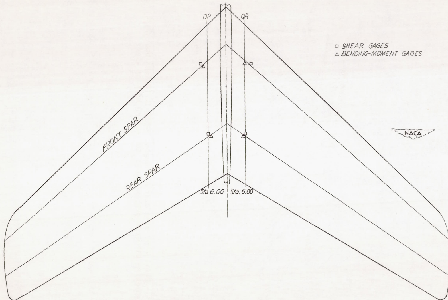
Figure 5.- Locations of strain gages on the horizontal tail of the Douglas D-558-II (BuAero No. 37974) research airplane.
