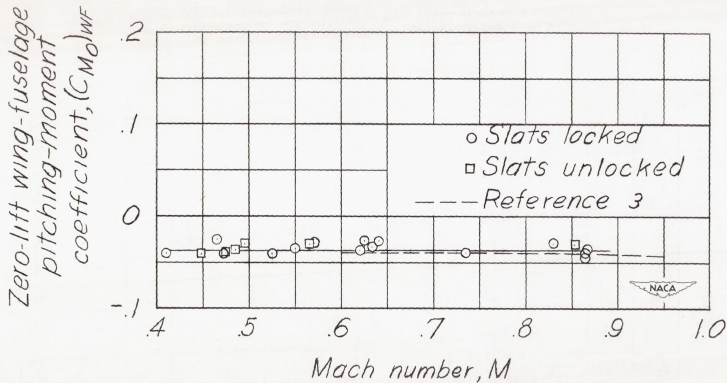
Figure 13.- Variation of the zero-lift wing-fuselage pitching-moment coefficient with Mach number.
