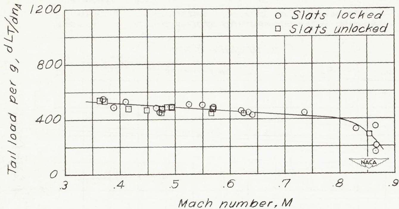
Figure 12.- Variation of the horizontal tail load per g with Mach number. W_0 , 9600 pounds; center of gravity, 26 percent mean aerodynamic chord.
