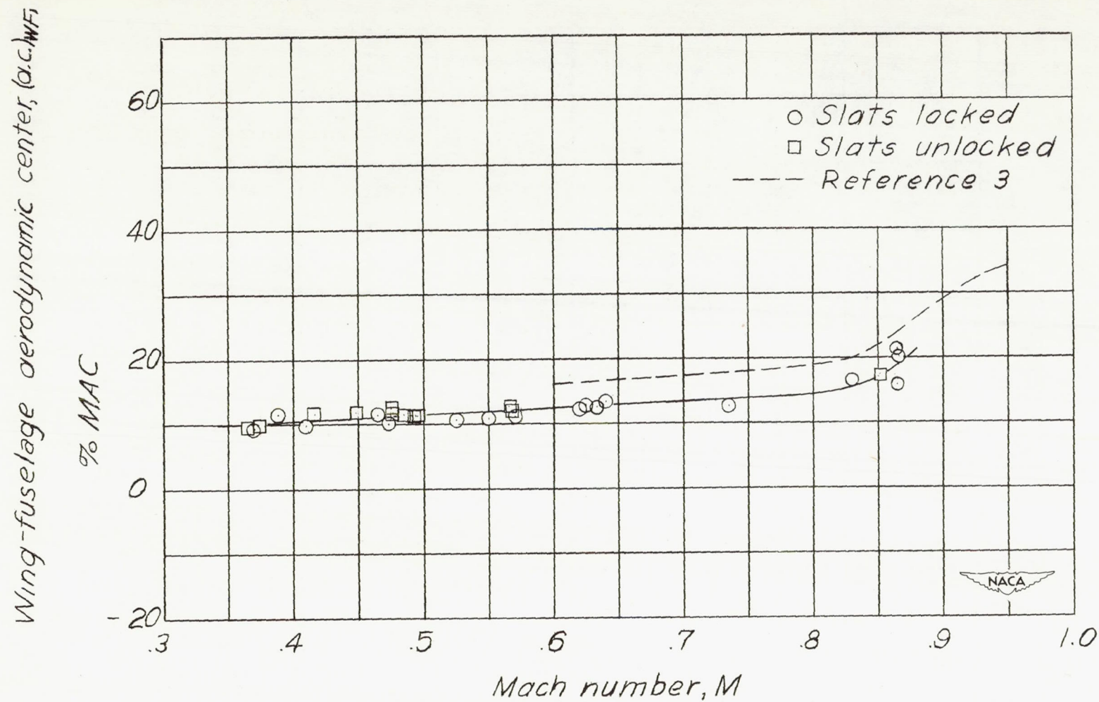
Figure 10.- Variation of the wing-fuselage aerodynamic center with Mach number.
