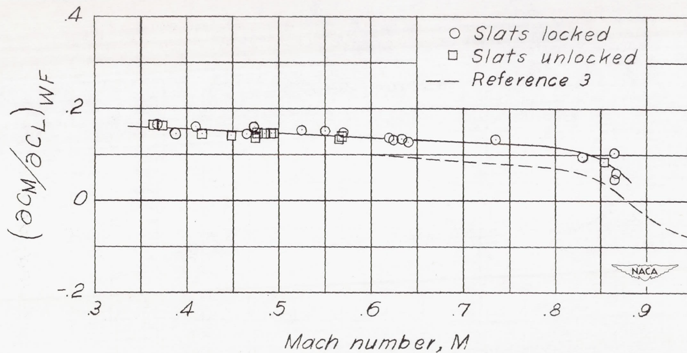
Figure 11.- Variation of the static-longitudinal-stability parameter (\partial C_M / \partial C_L)_{WF} with Mach number. Center of gravity, 26 percent mean aerodynamic chord.
