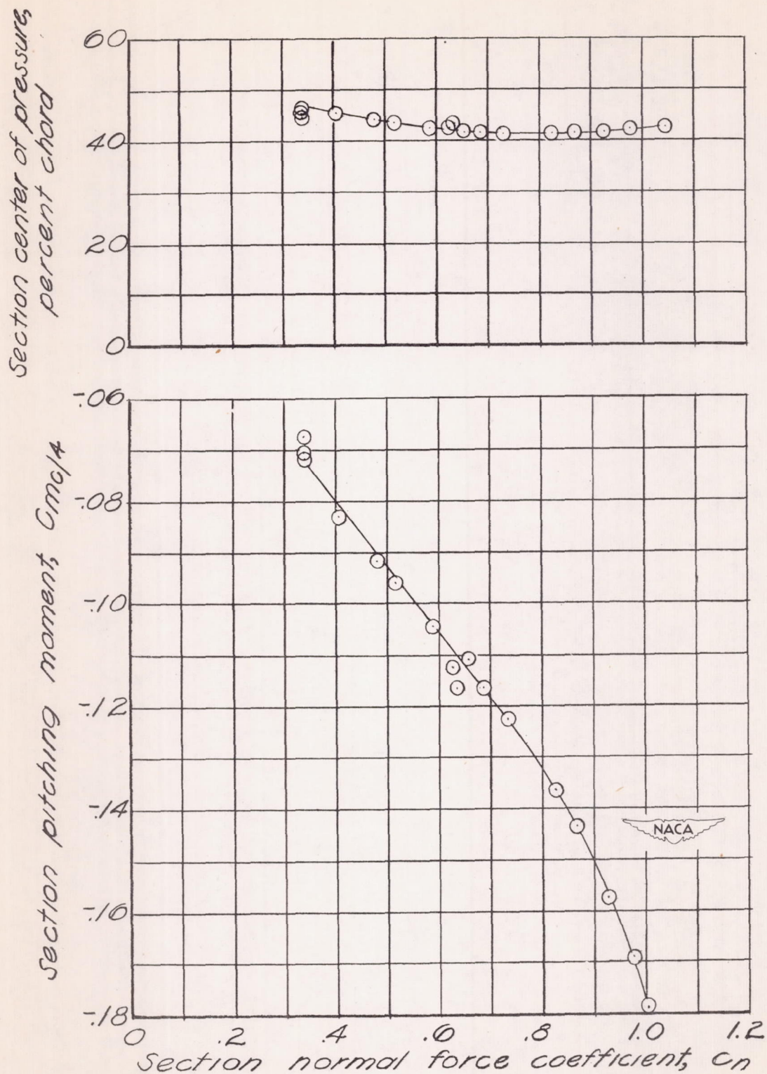
Figure 9.- Variation of section center of pressure and section pitching moment with section normal-force coefficient. M = 0.96 \pm 0.02 .
