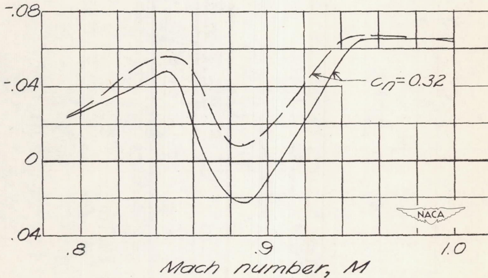
Figure 8.- Variation of section center of pressure and section pitching moment with Mach number. c_n = 0.32 \pm 0.08 .
