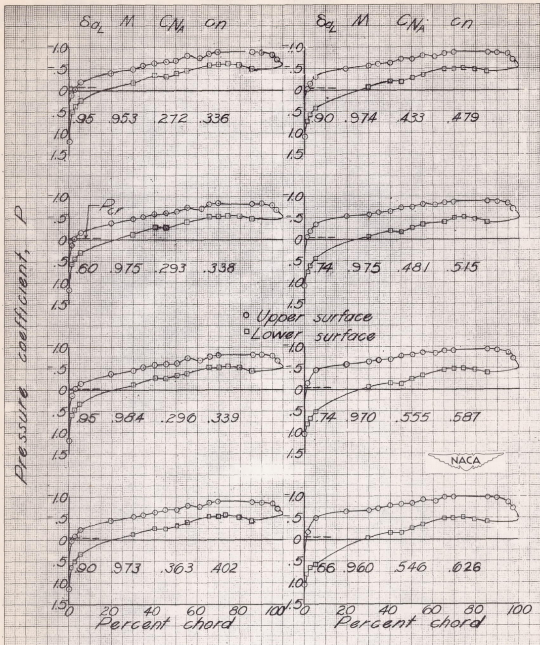
Figure 5.- Pressure distribution over one chordwise wing station of the X-1 airplane for several values of normal-force coefficient. \frac{2y}{b} = 0.644 ; M = 0.96 \pm 0.02 ; wing thickness, 0.10 chord.
