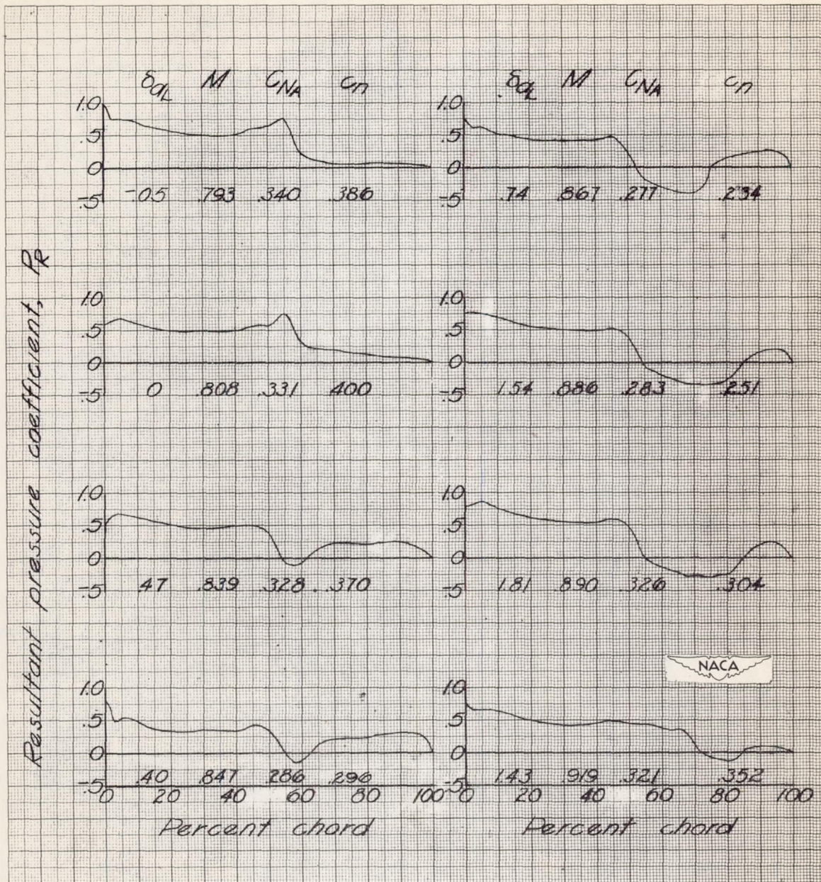
Figure 6.- Chordwise loading over one wing station of the X-1 airplane for several values of Mach number. \frac{2y}{b} = 0.644 ; c_n = 0.32 \pm 0.08 ; wing thickness, 0.10 chord.
