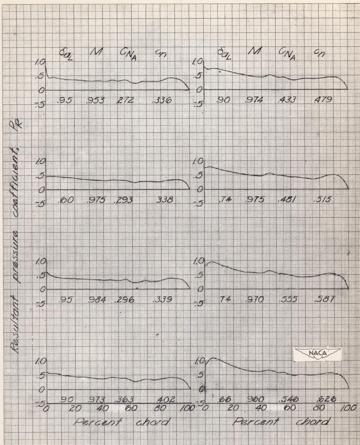
Figure 7.- Chordwise loading over one wing station of the X-1 airplane for several values of normal-force coefficient. \frac{2y}{b} = 0.644 ; M = 0.96 \pm 0.02 ; wing thickness, 0.10 chord.
