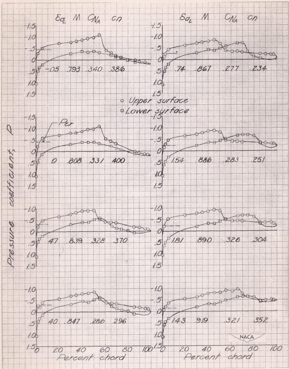
Figure 4.- Pressure distribution over one chordwise wing station of the X-1 airplane for several values of Mach number. \frac{2y}{b} = 0.644 ; c_n = 0.32 \pm 0.08 ; wing thickness, 0.10 chord.
