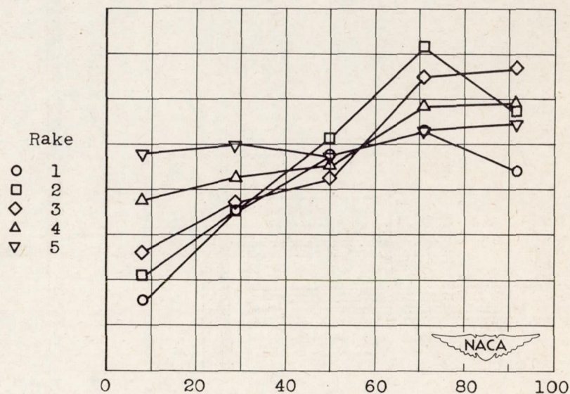
(b) Combustion chamber 3.
