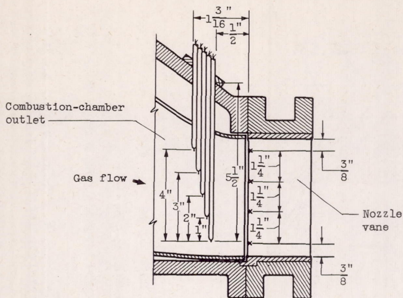
(a) Radial location of thermocouples.
