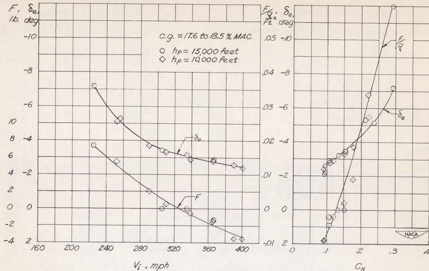
Figure 3. — Longitudinal-stability and-control characteristics in straight flight of X-4 airplane.
