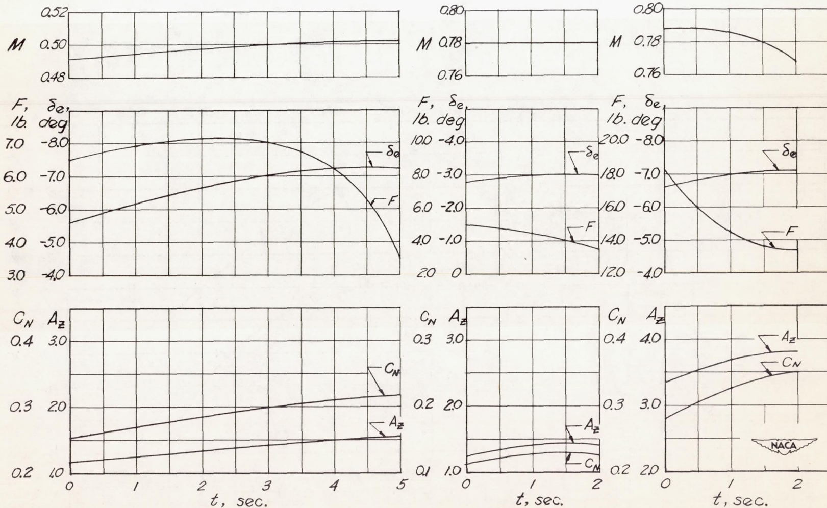
Figure 4.— Time histories of pertinent variables during several accelerated stability runs. X-4 airplane.
