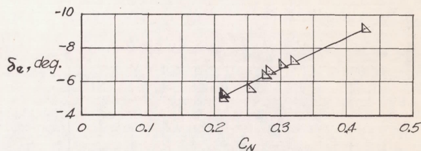
Figure 6. — Variation of elevon control angle and control force with airplane normal-force coefficient and normal-acceleration factor, respectively, for several values of Mach number. X-4 airplane.
