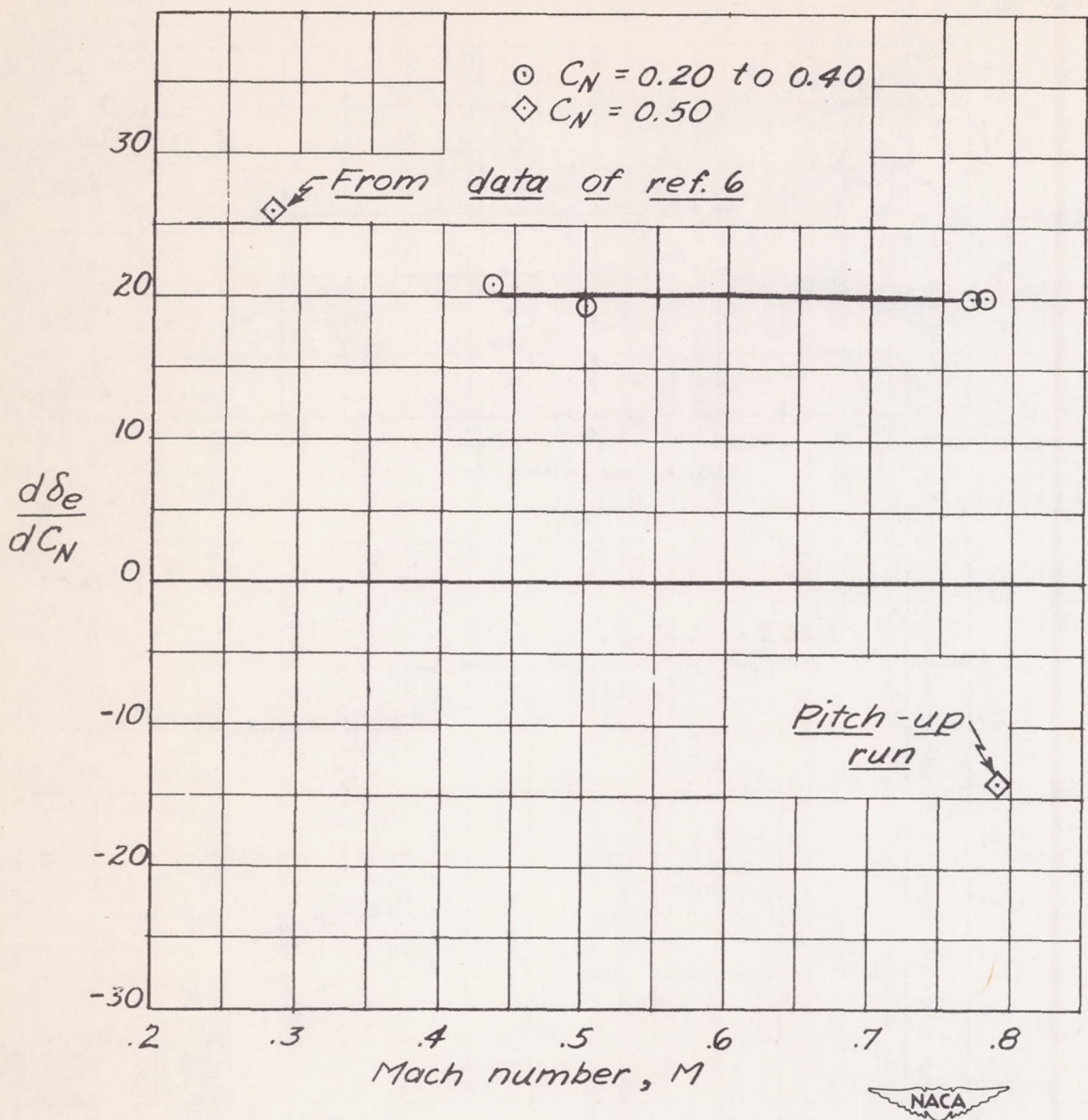
Figure 7. — Variation with Mach number of the elevon control-angle gradient. X-4 airplane.
