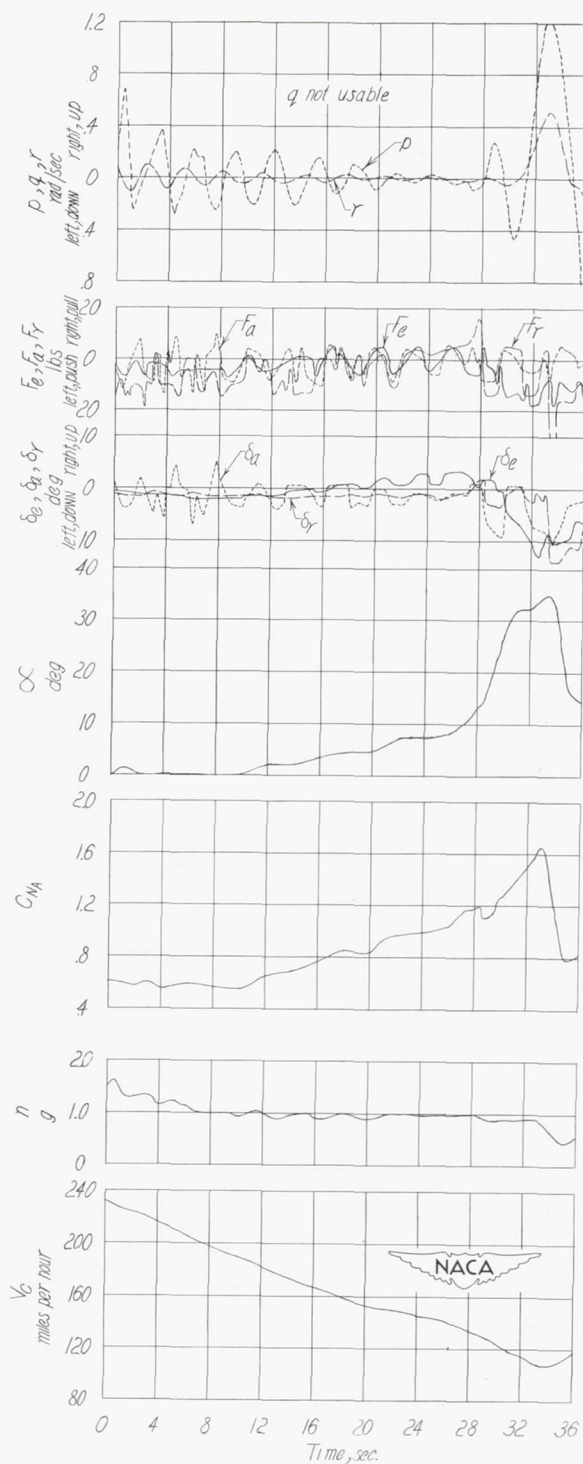
Figure 15.- Time history of a stall with the Douglas D-558-II (BuAero No. 37974) research airplane. Flaps down; landing gear down; slats locked; inlet-duct flaps open; stabilizer setting 0.7^\circ ; center of gravity at 26.6 percent mean aerodynamic chord.
