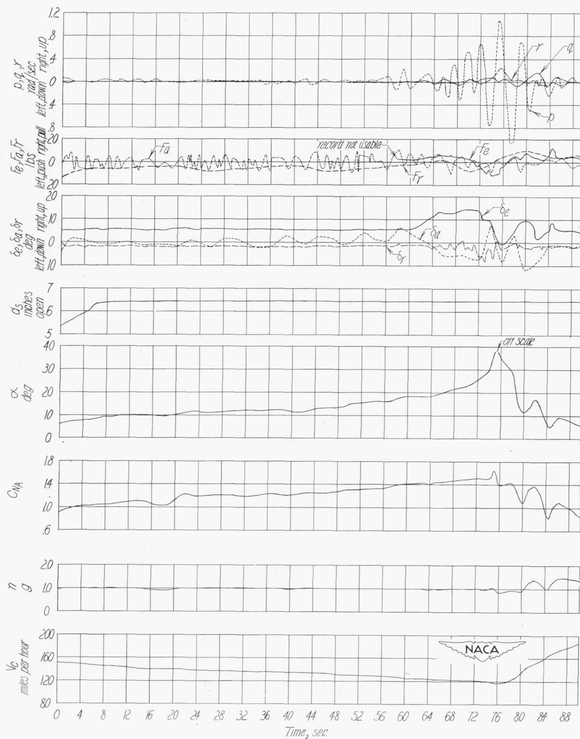
Figure 17.- Time history of a stall with the Douglas D-558-II (BuAero No. 37974) research airplane. Flaps down; landing gear down; slats unlocked; inlet-duct flaps open; stabilizer setting 1.72^\circ ; center of gravity at 26.3 percent mean aerodynamic chord.
