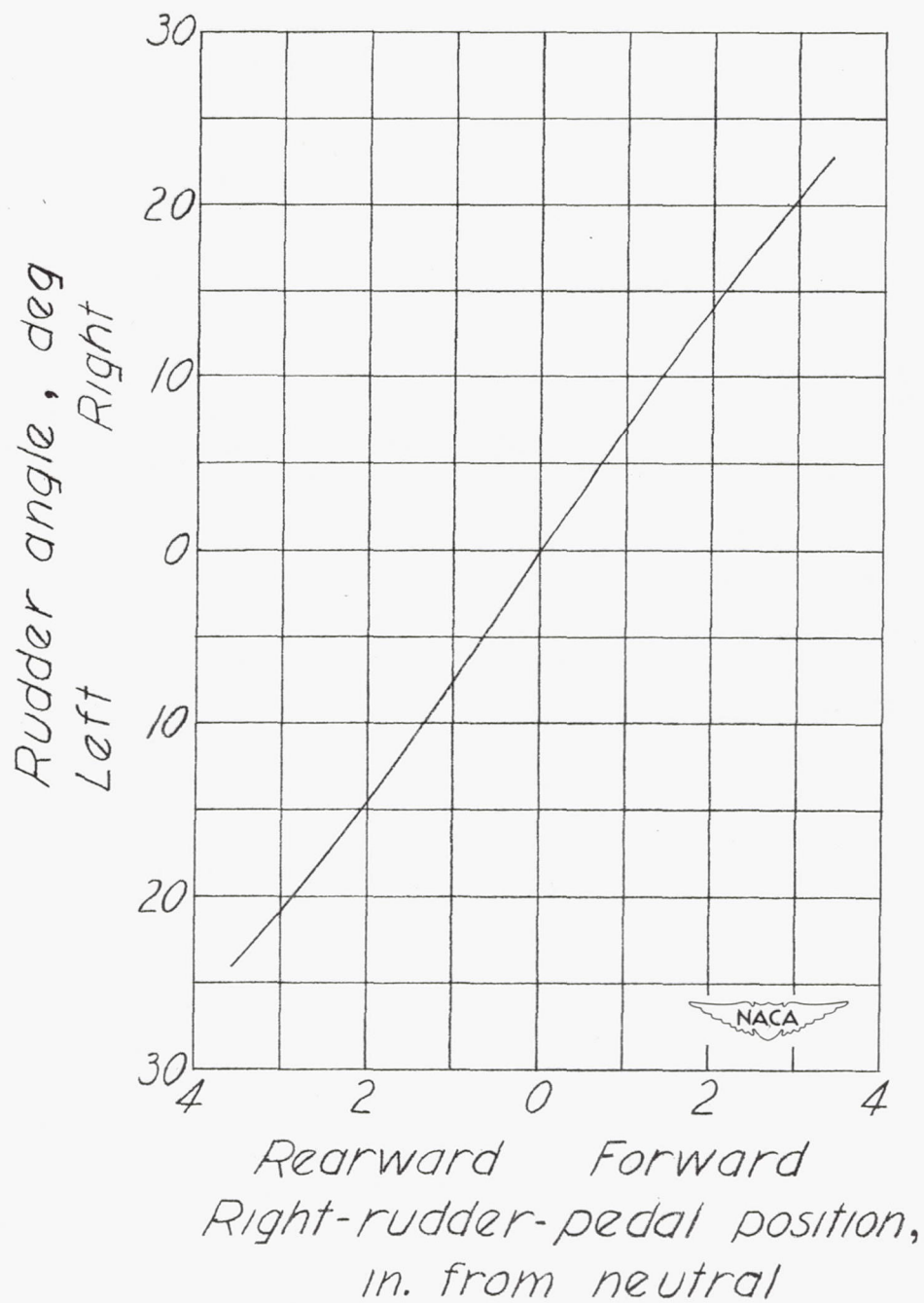
Figure 7.- Variation of rudder position with right-rudder-pedal position. No load on system.
