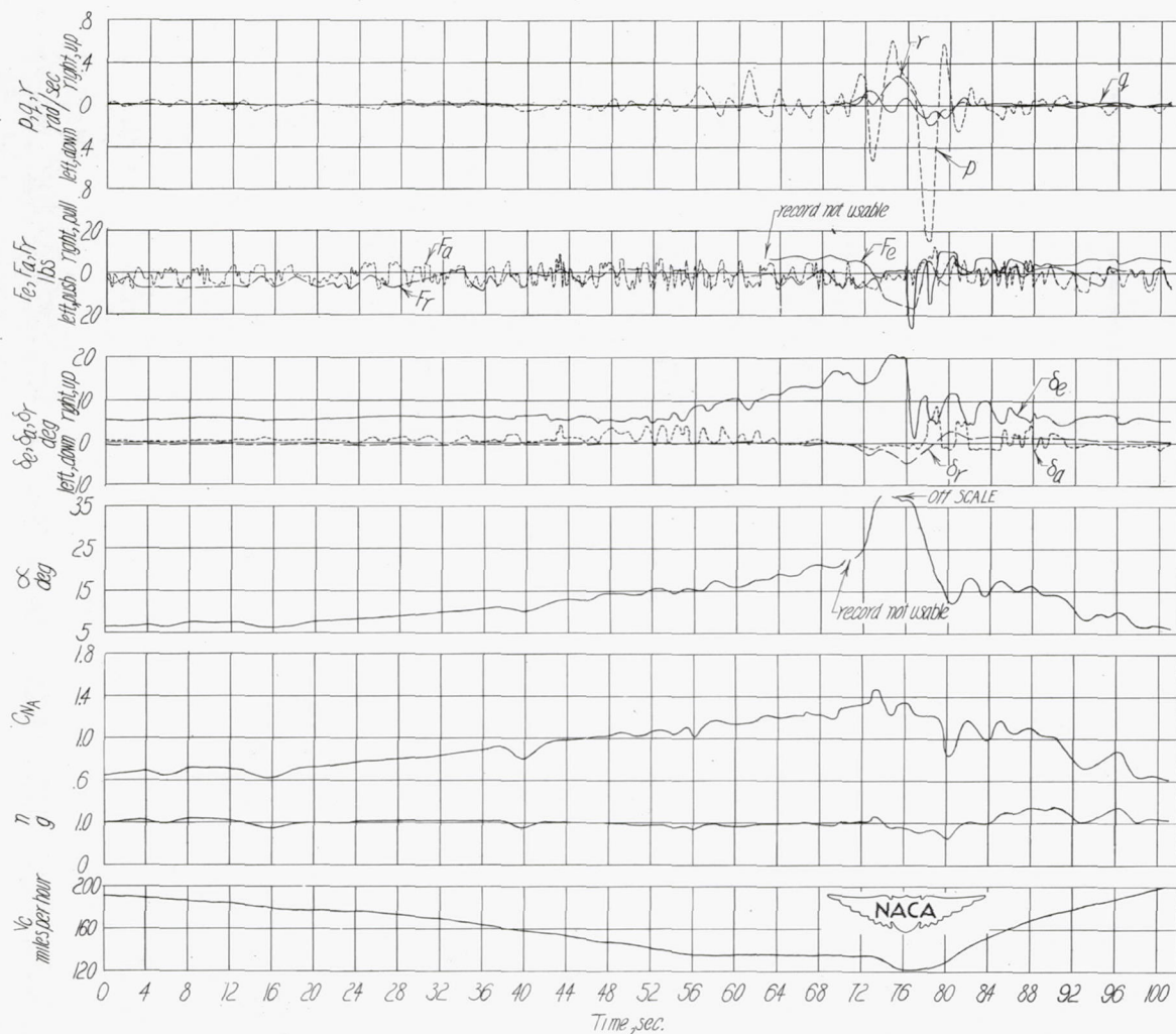
Figure 13.- Time history of a stall with the Douglas D-558-II (BuAero No. 37974) research airplane. Flaps up; landing gear up; slats unlocked; inlet duct-flaps closed; stabilizer setting 1.72^\circ ; center of gravity at 26.7 percent mean aerodynamic chord.
