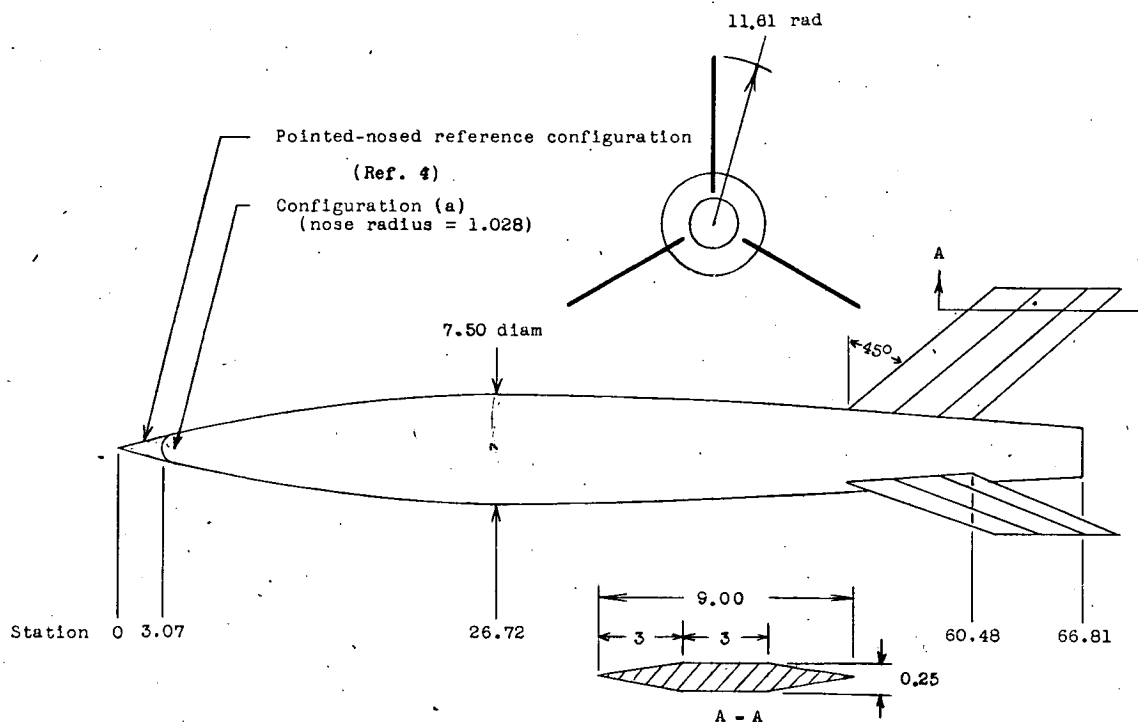
(a) Parabolic bodies.
