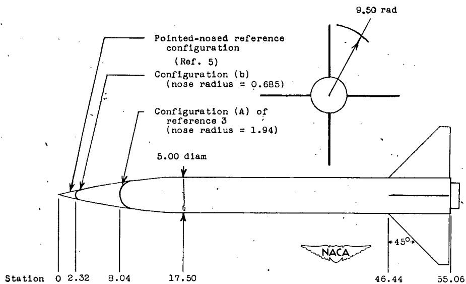
(b) Cylindrical bodies.
