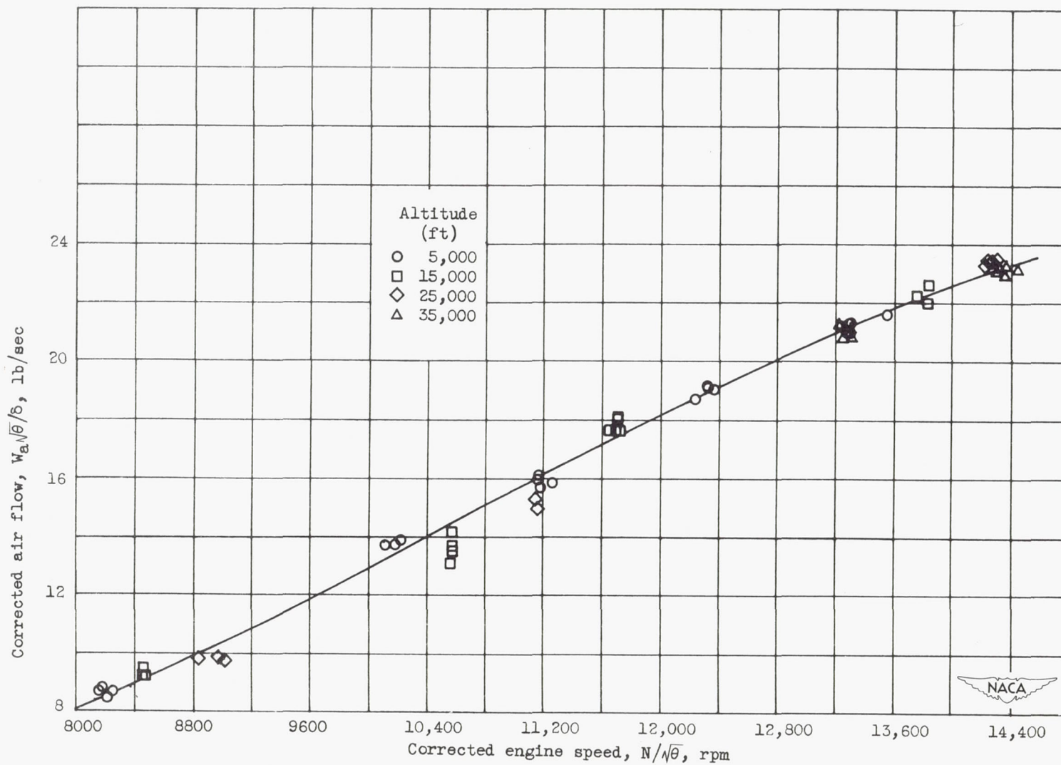
Figure 14. - Variation of corrected air flow with corrected engine speed. Compressor-inlet ram pressure ratio, 1.00.
