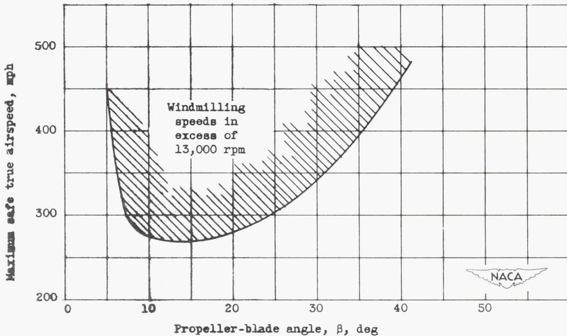
Figure 25. - Variation of maximum safe true airspeed with propeller-blade angle for windmilling engine.
