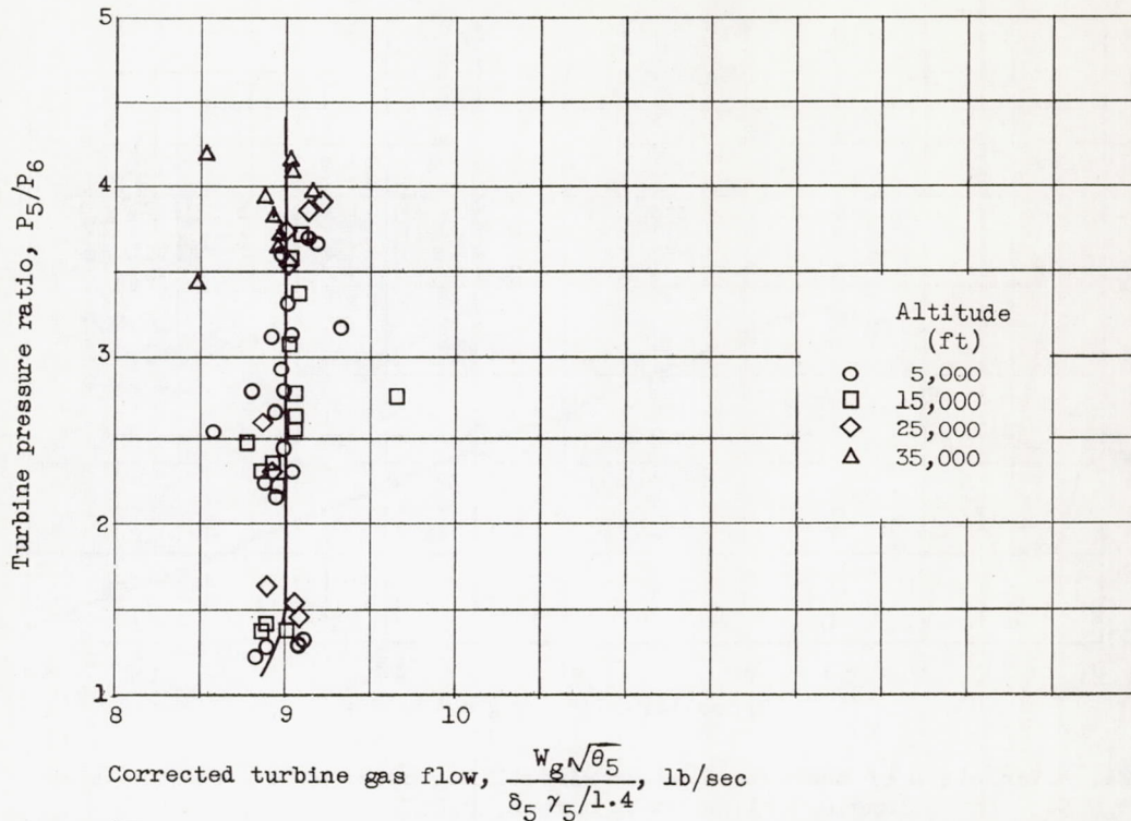
Figure 22. - Variation of turbine pressure ratio with corrected turbine gas flow. Compressor-inlet ram pressure ratio, 1.00.
