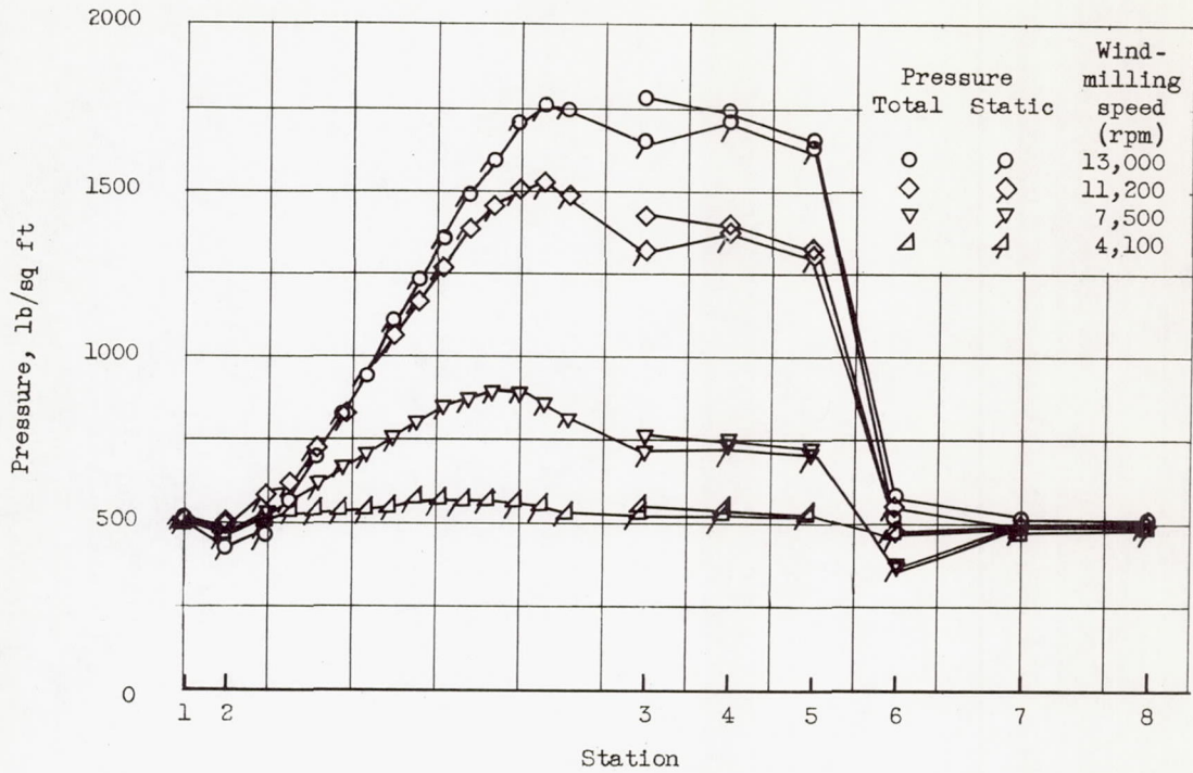
Figure 26. - Total and static pressures through engine at various windmilling speeds. Altitude, 35,000 feet; propeller-blade angle, 12°.
