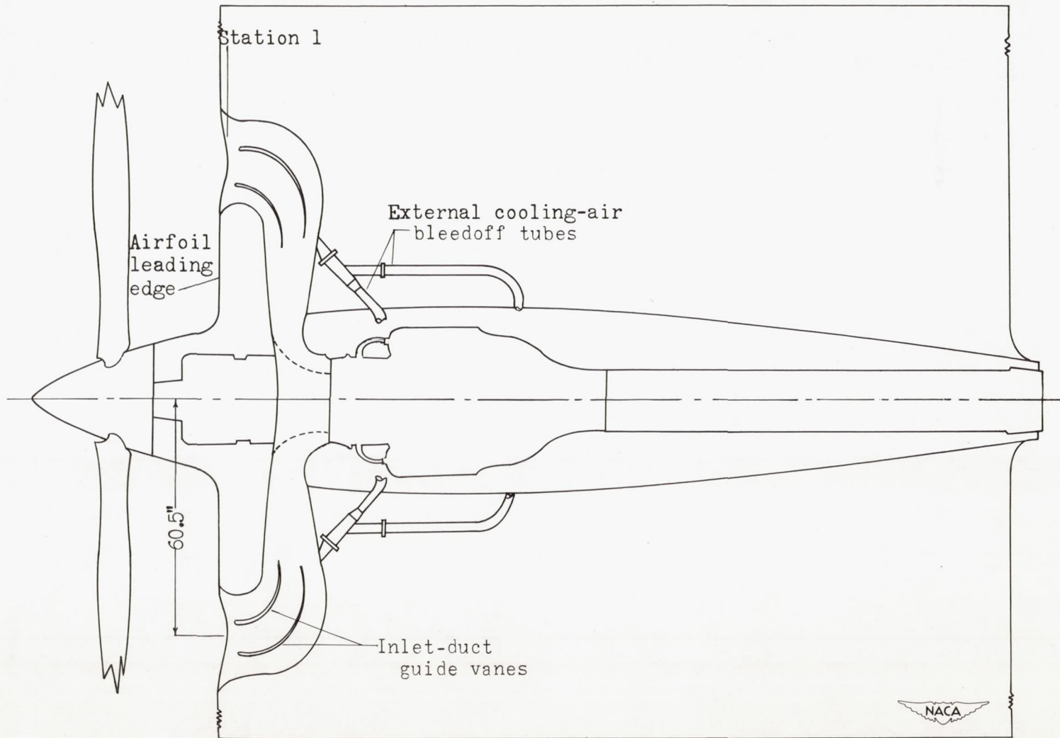
Figure 5. - Sketch of turbine-propeller-engine installation showing location of wing ducts and inlets.
