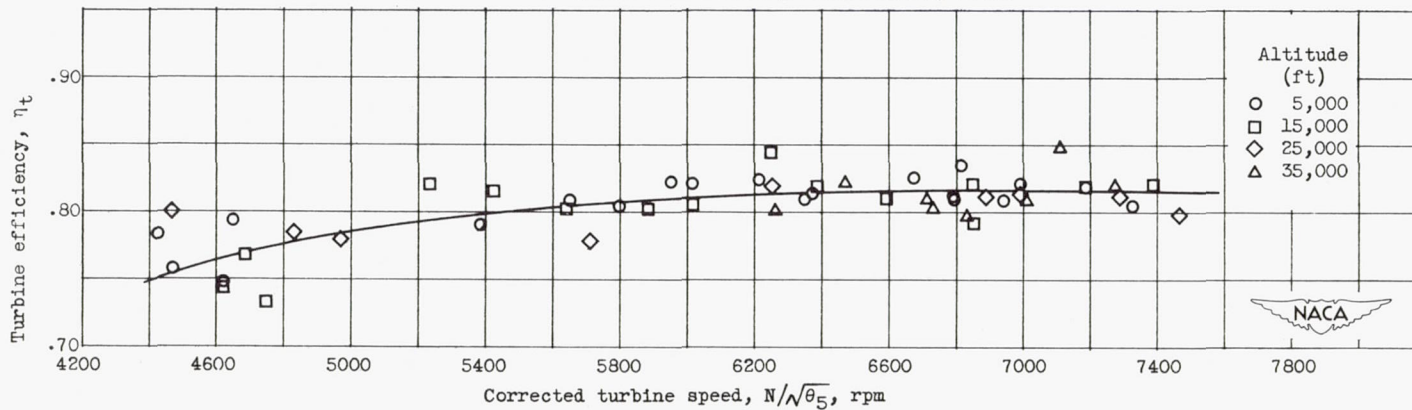
Figure 21. - Variation of turbine efficiency with corrected turbine speed. Compressor-inlet ram pressure ratio, 1.00.
