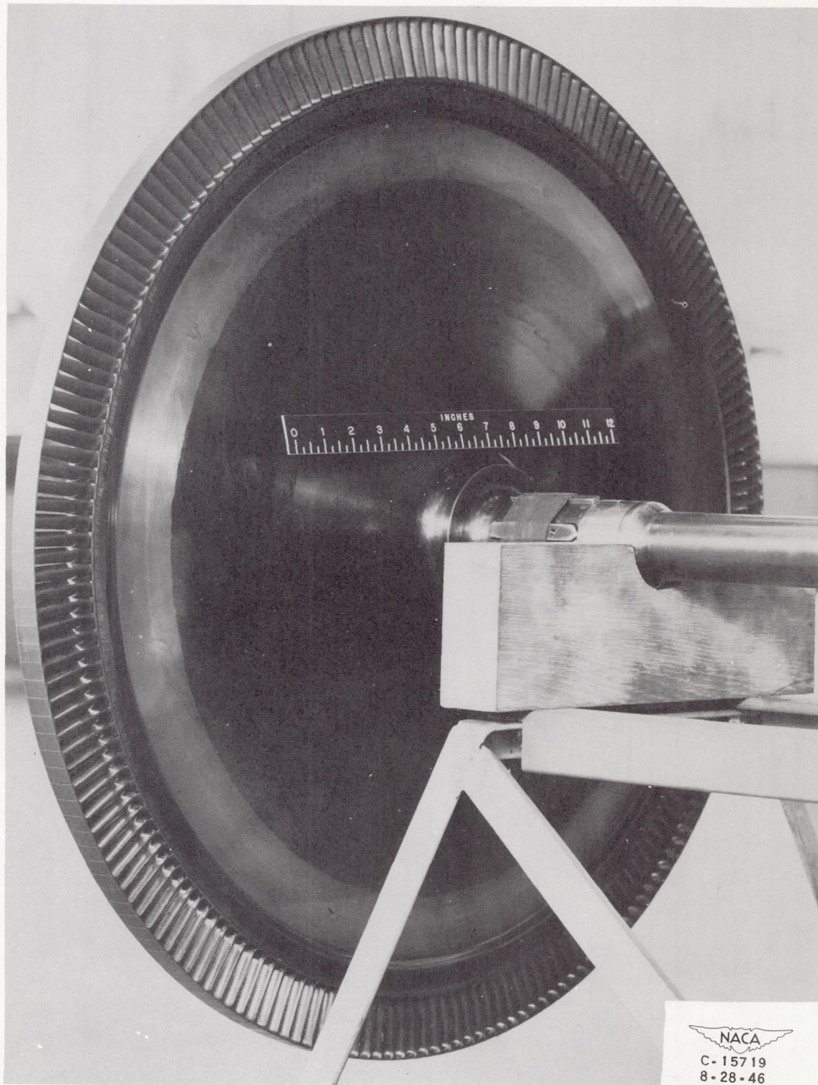
Figure 4. - Turbine wheel used in axial-flow-compressor turbine-propeller engine.
