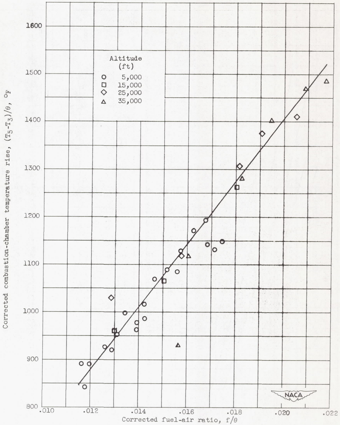
Figure 19. - Effect of altitude on engine combustion process. Corrected engine speed, 8200 to 14,200 rpm.
