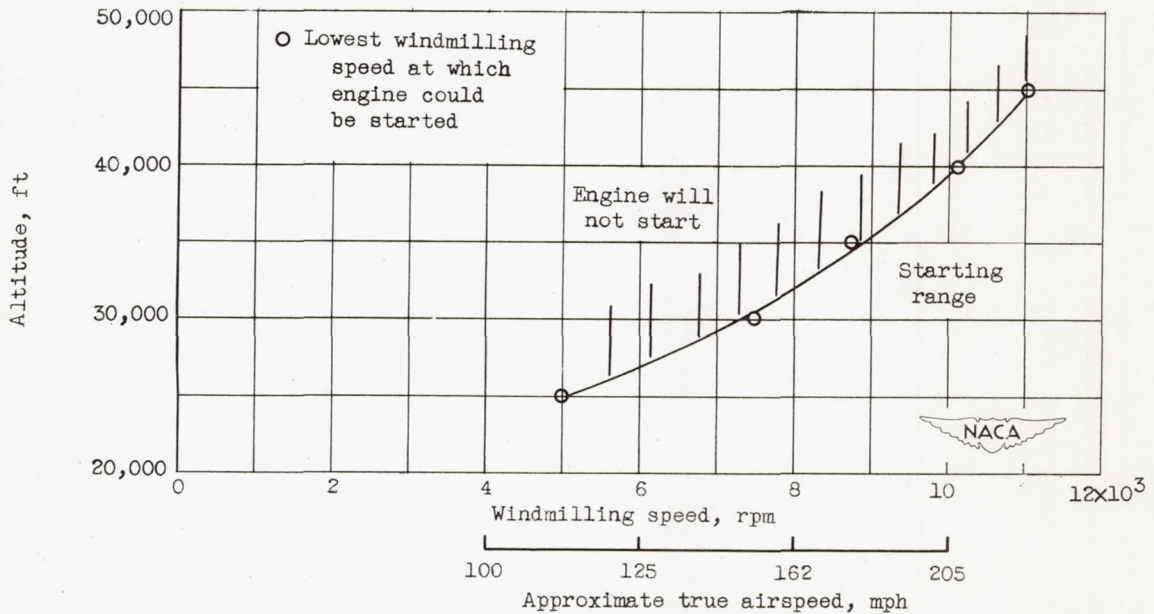
Figure 27. - Variation of minimum windmilling speed at which engine can be started with altitude.
