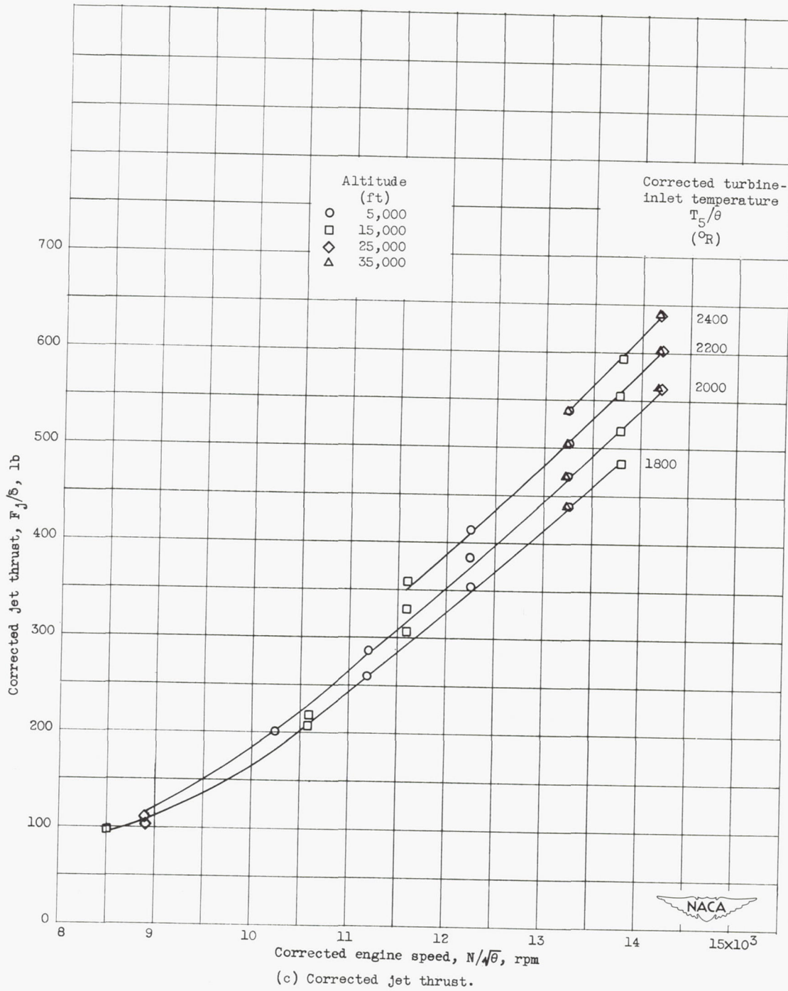
Figure 11. - Concluded. Variation of corrected engine parameters with corrected engine speed. Compressor-inlet ram pressure ratio, 1.00.
