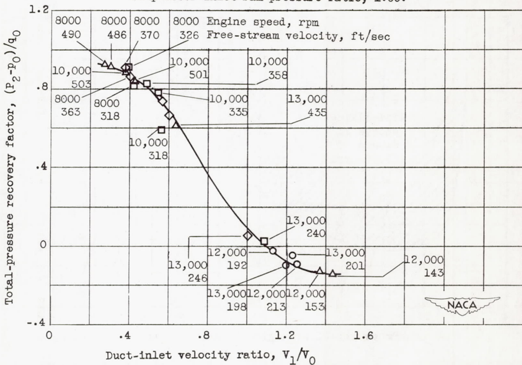
Figure 23. - Variation of induction-system total-pressure recovery with duct-inlet velocity ratio.
