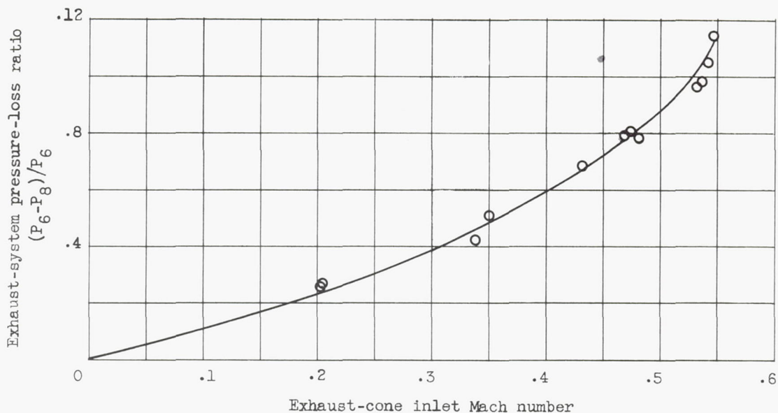
Figure 8. - Variation of exhaust-system pressure-loss ratio with exhaust-cone inlet Mach number. Exhaust-gas temperature, approximately 1500° R.
