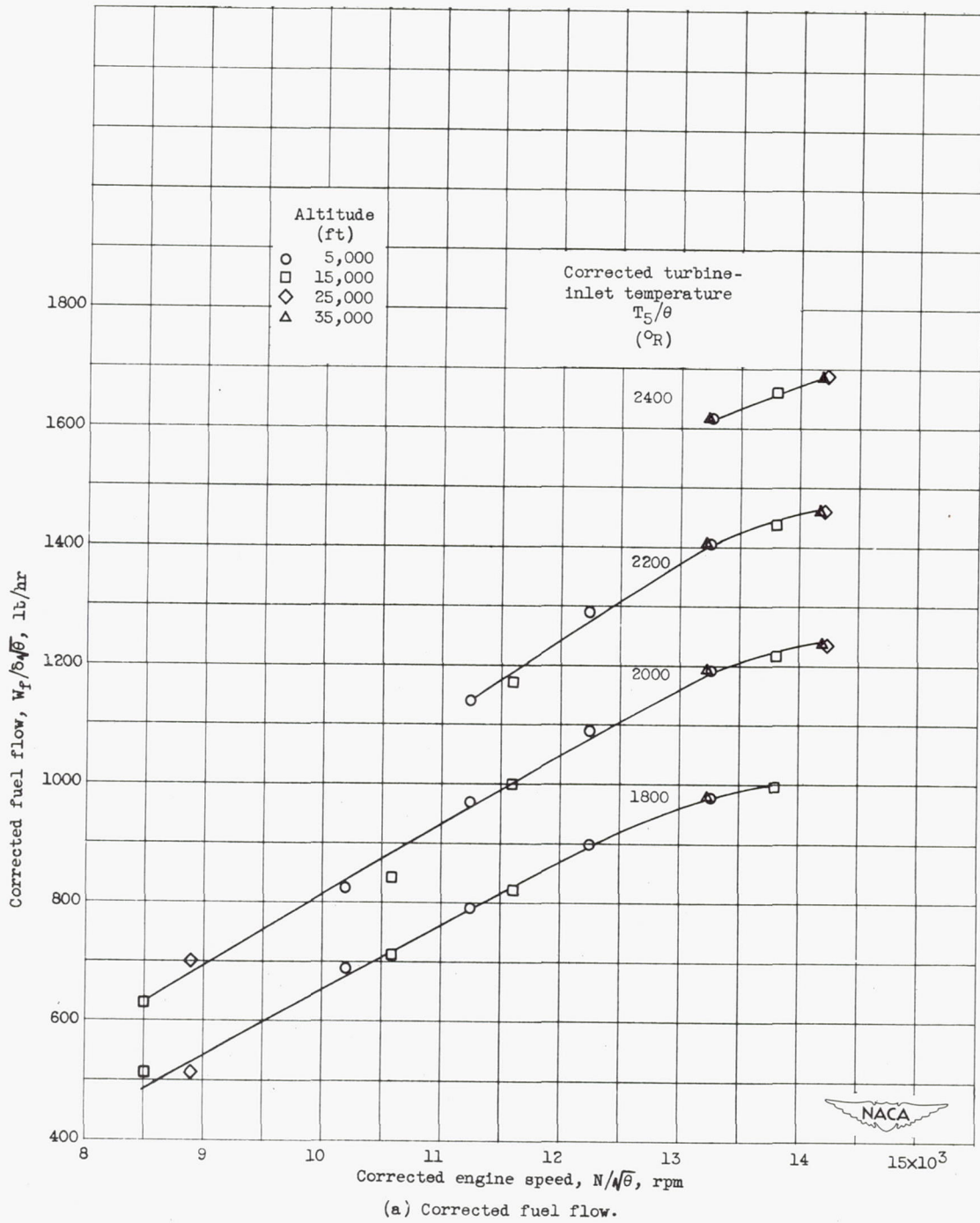
Figure 11. - Variation of corrected engine parameters with corrected engine speed. Compressor-inlet ram pressure ratio, 1.00.
