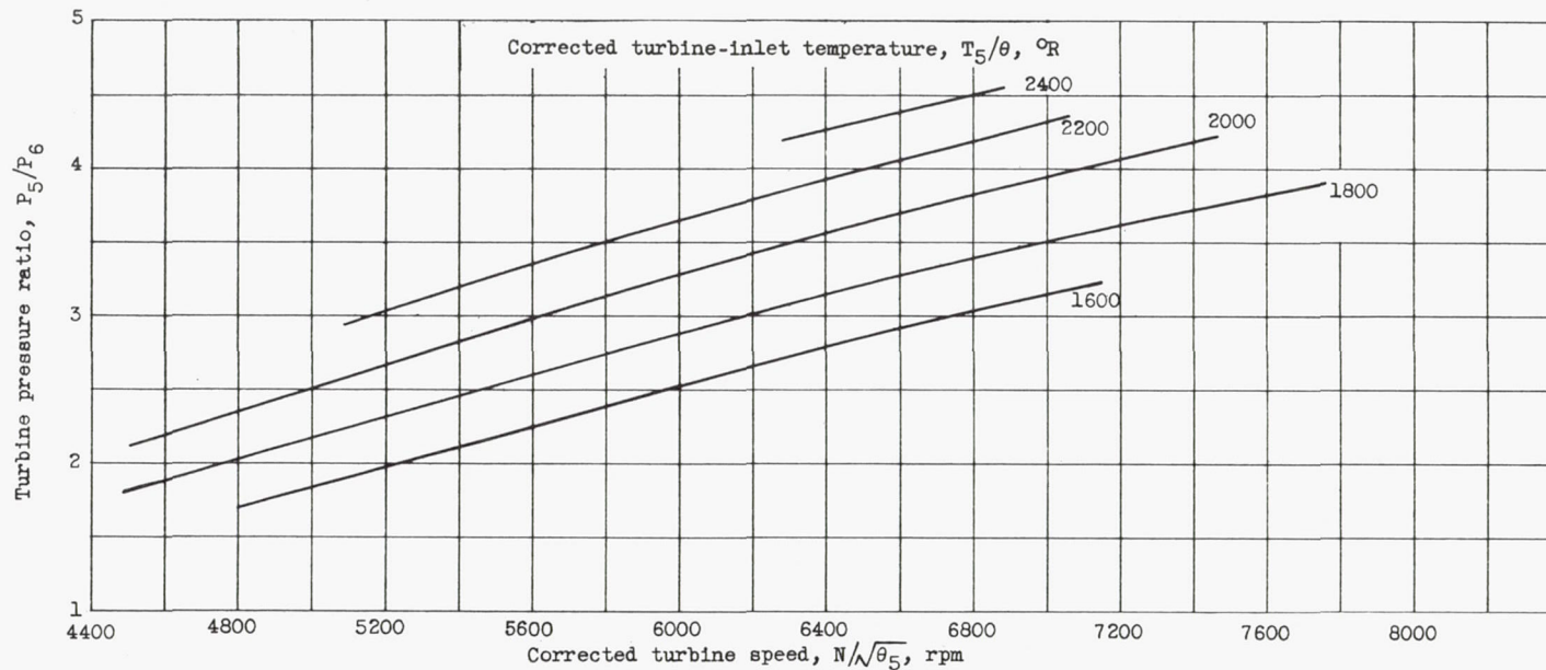
Figure 20. - Variation of turbine pressure ratio with corrected turbine speed at constant corrected turbine-inlet temperatures. Compressor-inlet ram pressure ratio, 1.00.
