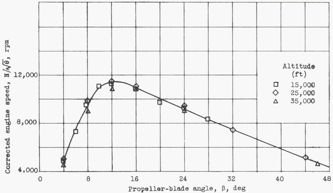
Figure 24. - Variation of corrected engine windmilling speed with propeller-blade angle. Flight Mach number, 0.285.
