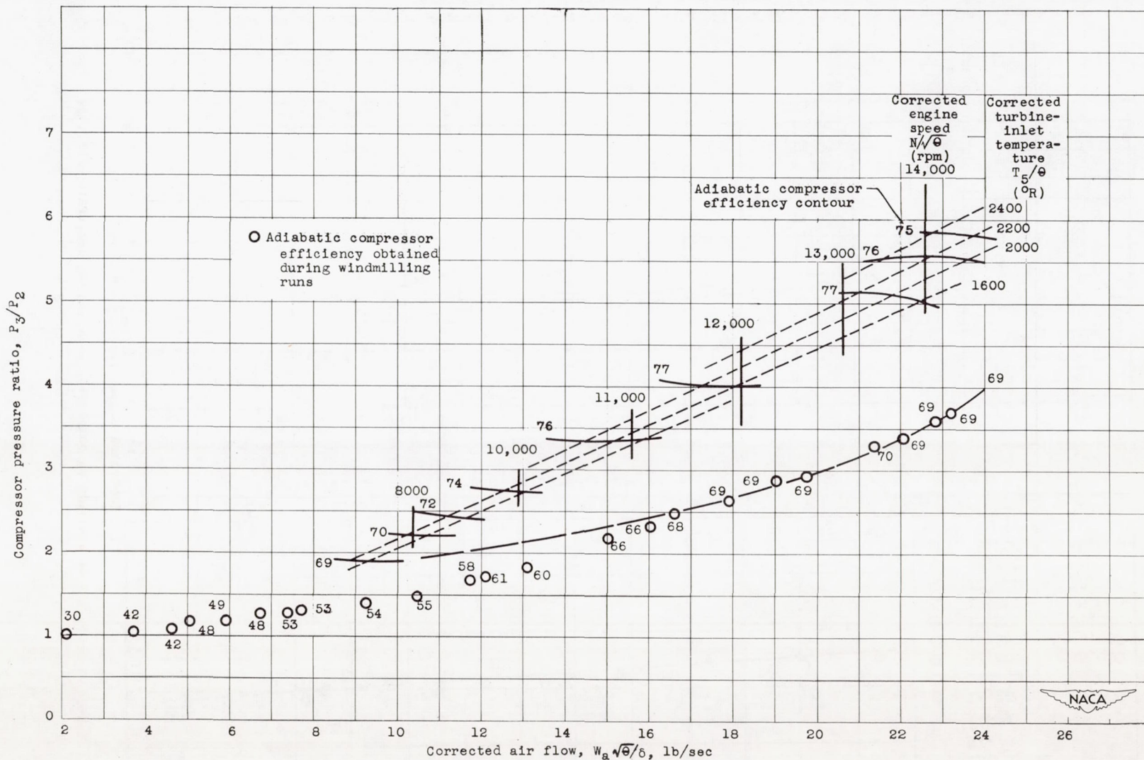
Figure 17. - Over-all compressor performance curves. Compressor-inlet ram pressure ratio, 1.00.
