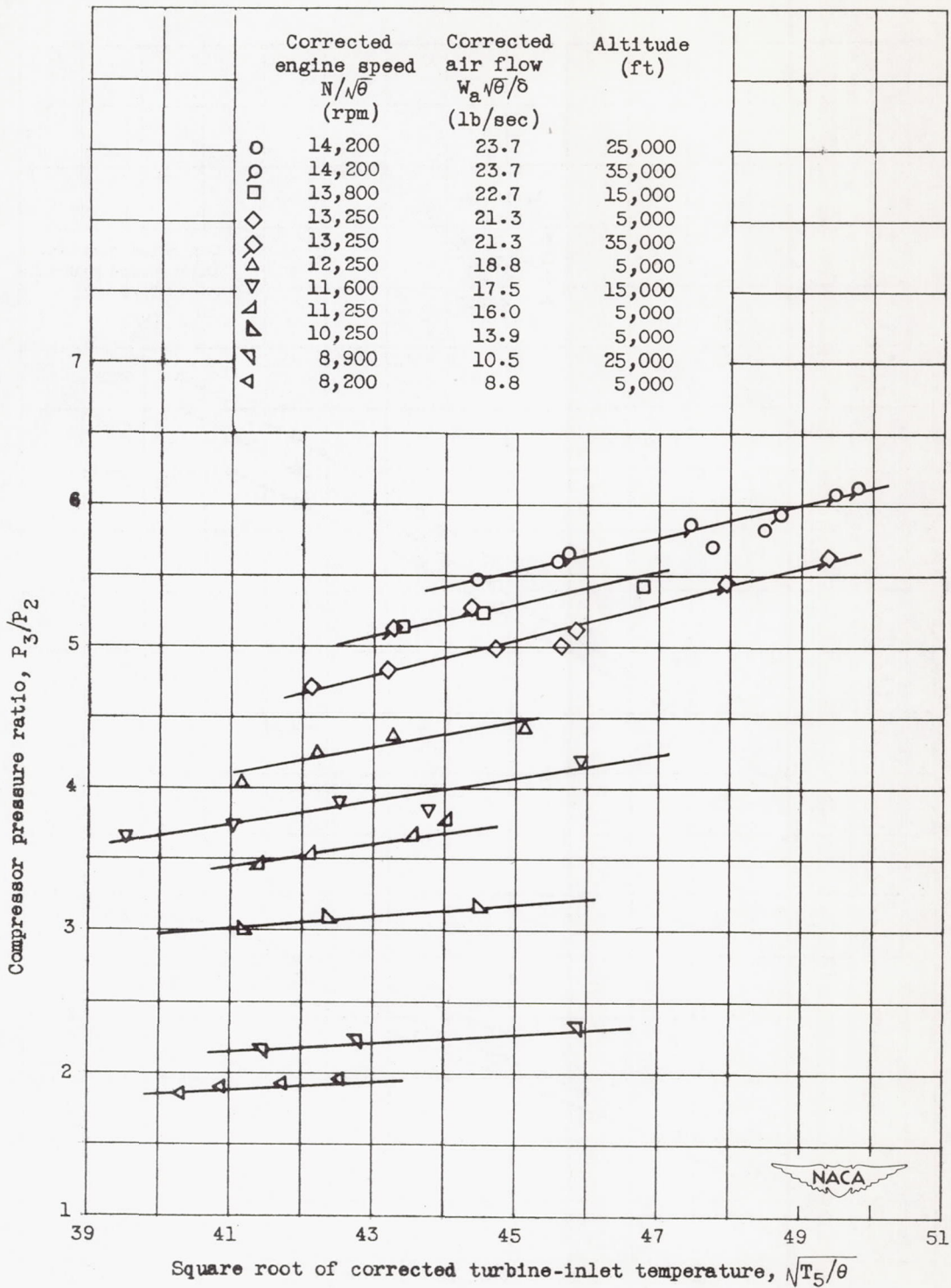
Figure 15. - Variation of compressor pressure ratio with corrected turbine-inlet temperature. Compressor-inlet ram pressure ratio, 1.00.
