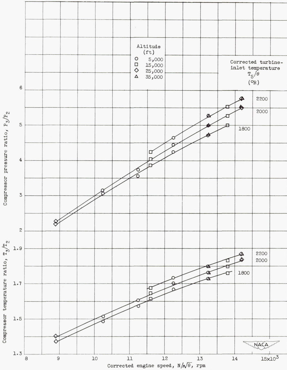
Figure 16. - Effect of altitude on compressor pressure and temperature ratios.
