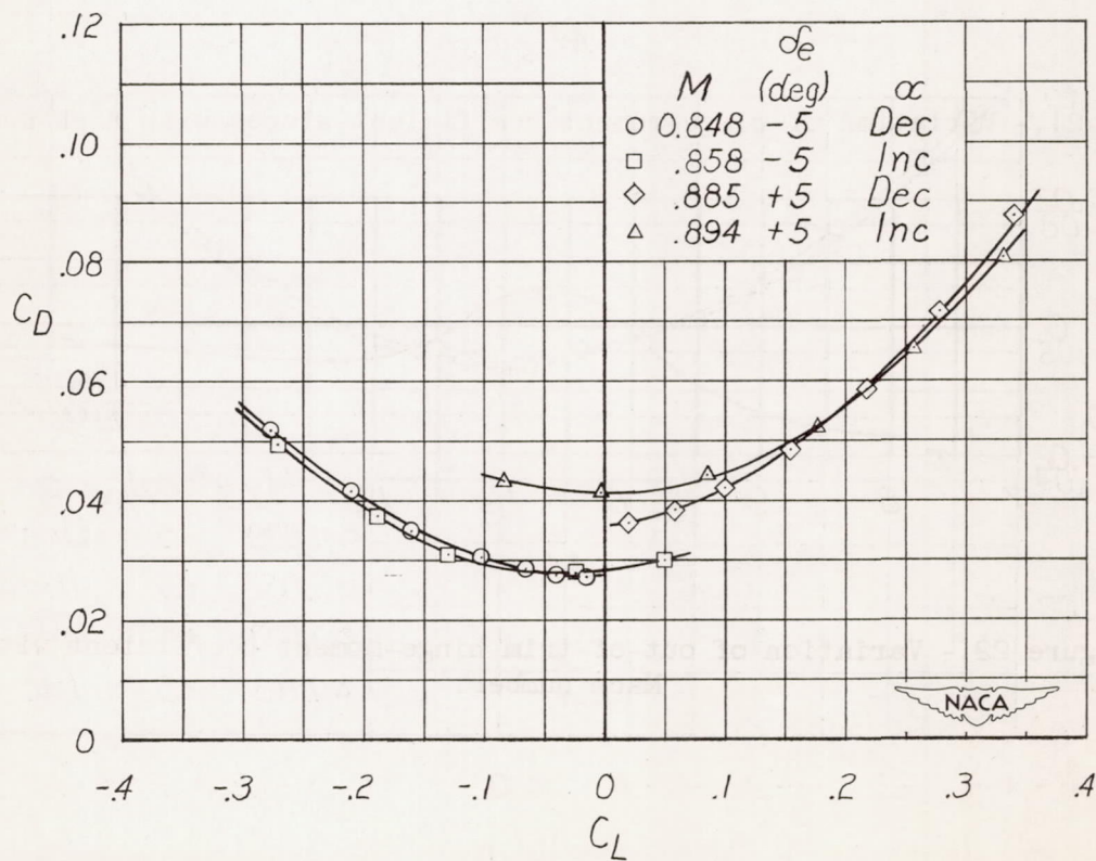
Figure 23.- Lift-drag polar.
