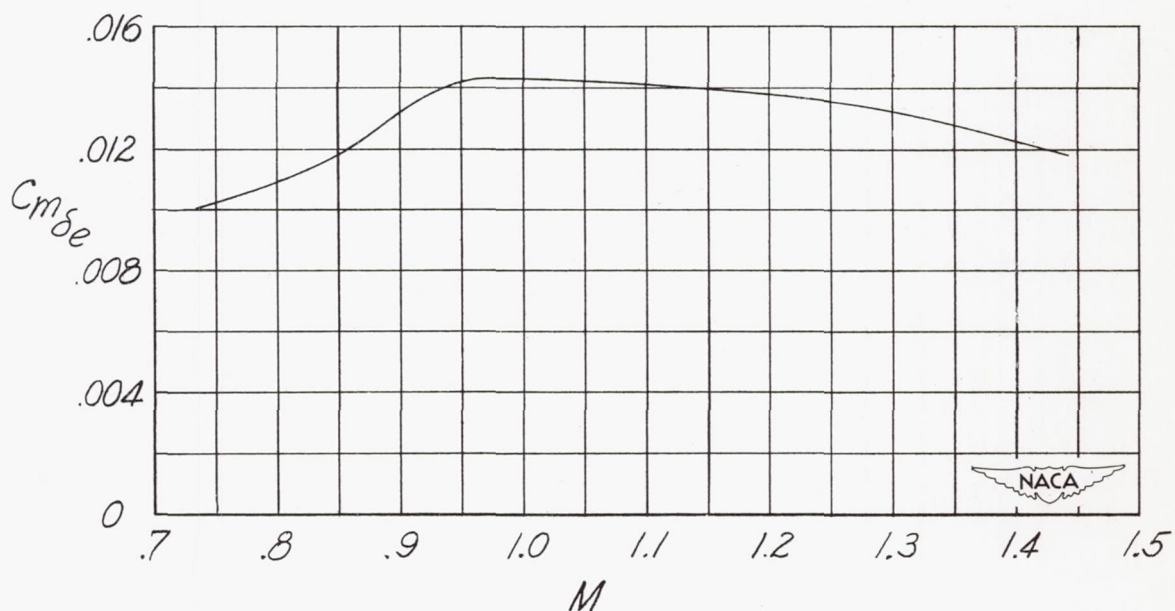
Figure 15.- Pitching effectiveness of canard control surfaces.
