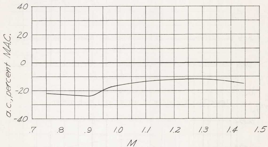
Figure 13.- Variation of aerodynamic-center position with Mach number.
