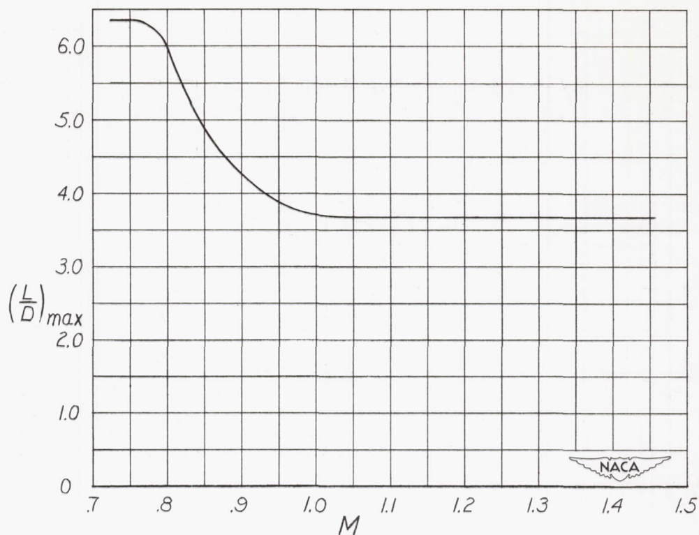
Figure 24.- Variation of maximum lift-drag ratio with Mach number.
