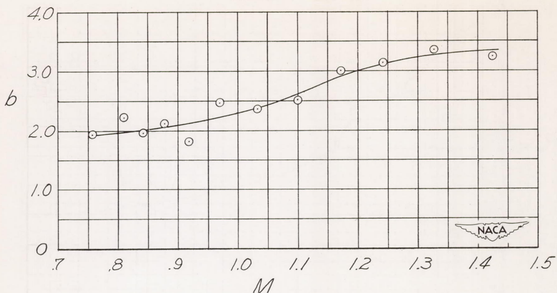
Figure 9.- Variation of exponential damping constant b with Mach number.
