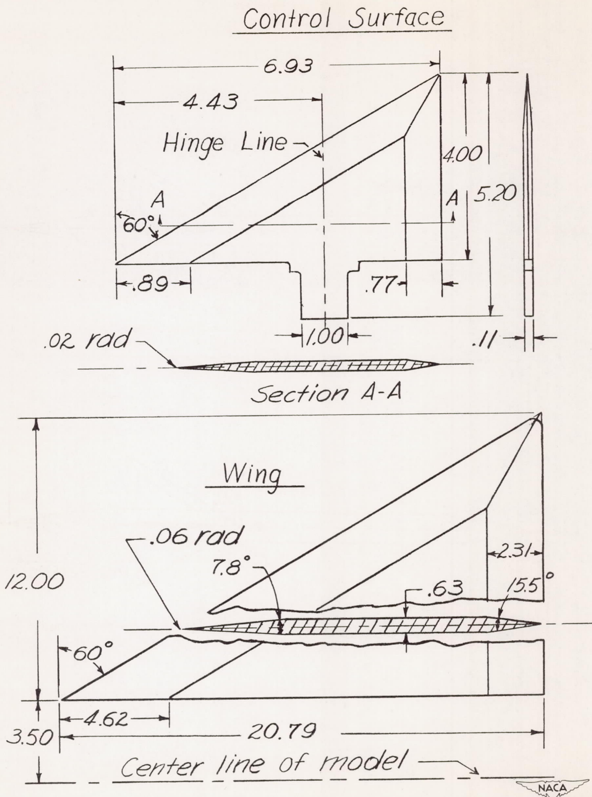
Figure 2.- Wing and control-surface detail. (All dimensions are in inches.)
