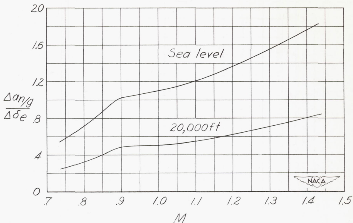
Figure 18.- Trim normal acceleration produced by a unit control deflection.
