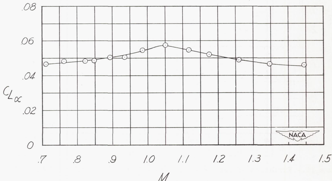
Figure 8.- Variation of lift-curve slope with Mach number.
