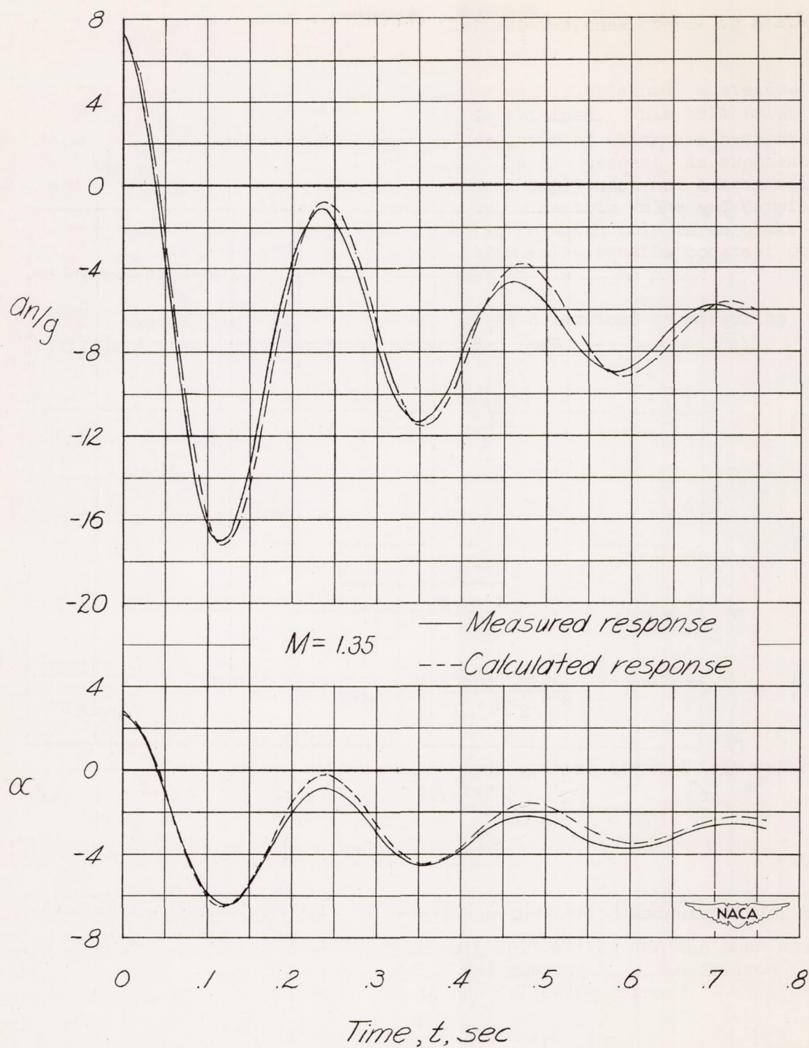
Figure 4.- Comparison of measured and calculated response curves.
