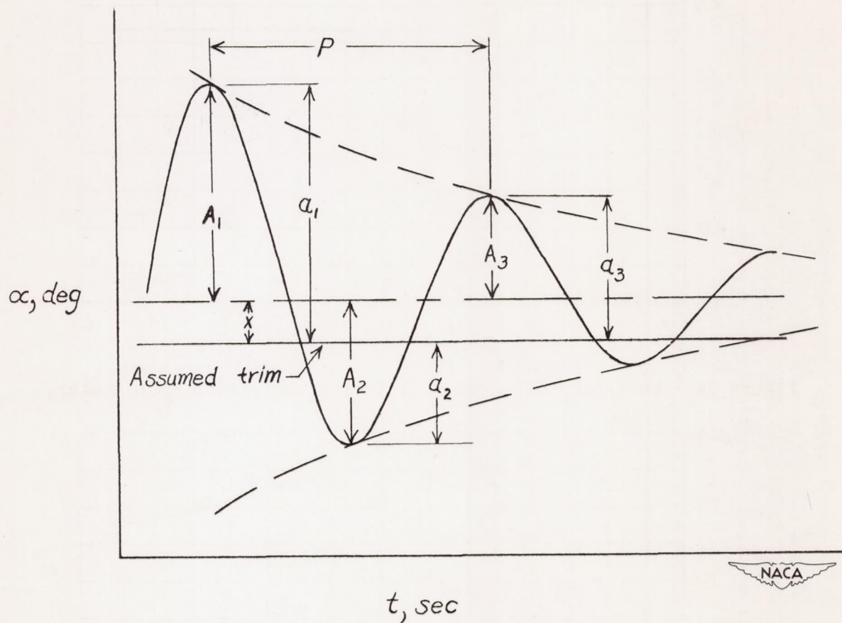
Figure 26.- Angle-of-attack response to step control input.
