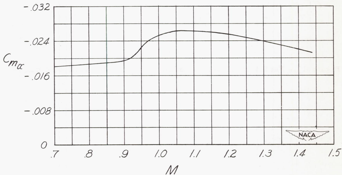
Figure 12.- Variation of static pitching-moment derivative C_{m\alpha} with Mach number.
