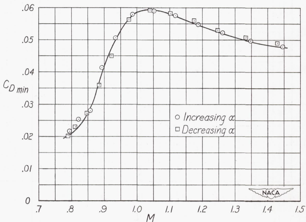
Figure 25.- Variation of minimum drag coefficient with Mach number.
