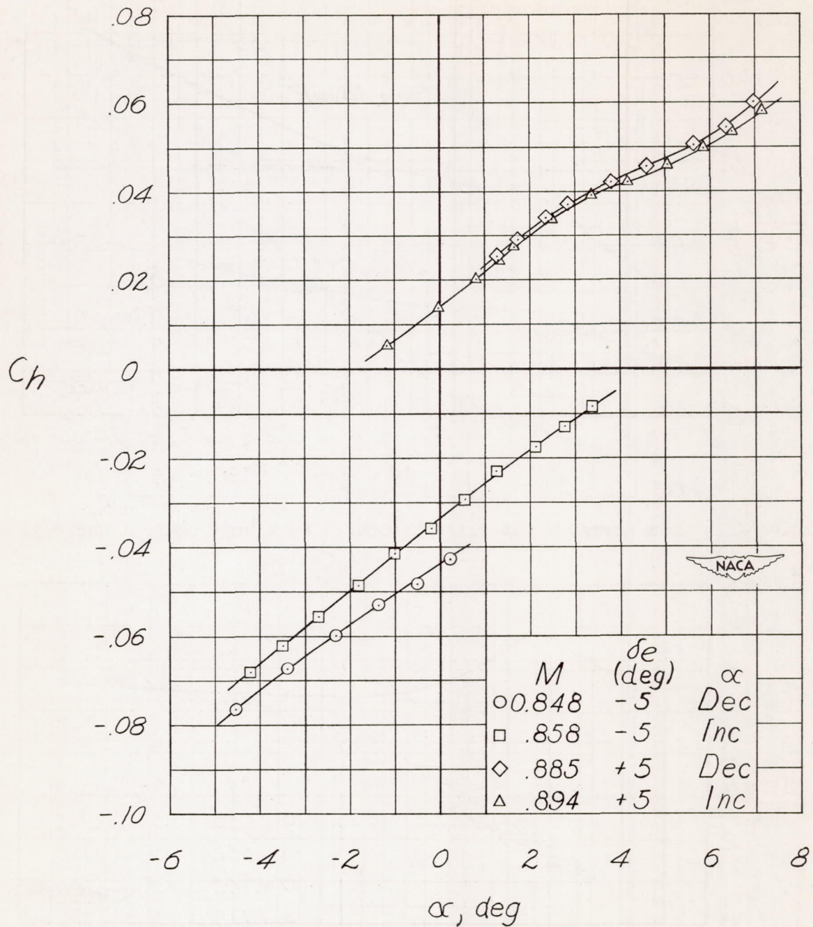
Figure 20.- Variation of control-surface hinge-moment coefficient with angle of attack.
