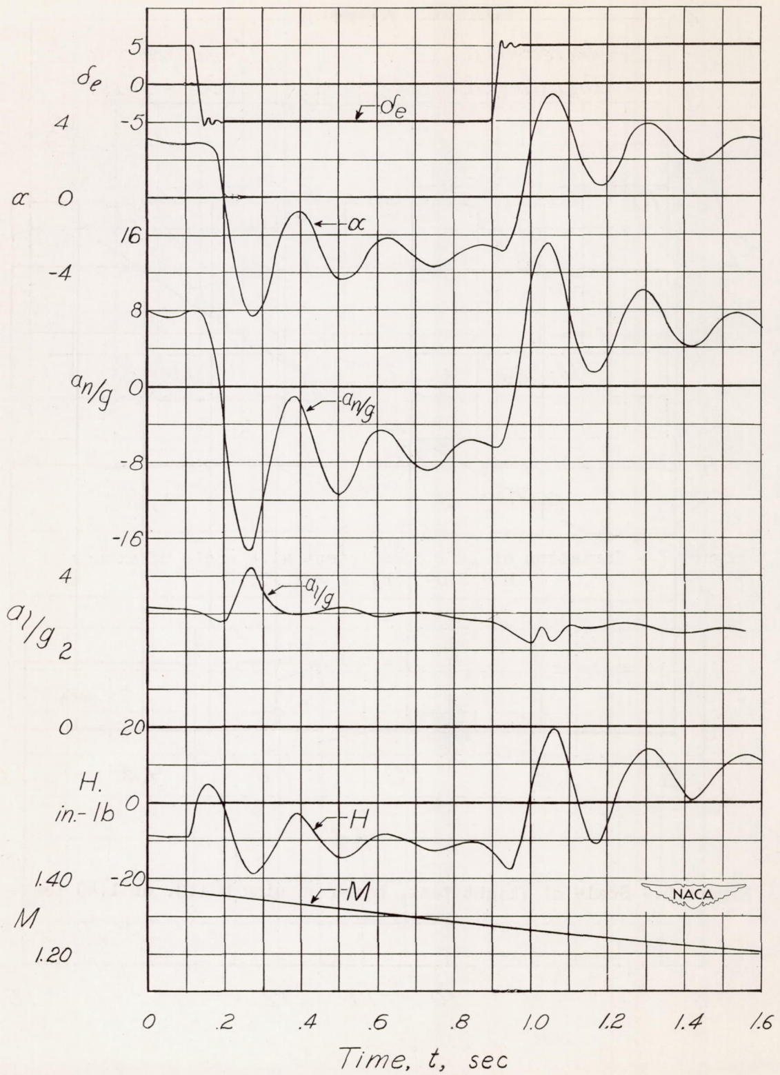
Figure 6.- Sample time history of model flight.
