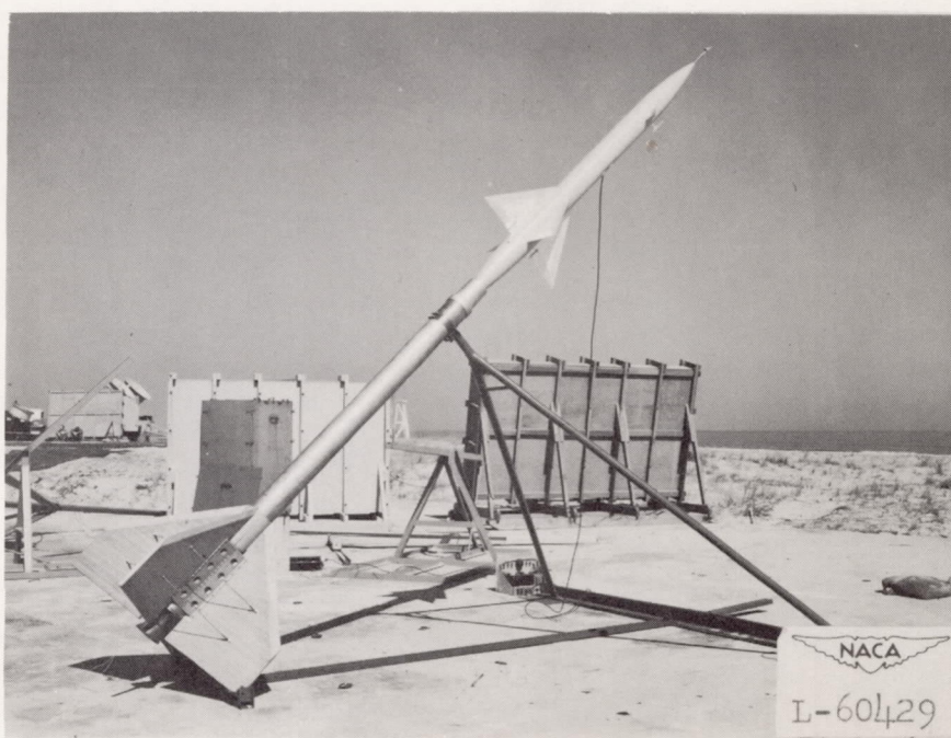
Figure 3.- Model alone and model-booster combination.
