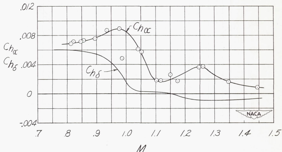
Figure 21.- Variation of hinge-moment-coefficient-slopes with Mach number.
